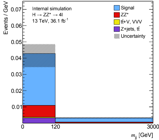
Figure 12.19 – Expected signal and background yields, and significances for the m_{jj} differential variable [215].
