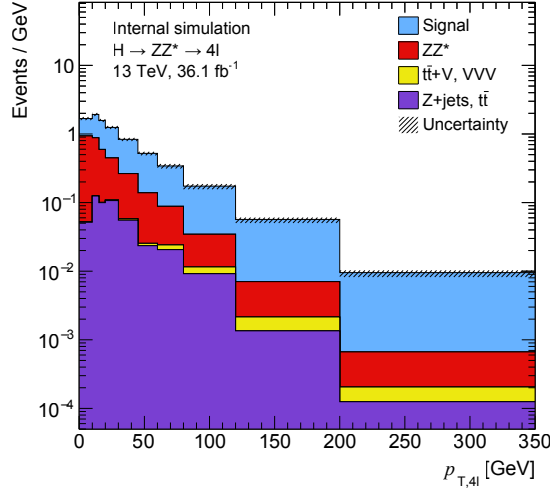
Figure 12.12 – Expected signal and background yields, and significances for the p_T^{4\ell} differential variable [215].
