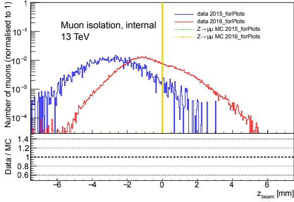
(a) z_{\text{beam}}
