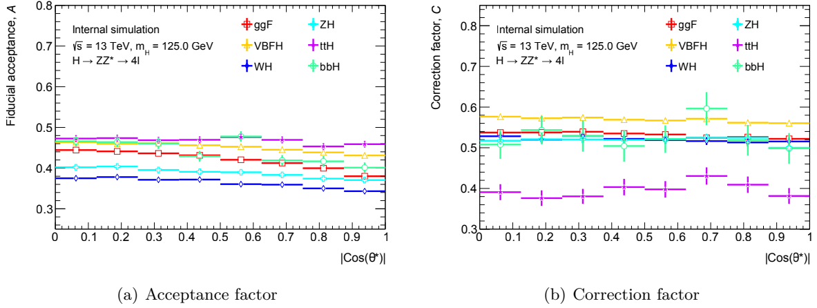
Figure 12.35 – Acceptance and correction factors per production mode, in bins of |\cos(\theta^*)| [215]. Errors are statistical only.
