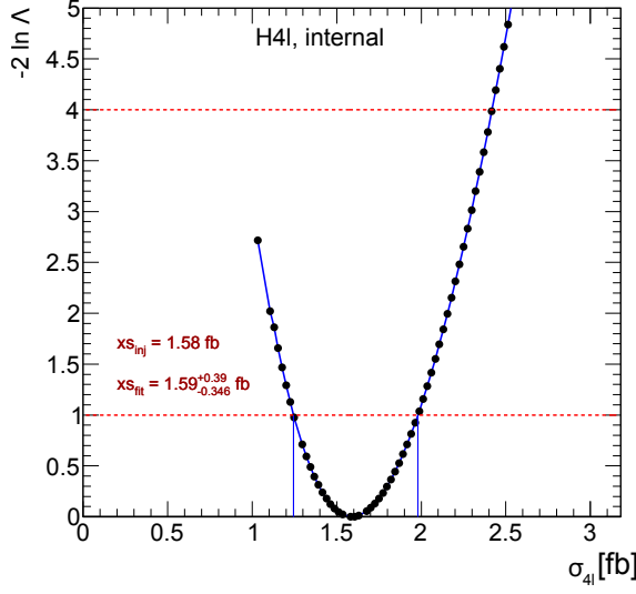
(a) \text{POI}_2^{4\mu+4e}
