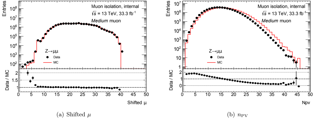
Figure 7.2 – Data-MC comparison of shifted \mu and n_{PV} after MC reweighting [69].
