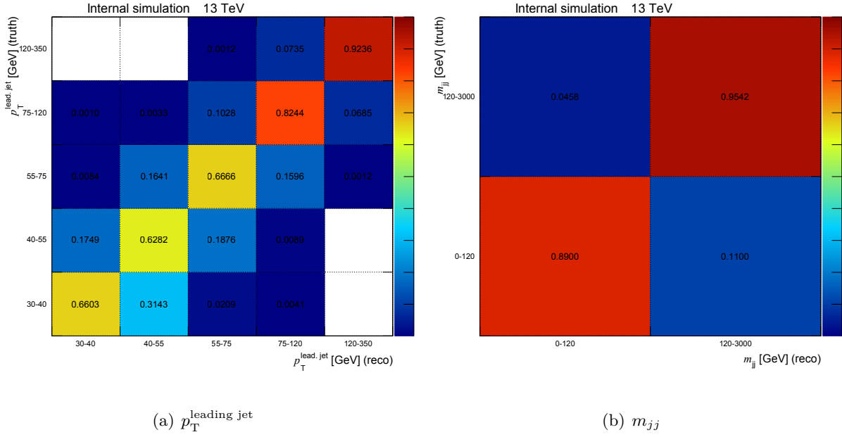
Figure 12.26 – p_T^{\text{leading jet}} and m_{jj} migration matrices [215].
