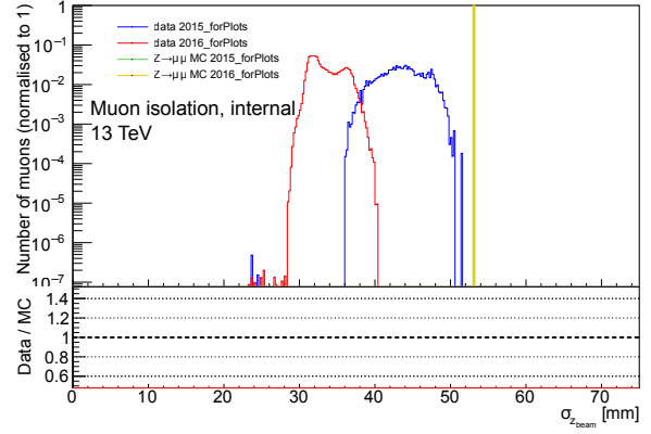
(b) \sigma_{z_{\text{beam}}}
