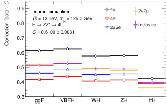
(d) \mathcal{C} factors using born leptons.
