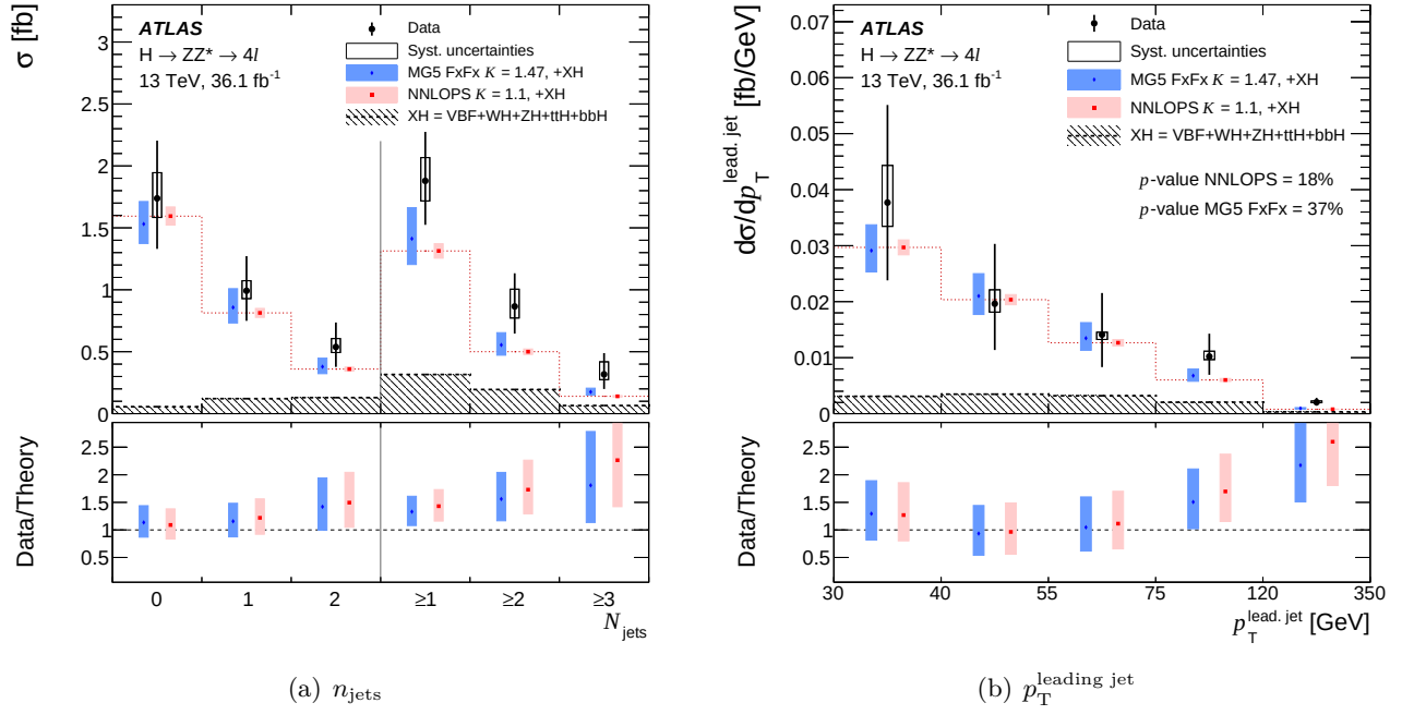
Figure 12.44 – Comparison of measured and expected differential fiducial cross section in bins of n_{\text{jets}} and p_{\text{T}}^{\text{leading jet}} [215].
