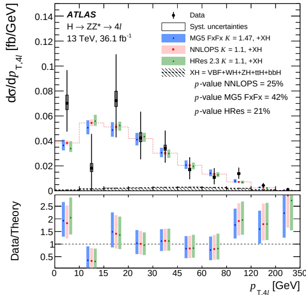
Figure 12.42 – Comparison of measured and expected differential fiducial cross section in bins of p_T^{4\ell} [215].
