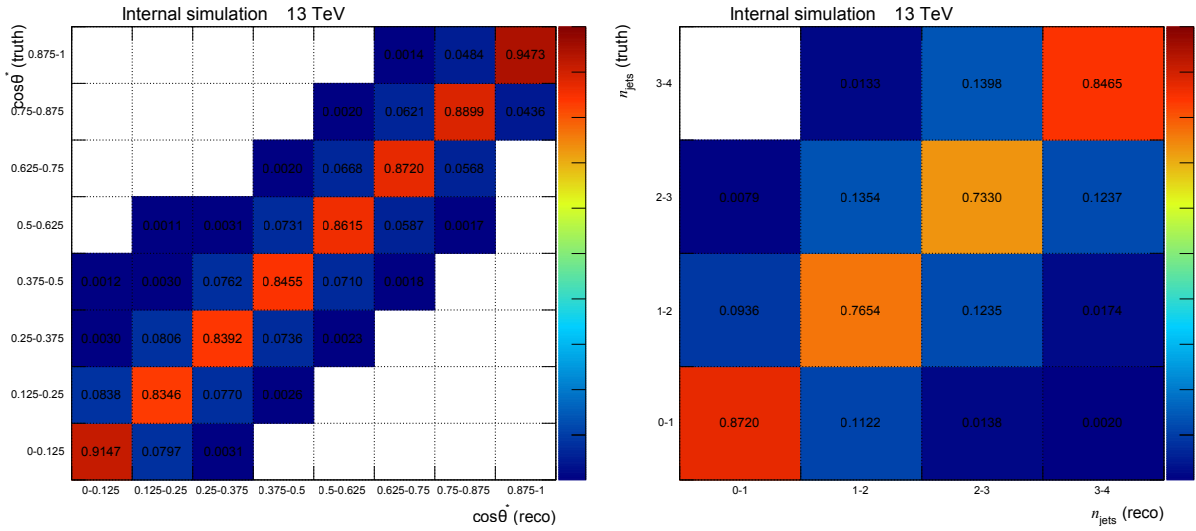
(a) |\cos(\theta^*)|
