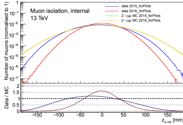
(c) z_{\text{p-vtx}}
