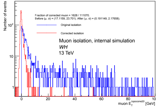
Figure 8.4 – Muon distribution of E_T^{\text{topocone20}} before (blue) and after (red) correction for close-by objects [69]. Only muons for which the correction was not nil are selected.
