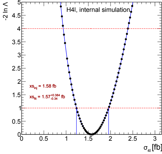
(a) \text{POI}_2^{4\mu+4e}
