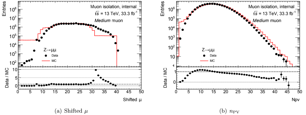
Figure 7.1 – Data-simulation comparison of shifted \mu and n_{PV} before MC reweighting.
