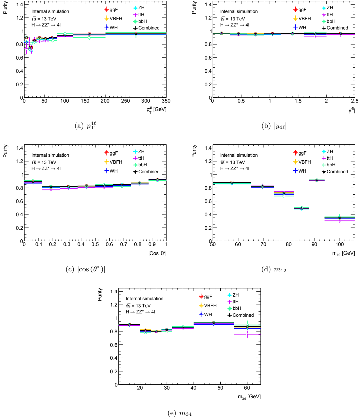
Figure 12.29 – Purity of production modes for variables (a) p_T^{4\ell} , (b) |y_{4\ell}| , (c) |\cos(\theta^*)| , (d) m_{12} and (e) m_{34} in each bin [215].
