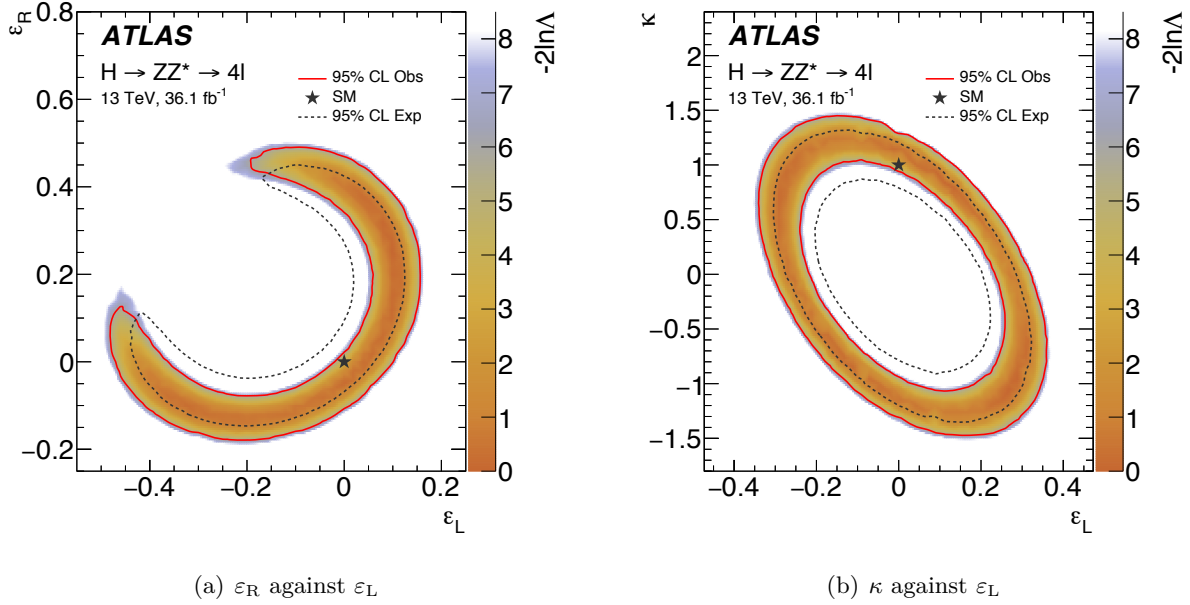
Figure 12.58 – Limits on contact-interaction decay to the left ( \varepsilon_L ) and right-handed ( \varepsilon_R ) leptons, and coupling to the Z bosons ( \kappa ) for the Higgs-to-four-lepton channel. The limits are presented for (a) \varepsilon_R against \varepsilon_L and (b) \kappa against \varepsilon_L ( \varepsilon_R = 0.48 \times \varepsilon_L ). The use of the double-differential cross-section measurements in bins of (m_{12}, m_{34}) improves the limits, especially in the region having \varepsilon_R > 0 and \varepsilon_L < 0 . Expected and observed limits are shifted, but no significant deviations with respect to the SM are found [215].
