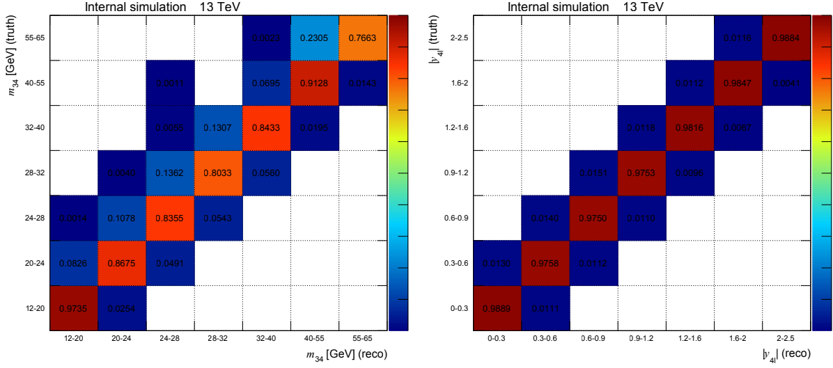
(a) m_{34}
