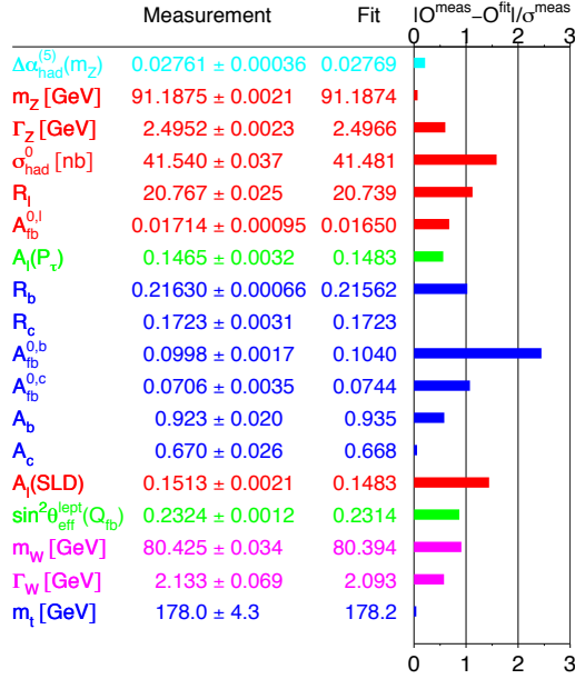
(a) Electroweak precision measurements from experiments at the LEP, SLC and Tevatron.
