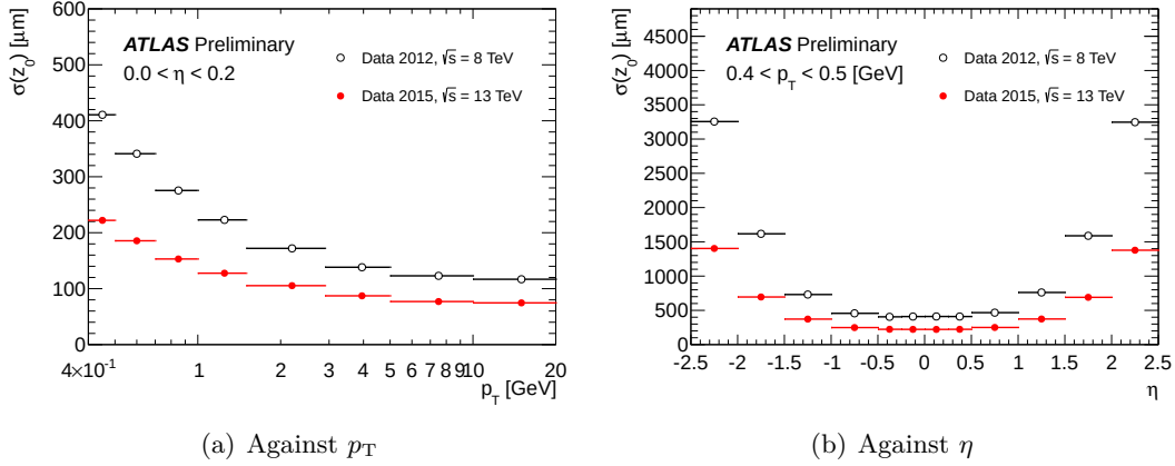
Figure 3.9 – Measured longitudinal impact parameter resolution in data as a function of (a) p_T and (b) \eta , compared between Run 1 and Run 2 [33].
