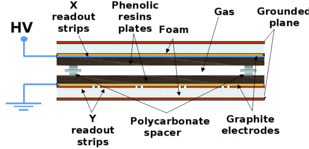
Figure 3.23 – Details of the design of a RPC chamber [52].
