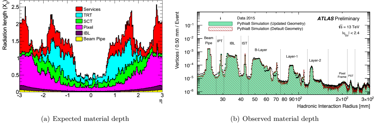
Figure 3.4 – Distribution of the material in the ID. (a) The expected material budget is given in X_0 units as a function of \eta [27]. (b) The material width is measured using 2015 data, and is expressed in hadronic interaction radius units [28].
