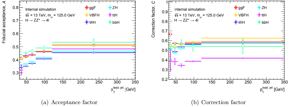
Figure 12.37 – Acceptance and correction factors per production mode, in bins of p_T^{\text{leading jet}} [215]. Errors are statistical only.
