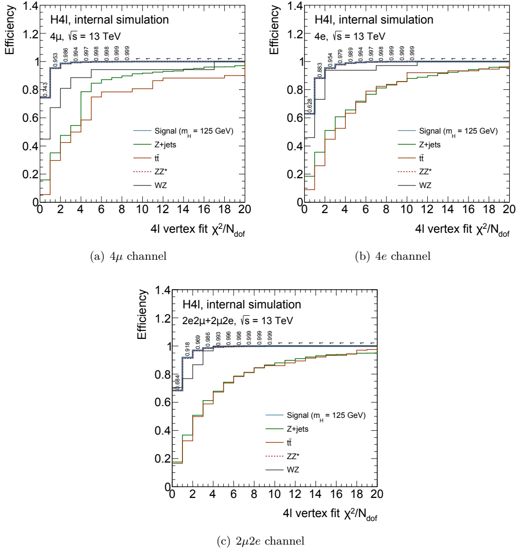
Figure 11.2 – 4\ell vertex cut efficiencies for the various decay channels. Efficiencies are presented for various cuts on the vertex \chi^2/N_{\text{dof}} , for signal and background events generated using simulation [198]. The two major contributions from the reducible background ( t\bar{t} and Z+\text{jets} ) are suppressed by the new cut, for a relative stable signal efficiency. The WZ and ZZ^* background contributions are not strongly impacted by the new cut, as the vertices have same signatures as for the signal.
