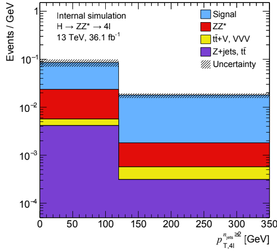
Figure 12.49 – Expected signal and background yields, and significances for the p_T^{4\ell} (n_{\text{jets}} \geq 2) differential variable [215].
