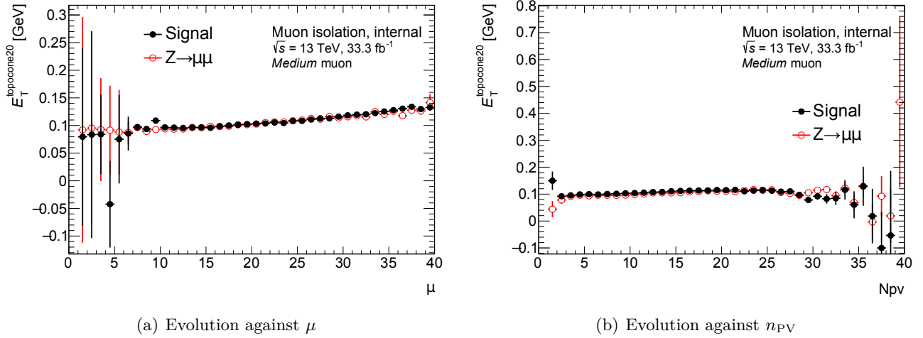
Figure 7.14 – Evolution of topoetcone20 with pile-up: as a function of (a) \mu and (b) n_{PV} [69]. The distributions are flat, which proves the adequate correction for pile-up.
