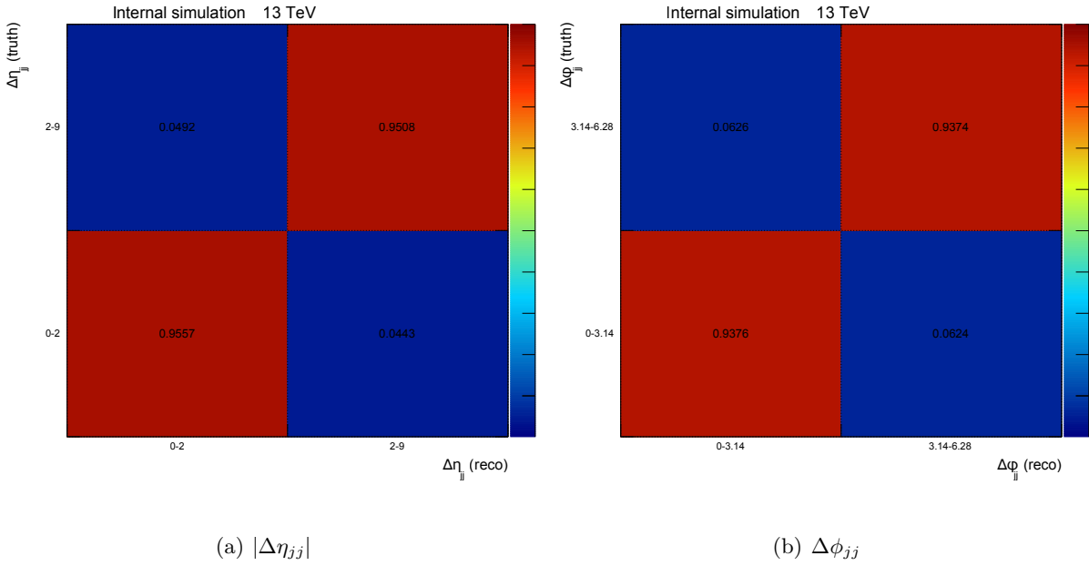
Figure 12.27 – |\Delta\eta_{jj}| and \Delta\phi_{jj} migration matrices [215].
