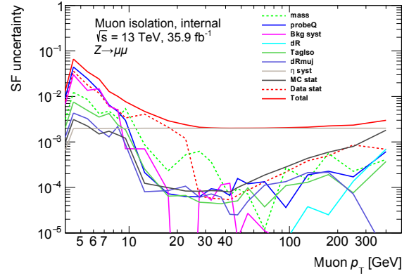
(b) Loose
