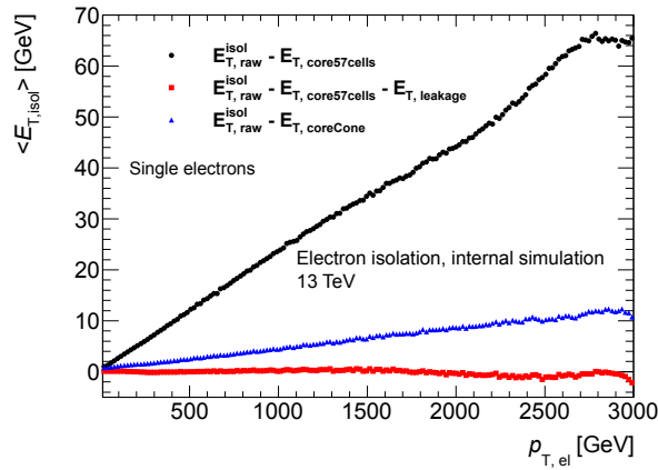
Figure 5.8 – Evolution against p_{\text{T}}^e of E_{\text{T}}^{\text{topocone20}} for electrons with and without leakage correction [69]. The electrons are taken from single electron MC. The uncorrected and corrected variables are plotted in black and red. As a comparison, the muon-like core energy subtraction (coreCone, or E_{\text{T}}^{\text{topocore}} ) is represented in blue.
