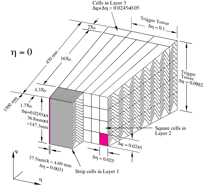
Figure 3.13 – Geometry of the electromagnetic calorimeters [14].
