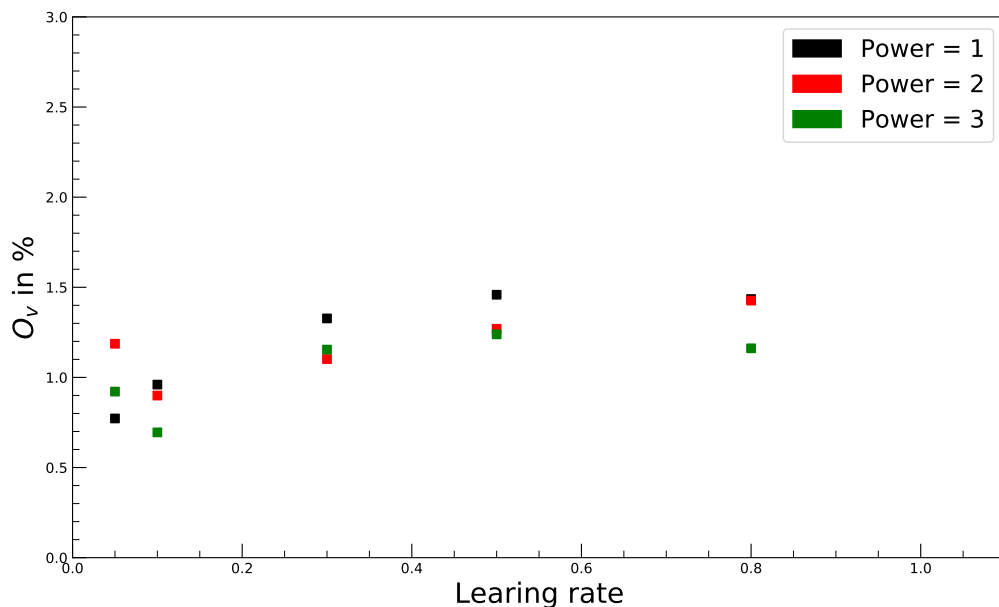
Figure A.8: Overtraining of RNNs as a function of the learning rate for different powers of the decaying polynomial. (ADAM)
