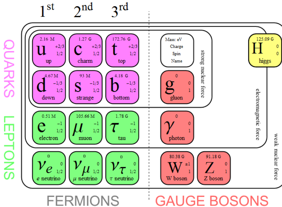
Figure 2.1: Schematic depiction of the SM [6]. The masses of the massive particles in the SM are taken from [7]. The electroweak force is divided into the electromagnetic force and the weak nuclear force.
