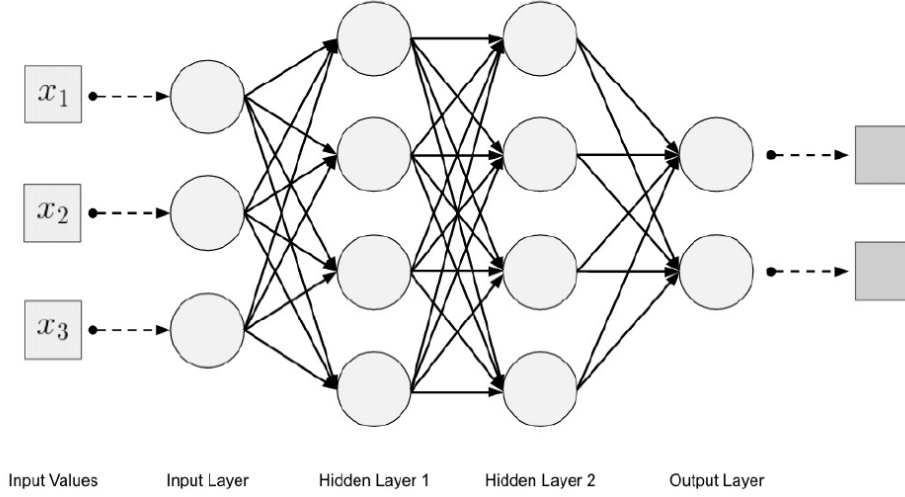
Figure 5.1: Schematic structure of a deep neural network with fully connected layers [38]. The input values of the given task x_i are fed into the neurons (depicted as circles) of the input layer and processed in the hidden layers. The weights which connect neurons located at different layers are represented by a solid arrow. In the output layer, all information is combined and predictions (depicted as dark squares) about the classes are made.
