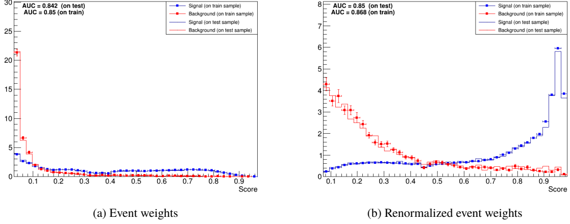
Figure 6.3: The difference in classification between a Neural Network trained with and without renormalization event weights.
