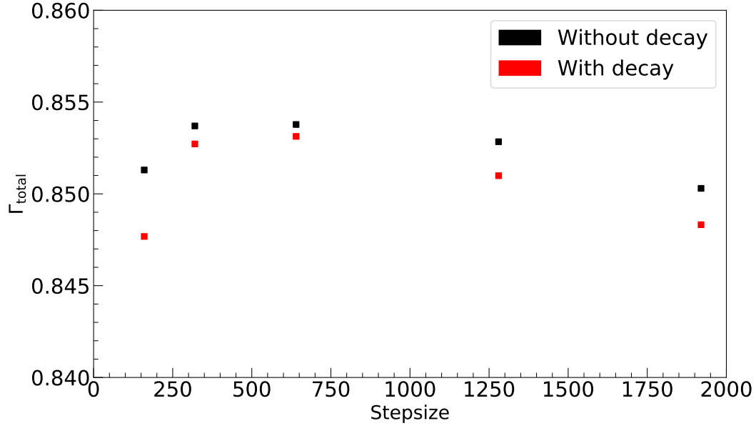
Figure 7.16: Dependence of the AUC on the stepsize chosen for the cyclic learning rate decay.
