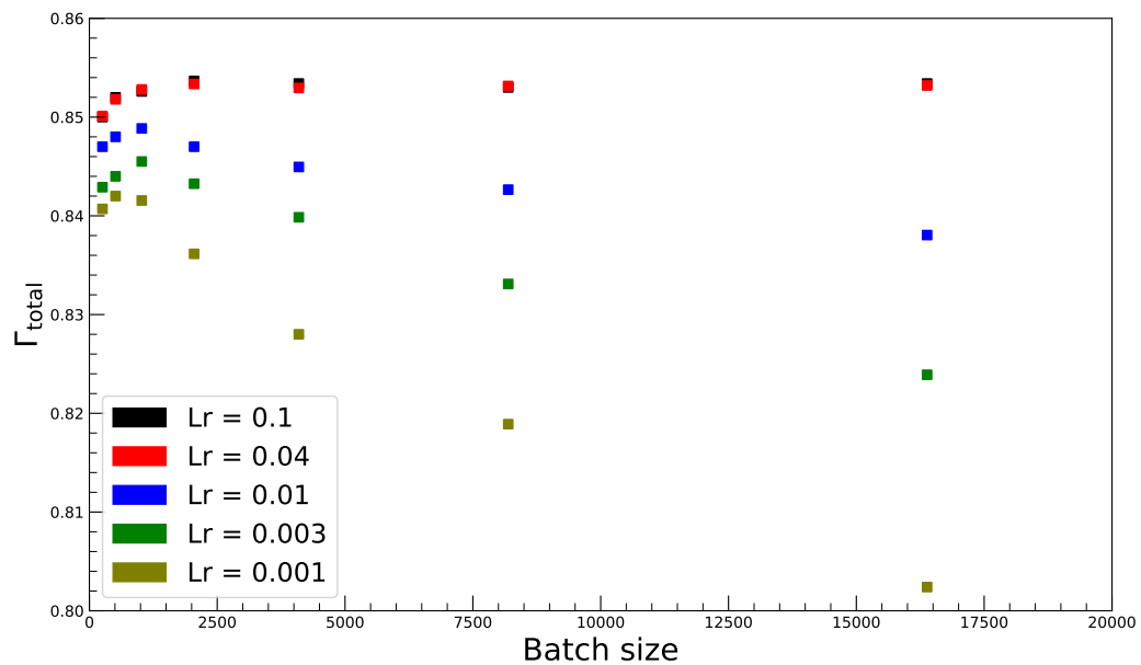
Figure 7.9: The AUC as a function of the batch size for different learning rates Lr . The Neural Networks are trained using SGD.
