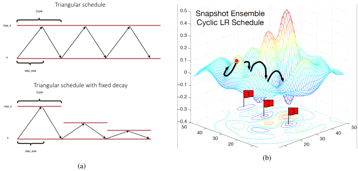
Figure 7.13: a) The learning rate schedule for cyclic learning rate decay with (bottom) and without (top) additional decay of the maximum learning rate “max_lr”. b) Topology of a loss function for which cyclic learning rate decay can improve the performance of a Neural Network. The flags 1, 2 indicate the position of local minima whereas flag 3 indicates the position of the global minimum [62, 63].
