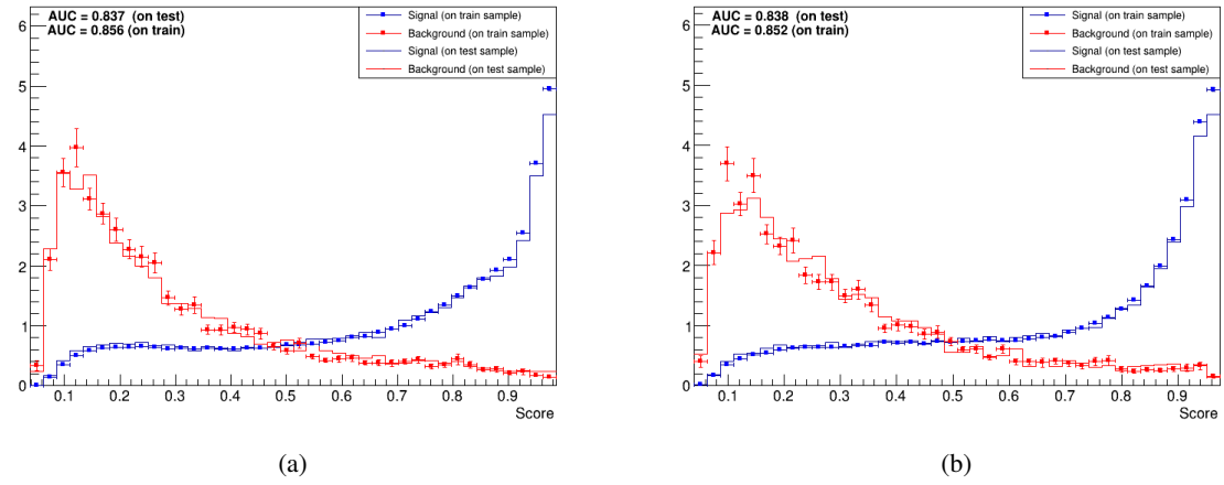
Figure A.6: Observed Neural Network scores for the RNNs trained with the background dataset containing even event numbers (a) and on the background dataset constraining odd event numbers (b).
