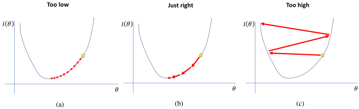
Figure 7.10: Training of a Neural Network trained with a too low (a), a too high (c) and a polynomial decaying learning rate (b) [60].
