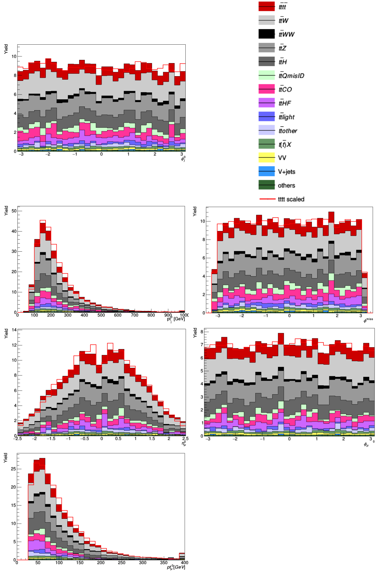
Figure A.5: Input features of the Recurrent Neural Network. The last bin of all diagrams additionally contain all events above the maximum x-axis range (overflow).
