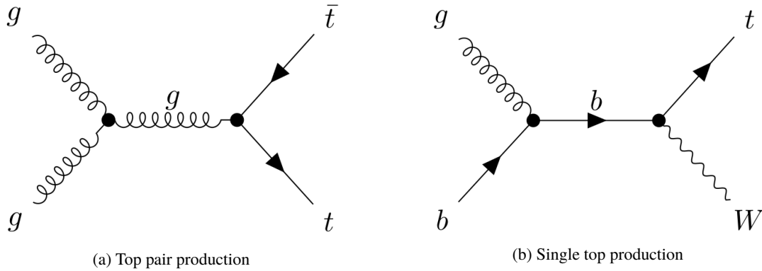
Figure 2.2: The two different categories of top production.
