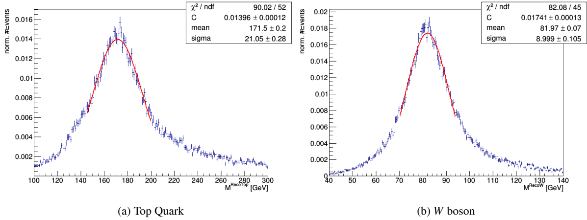
Figure 7.32: Mass distributions of the reconstructed, truth-matched top quarks (a) and W bosons (b).
