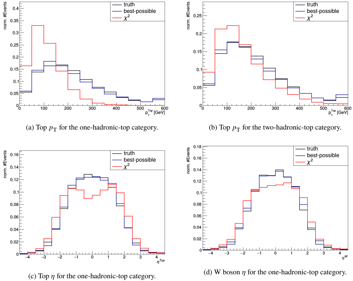
Figure 7.35: Kinematic distributions for the truth and reconstructed top quarks and W bosons. The last bin in all distributions contains additionally the events which fall into bins above the maximum x-axis range.
