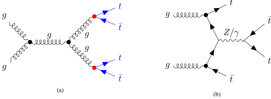
Figure 2.3: Two possible production processes of t\bar{t}t\bar{t} in the SM.
