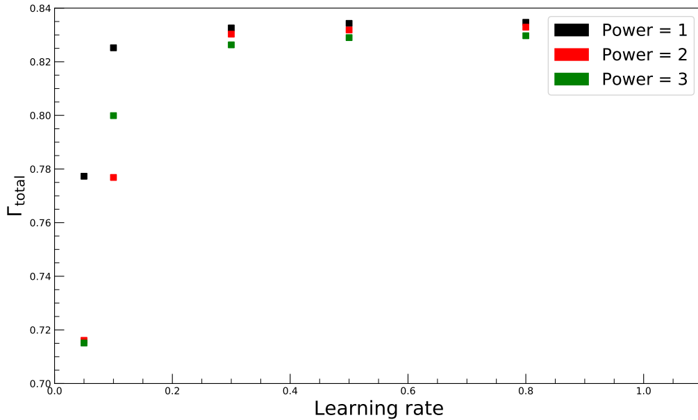
Figure 7.26: Average AUC of RNNs as a function of the learning rate and the power of the polynomial used for learning rate decay. The average includes the AUCs of the 2 best-performing Neural Networks with different batch sizes.
