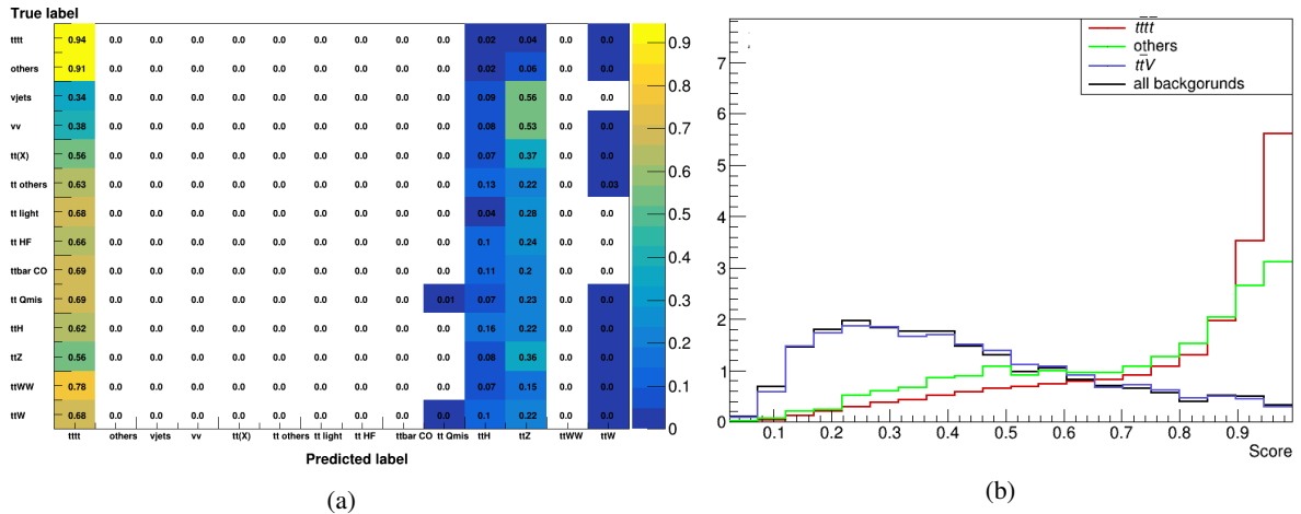
Figure 7.22: The confusion matrix (a) and the Neural Network score (b) for the multi classification with 14 classes.
