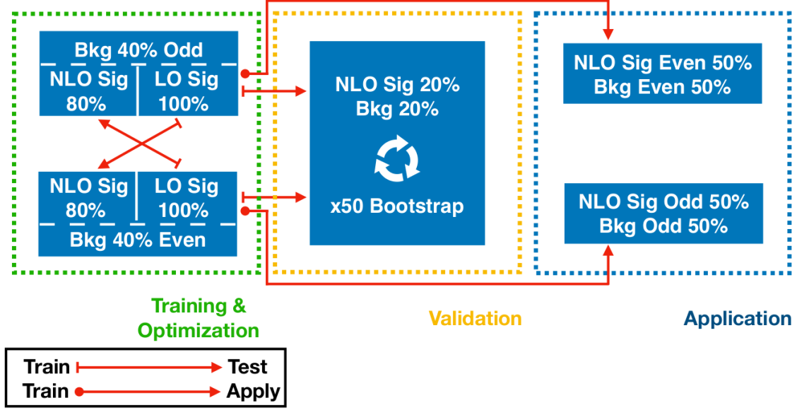
Figure 6.1: Splitting strategy applied to ensure an unbiased estimation of both, overtraining and performance (plot by Ö. Oğul Oncel).
