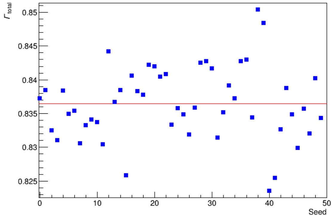
Figure 7.29: AUCs observed by using the bootstrap method on the validation set. The seed quoted (divided by 365) is the random seed used to generate the different resampled versions of the validation set. The red line indicates the mean of all observed AUCs.
