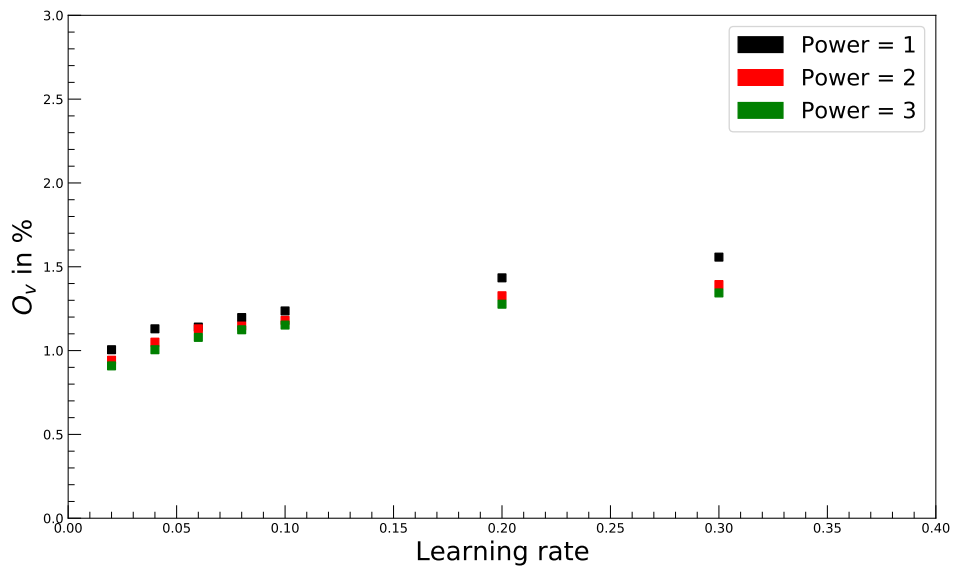
Figure 7.12: The overtraining for FNNs trained using polynomial learning rate decay (SGD).
