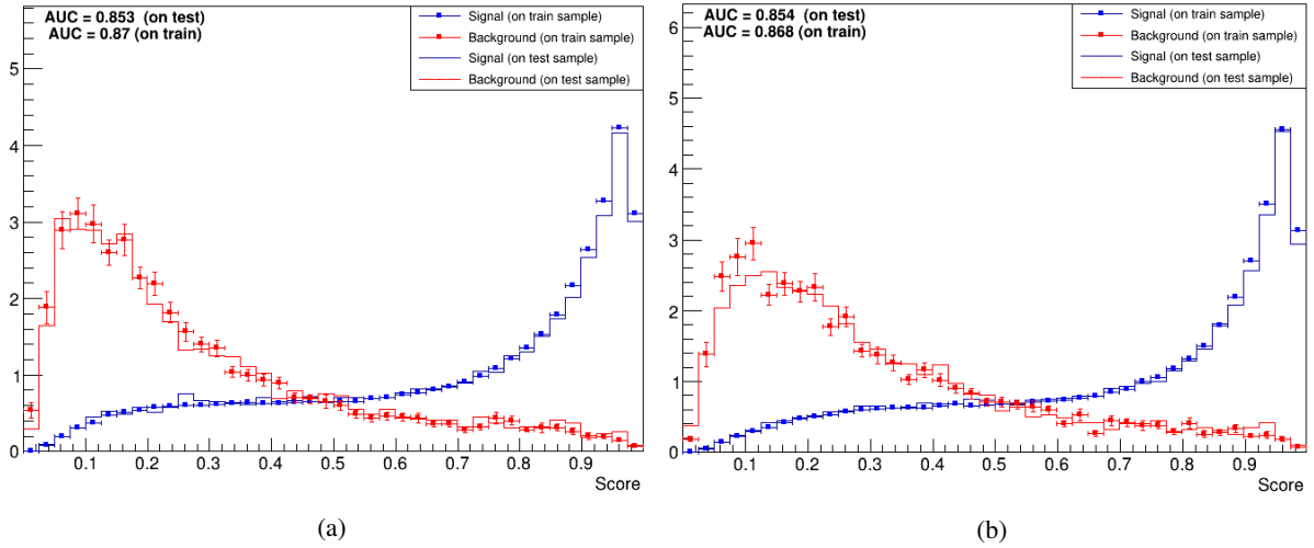
Figure 7.19: Neural Network scores for the Neural Network trained with the background dataset containing even event numbers (a) and on the background dataset containing odd event numbers (b).
