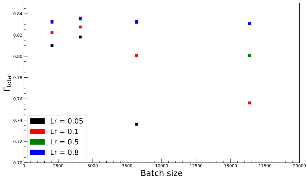
Figure 7.27: The AUC as a function of the batch size for different the learning rates.
