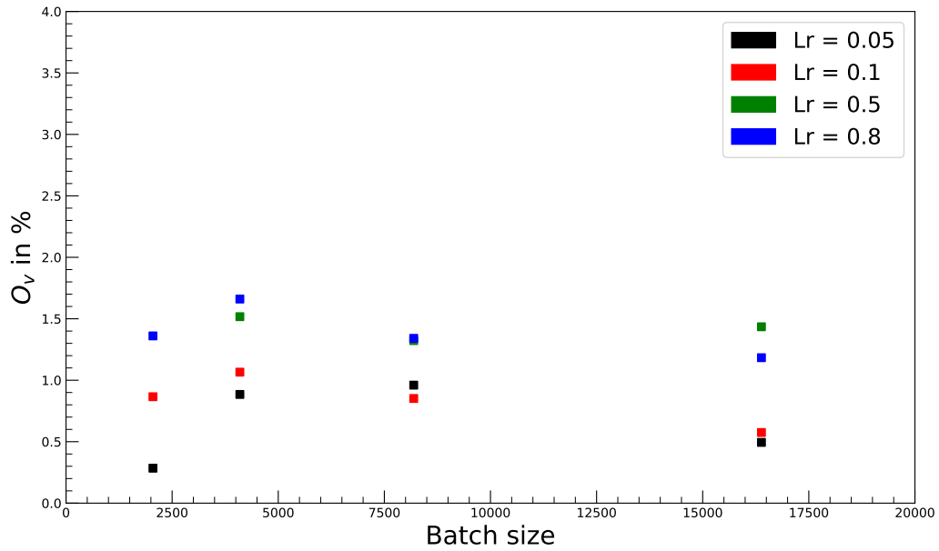
Figure A.7: The overtraining of RNNs as a function of the batch size and the learning rate. (ADAM)
