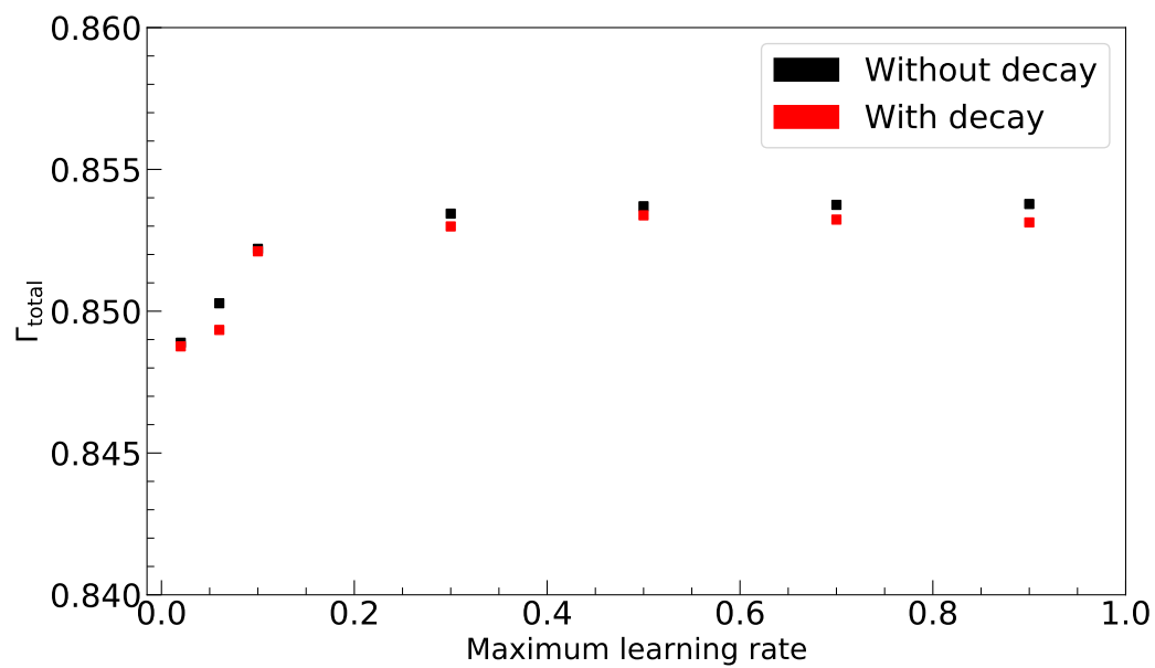
Figure 7.15: Observed AUCs for different maximum learning rate using cyclic decay with and without additional decay.
