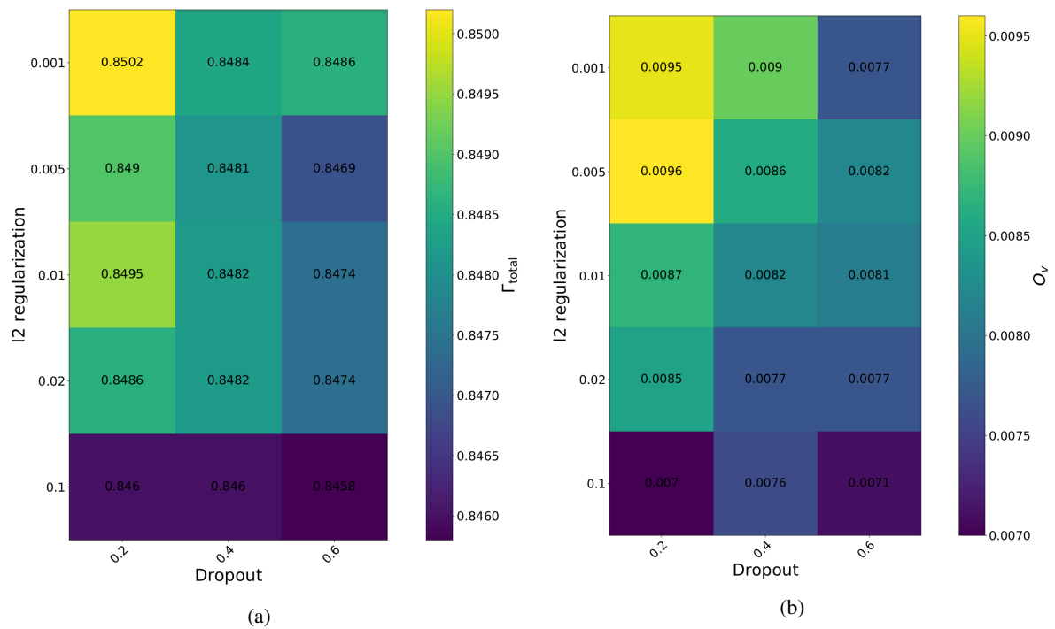
Figure 7.18: Dependence of the AUC (a) and the overtraining (b) for different Dropout probabilities and Ridge ( \ell_2 ) regularization.
