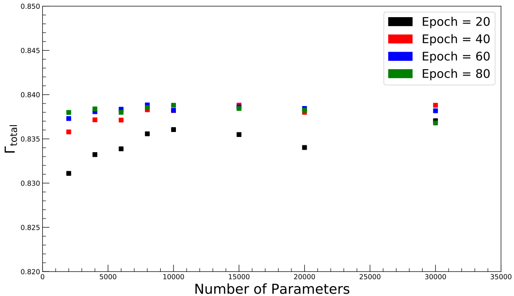
Figure 7.25: The average AUC for different RNNs configurations. The training is stopped after 20, 40, 60, or after 80 epochs. The average includes the AUCs of the 4 best-performing Neural Networks of different depth.
