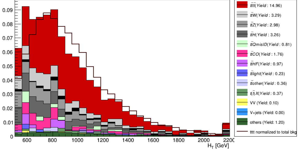
Figure 7.28: The H_T distribution after applying a cut (optimized on the significance) to the RNN score obtained for the training on the background dataset containing even event numbers. The last bin additionally contains all events with H_T > 2200 GeV.
