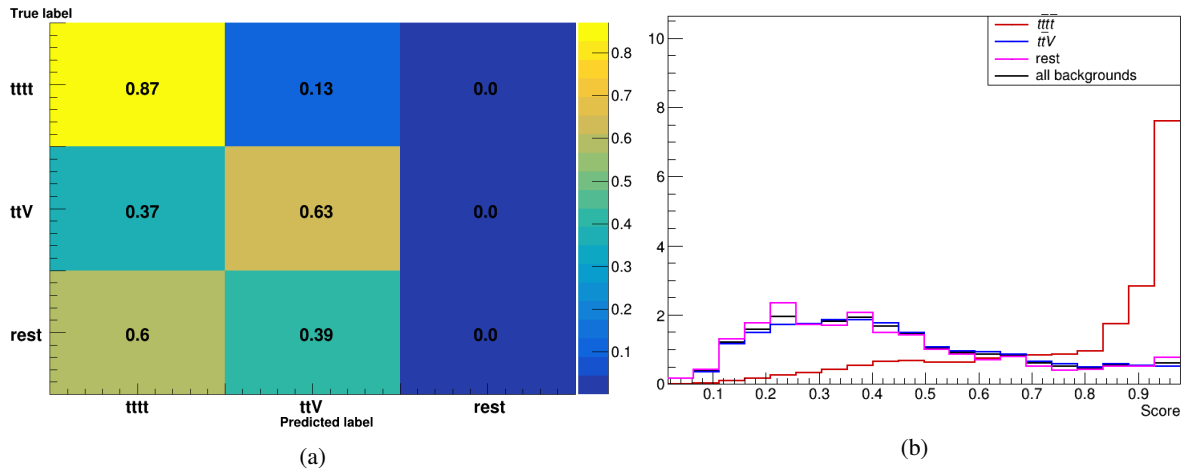
Figure 7.24: The confusion matrix (a) and the Neural Network score (b) for the multi classification with 3 classes.
