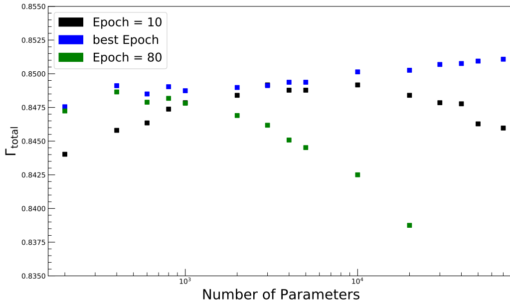
Figure 7.1: The averaged AUCs of FNNs with different number of parameters where the training is stopped after 10, 80 and at the best-performing epoch. The average includes the AUCs of the 4 best-performing Neural Networks of different depth.
