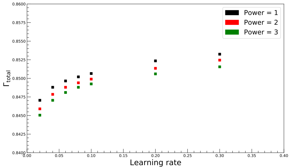
Figure 7.11: AUCs for FNNs trained using polynomial learning rate decay (SGD).
