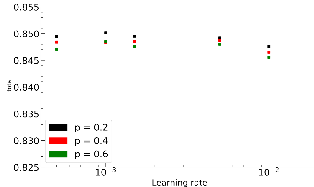
Figure 7.17: AUCs as a function of learning rates for 3 choices of p , the Dropout probability. (ADAM)
