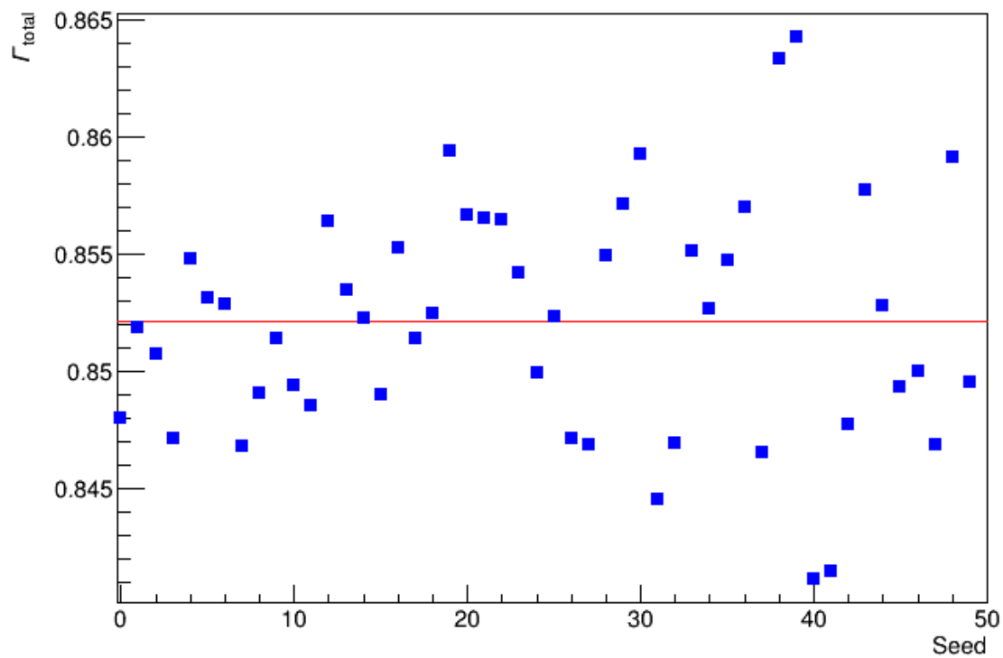
Figure 7.21: AUCs observed by using the bootstrap method on the validation set. The seed quoted (divided by 365) is the random seed used to generate the different resampled versions of the validation set. The red line indicates the mean of all observed AUCs.
