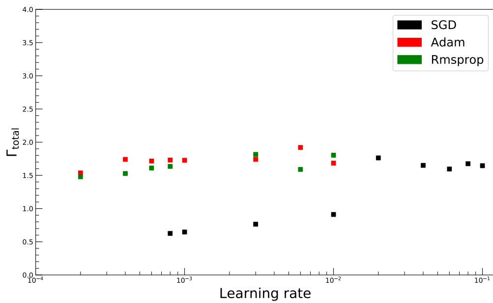
Figure 7.8: The overtraining of FNNs as a function of the learning rates for three optimization algorithms.
