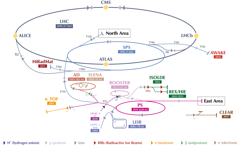
Figure 3.1: The accelerator complex of CERN including the LHC. The accelerator chain for the protons is shown as well as the four major experiments [23].
