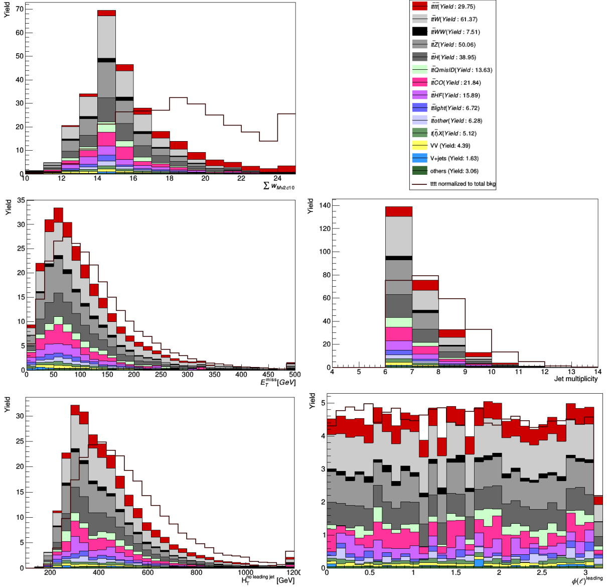
Figure A.1: High-level input features of the Feedforward Neural Network. The last bin of all diagrams additionally contain all events above the maximum x-axis range (overflow).
