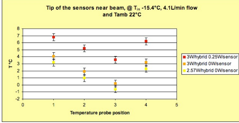
Figure 4.23: Measurements of the temperatures on the tips of the sensors near the beam with the coolant at T_{in} = -15.4^\circ\text{C} and 4.1l/min flow. The temperature outside the box was 22^\circ\text{C} . The colours correspond to various thermal power simulating the hybrids and sensors.
