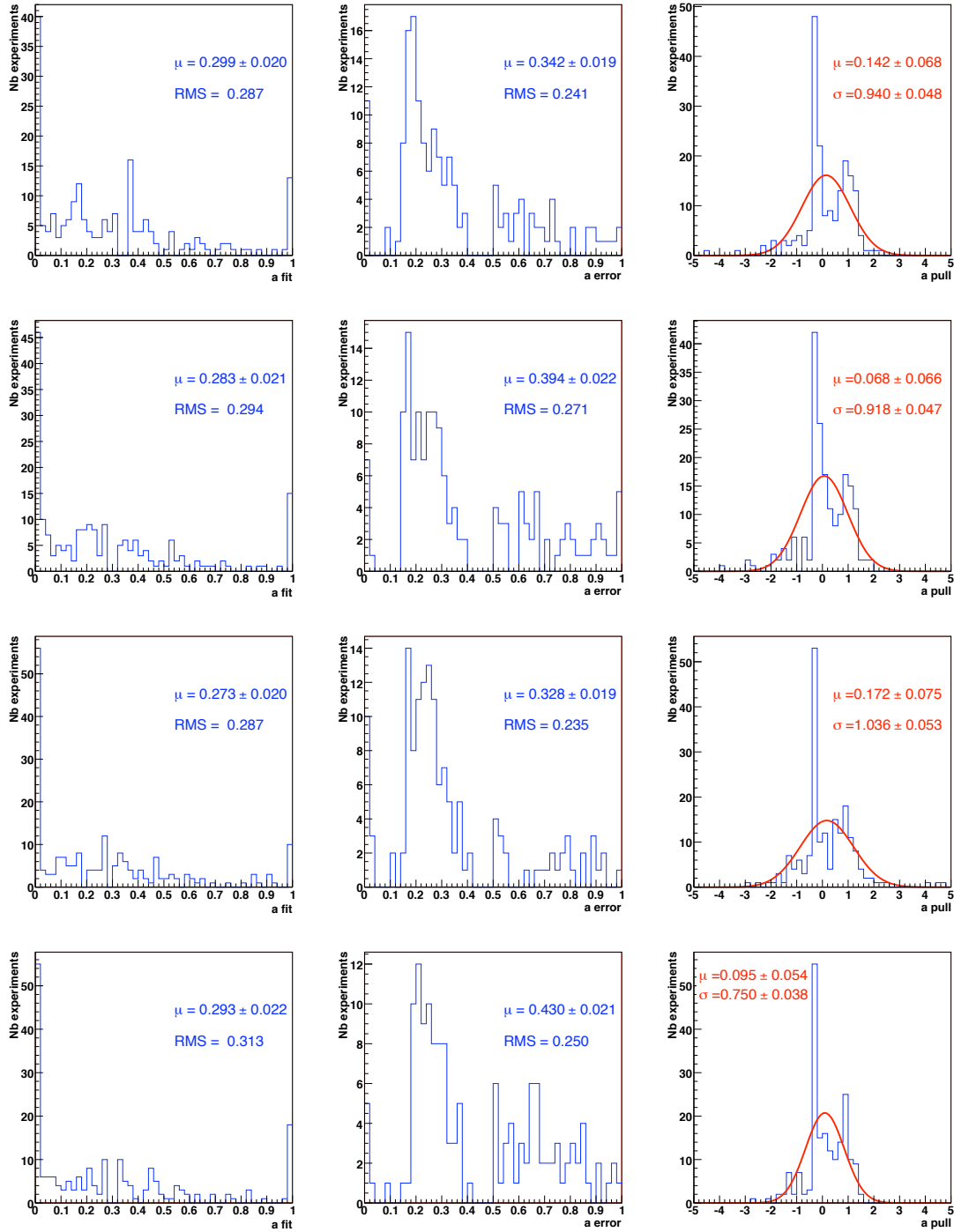
Figure B.6: a likelihood fit output, error and pull distributions for 200 experiments using a luminosity of 10\text{fb}^{-1} , B/S=3.33 and fixing \theta at 10° (first row) 20° (second row), 30° (third row) and 50° (fourth row). The pull distribution is fitted with a single Gaussian.
