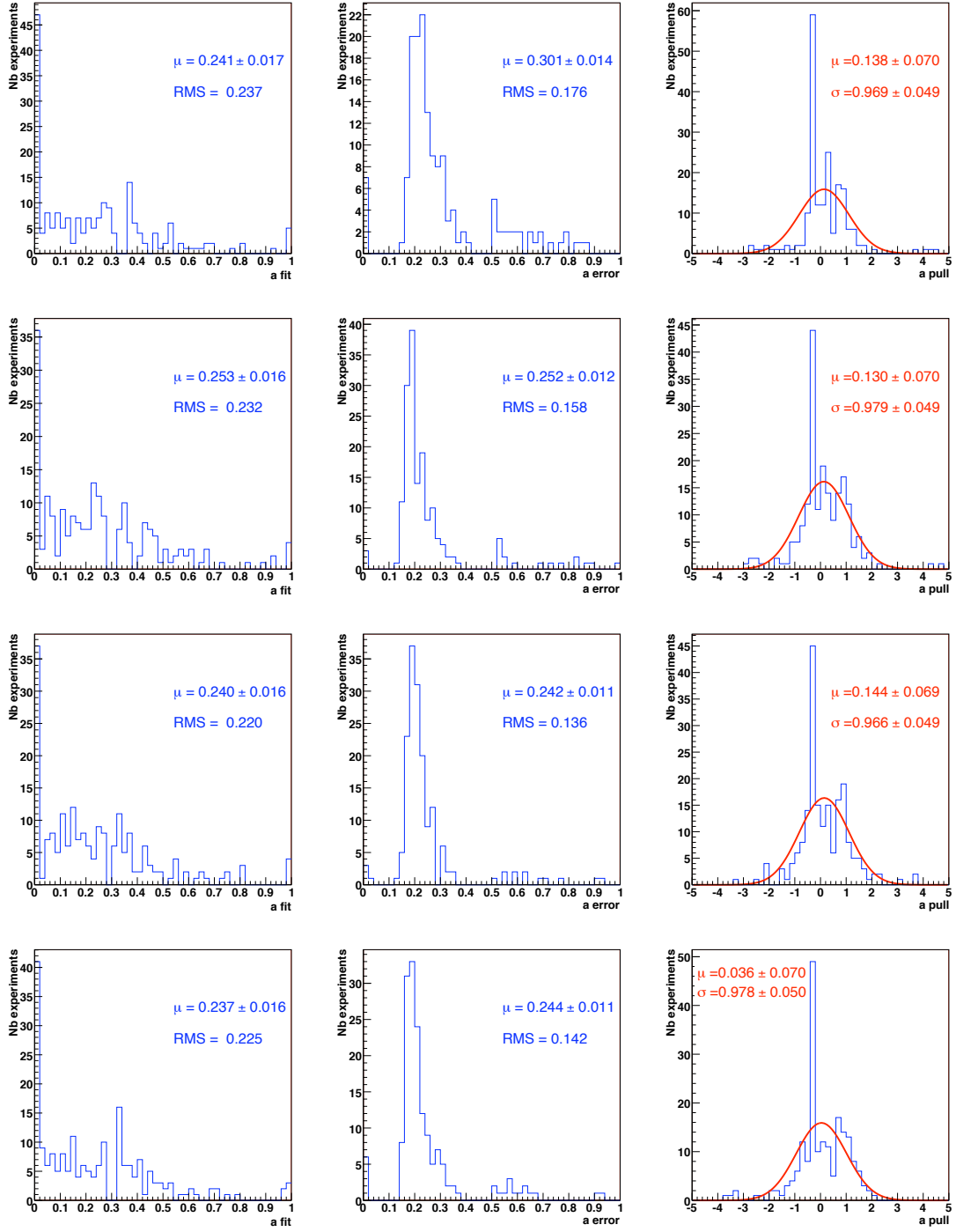
Figure B.5: a likelihood fit output, error and pull distributions for 200 experiments using a luminosity of 10 \text{ fb}^{-1} , B/S=1 and fixing \theta at 10° (first row) 20° (second row), 30° (third row) and 50° (fourth row). The pull distribution is fitted with a single Gaussian.
