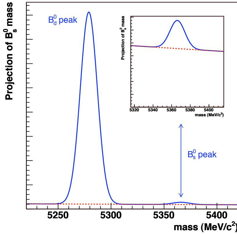
Figure 5.24: Mass distributions of B_d^0 and B_s^0 after one year of run at 2\text{ fb}^{-1} . The B/S ratio considered here is 3.33 in a mass window of \pm 2\sigma around the B_s^0 nominal mass after the L0 trigger. The red dashed line corresponds to the b\bar{b} background level.
