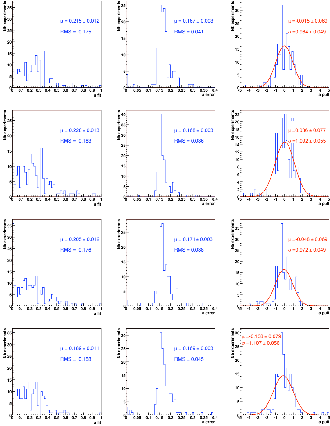
Figure B.4: a likelihood fit output, error and pull distributions for 200 experiments using a luminosity of 10\text{fb}^{-1} , B/S=0 and fixing \theta at 10° (first row) 20° (second row), 30° (third row) and 50° (fourth row). The pull distribution is fitted with a single Gaussian.
