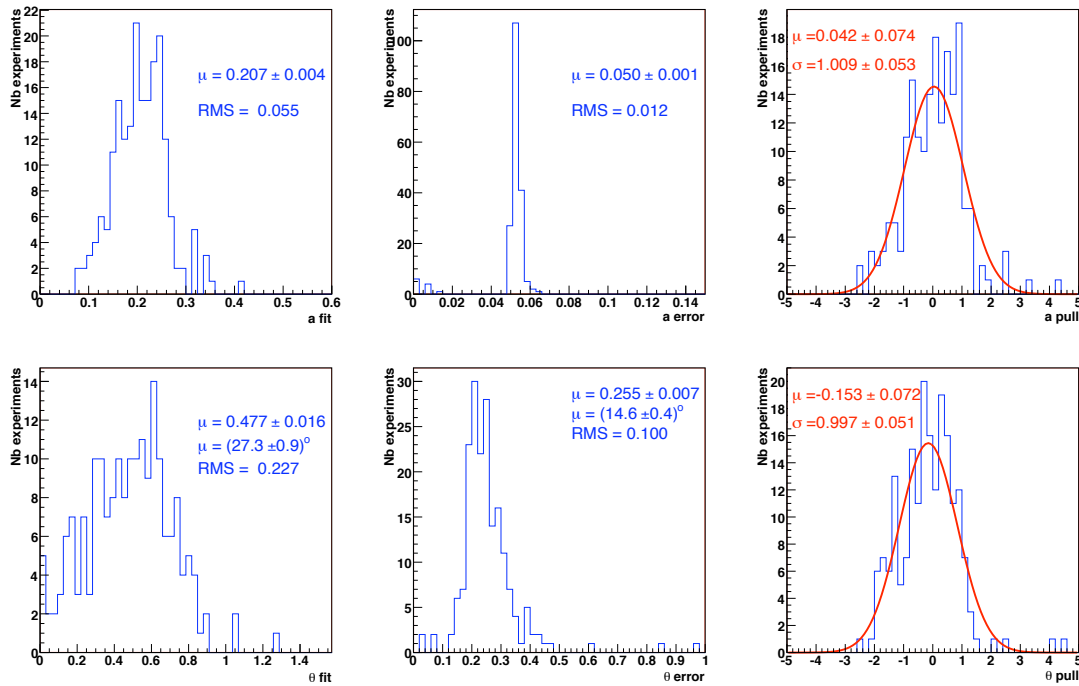
Figure B.11: a (top) and \theta (bottom) likelihood fit output, error and pull distributions for 200 experiments using a luminosity of 100\text{fb}^{-1} and B/S=0. The pull distribution is fitted with a single Gaussian.
