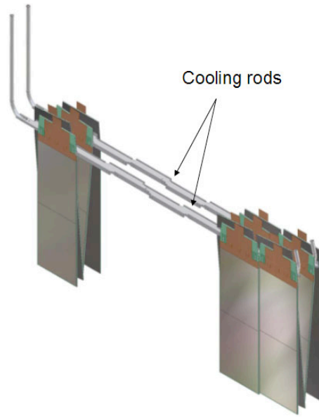
Figure A.3: Design of the cooling rods.
