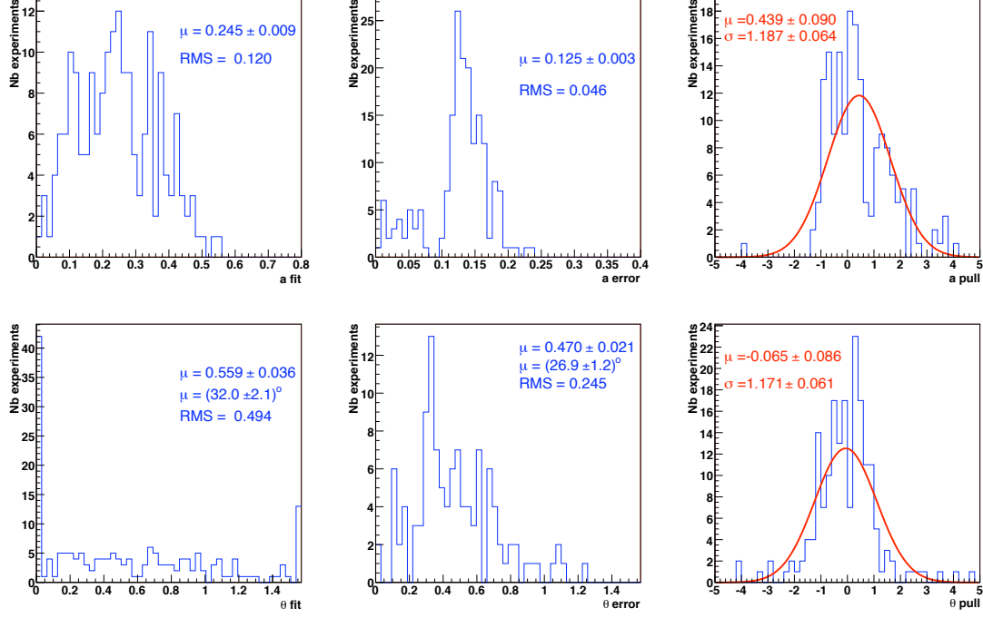
Figure B.9: a (top) and \theta (bottom) likelihood fit output, error and pull distributions for 200 experiments using a luminosity of 50 \text{ fb}^{-1} and B/S=3.33 . The pull distribution is fitted with a single Gaussian.
