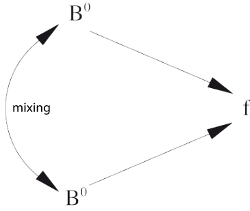
Figure 1.3: Schematic of the mixing between B_q^0 and \bar{B}_q^0 decaying in the same f final state.
