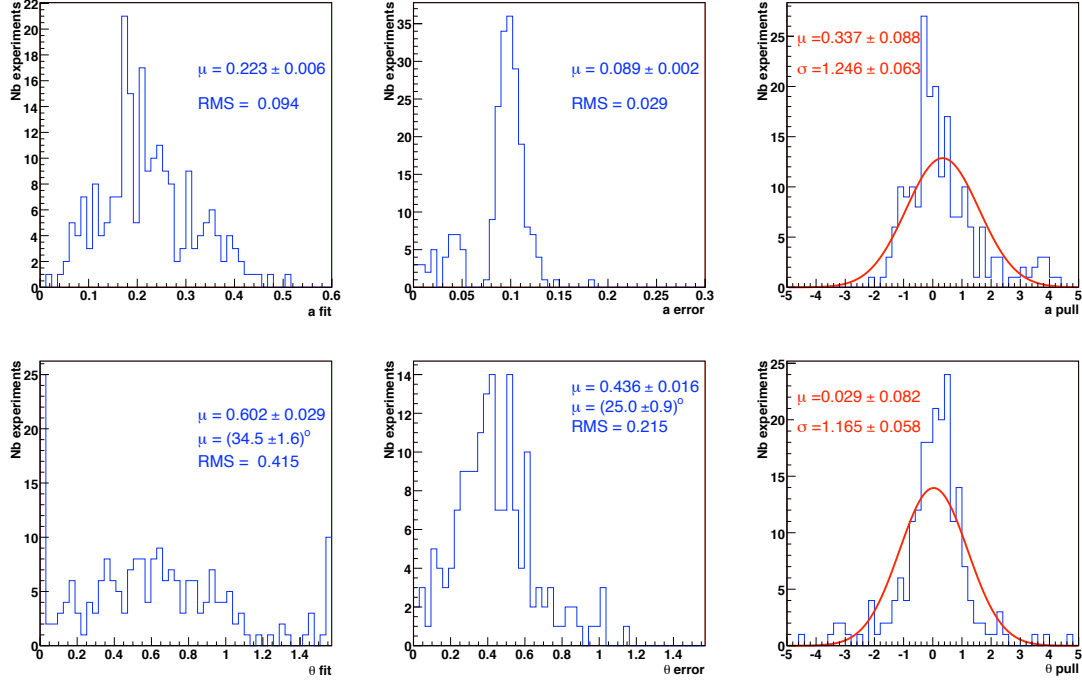
Figure B.13: a (top) and \theta (bottom) likelihood fit output, error and pull distributions for 200 experiments using a luminosity of 100\text{fb}^{-1} and B/S=3.33 . The pull distribution is fitted with a single Gaussian.
