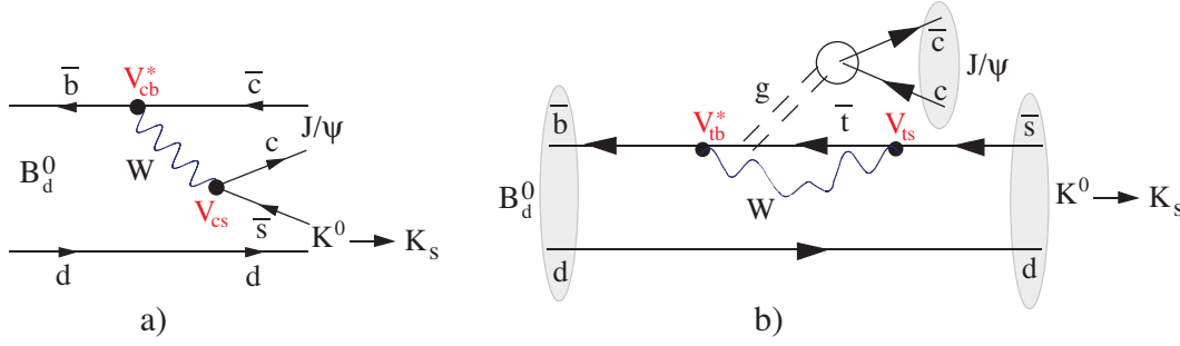
Figure 1.5: Feynman diagrams contributing to B_{d,s}^0 \rightarrow J/\psi K_s^0 . a) the tree (current-current) diagram and b) the penguin one. The dashed lines in the penguin topology represent a colour-singlet exchange.
