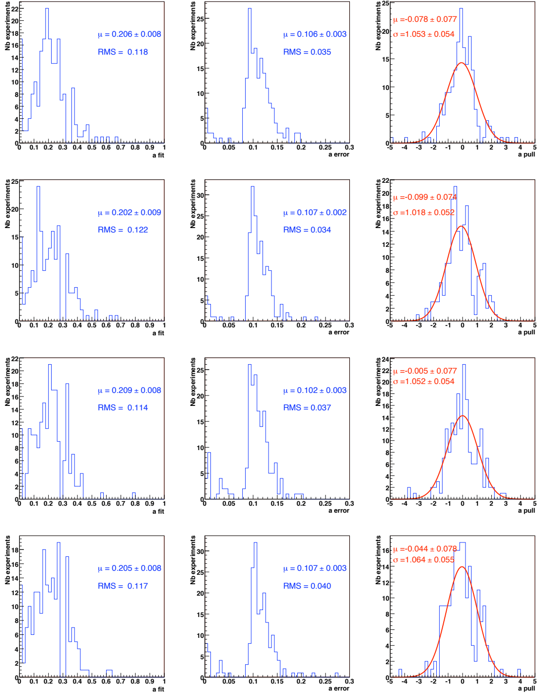
Figure B.10: a likelihood fit output, error and pull distributions for 200 experiments using a luminosity of 50 \text{ fb}^{-1} , B/S=3.33 and fixing \theta at 10° (first row) 20° (second row), 30° (third row) and 50° (fourth row). The pull distribution is fitted with a single Gaussian.
