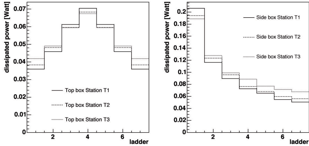
Figure 4.12: The power dissipation in the various ladders at 10°C after 10 years of operation for a bias voltage of 300V.
