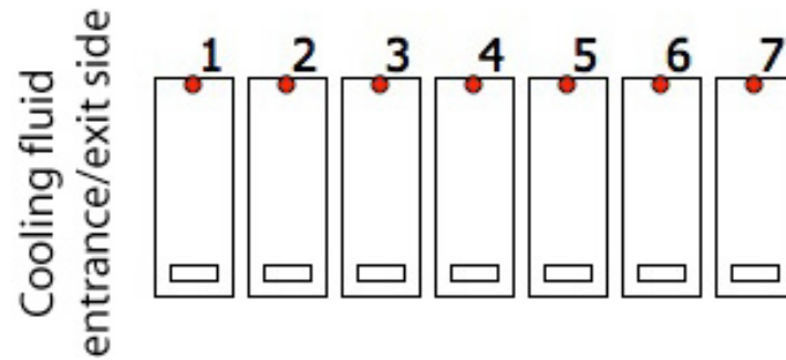
Figure 4.24: This figure shows the position of the temperature probes as discussed in Fig. 4.25. While temperature probes 1-5 are glued onto the CF-support directly, probes 6 and 7 are glued to a glass or silicon plate that is equipped with a resistive coil heater simulating the Si-sensor dissipation.
