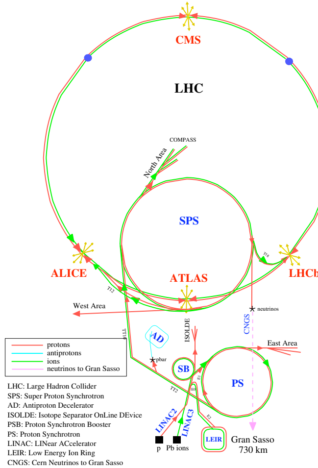
Figure 2.2: The CERN accelerator complex chain. Picture from [33]
