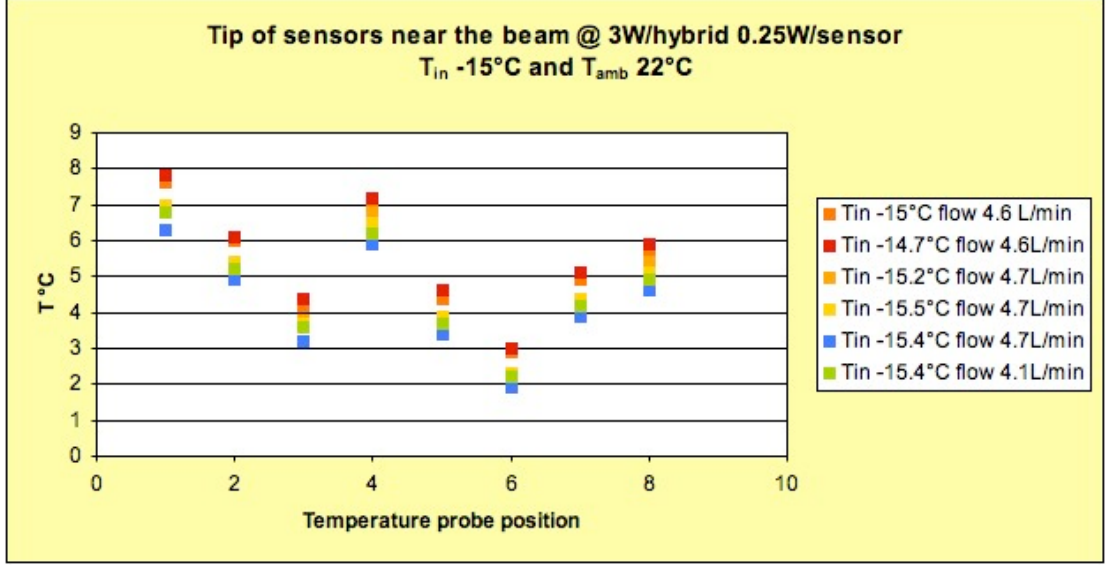
Figure 4.21: Measurements of the temperatures on the tip of the sensors on ladders 1 to 8, with a dissipation of 3 W per hybrid, 0.25 W per “sensor” and for an outside temperature of 22°C. The different colours correspond to different temperatures and flows of the coolant.
