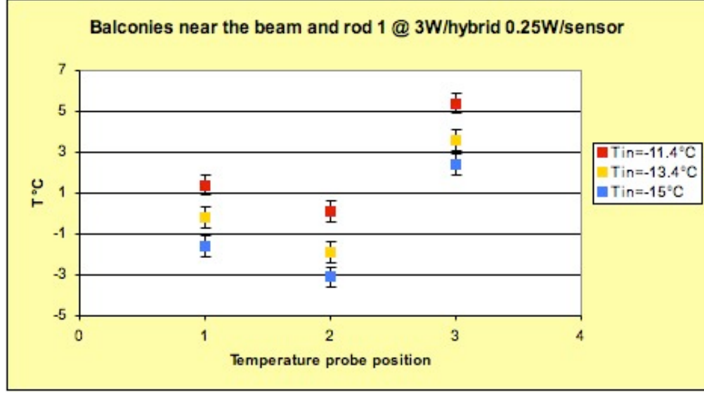
Figure 4.27: Measurements of the temperature of the balconies and comparison to the temperature of the cooling rod at the same place. The power dissipated by the resistors simulating the hybrids is 3 W and the ones for this sensors is 0.25 W.
