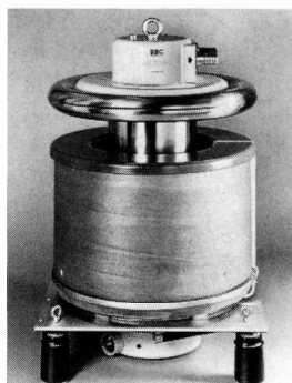
Special high-vacuum tetrodes for fast DC switching and control up to 170 kV, 120 A. Switching times in the order of \mu s. Integrated x-ray shield, SF 6 insulation and antiparasitic damping.
