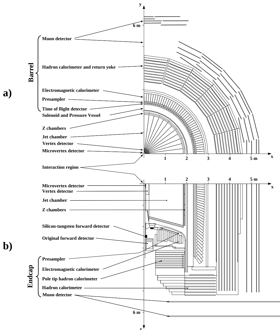
Figure 4.3: Cut-away view of the OPAL detector. In (a), the x, y view of the detector is shown, in (b) the x, z view.
