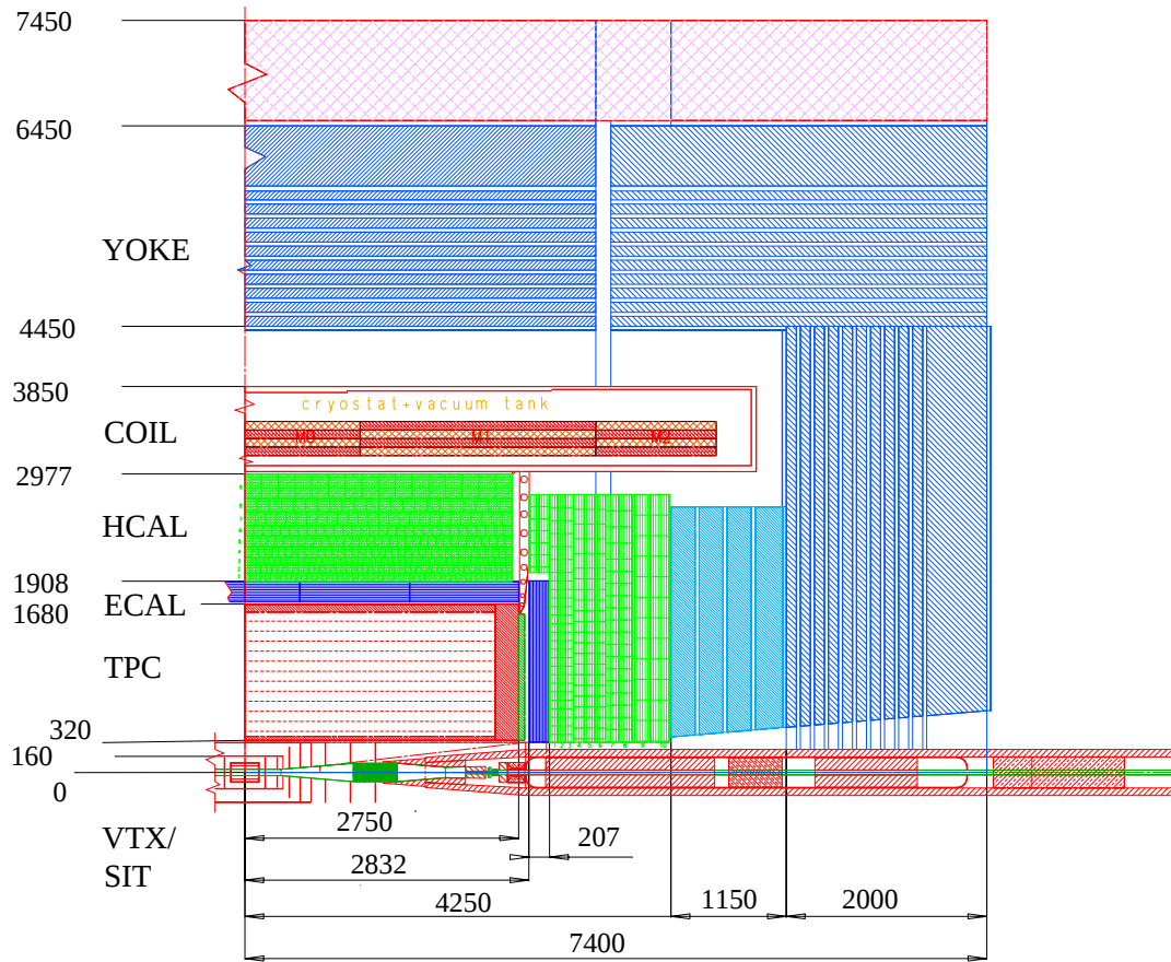
Figure 4.11: One quarter of the TESLA detector. The tracking system extends up to r = 1.68 m. The complete calorimetry is inside the 4 T coil, the muon system outside.
