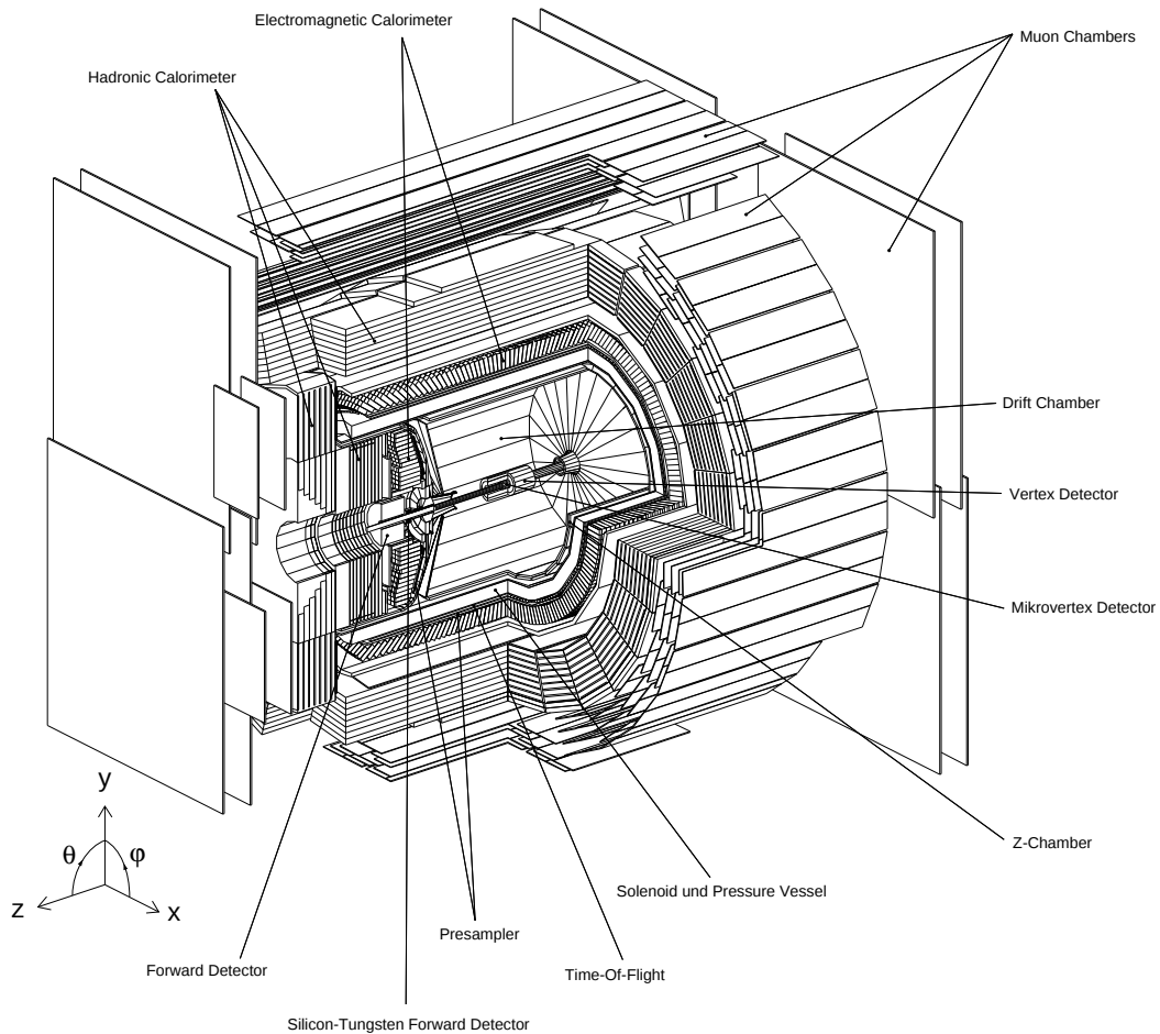
Figure 4.2: The OPAL detector. It is a collider detector with almost complete coverage of the solid angle, located at the LEP e^+e^- collider at CERN. It has a diameter of 10 m and a length of 12 m.
