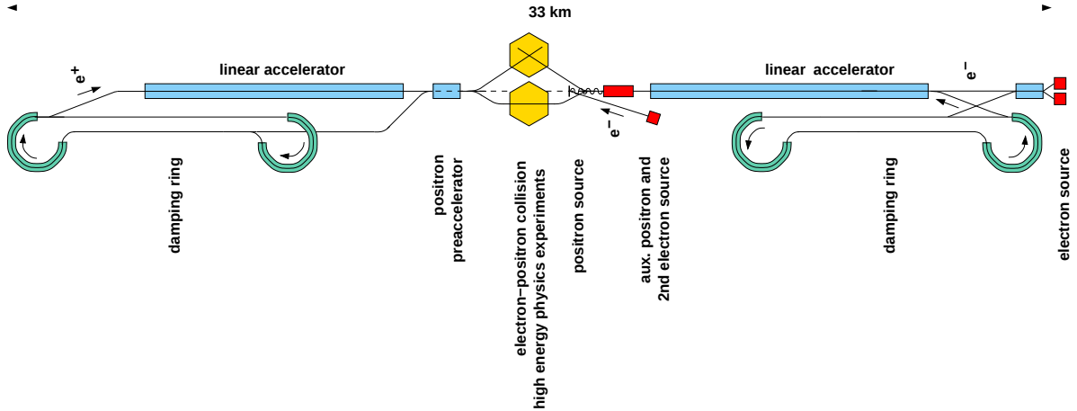
Figure 4.9: The TESLA linear accelerator. Particles are accelerated in two separate machine arms with 16.5 km length each and brought to collision at one or two central interaction regions with \sqrt{s} = 91.2 to \sqrt{s} = 800 GeV.
