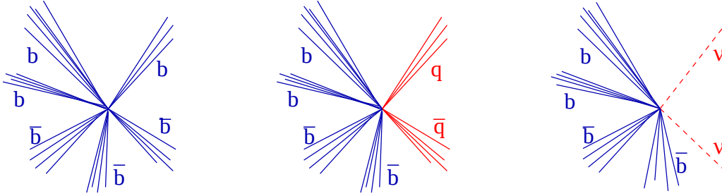
Figure 3.6: The signatures of cascade-decay channels of Higgs bosons at e^+e^- colliders. In the MSSM, the decay \mathcal{H}_2 \rightarrow \mathcal{H}_1\mathcal{H}_1 \rightarrow b\bar{b}b\bar{b} can be dominant in some regions of the parameter space.
