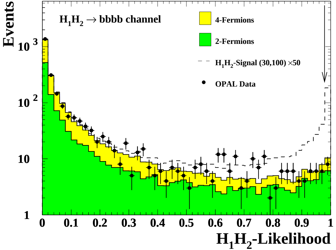
Figure 5.10: Likelihood distribution in the e^+e^- \rightarrow H_1 H_2 \rightarrow b\bar{b}b\bar{b} channel for light m_{\mathcal{H}_1} .
