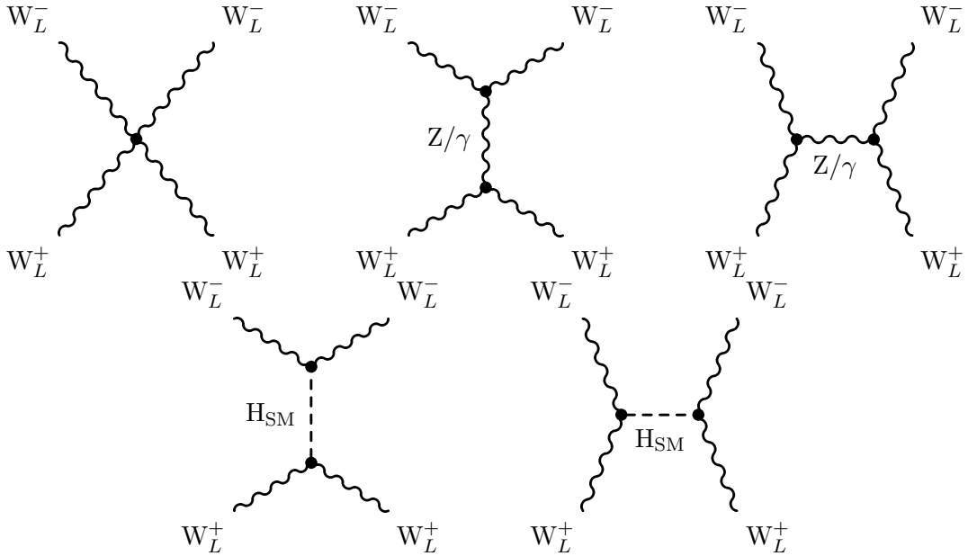
Figure 2.3: Divergent WW cross-section graphs and their cancellation. The upper three diagrams violate unitarity starting from \sqrt{s} \approx 1.2 TeV. These unitarity violations are cancelled by the lower two diagrams involving Higgs boson exchange.
