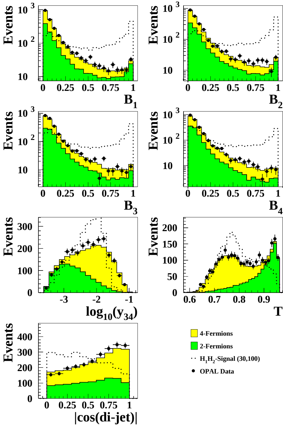
Figure 5.9: Likelihood input distributions for light m_{H_1} .
