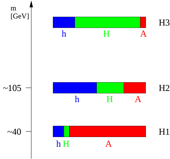
Figure 2.15: Mass and weak eigenstates of Higgs bosons in CPV models. In this schematic model for a specific parameter set, the Higgs boson mass eigenstate H_1 at m_{H_1} = 40 GeV has a large admixture of the CP-odd weak eigenstate, and therefore has a small coupling to the Z boson in Higgsstrahlung.
