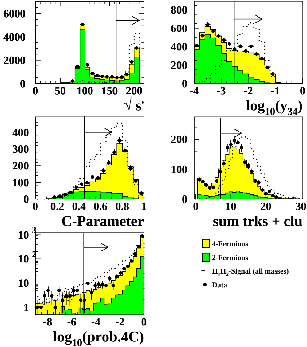
Figure 5.2: Distribution of the preselection variables in the search for e^+e^- \rightarrow \mathcal{H}_1\mathcal{H}_2 for heavy m_{\mathcal{H}_1} and for the data at \sqrt{s} = 199 - 209 GeV recorded in the year 2000.
