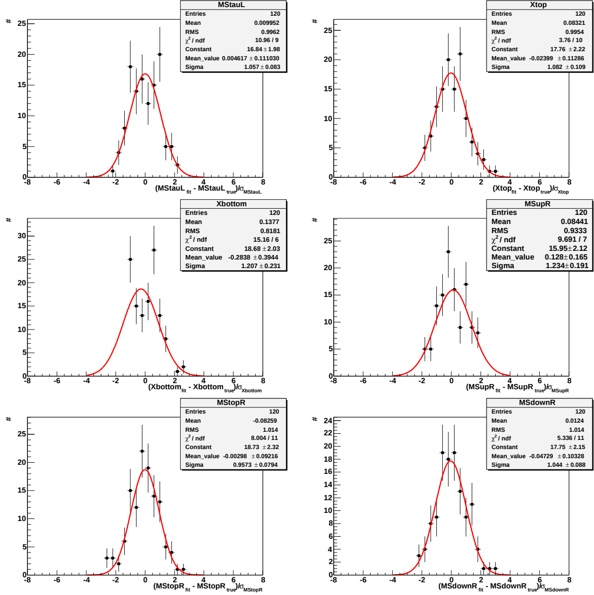
Figure 7.10: Pull distributions of the parameters of the SPS1a fit for 120 independent fits with observables smeared within their uncertainties. The uncertainties of all parameters are well described, apart from X_{\text{bottom}} .
