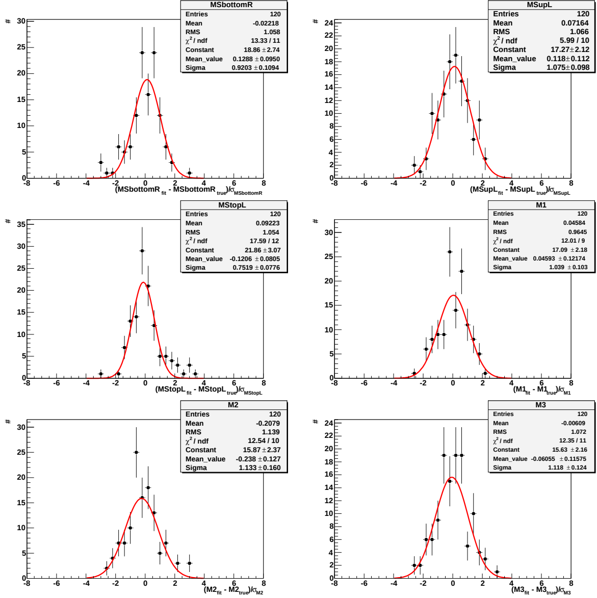
Figure 7.11: Pull distributions of the parameters of the SPS1a fit for 120 independent fits with observables smeared within their uncertainties. The uncertainties of all parameters are well described.
