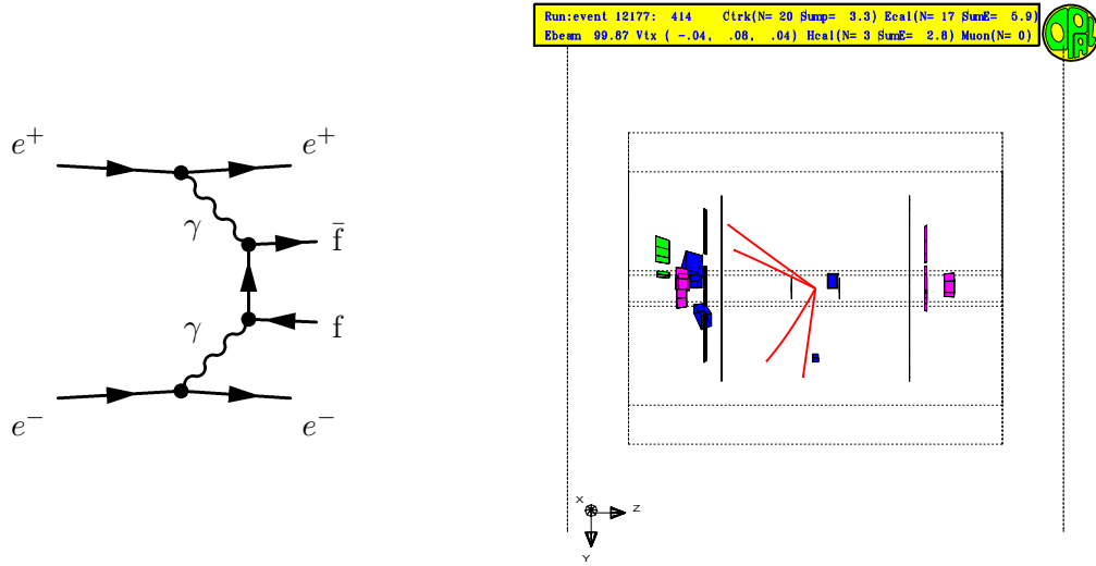
Figure 4.5: The \gamma\gamma process at LEP. Two photons are radiated from the incoming beams. They can create hadronic final states in their collision, which appears in the detector with small energy and unbalanced momentum.
