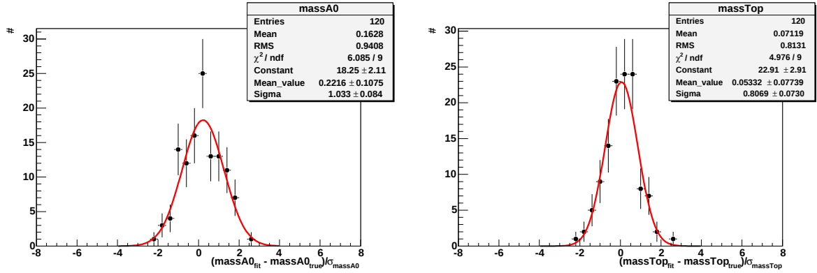
Figure 7.12: Pull distributions of the parameters of the SPS1a fit for 120 independent fits with observables smeared within their uncertainties. The uncertainties of all parameters are well described.
