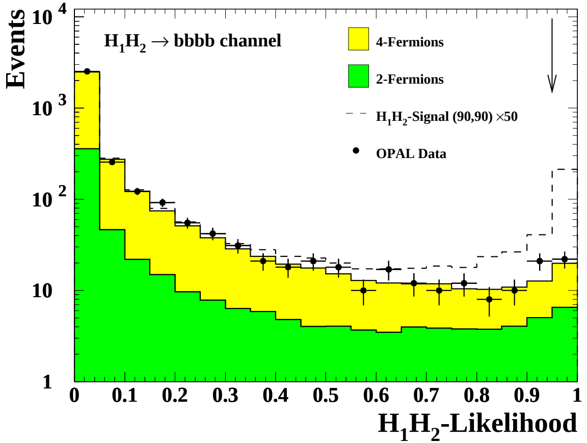
Figure 5.4: Likelihood distribution in the e^+e^- \rightarrow H_1H_2 \rightarrow b\bar{b}b\bar{b} channel for heavy m_{H_1} . There is good agreement between data and background simulation.
