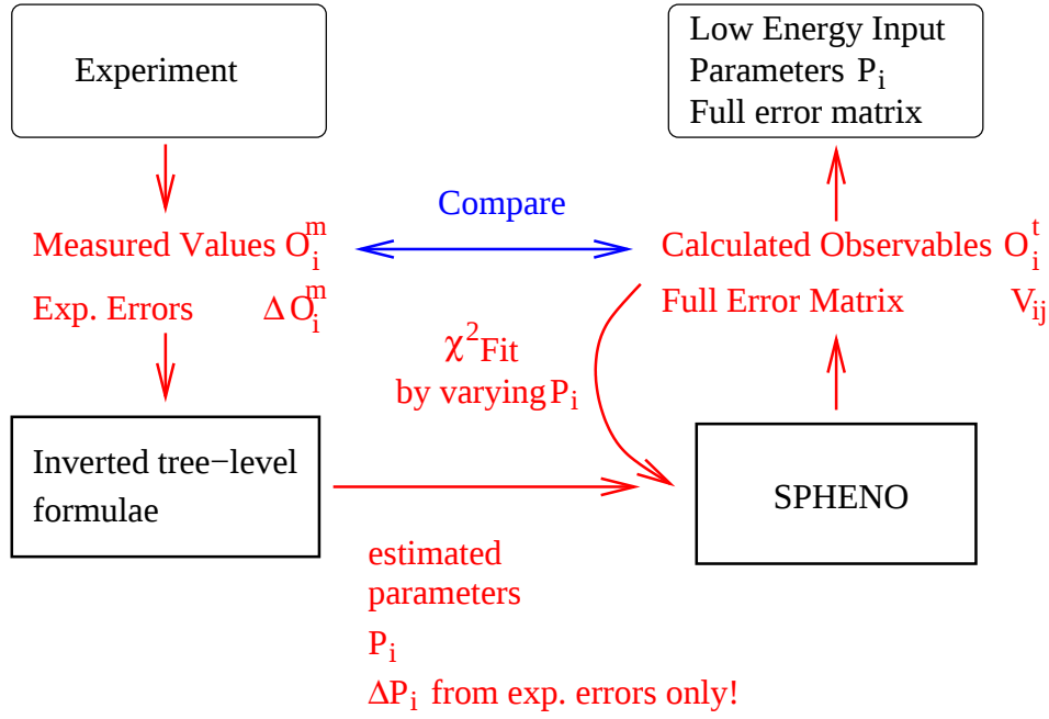
Figure 7.5: The iterative fit procedure of Fittino. From the observables O_i and their uncertainties \Delta O_i , the start values for parameters P_j of the fit are calculated in a bias-free way using tree-level relations. After the fit, the fitted parameters P_j and their uncertainties \Delta P_j are obtained, including their full correlation matrix.
