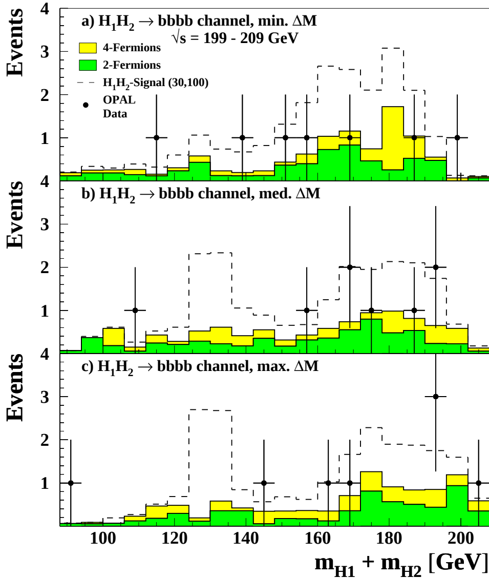
Figure 5.11: Mass distributions for light m_{\mathcal{H}_1} . In the uppermost plot, the sum of the reconstructed Higgs boson masses m_{\mathcal{H}_1} + m_{\mathcal{H}_2} is shown for the jet mass combination with the lowest \Delta m = m_{\mathcal{H}_2} - m_{\mathcal{H}_1} . The plot in the middle shows m_{\mathcal{H}_1} + m_{\mathcal{H}_2} for the di-jet combination with intermediate \Delta m , the lowest plot shows the di-jet combination with largest \Delta m .
