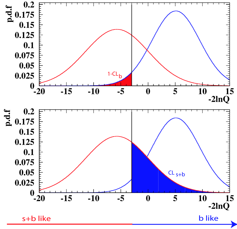
Figure 6.2: Test statistic of the confidence level calculation. The weight of each event is calculated according to its expected signal and background.
