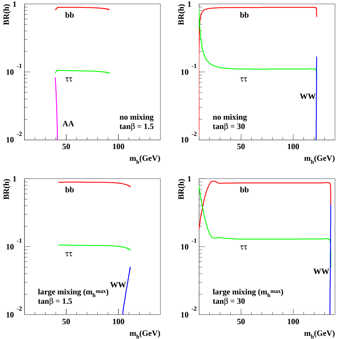
Figure 3.4: Typical Higgs boson branching ratios for two of the MSSM scenarios described in Section 6 for different values of \tan\beta . The predictions are calculated using FEYN-HIGGS(DECAY) [54].
