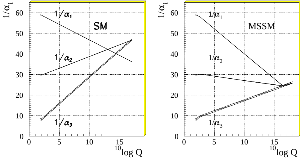
Figure 2.9: Unification of the forces in supersymmetric models. The three coupling constants \alpha_1, \alpha_2 and \alpha_3 are not unified at any scale in the SM. Additional SUSY particles alter the running of the coupling constants, leading to unification at the GUT scale.
