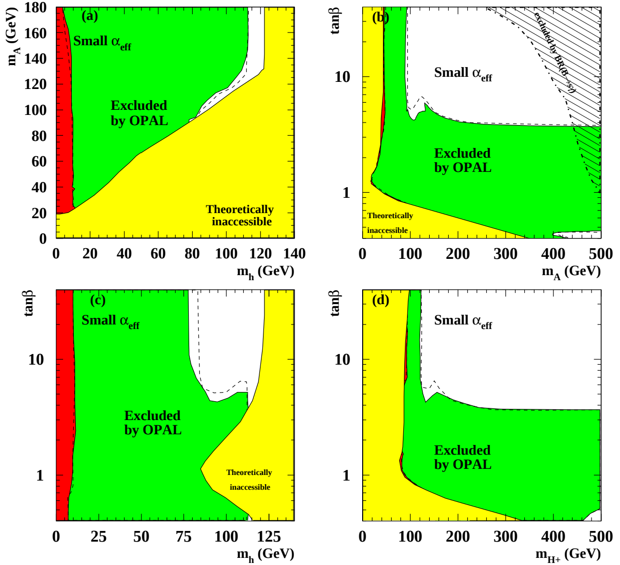
Figure 6.15: Results for the “small \alpha_{\text{eff}} ” benchmark scenario described in the text of Section 6.4.1. See Fig. 6.8 for the notation.
