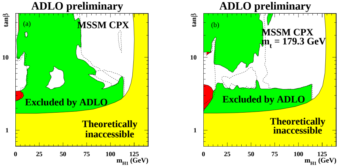
Figure 6.23: The “CPX” MSSM 95 % CL exclusion areas in the (m_{H_1}, \tan \beta) plane for the combination of the data of all four LEP experiments, using (a) a central value of m_{\text{top}} = 174.3 GeV for the top quark mass and (b) a value of m_{\text{top}} = 179.3 GeV.
