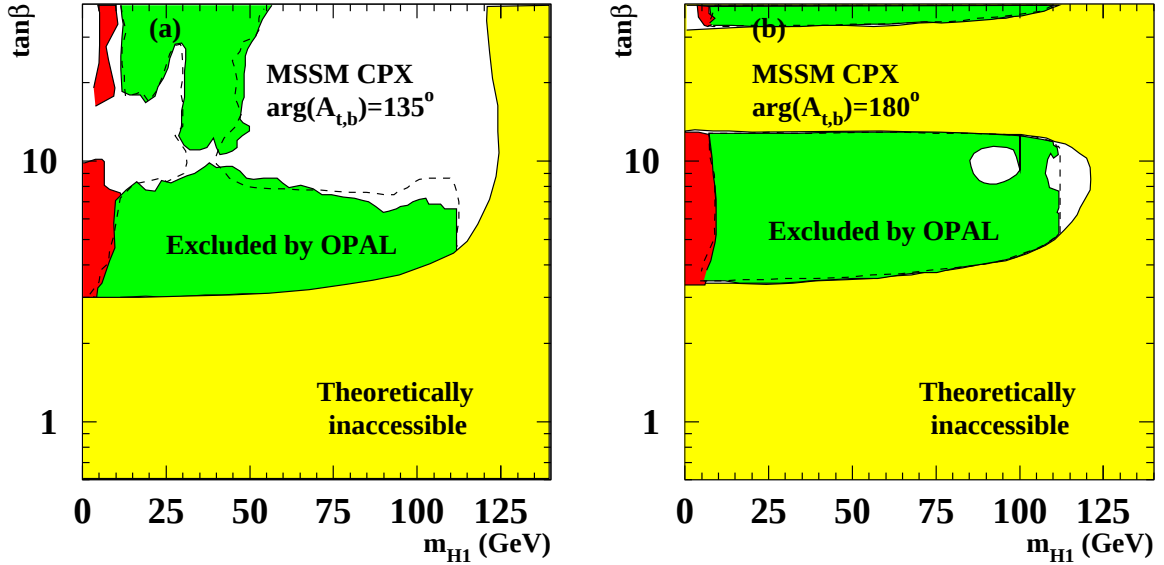
Figure 6.20: The “CPX” MSSM 95 % CL exclusion areas in the (m_{H_1}, \tan\beta) plane, using scans with (a) \arg(A_{t,b}) = \arg(m_{\tilde{g}}) = 135^\circ and (b) \arg(A_{t,b}) = \arg(m_{\tilde{g}}) = 180^\circ . See Fig. 6.8 for the notation.
