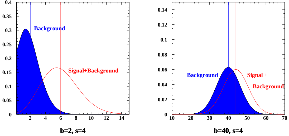
Figure 6.1: Test statistic of a counting experiment. Each observed event in data, background and signal has the same weight.
