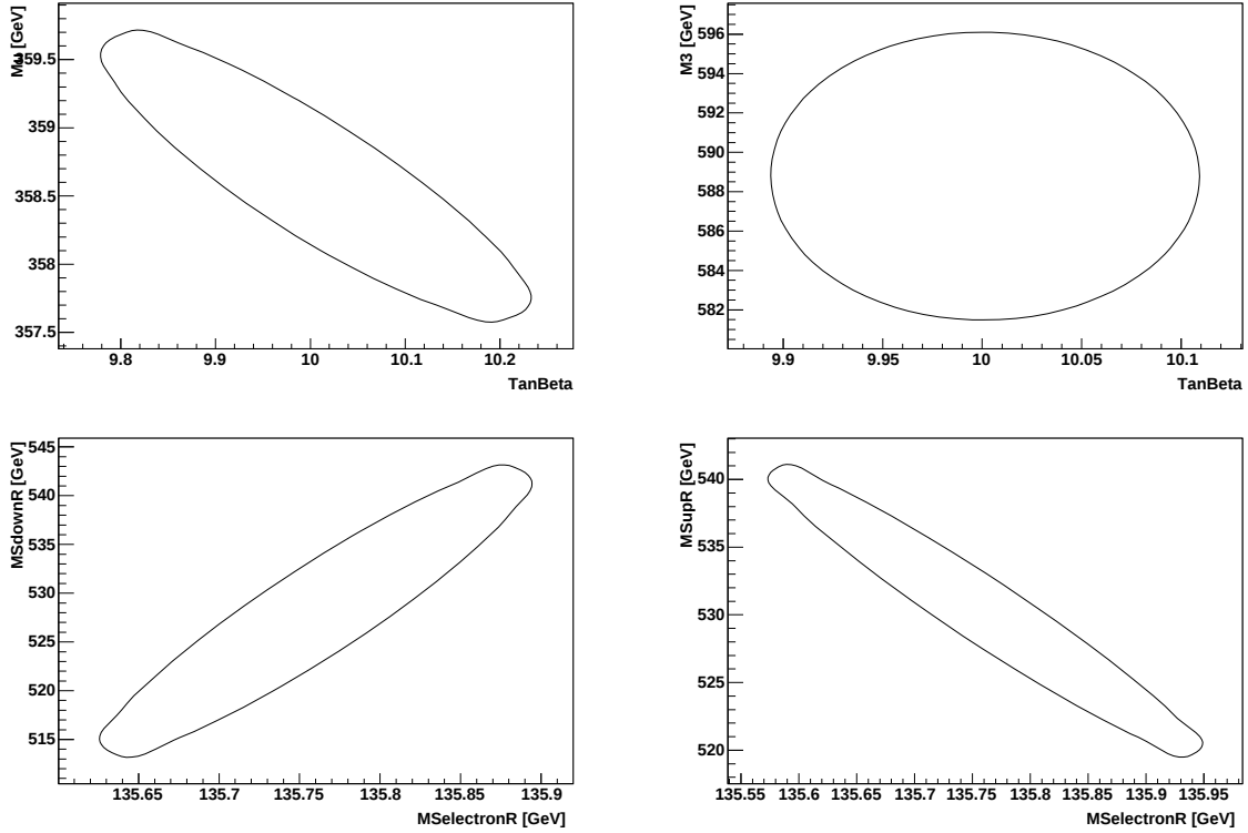
Figure 7.7: Examples of the two-dimensional uncertainty contours of the Fittino SPS1a fit.
