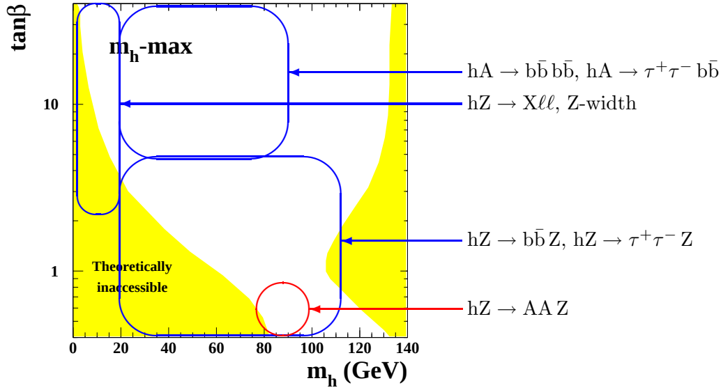
Figure 6.7: The use of the individual searches in the “ m_h –max” scenario. In red, the areas are shown where the exclusion is difficult, although the Higgs boson is kinematically accessible.
