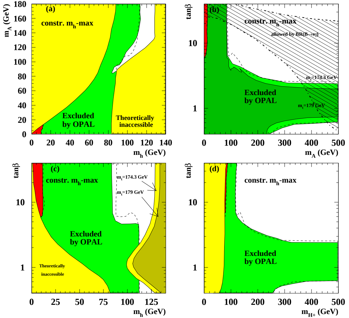
Figure 6.12: Results for the constrained “ m_h -max” benchmark scenario described in the text of Section 6.4.1. See Fig. 6.8 for the notation. The differently shaded regions in (b) show the exclusion for different values of m_{\text{top}} , as written in the Plot. The upper limit on m_h for different values of m_{\text{top}} is shown in (c), as also expressed in the plot.
