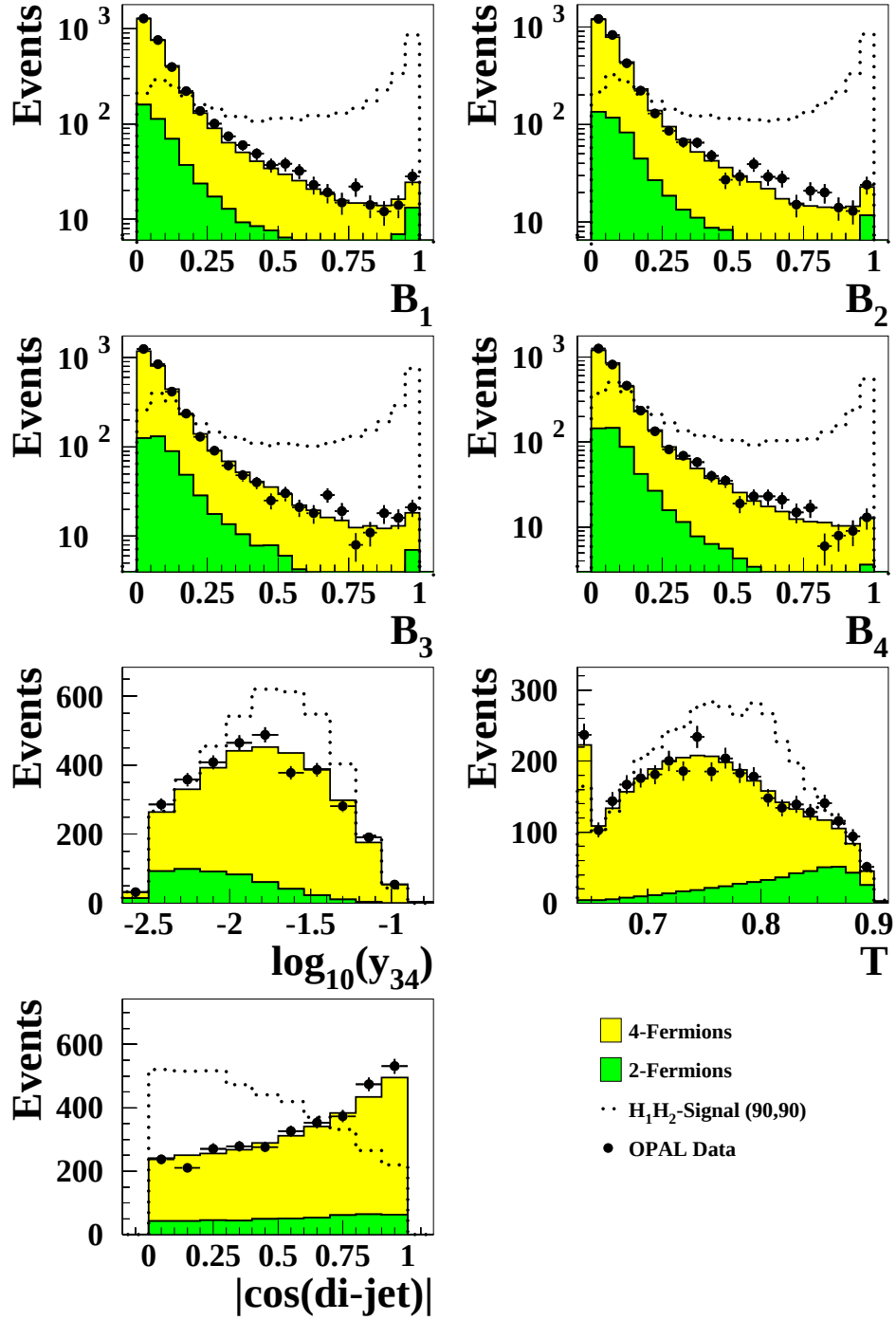
Figure 5.3: Likelihood input distributions for heavy m_{H_1} in the search for e^+e^- \rightarrow m_{H_1}m_{H_2} \rightarrow b\bar{b}b\bar{b} . There is good agreement between data and background simulation.
