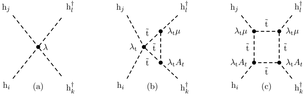
Figure 2.13: Introduction of CPV effects into the Higgs potential. The non-zero minimum of the Higgs potential is formed by the quartic coupling graph. It is subject to loop corrections from stop loops, which radiatively introduce CP violation into the Higgs potential.
