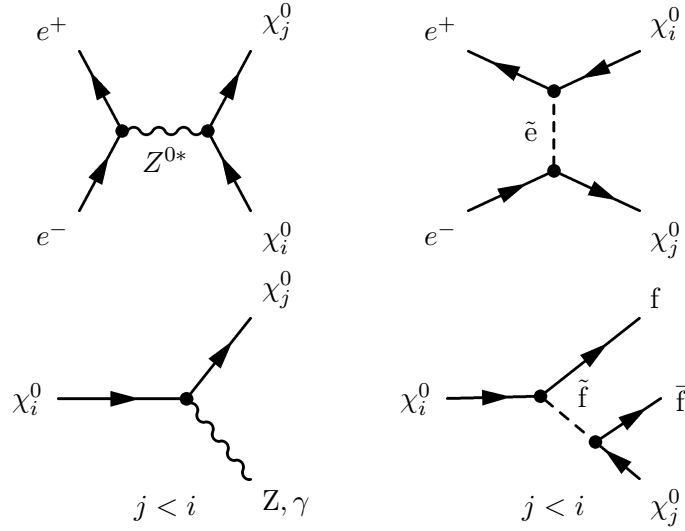
Figure 7.3: Production and decay of neutralinos at e^+e^- colliders. It is assumed that the lightest neutralino is the LSP.
