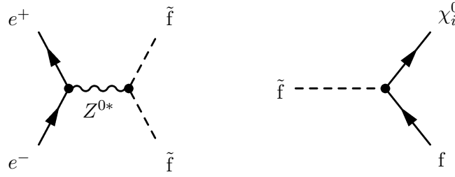
Figure 7.1: Production and decay of sfermions at e^+e^- colliders. It is assumed that the lightest neutralino is the LSP.
