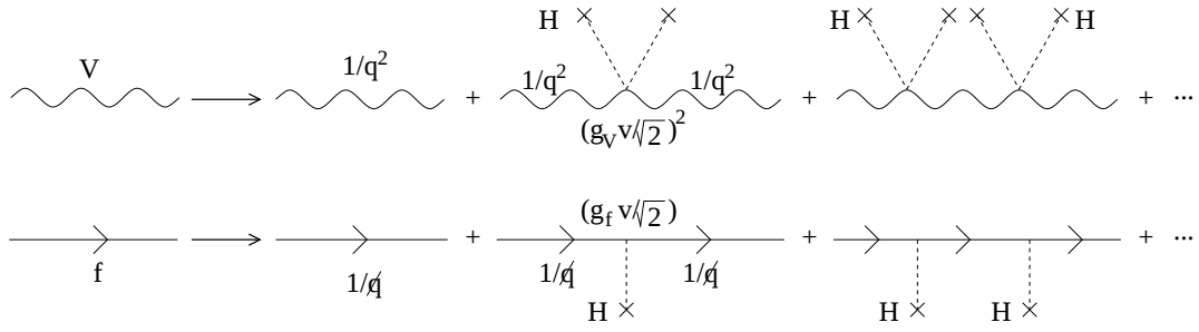
Figure 2.2: The generation of particle masses through the Higgs mechanism. In the upper diagram, the mass generation for spin-1 bosons is shown. The massless propagator 1/q^2 interacts with the Higgs background field. In the lower diagram, the same mechanism is shown for fermions.
