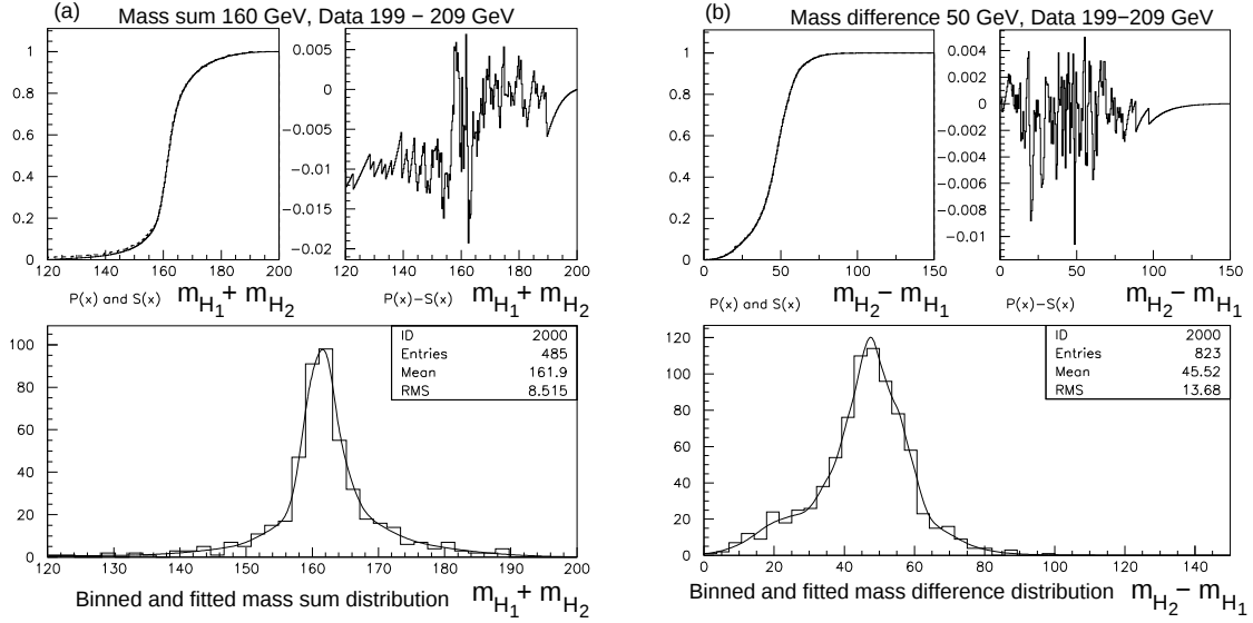
Figure 5.13: Fit of the e^+e^- \rightarrow \mathcal{H}_1\mathcal{H}_2 \rightarrow b\bar{b}b\bar{b} signal mass sum shape (a) and the mass difference shape (b). The sum of the Higgs boson masses m_{\mathcal{H}_1} + m_{\mathcal{H}_2} is 160 GeV, the difference is 50 GeV. The plots are explained in the text.
