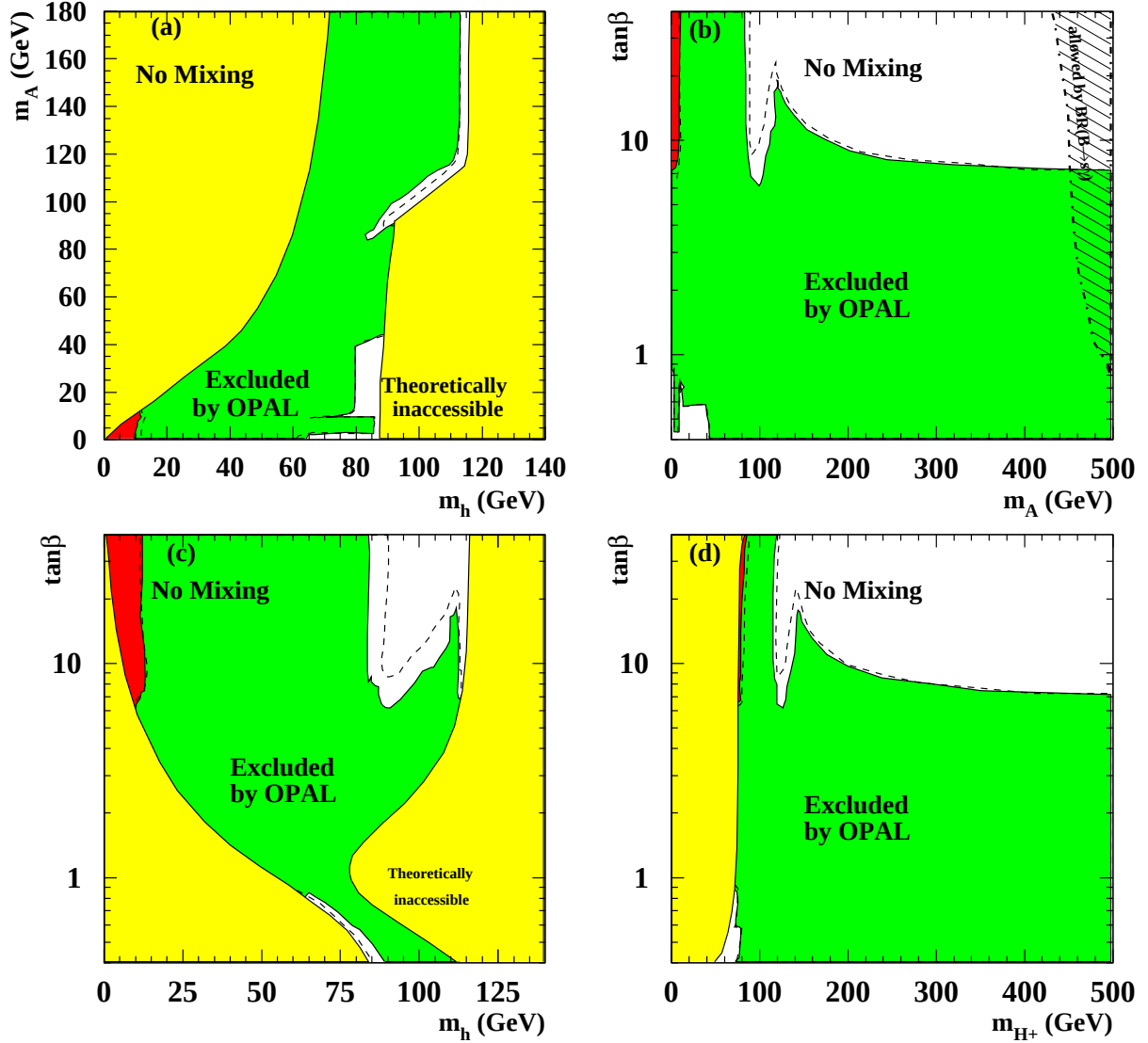
Figure 6.8: Results for the “no mixing” benchmark scenario. The figure shows the excluded regions in darker grey (green) and theoretically inaccessible regions in light grey (yellow) as functions of the MSSM parameters in four projections: (a) the (m_h, m_A) plane, (b) the (m_A, \tan\beta) plane, (c) the (m_h, \tan\beta) plane and (d) the (m_{H^\pm}, \tan\beta) plane. The dashed lines indicate the boundaries of the regions expected to be excluded at the 95% CL if only SM background processes are present. The region excluded by Yukawa searches, Z-width constraints or decay independent searches is shown in dark grey (red). In (b) the hatched area is still allowed by \text{BR}(b \rightarrow s\gamma) searches.
