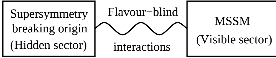
Figure 2.11: The mediation of SUSY breaking from the hidden sector. Unspecified physics at the GUT scale in a so-called hidden sector leads to SUSY breaking. This breaking is then transferred to the visible sector via a messenger field, which can be a known field like gauge fields of gravity or new physics.
