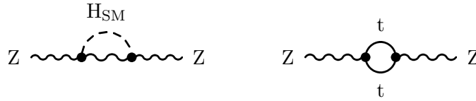
Figure 2.6: Loop contributions to the Z boson mass. These loop corrections allow the indirect measurement of the Higgs mass, if the top quark mass is known.
