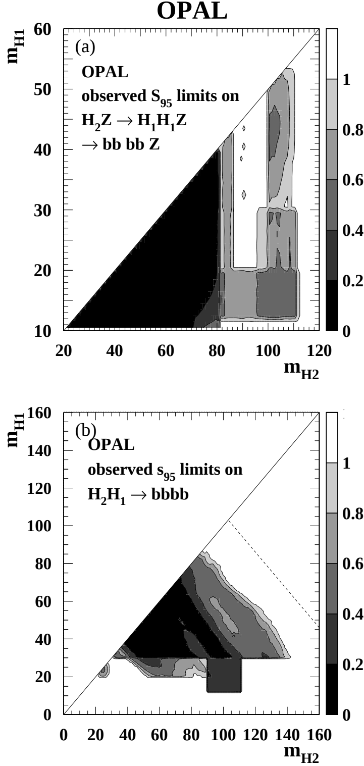
Figure 6.5: Model-independent upper bounds on \sigma \times \text{BR} for (a) the e^+e^- \rightarrow \mathcal{H}_2Z \rightarrow \mathcal{H}_1\mathcal{H}_1Z \rightarrow b\bar{b}b\bar{b}Z channel and (b) the e^+e^- \rightarrow \mathcal{H}_1\mathcal{H}_2 \rightarrow b\bar{b}b\bar{b} channel. For (a), the SM cross-section for H_{\text{SM}}Z production is taken as normalization. For (b), The MSSM cross-section for \mathcal{H}_1\mathcal{H}_2 production with \cos^2(\beta - \alpha) = 1 is taken as normalization. The dashed line indicates the kinematic limit for \sqrt{s} = 206 GeV.
