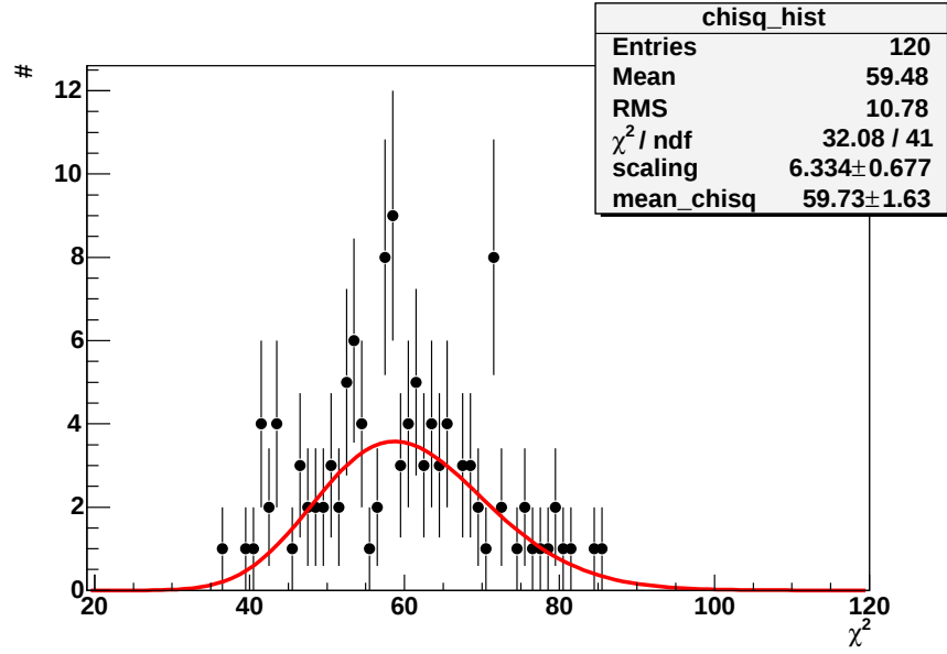
Figure 7.8: Distribution of \chi^2 for the SPS1a fit. 120 fits with 62 d.o.f. are performed. The observables of the simulated measurements are smeared in each fit according to their uncertainties. The mean of the distribution is \chi^2_{\text{mean}} = 59.7 \pm 1.6 .
