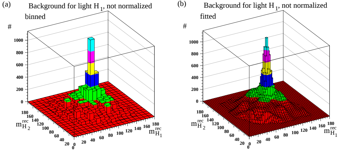
Figure 5.15: Fit of the two-dimensional background mass distribution for light m_{H_1} . In (a), the unfitted binned background distribution is shown. In (b), the fitted distribution for \sqrt{s} = 199 - 209 GeV is given.
