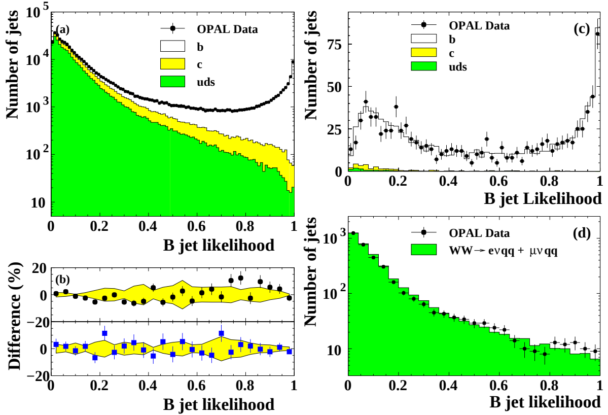
Figure 5.1: The OPAL b -tag calibration distributions. In (a) the B probability of jets in the calibration data at \sqrt{s} = m_Z in the year 1999 is shown. The simulation of b jets (open), c jets (yellow, light grey) and uds jets (green, dark grey) shows a very good agreement with the data. Jets from b quarks tend to have a large B probability. In (b), the relative difference between the data and the Monte Carlo is tested (see text). In (c), the B probability of jets opposite to b -tagged jets is given, and in (d) the B probability in W^+W^- events is shown [114].
