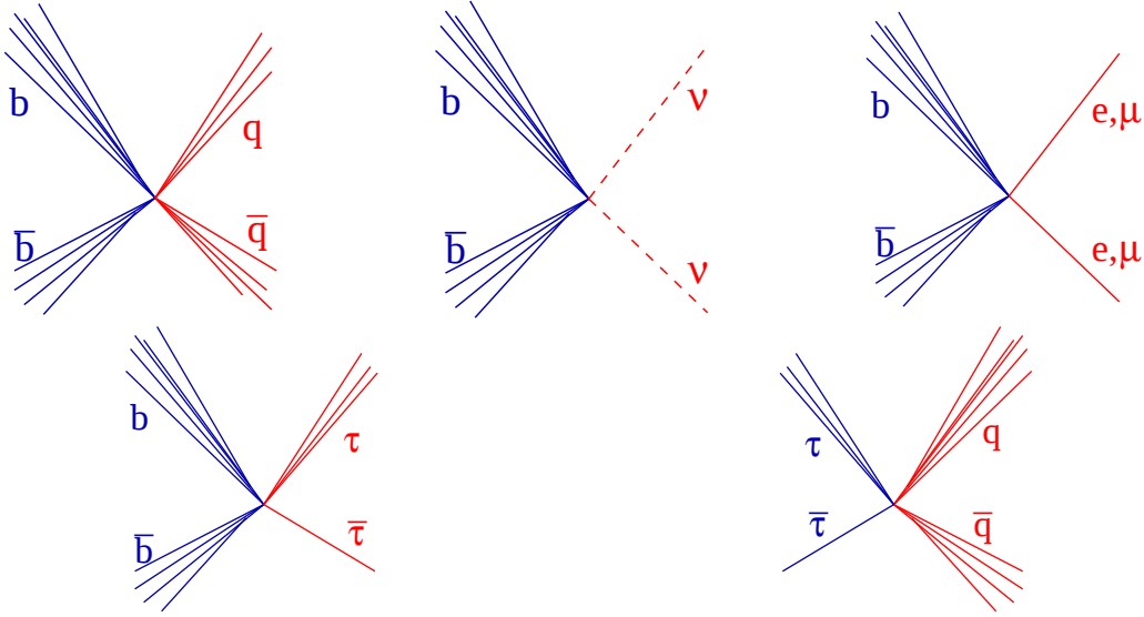
Figure 3.3: The signatures of SM-like Production channels of Higgs bosons at e^+e^- colliders. The Higgs boson decay products are shown in blue (dark, left side), the Z decay products in red (light, right side).
