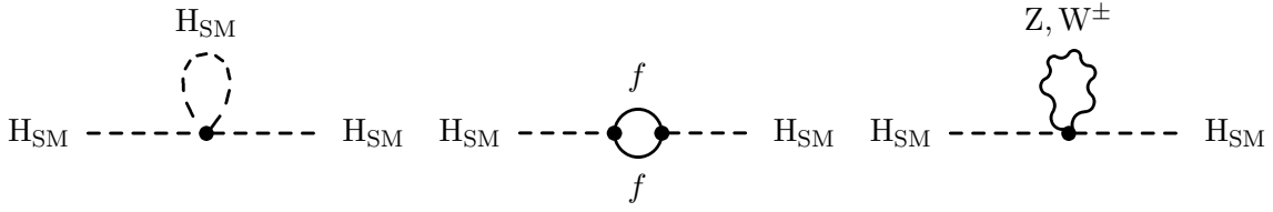
Figure 2.8: Divergent loop contributions to the Higgs boson mass. The quadratic divergencies from these graphs are not cancelled in the SM.
