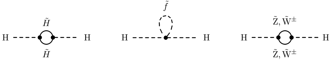
Figure 2.10: SUSY contributions to the Higgs boson mass. The quadratic divergencies to the Higgs mass introduced by the graphs in Fig. 2.8 are cancelled by the graphs above.
