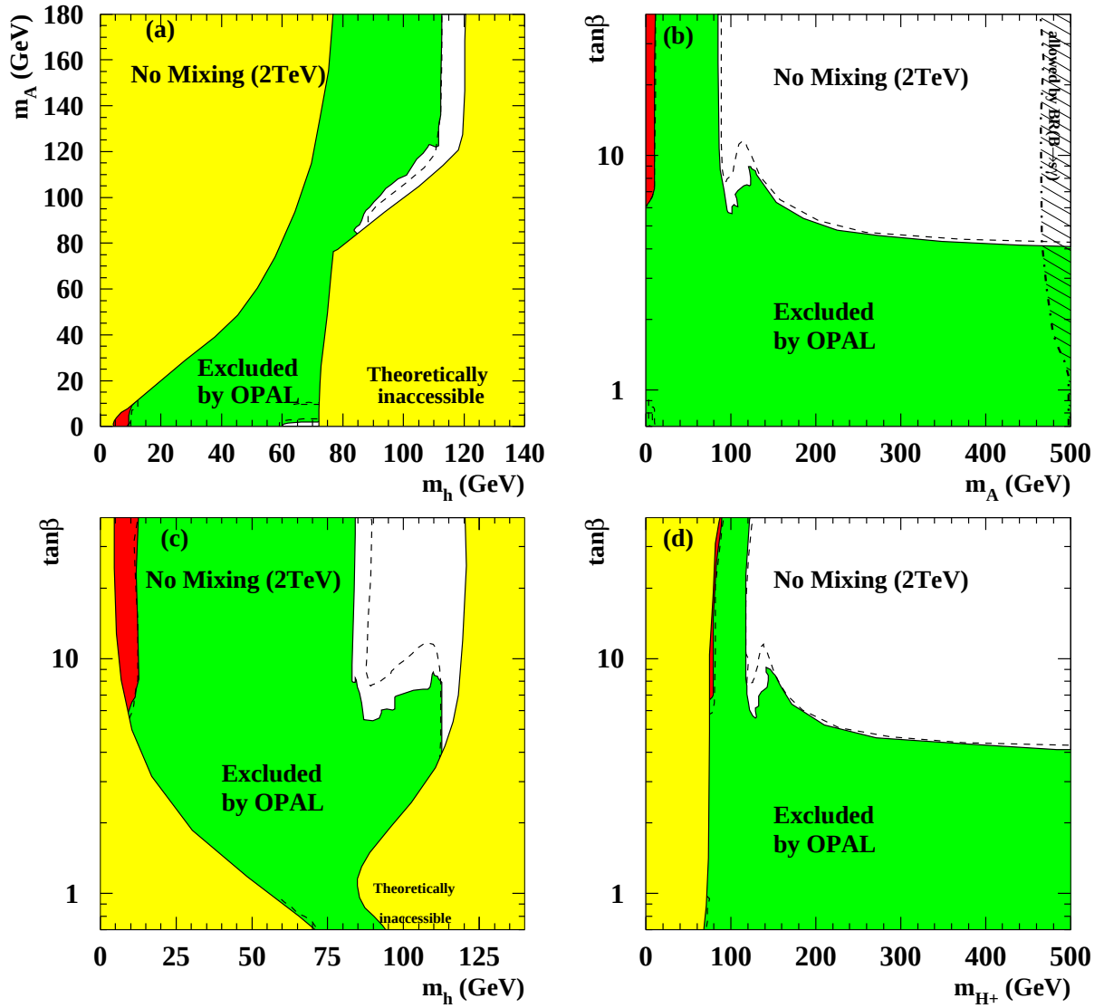
Figure 6.9: Results for the “no mixing (2 TeV)” benchmark scenario described in the text of Section 6.4.1. See Fig. 6.8 for the notation.
