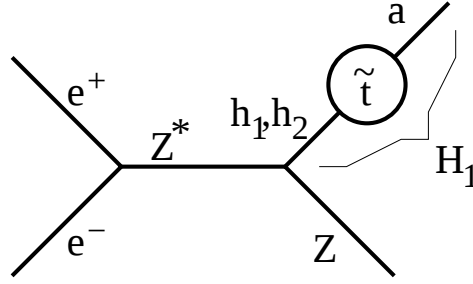
Figure 2.14: The mixing of weak Higgs boson eigenstates in CPV models. Also in CPV models, only the CP even weak Higgs states h_1 and h_2 couple to the Z boson. However, the Higgs mass eigenstate also carries a CP-odd component a that does not couple to the Z, reducing the total coupling of the mass state H_1 .
