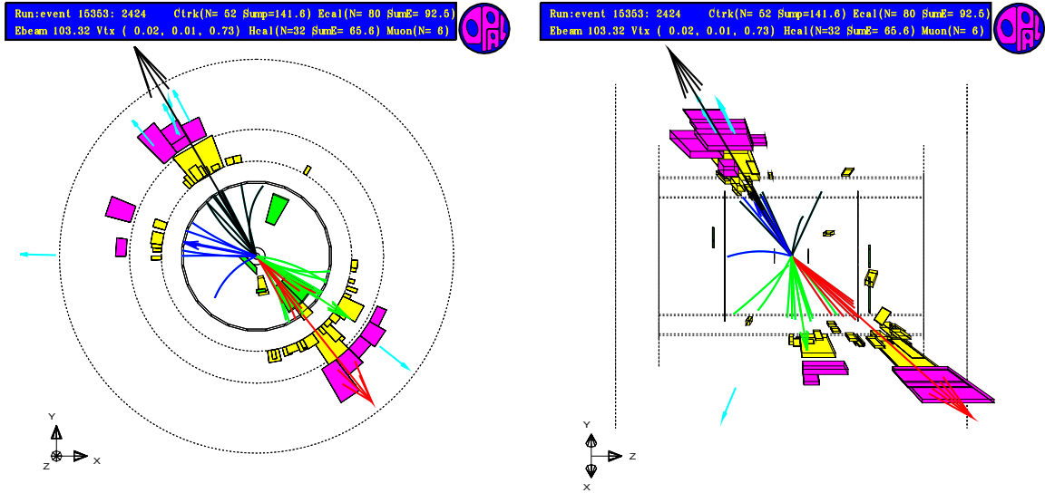
Figure 5.12: An event selected by the search for pair production with light m_{\mathcal{H}_1} . The more three-jet like shape with respect to the selected event shown in Section 5.2 is clearly visible.
