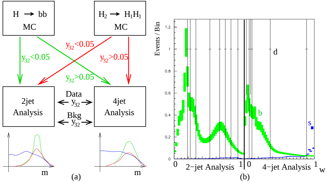
Figure 6.3: Input method of the missing energy channel for the simultaneous search for e^+e^- \rightarrow \mathcal{H}Z \rightarrow b\bar{b}\nu\bar{\nu} and e^+e^- \rightarrow \mathcal{H}_2Z \rightarrow \mathcal{H}_1\mathcal{H}_1\nu\bar{\nu} \rightarrow b\bar{b}b\bar{b}\nu\bar{\nu} . In (a) the scheme of the two selections is shown. In (b) the input distributions of the two selections are presented. The background is displayed in green (grey), the signal in blue (dark) and the data is shown in the form of the vertical lines.
