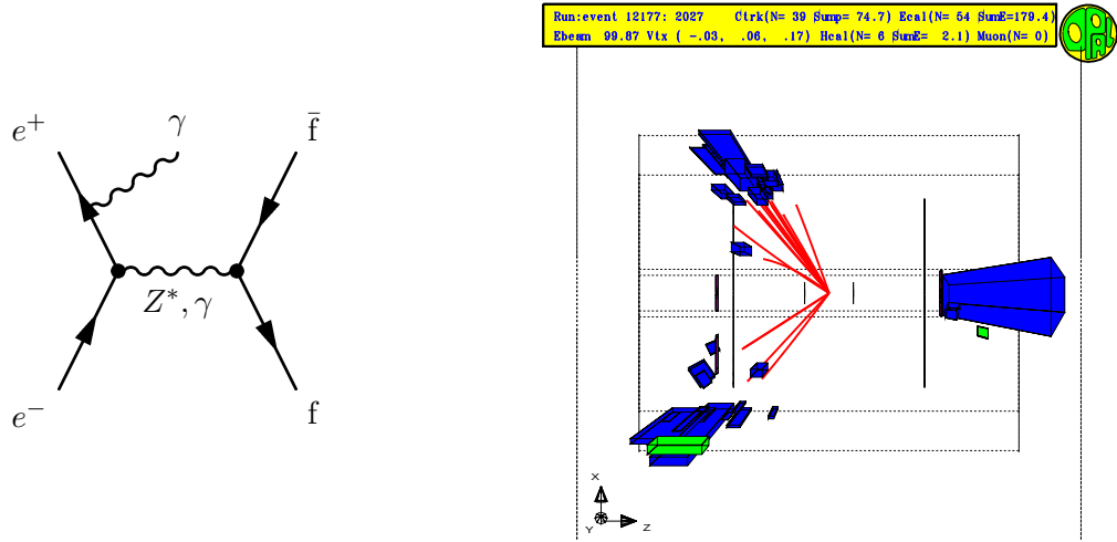
Figure 4.6: A radiative return event at LEP 2. In this event, the radiated photon is visible in the detector, which is not generally the case.
