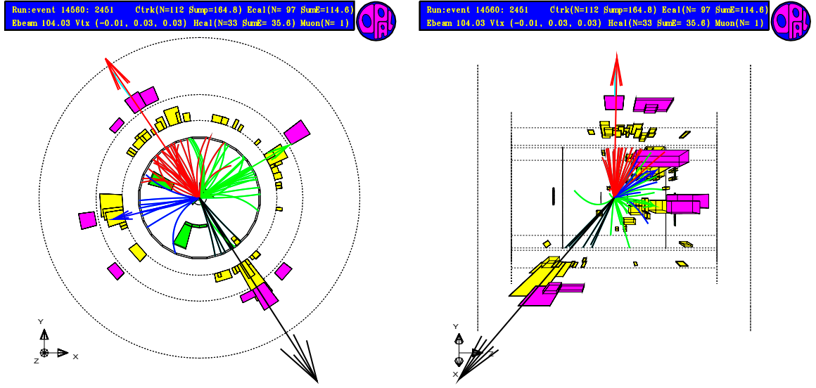
Figure 5.7: An event selected by the search for pair production with heavy m_{\mathcal{H}_1} . The r\phi view is shown on the left and the rz view is shown on the right. The four-jet structure is clearly visible.
