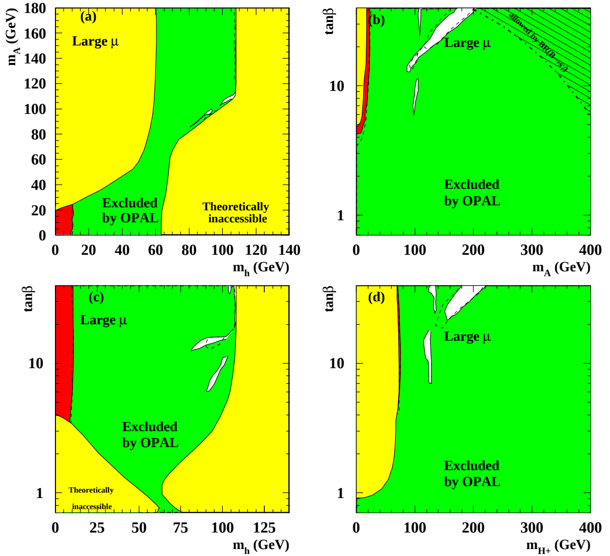
Figure 6.13: Results for the “large \mu ” benchmark scenario described in the text of Section 6.4.1. See Fig. 6.8 for the notation.
