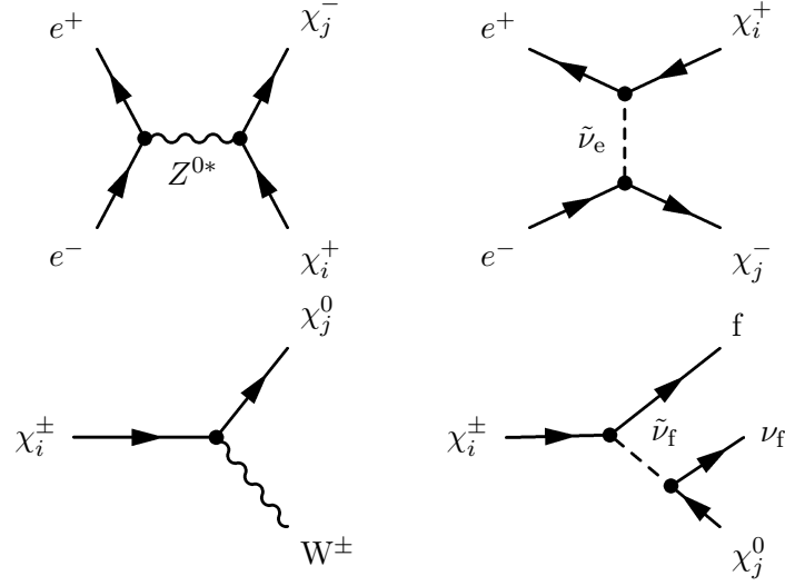
Figure 7.2: Production and decay of charginos at e^+e^- colliders. It is assumed that the lightest neutralino is the LSP.
