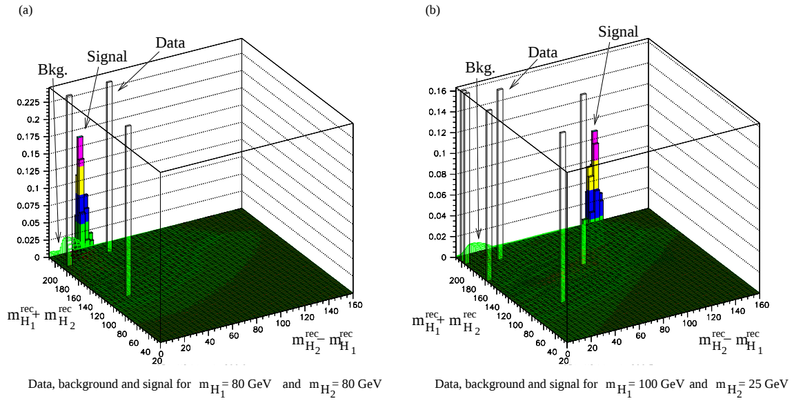
Figure 5.16: Data, signal and background distributions. The distributions given above are used in the limit calculation of Section 6 as discriminating variable. The reconstructed masses are given in terms of m_{H_1} + m_{H_2} and m_{H_2} - m_{H_1} . The opaque green (light grey) distribution is the background, the coloured peak is the signal and the data is given in the opaque black peaks. In (a), the search for heavy m_{H_1} is shown, while (b) shows the search for light m_{H_1} .
