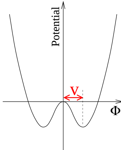
Figure 2.1: The one-dimensional projection of the potential of the Higgs field. The minimum at \Phi = v obeys a rotational symmetry, which is broken spontaneously.
