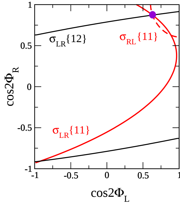
Figure 7.6: The approximate initial determination of the chargino mixing angles from LR and RL chargino cross-sections. From the measurements of three chargino cross-sections at different beam polarisation, the chargino mixing angles can be initially determined [168].
