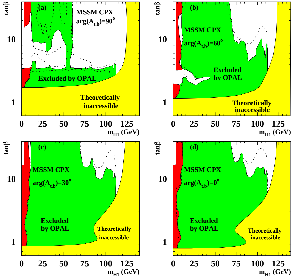
Figure 6.19: The “CPX” MSSM 95% CL exclusion areas in the (m_{H_1}, \tan\beta) plane, using scans with (a) \arg(A_{t,b}) = \arg(m_{\tilde{g}}) = 90^\circ , (b) \arg(A_{t,b}) = \arg(m_{\tilde{g}}) = 60^\circ , (c) \arg(A_{t,b}) = \arg(m_{\tilde{g}}) = 30^\circ and (d) \arg(A_{t,b}) = \arg(m_{\tilde{g}}) = 0^\circ . While the CPV phases decrease, effects from CP violation like the strong H_2 \rightarrow H_1 H_1 contribution vanish. See Fig. 6.8 for the notation.
