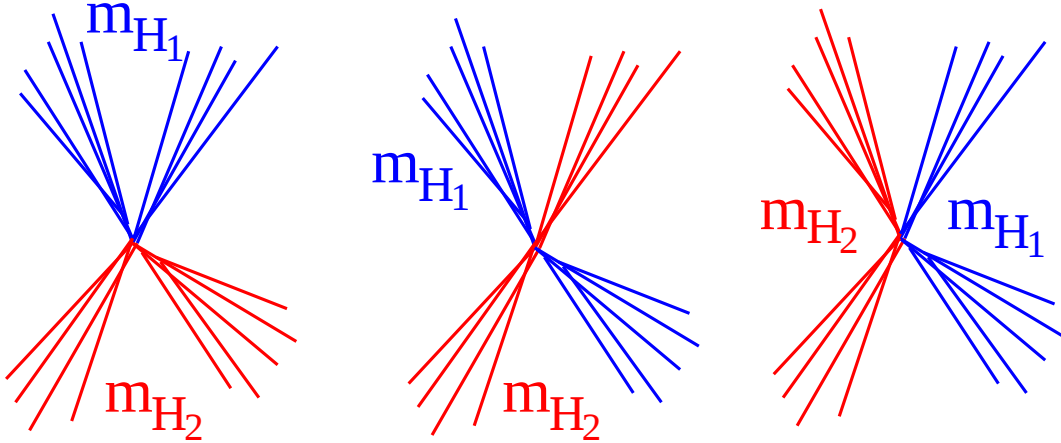
Figure 5.5: The 3 different di-jet mass combinations. The jets of each four-jet event can be grouped to two pairs of jets (di-jets) such that three different mass combinations occur.
