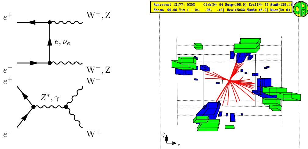
Figure 4.8: The four-fermion process at LEP. Clear four-jet events with balanced energy and momentum are visible in the detector.
