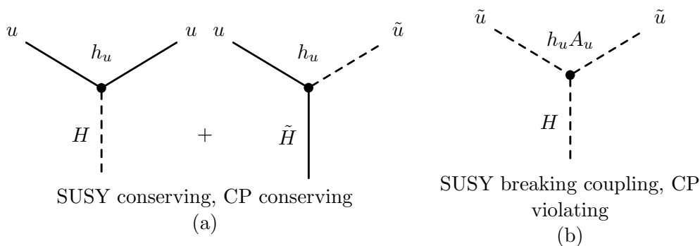
Figure 2.12: Trilinear couplings in the MSSM. The first two graphs together conserve SUSY and CP symmetries. The third graph represents the trilinear coupling. This coupling violates SUSY symmetry and complex phases of the coupling constant A can be used to introduce CP violation.
