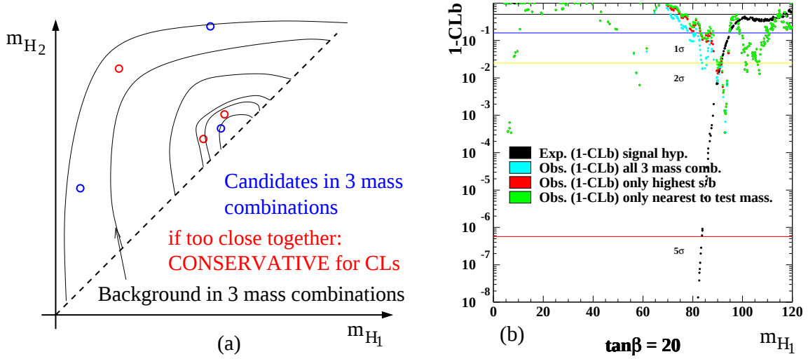
Figure 6.4: Input test of the inputs of the e^+e^- \rightarrow \mathcal{H}_2\mathcal{H}_1 \rightarrow b\bar{b}b\bar{b} pair production channel. In (a) the general problem of doublecounting is shown schematically. In (b) observed and expected (1 - \text{CL}_b) for different input schemes are presented.
