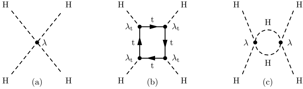
Figure 2.4: Loop corrections to the quartic Higgs self coupling. For a light Higgs boson, the dominant loop contribution to the Higgs mass arises from top quark loops (b). For heavy Higgs bosons, Higgs loops form the dominant contribution (c).
