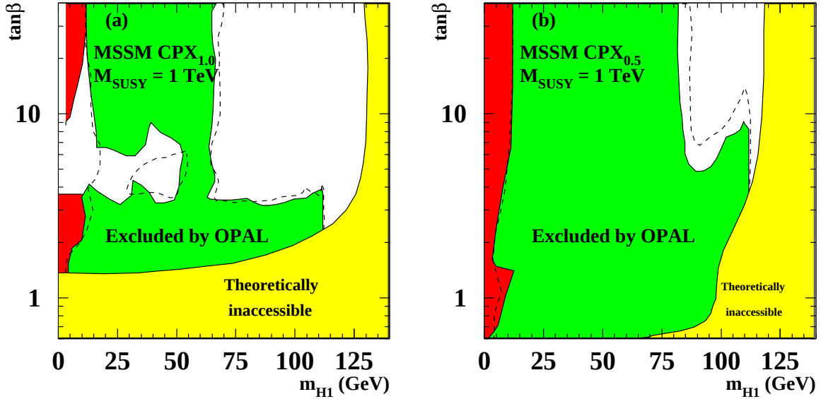
Figure 6.22: The “CPX” MSSM 95 % CL exclusion areas in the (m_{H_1}, \tan \beta) plane, using scans (a) preserving the “CPX” ratios of \mu , A_{b,t} and m_{\text{SUSY}} , using m_{\text{SUSY}} = 1 \text{ TeV} , and (b) m_{\text{SUSY}} = 1 \text{ TeV} keeping \mu and A_{b,t} at their “CPX” values. See Fig. 6.8 for the notation.
