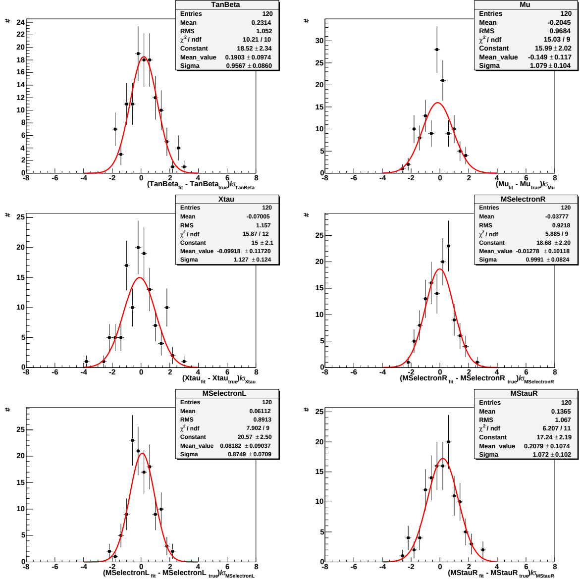
Figure 7.9: Pull distributions of the parameters of the SPS1a fit for 120 independent fits with observables smeared within their uncertainties. The uncertainties of all parameters are well described.
