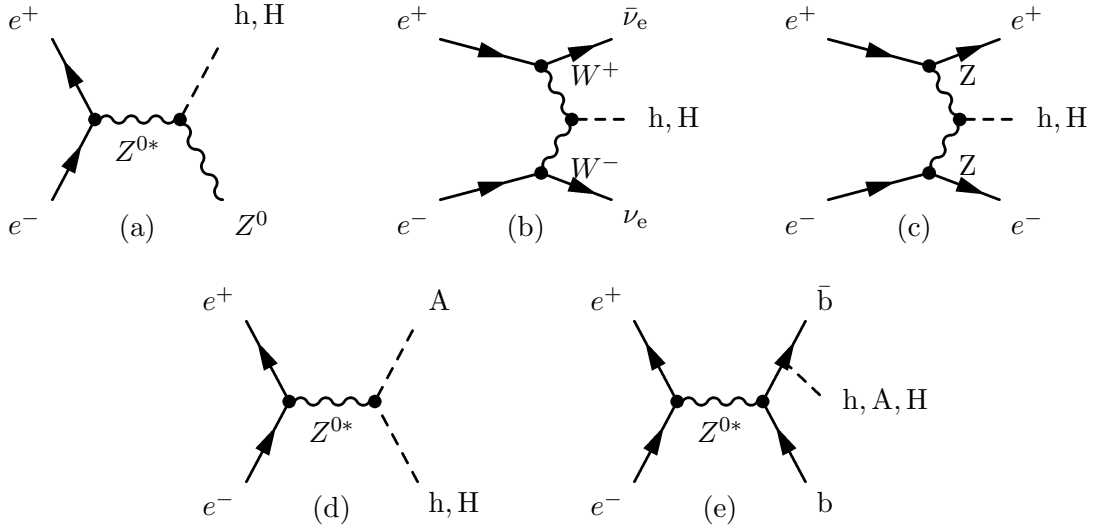
Figure 3.1: Higgs boson production mechanisms in the MSSM at e^+e^- colliders. Mechanism (a) is the Higgsstrahlung process, mechanisms (b) and (c) represent the boson fusion channels. These three channels are the dominant production channels in the SM. Pair production, shown in (d), is added in the MSSM. Finally, (e) shows the Yukawa production channel, which can be dominant in some regions of the MSSM parameter space and which plays a minor role in the SM.
