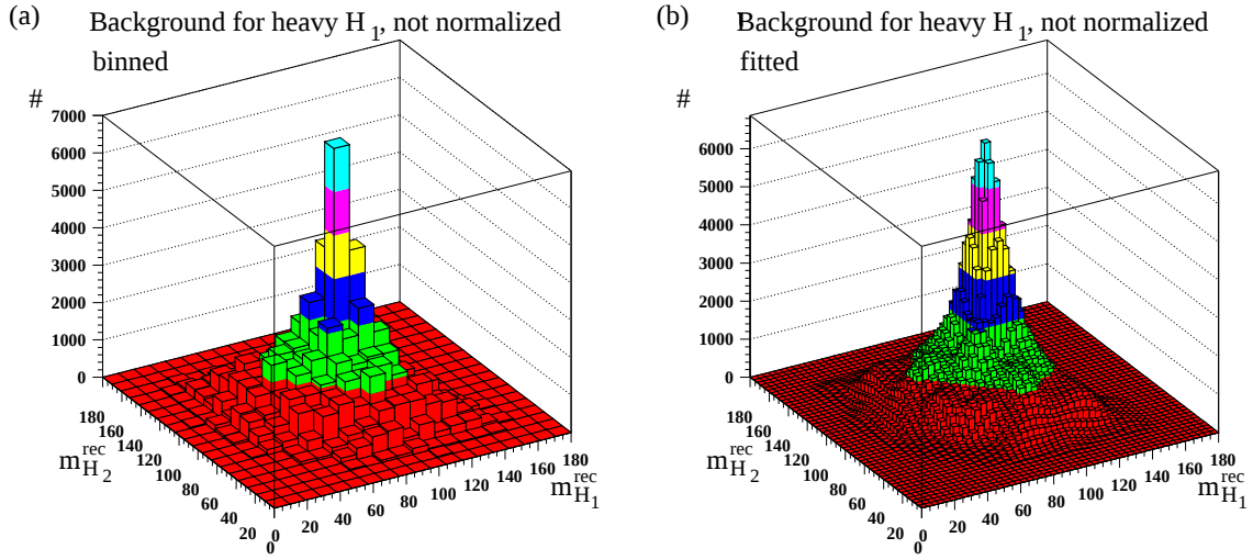
Figure 5.14: Fit of the two-dimensional background mass distribution for heavy m_{H_1} . In (a), the unfitted binned background distribution is shown. In (b), the fitted distribution for \sqrt{s} = 199 - 209 GeV is given.
