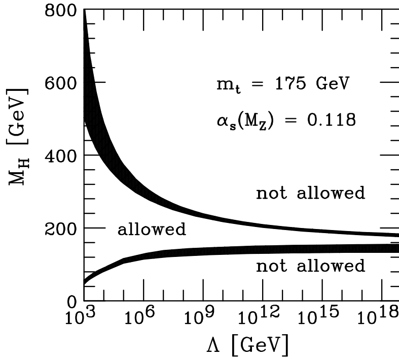
Figure 2.5: Theoretical bounds on the SM Higgs mass as a function of the cut-off scale. It is assumed that the SM is a valid theory up to the scale \Lambda . Then the upper and lower bound on the Higgs mass, stemming from Higgs-self-energy corrections, are shown by the black line [22].
