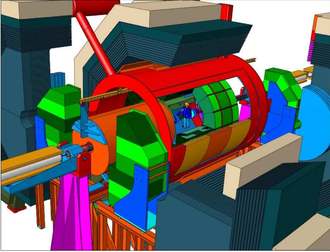
Figure 4.10: Three dimensional sketch of the TESLA detector. A coil with 8 m length and 6 m inner diameter contains the complete vertexing, tracking and calorimetry. The muon system is installed outside the coil.
