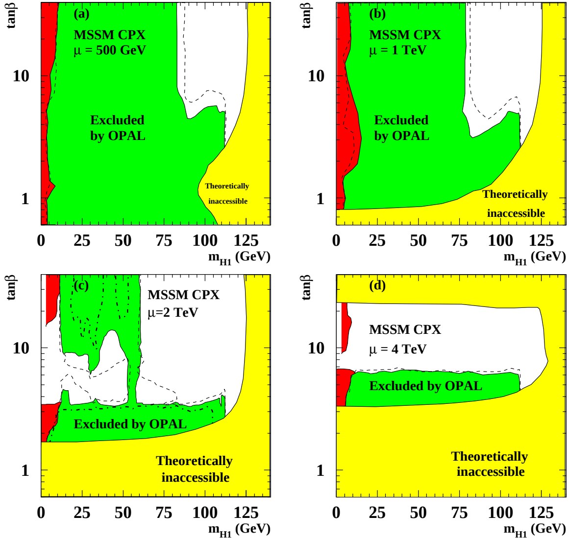
Figure 6.21: The “CPX” MSSM 95 % CL exclusion areas in the (m_{H_1}, \tan\beta) plane, using scans with (a) \mu = 500 GeV, (b) \mu = 1000 GeV, (c) \mu = 2000 GeV (“CPX”) and (d) \mu = 4000 GeV. See Fig. 6.8 for the notation.
