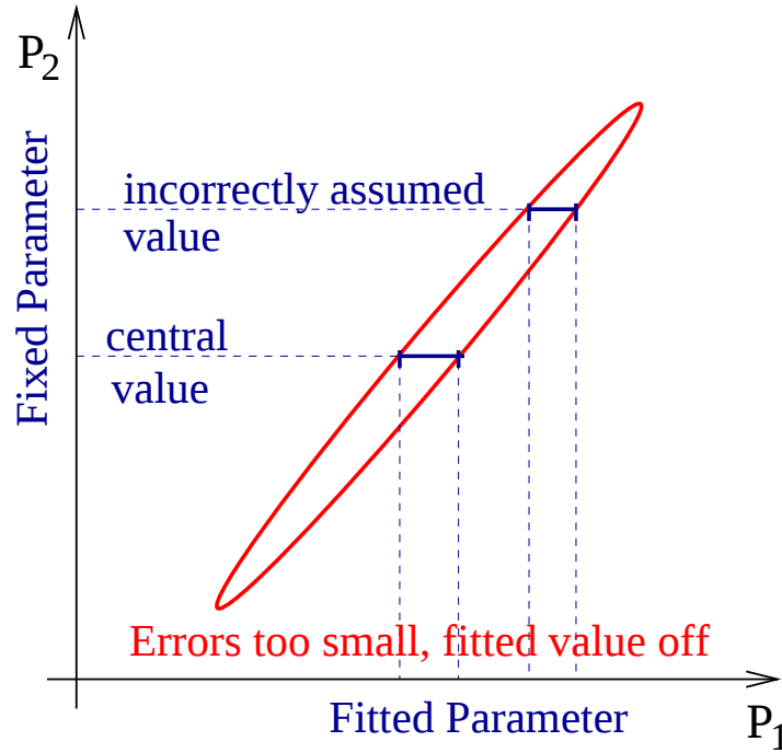
Figure 7.4: The effect of correlations among parameters on the uncertainty. If only parameter P_1 is fitted and P_2 is kept fixed, the uncertainty on P_1 is too small. Additionally, if P_2 is kept fixed on a slightly wrong value, the result on P_1 can be wrong, too.
