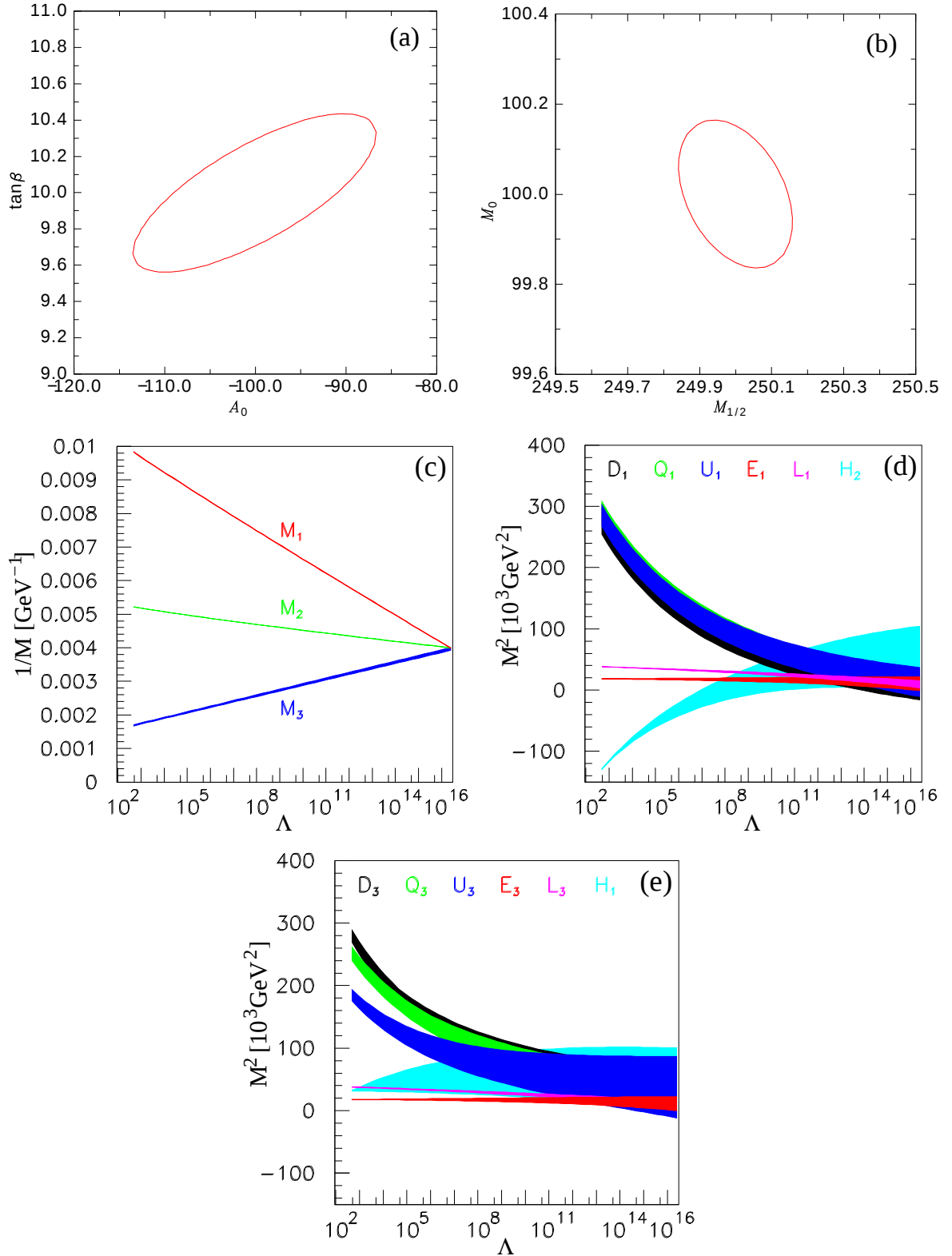
Figure 7.13: Determination of the mSUGRA parameters, using the results of the MSSM parameter fit from Tab. 7.2. In (a) and (b), the two-dimensional uncertainty contours of the results of a top-down fit of the mSUGRA parameters is shown. (c), (d) and (e) present the evolution of the MSSM parameters to \Lambda_{\text{GUT}} [174].
