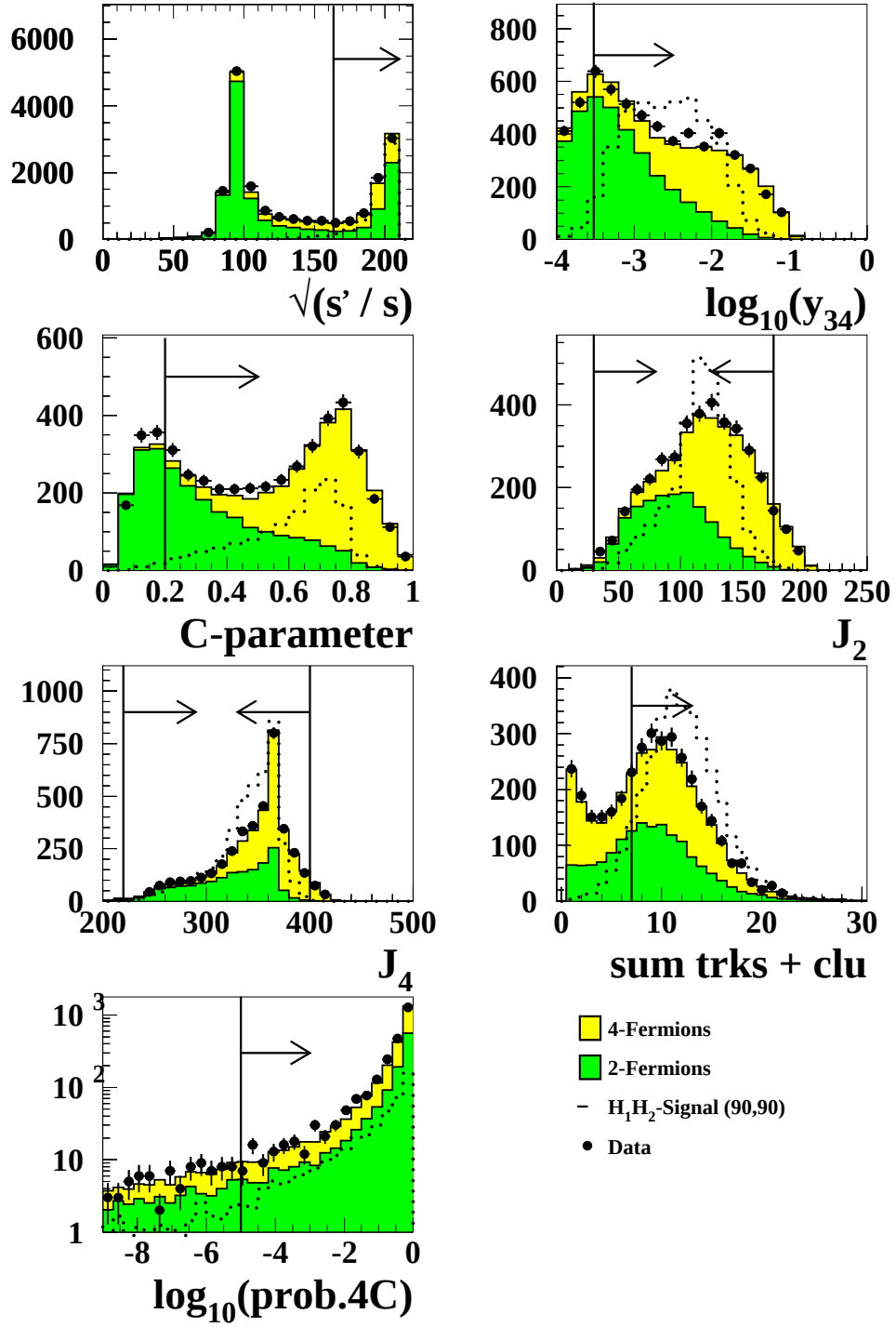
Figure 5.8: Distribution of the preselection variables in the search for e^+e^- \rightarrow \mathcal{H}_1\mathcal{H}_2 for light m_{\mathcal{H}_1} .
