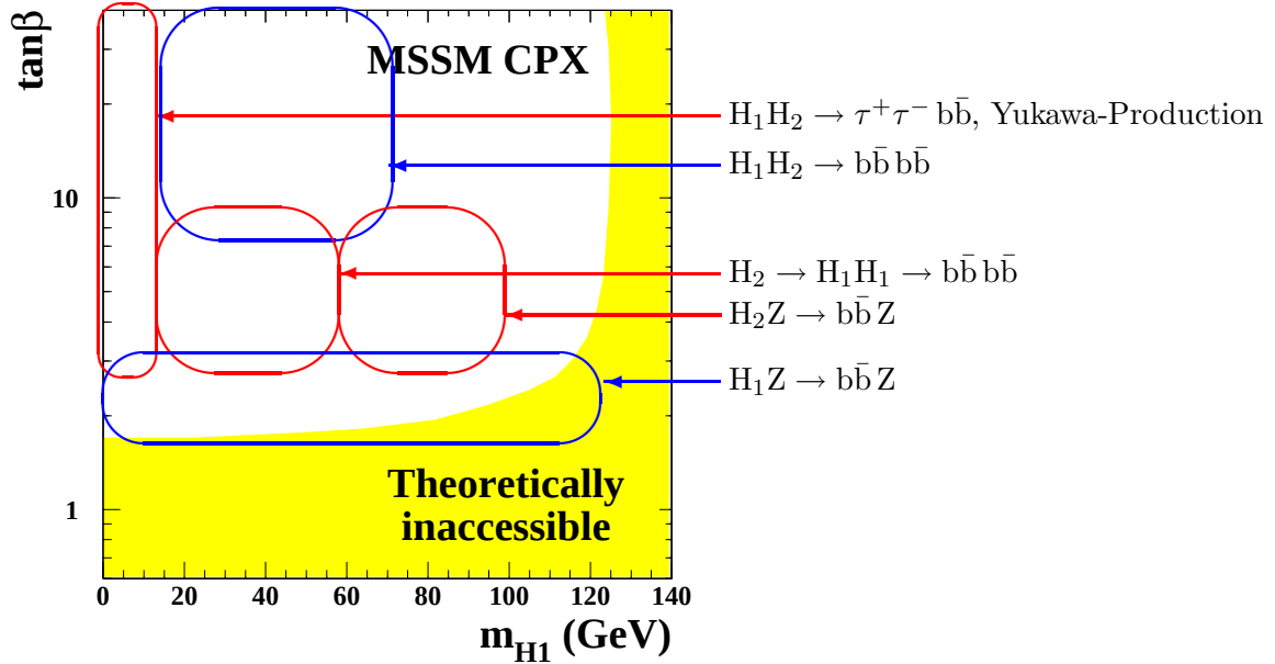
Figure 6.16: The use of the individual searches in the “CPX” scenario. In red, the areas are shown where the exclusion is difficult, although the Higgs boson is kinematically accessible.
