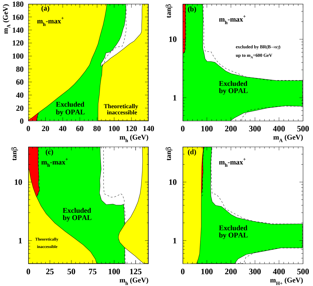
Figure 6.11: Results for the “ m_h\text{-max}^+ ” benchmark scenario described in the text of Section 6.4.1. See Fig. 6.8 for the notation.
