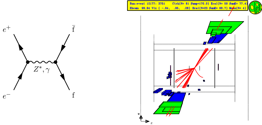
Figure 4.7: The e^+e^- \rightarrow q\bar{q} process at LEP. The events have a clear two-jet structure and have a balanced momentum sum.
