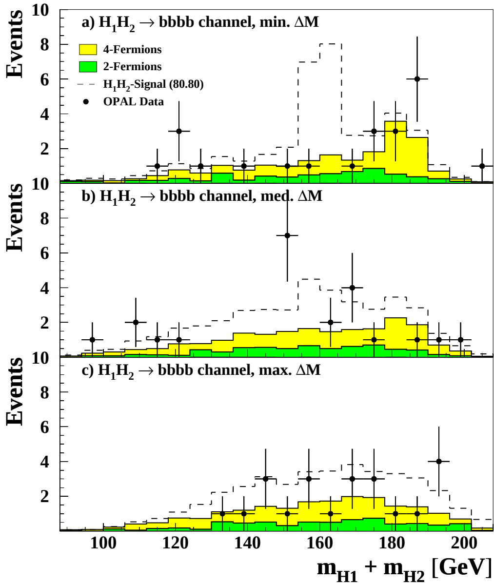
Figure 5.6: Mass distributions for heavy m_{H_1} . In (a), the sum of the reconstructed Higgs boson masses m_{H_1} + m_{H_2} is shown for the jet mass combination with the lowest \Delta m = m_{H_2} - m_{H_1} . Plot (b) shows m_{H_1} + m_{H_2} for the di-jet combination with intermediate \Delta m , and (c) shows the di-jet combination with largest \Delta m .
