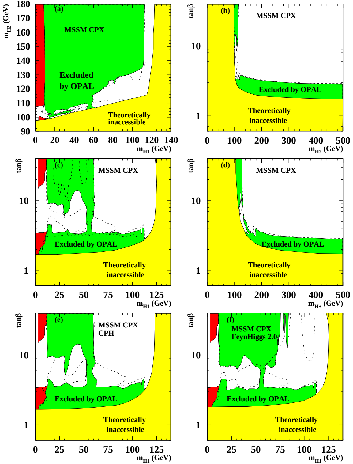
Figure 6.17: The “CPX” MSSM 95% CL exclusion areas. Excluded regions are shown for (a) the (m_{H_1}, m_{H_2}) plane, (b) the (m_{H_2}, \tan\beta) plane, (c) the (m_{H_1}, \tan\beta) plane and (d) the (m_{H^\pm}, \tan\beta) plane. Figure (e) shows the (m_{H_1}, \tan\beta) of the CPH calculation alone, (f) shows the same projection of the FEYNHIGGS 2.0 calculation. See Fig. 6.8 for the notation. The dash-dotted line in (c) shows the area excluded on the 99.9% confidence level. In (b) and (d) the area excluded by Z width constraints or by decay independent searches is too small to be displayed.
