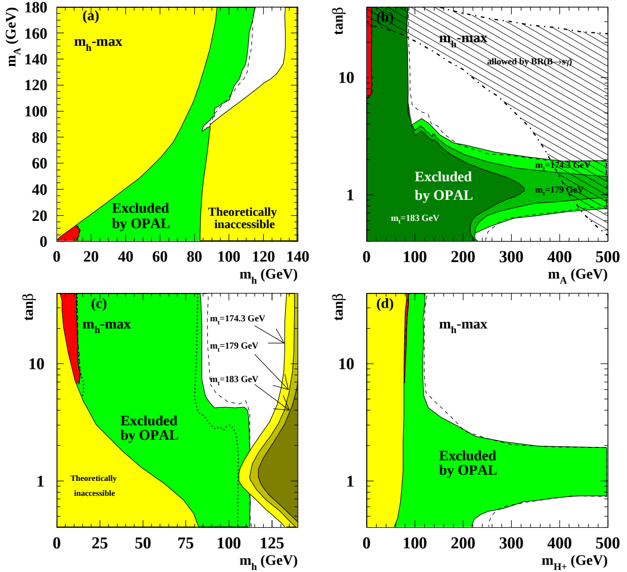
Figure 6.10: Results for the m_h -max benchmark scenario. See Fig. 6.8 for the notation. The dotted line in (c) shows the observed 99.9% confidence limit. The differently shaded regions in (b) show the exclusion for different values of m_{\text{top}} , as written in the Plot. The upper limit on m_h for different values of m_{\text{top}} is shown in (c), as expressed in the plot.
