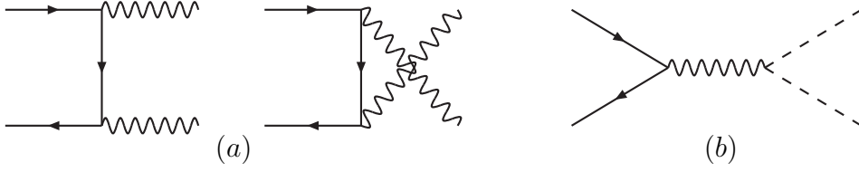
Figure 3.1: These diagrams represent (a) transverse and (b) longitudinal gauge boson pair production in fermion-antifermion annihilation at high energy in the Born approximation.
