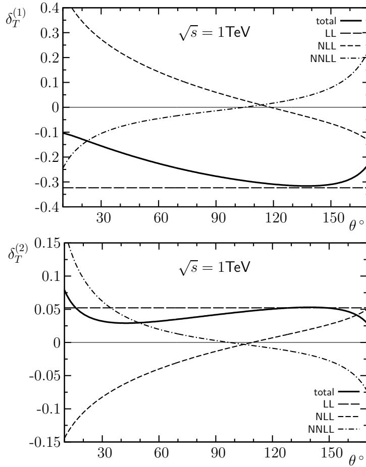
Figure 4.2: One-loop and two-loop corrections to the differential cross section relative to the Born approximation for the production of transversely polarized W bosons at \sqrt{s} = 1 \text{ TeV} .
