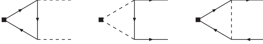
Figure 4.1: The one-loop diagrams contributing to the anomalous dimension matrix \zeta . The arrow lines correspond to the third generation quarks. The dashed lines correspond to the Higgs, neutral or charged Goldstone bosons. The black square represent an external singlet vector field
