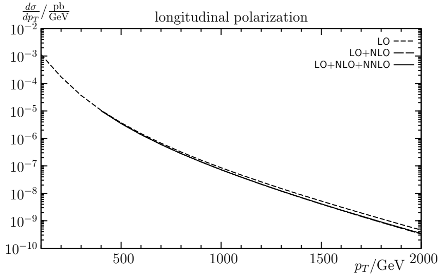
Figure 5.4: p_T distribution for the production of longitudinally polarized W pairs with same notation as fig. 5.3.
