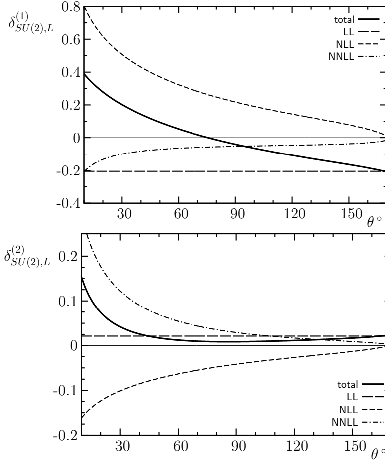
Figure 3.6: The one-loop and two-loop SU(2) corrections to the differential cross section relative to the Born approximation for the production of scalar bosons at \sqrt{s} = 1 TeV.
