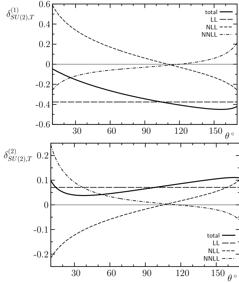
Figure 3.7: The one-loop and two-loop SU(2) corrections to the differential cross section relative to the Born approximation for the production of transversely polarized W bosons at \sqrt{s} = 1 TeV.
