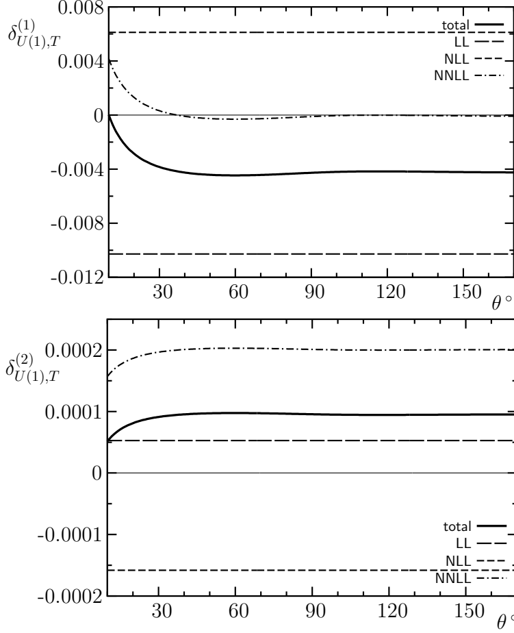
Figure 3.3: The one-loop and two-loop U(1)_Y corrections to the differential cross section relative to the Born approximation for the production of transversely polarized W bosons at \sqrt{s} = 1 TeV.
