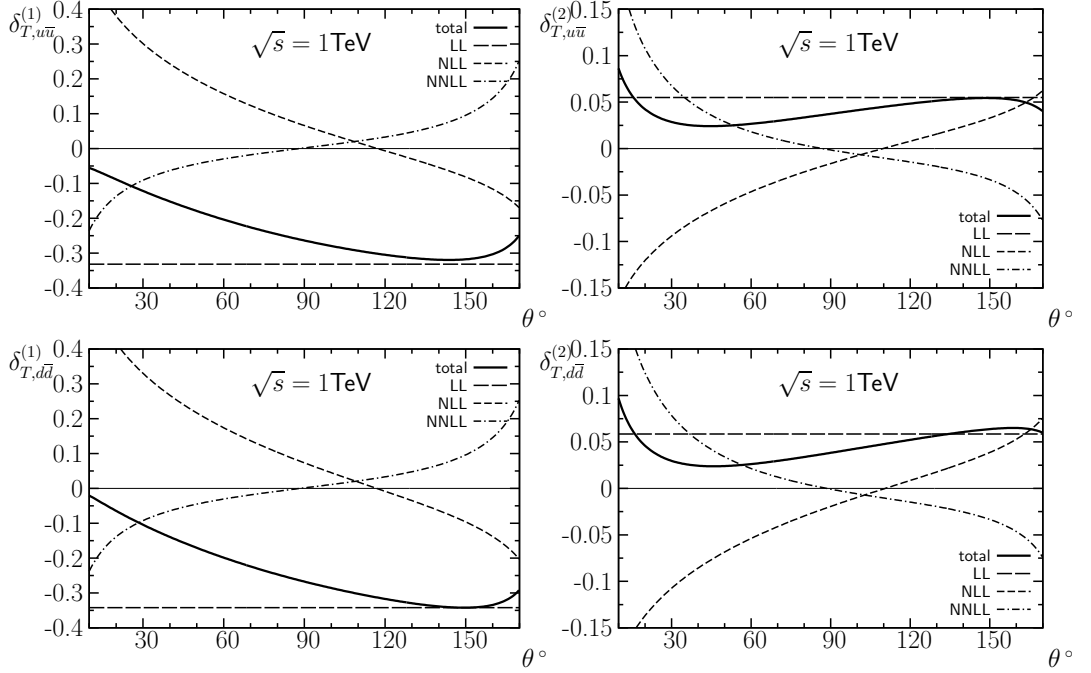
Figure 5.1: One-loop (left-hand side) and two-loop (right-hand side) corrections to the partonic differential distribution for the pair-production of transversely polarized W -boson with up-type (upper half) and down-type (lower half) quark initial states.
