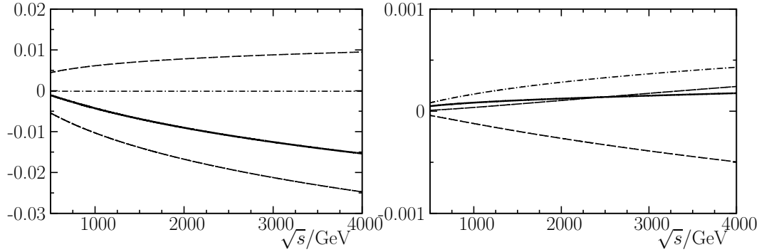
Figure 3.5: The same as fig. 3.4 but for the transverse case.
