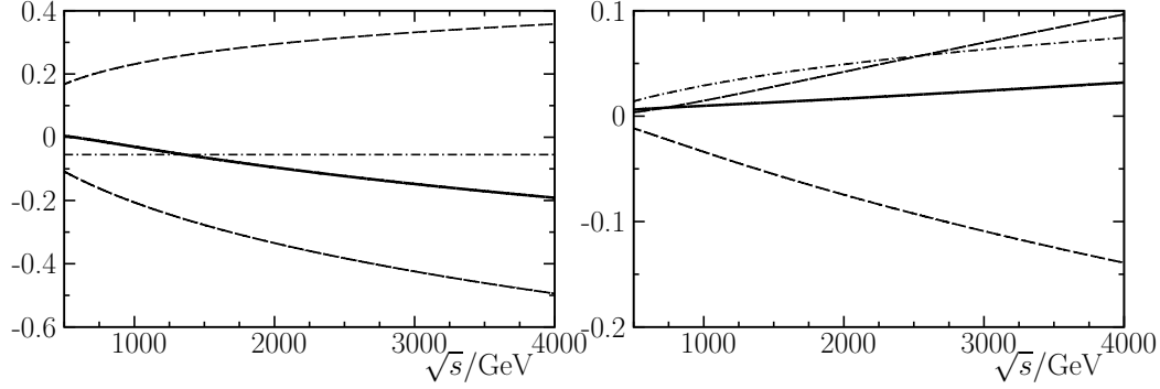
Figure 3.8: The one-loop (left diagram) and two-loop (right diagram) SU(2) corrections to the total cross section relative to the Born approximation for the production of scalar bosons. The long-dashed, short-dashed and dot-dashed lines denote the LL, NLL and NNLL corrections, as defined in the legend of figs. 3.6, 3.7
