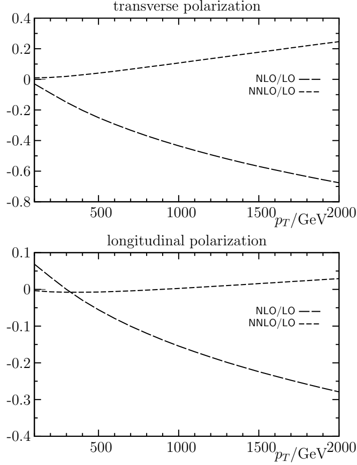
Figure 5.5: p_T distribution of one-loop and two-loop corrections relative to the leading order for the production of transverse and longitudinally polarized W pairs.
