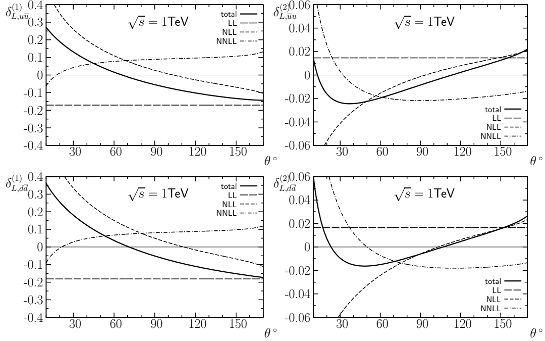
Figure 5.2: The same as fig. 5.1 but for the production of a pair of longitudinally polarized W -bosons.
