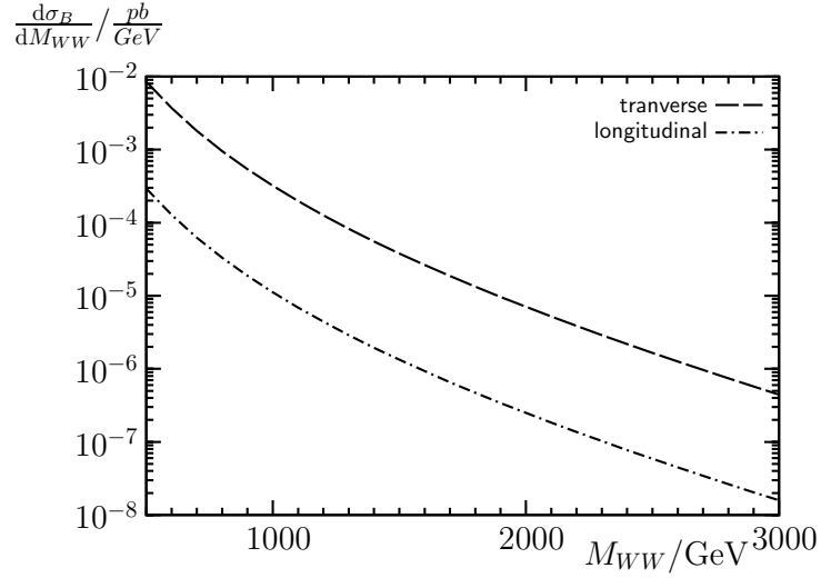
Figure 5.6: The invariant mass distribution relative to the Born approximation for the production of transversely and longitudinally polarized W pairs.
