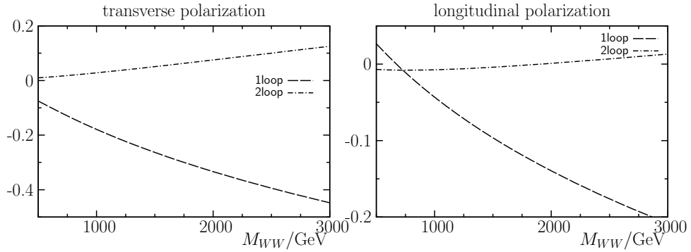
Figure 5.7: The electroweak one-loop and two-loop corrections to the invariant mass distribution relative to the Born approximation.
