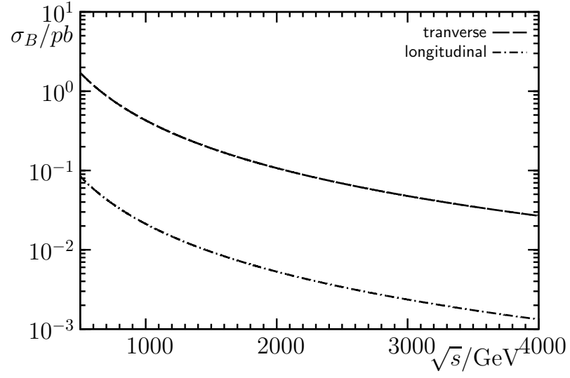
Figure 2.3: The total cross section at leading order with an angular cutoff of 30^\circ .
