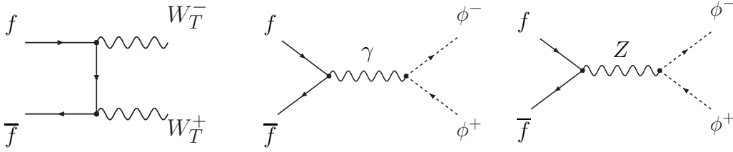
Figure 2.4: Diagrams contributing to the leading order cross section. The t -channel diagram corresponds to the production of transversely polarized W -boson, the s -channel to the production of Goldstone boson related to the corresponding longitudinally polarized W -bosons.
