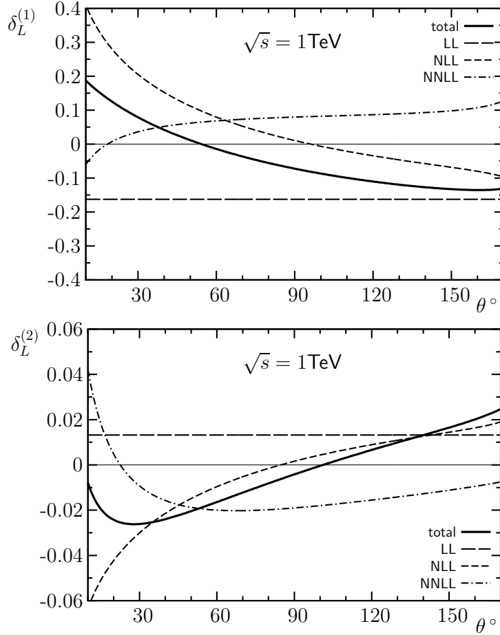
Figure 4.3: One-loop and two-loop corrections to the differential cross section relative to the Born approximation for the production of longitudinally polarized W bosons at \sqrt{s} = 1 \text{ TeV} .
