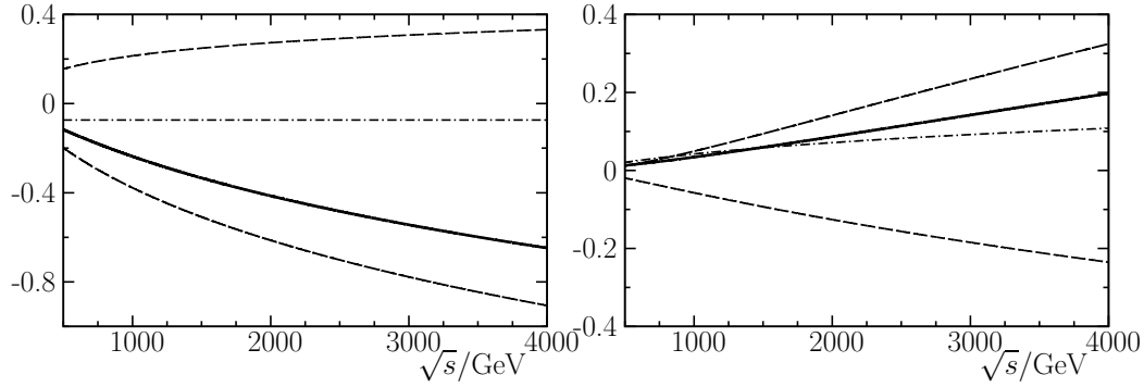
Figure 3.9: The same as fig. 3.4 but for the transverse case.
