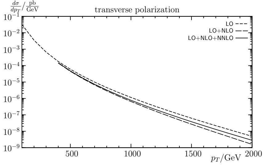
Figure 5.3: The p_T distribution for the production of transversely polarized W pairs. LO denotes the leading order contribution and NLO(NNLO) denotes the one-loop and two-loop corrections relative to the leading order.
