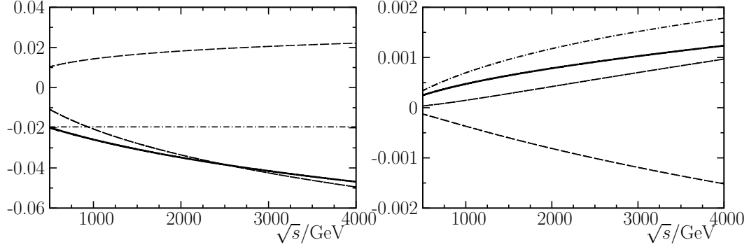
Figure 3.4: The one-loop (left diagram) and two-loop (right diagram) U(1)_Y corrections to the total cross section relative to the Born approximation for the production of scalar bosons. The long-dashed, short-dashed and dot-dashed lines denote the LL, NLL and NNLL corrections, as defined in the legend of figs. 3.2, 3.3
