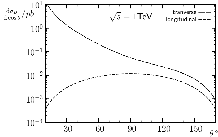
Figure 2.2: The differential distribution of the leading order cross section for pair-production of transverse and longitudinally polarized W -bosons in e^+e^- annihilation.
