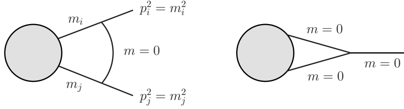
Figure 2.1: Diagrams leading to soft (left hand side) and collinear (right hand side) singularities
