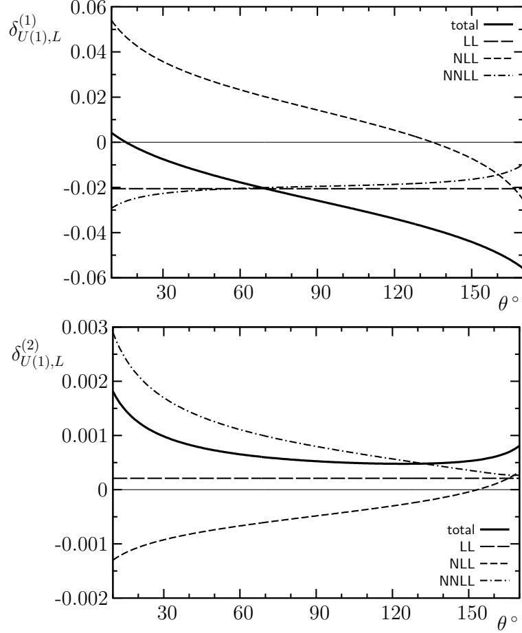
Figure 3.2: The one-loop and two-loop U(1)_Y corrections to the differential cross section relative to the Born approximation for the production of scalar bosons at \sqrt{s} = 1 TeV.
