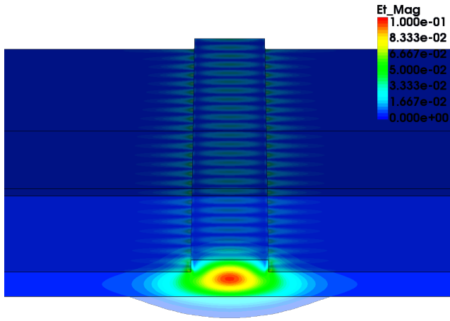
Fig. 9: |\vec{E}_T|^2 plot of a 10.0 \mu\text{m} -long device. Along direction of propagation there are amplitude fluctuations.
