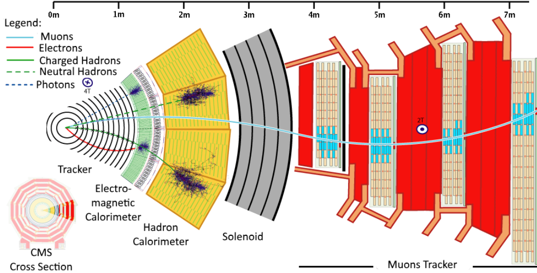
Figure 1.4: Cross section of one sector of the CMS barrel.
