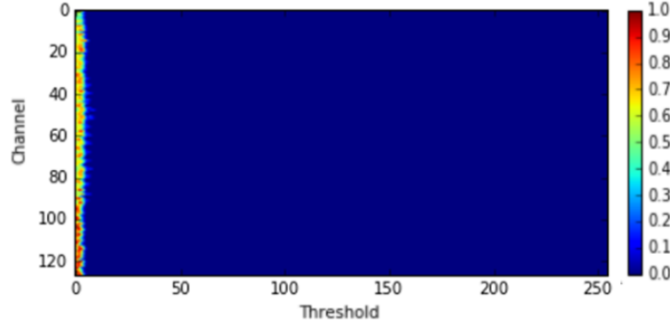
Figure 6.3: Threshold scan by channel for the VFAT on position 1.
