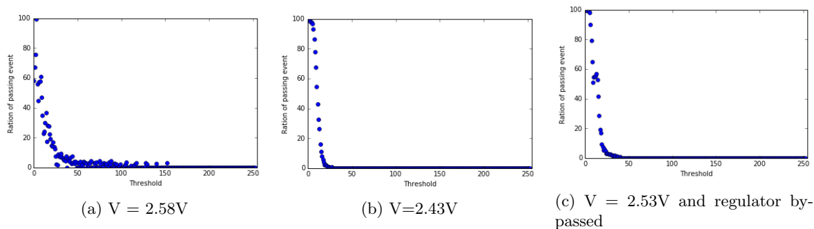
Figure 6.7: Effect of the LP38501 voltage regulator on the threshold scan depending of its use.
