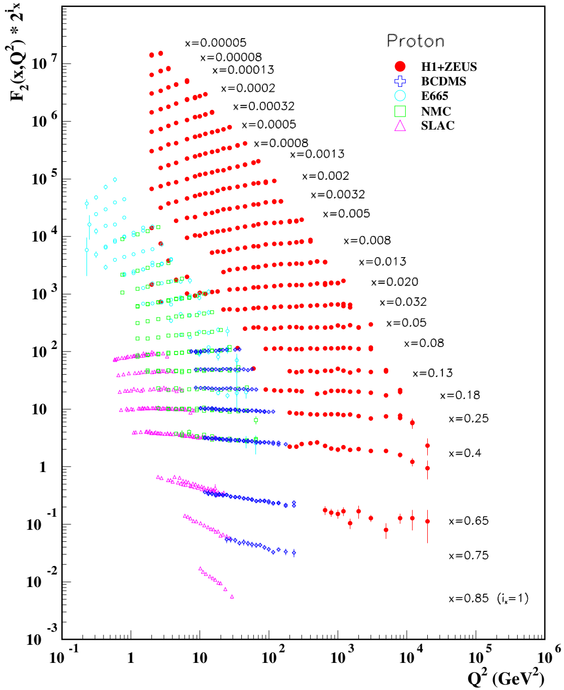
Figure 2.4: The proton structure function F_2 measured in electromagnetic scattering of electrons and positrons on protons (collider experiments H1 and ZEUS for Q^2 \geq 2 GeV 2 ), in the kinematic domain of the HERA data, and for electrons (SLAC) and muons (BCDMS, E665, NMC) on a fixed target. The data are plotted as a function of Q^2 in bins of fixed x . Some points have been slightly offset in Q^2 for clarity. The H1+ZEUS combined binning in x is used in this plot; all other data are rebinned to the x values of these data. For the purpose of plotting, F_2 has been multiplied by 2^{i_x} , where i_x is the number of the x bin, ranging from i_x = 1 ( x = 0.85 ) to i_x = 24 ( x = 0.00005 ). The plot is taken from [7].
