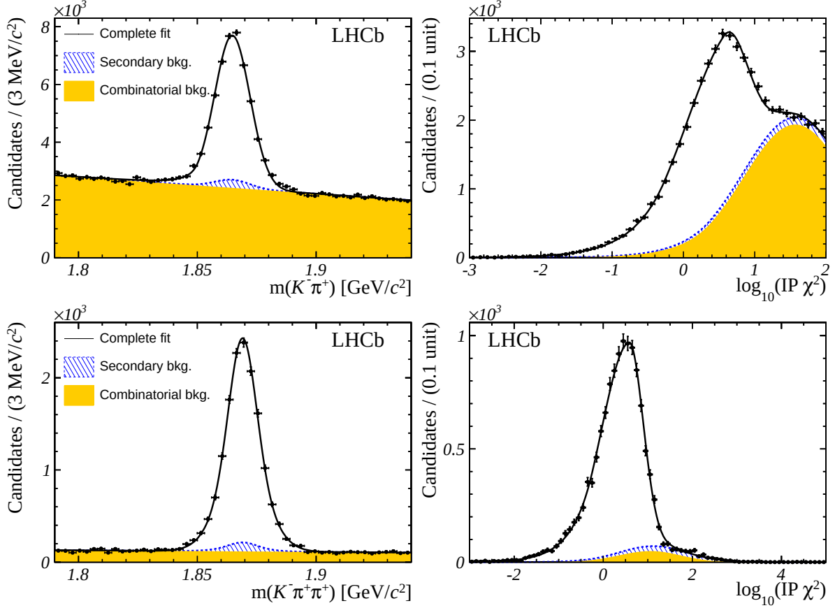
Figure 3.12: Mass and \log_{10}(\text{IP} \chi^2) distributions for selected D^0 \rightarrow K^- \pi^+ and D^+ \rightarrow K^- \pi^+ \pi^+ candidates from the LHCb measurement of prompt charm production [135] showing the masses of the D^0 candidates (top left), \log_{10}(\text{IP} \chi^2) distribution of D^0 candidates (top right), masses of the D^+ candidates (bottom left) and \log_{10}(\text{IP} \chi^2) distribution of D^+ candidates (bottom right). Projections of likelihood fits to the full data samples are shown with components as indicated in the legends.
