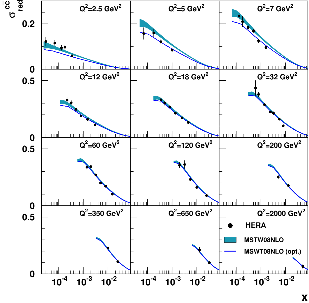
Figure 6.20: Combined measurements of \sigma_{red}^{c\bar{c}} (closed circles) shown as a function of x for particular Q^2 , compared to the prediction by MSTW at NLO. The predictions obtained using the standard (optimised) parametrisation are represented by the shaded bands (solid lines). The uncertainties for the optimised parametrisation are not evaluated by the authors of the predictions but are expected to be of same size as those for the standard parametrisation.
