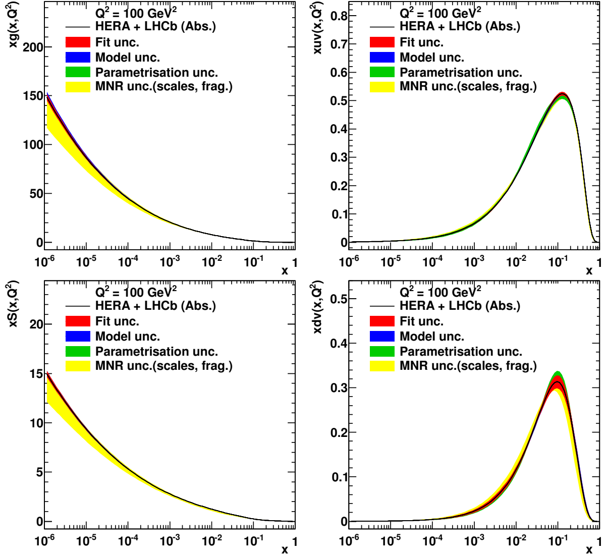
Figure F.5: The individual contributions to the uncertainties of the gluon (top left), u -valence (top right), sea (bottom left) and d -valence (bottom right) distributions at Q^2 = 100 \text{ GeV}^2 obtained in the fit with the HERA and LHCb data using the ‘LHCb Abs’ approach.
