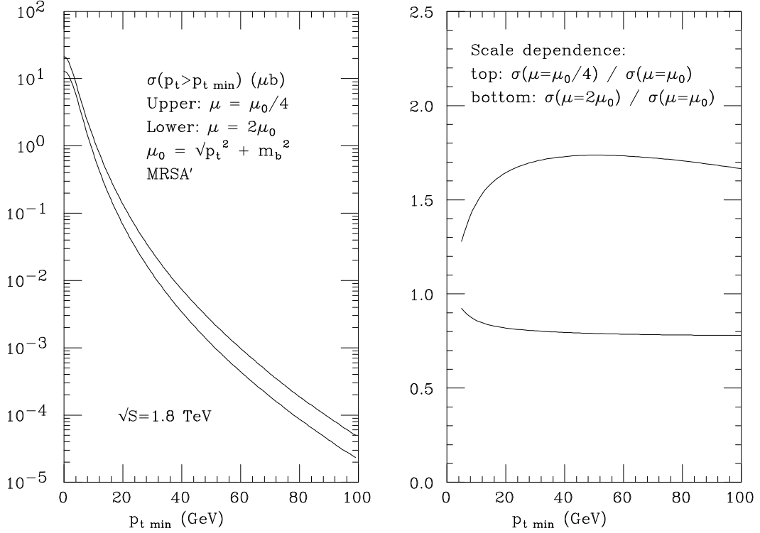
Figure 2.10: Scale dependence of the inclusive p_T distribution for b quarks, in p\bar{p} collisions at \sqrt{s} = 1.8 TeV. The plot is taken from [41].
