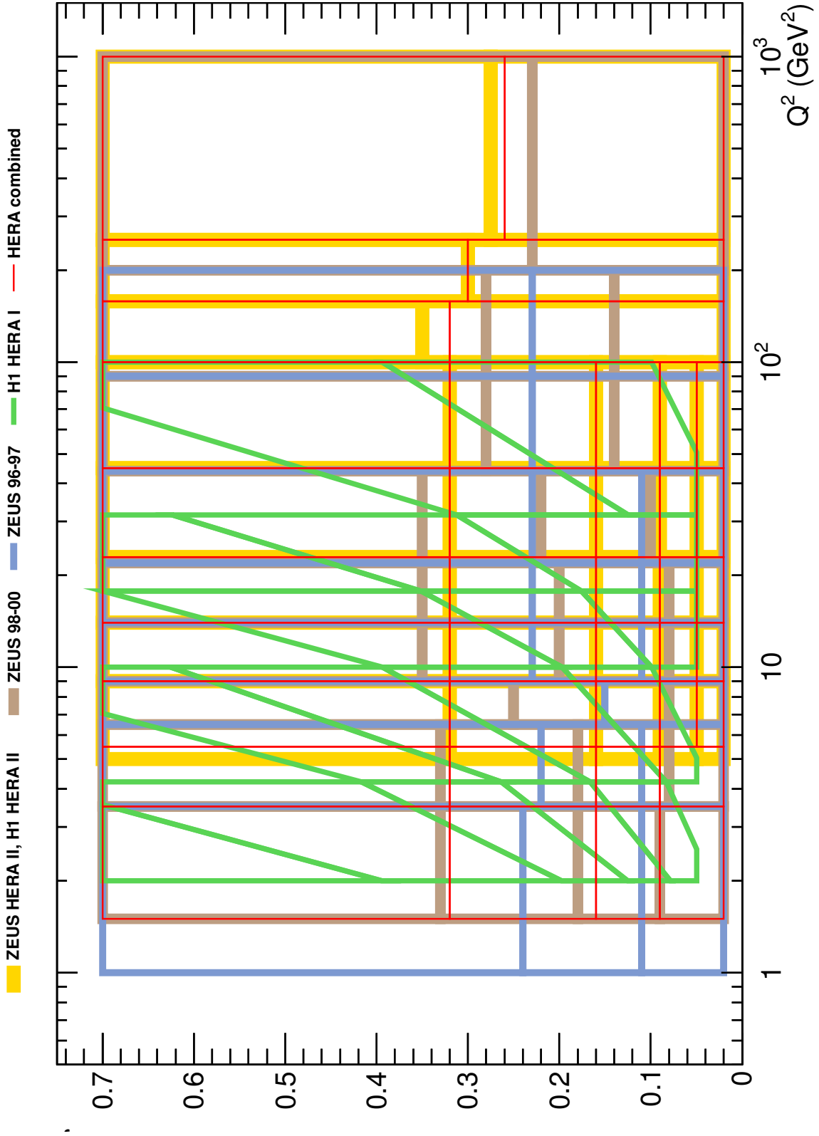
Figure 6.7: Overlap of the binning schemes for the D^{*+} double-differential cross section from input measurements and the new binning scheme.
