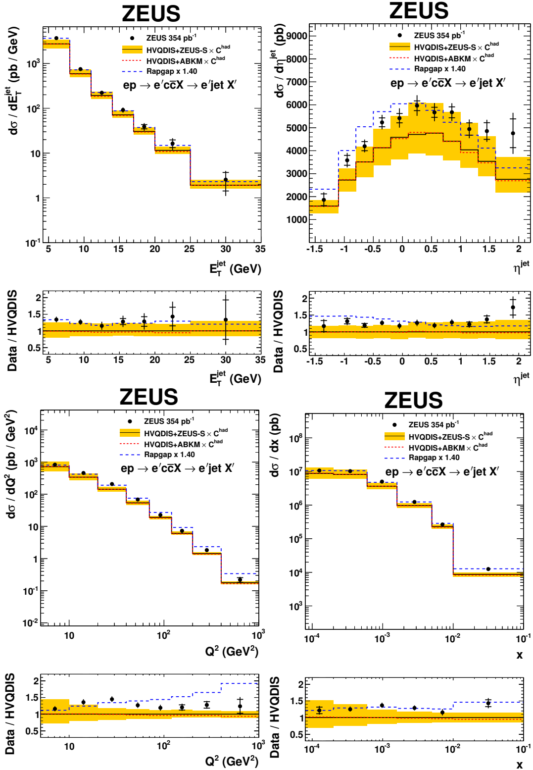
Figure 3.10: Differential cross section for inclusive jet production in charm events as a function of E_T^{\text{jet}} (top left), \eta^{\text{jet}} (top right), Q^2 (bottom left) and x (bottom right) measured in [19]. The data are compared to the NLO predictions obtained in the FFNS (HVQDIS) with different input PDFs and to the predictions from MC RAPGAP.
