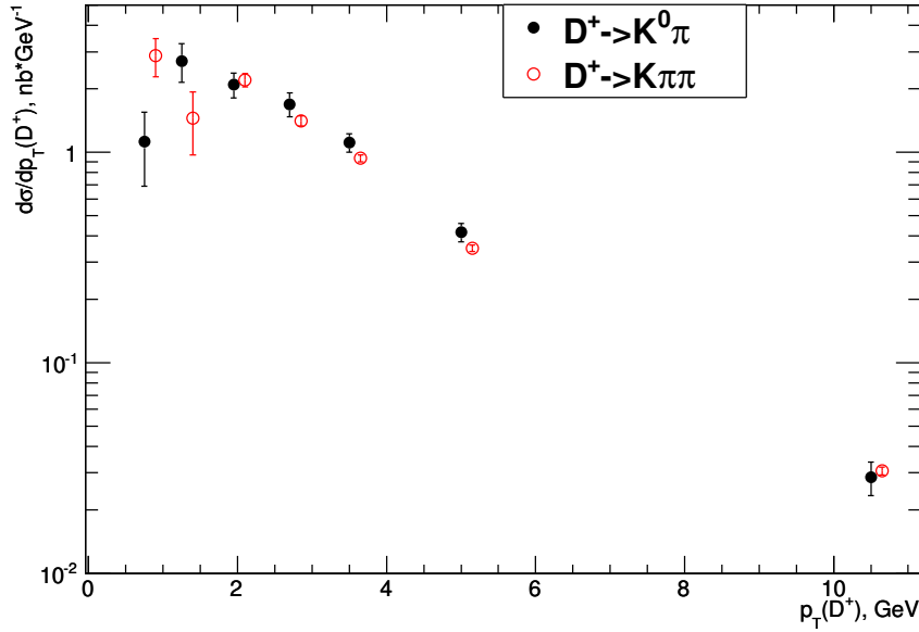
Figure B.17: The differential cross section as a function of p_T(D^+) , determined using decay channels D^+ \rightarrow K_S^0(\pi^+\pi^-)\pi^+ (filled circles) and D^+ \rightarrow K^-\pi^+\pi^+ (empty circles), shown with a small horizontal offset for better visibility.
