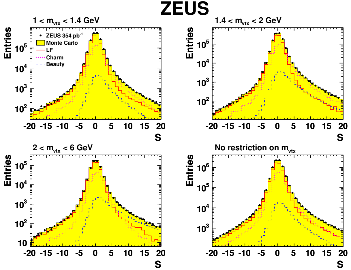
Figure 3.9: Distributions of the decay-length significance, S , for different bins of the secondary-vertex mass, m_{\text{vtx}} : 1 < m_{\text{vtx}} < 1.4 \text{ GeV} (top left), 1.4 < m_{\text{vtx}} < 2 \text{ GeV} (top right), 2 < m_{\text{vtx}} < 6 \text{ GeV} (bottom left) and no restriction on m_{\text{vtx}} (bottom right) from the ZEUS vertex measurement [19]. The data are compared to the sum of all MC distributions. The individual contributions from the beauty, charm and light-flavour MC subsamples are shown separately.
