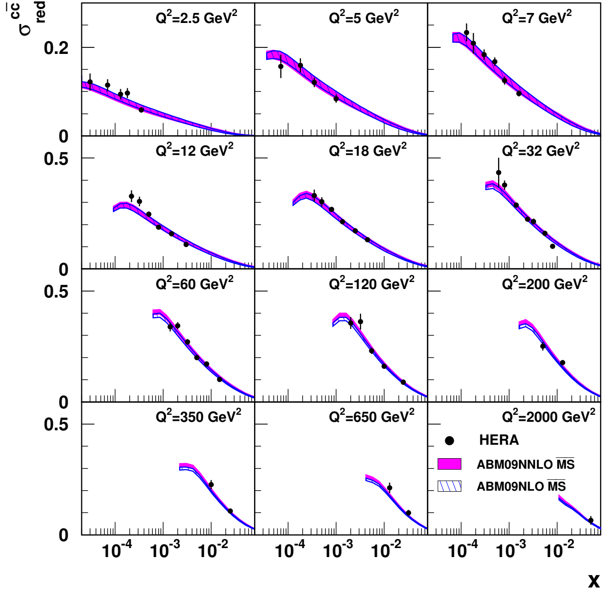
Figure 6.19: Combined measurements of \sigma_{red}^{c\bar{c}} (closed circles) shown as a function of x for particular Q^2 , compared to the prediction by the ABM group at NLO (hashed band) and NNLO (shaded band) in the FFNS using the \overline{MS} definition for the charm-quark mass.
