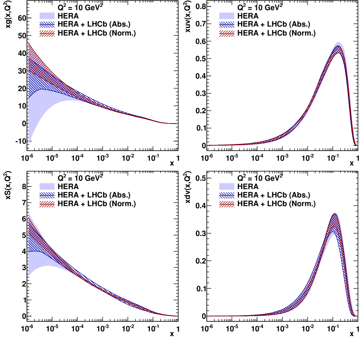
Figure 7.20: The gluon (top left), u -valence (top right), sea (bottom left) and d -valence (bottom right) distributions at Q^2 = 10 \text{ GeV}^2 obtained in the fit with the HERA-only, HERA and LHCb absolute, and HERA and LHCb normalised data. The widths of the bands represent the total uncertainties.
