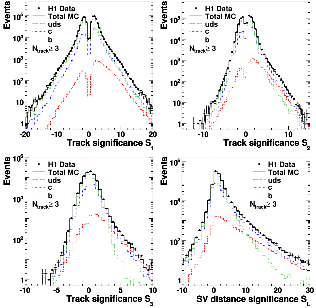
Figure 3.8: Distributions of discriminating variables from the H1 vertex measurement [141]: the impact-parameter significances, defined as the significance of the track with the highest, S_1 , (top left), second highest, S_2 , (top right) and third highest, S_3 , (bottom left) absolute significances, respectively, and the secondary-vertex significance, S_L , (bottom right). The data are compared to the MC expectation, obtained after applying the scale factors from the fit to the complete data sample. The charm, beauty and light-flavour contributions are shown separately.
