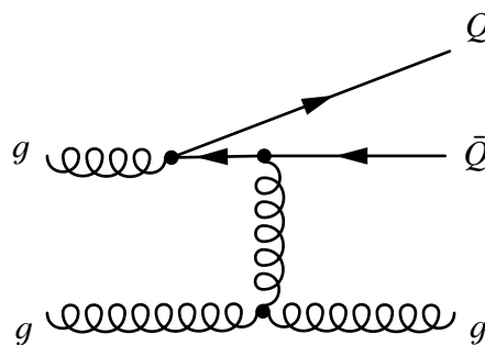
Figure 7.5: An example of the flavour-excitation diagram.
