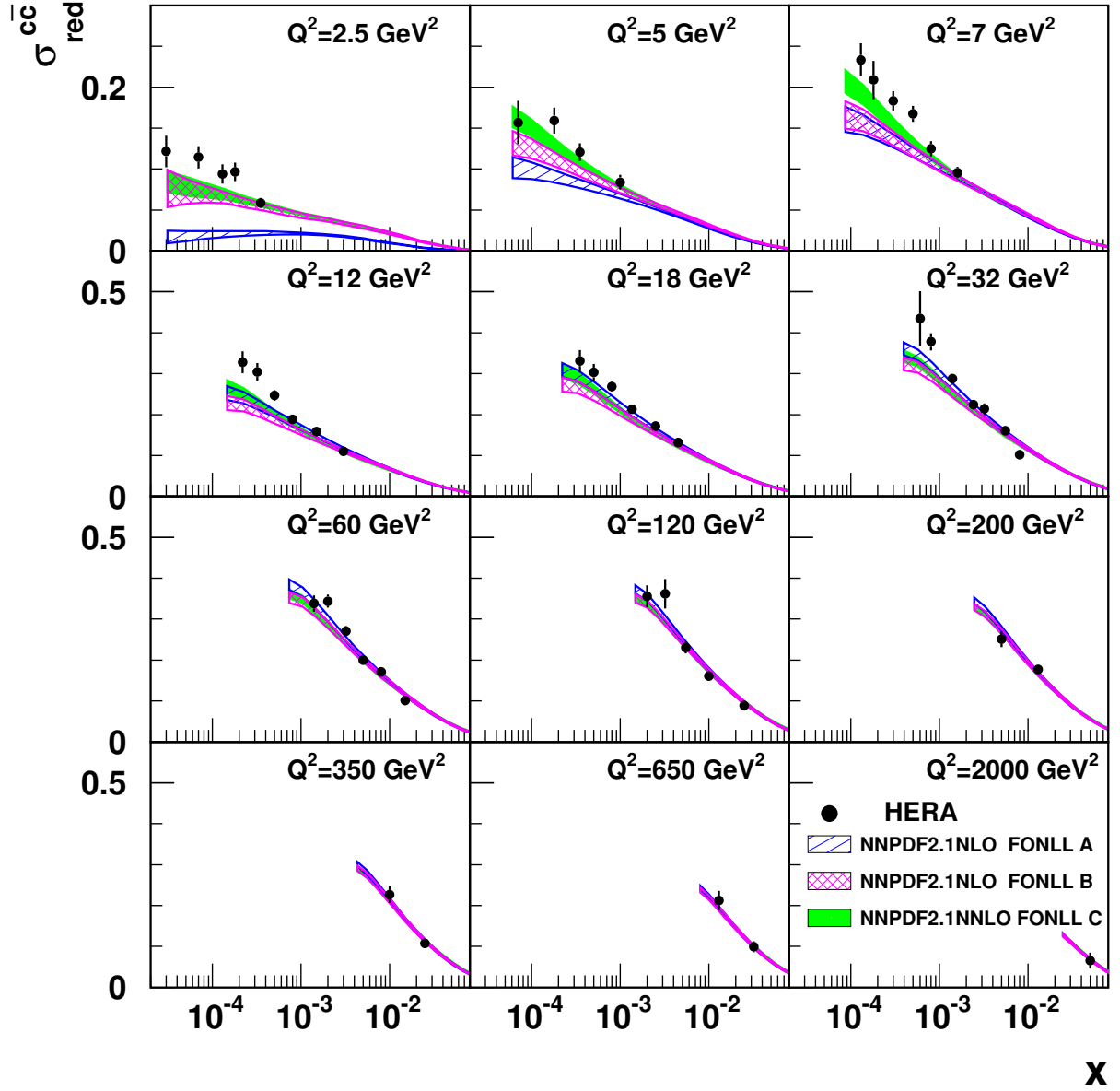
Figure 6.23: Combined measurements of \sigma_{red}^{cc} (closed circles) shown as a function of x for particular Q^2 , compared to the predictions by NNPDF. The predictions from NNPDF2.1 in FONLL-A, -B and -C schemes are available with their uncertainties and are represented by bands with different hatch styles.
