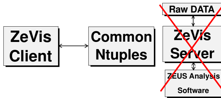
Figure 4.8: The architecture of CN-ZeVis.
