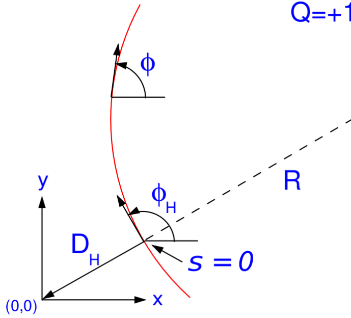
Figure B.24: Parametrisation of the track helix.
