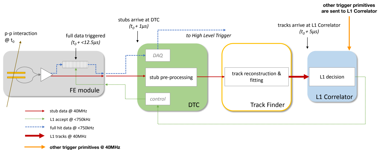
FIGURE 2.9. Illustration of dataflow and latency requirements from p_T -modules through to the off-detector electronics dedicated to forming the L1 trigger decision [56].
