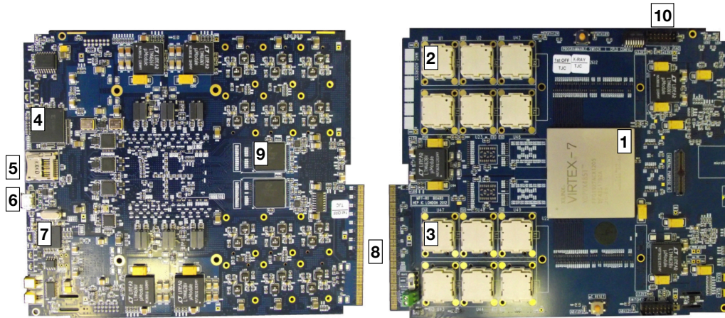
FIGURE 3.6. Photograph of the MP7 processing card [60]. The top side of the card is shown on the right hand side, and the bottom side of the card is shown on the left hand side. The optics and heat sinks are not mounted in these images. Some of the important components are labelled as follows: (1) the V7-690 FPGA; (2) six Avago MiniPOD transceivers; (3) six Avago miniPOD receivers; (4) the Xilinx CoolRunner-II XC2C256 CPLD [66], used for JTAG and boot management; (5) the USB-2 interface; (6) the microSD card interface; (7) the ATMEL microcontroller; (8) the MicroTCA backplane connector; (9) two 72 Mbit QDR-II SRAM chips; (10) CPLD and JTAG interface.
