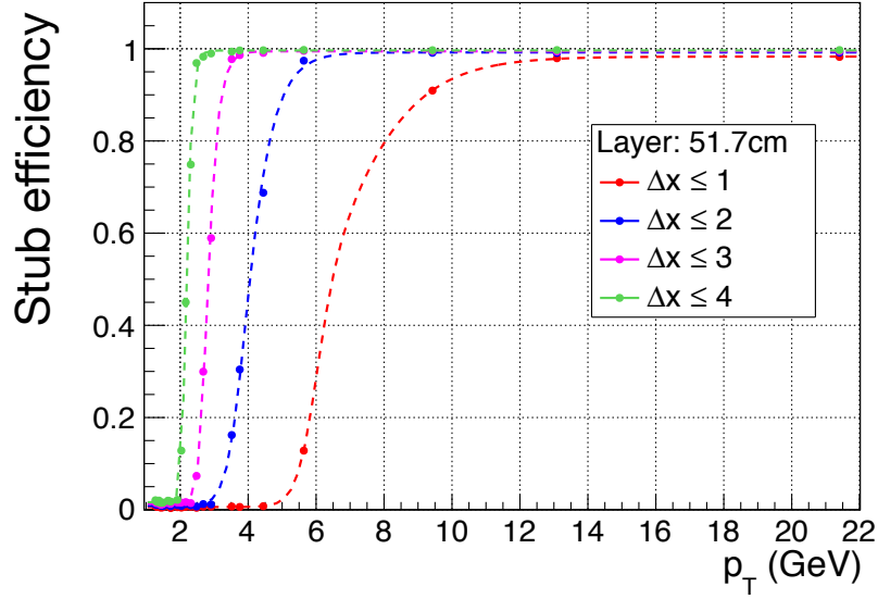
FIGURE 2.8. Stub reconstruction efficiency of a PS micro-module, the prototype MaPSA, at a 120 GeV proton test beam, at FNAL [31]. The denominator is determined by tracks reconstructed offline. This fraction is given as a function of p_T (at a reference radius of 51.7 cm), for values of \Delta x , the number of macro-pixels between the clusters in the top and bottom module sensor.
