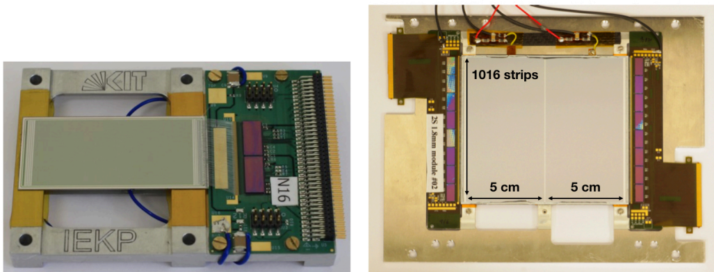
FIGURE 2.5. (Right) A full sized 2S module prototype (1.8 mm sensor spacing variant), equipped with eight CBC prototype chips, and two 10 cm long silicon strip sensors [31]. (Left) A 2S mini-module, assembled from a small prototype hybrid containing two prototype CBC readout chips, and two 5 cm long strip sensors mounted in an aluminium frame [31].
