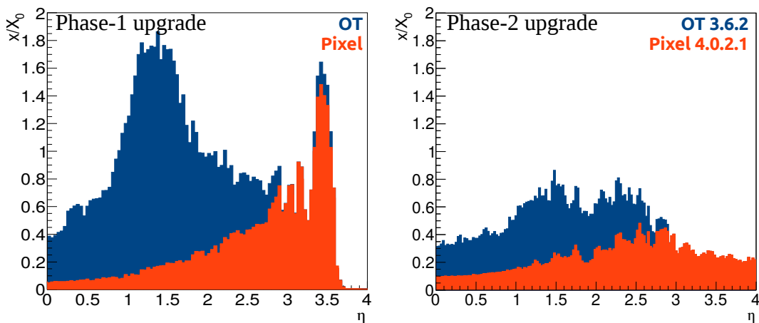
FIGURE 2.3. Material budget of the current (Phase I) tracker (left) and the proposed Phase II tracker with tilted barrel geometry (right). [31]. Material in the Inner Tracker is shown in red, and material in the outer tracker is in blue. The histograms are stacked.
