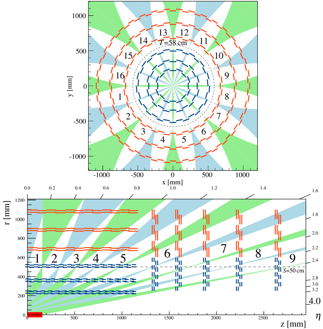
FIGURE 4.11. The segmentation of the tracker volume into \phi sub-sectors (upper) and \eta sub-sectors (lower), as used within the firmware implementation of the Hough transform preprocessor [56]. The numbered areas in white represent the regions that are associated with only one sector, whereas the coloured areas (where there is no difference in meaning between green or blue) represent the overlap region between neighbouring sectors where stubs may need to be assigned to both sectors. The two cylinders mentioned in the text of radius T = 58\text{ cm} and S = 50\text{ cm} , are indicated by dashes in the top and bottom figures, respectively.
