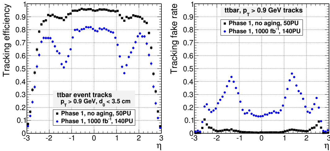
FIGURE 2.1. Tracking efficiency (left) and fake rate (right) for the current CMS tracker at 50 pileup without ageing (black), and at 140 pileup with ageing (blue) [31].
