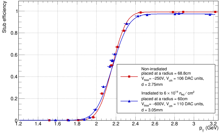
FIGURE 2.7. The stub turn on curve. Stub reconstruction efficiency for an irradiated (blue), and non-irradiated (red) 2S mini-module, as a function of p_T [31]. Irradiation fluence was 6 \times 10^{14} n_{eq}/cm^2 . The threshold setting V_{cth} , sensor spacing d , and bias voltage V_{bias} are given in the legend for each module. The V_{cth} values used correspond to about 4,900 and 3,500 electrons for the unirradiated, and irradiated module respectively. As the modules have different sensor spacing, different radii (68.8 cm and 60 cm) were used to calculate a p_T from the angle of incidence, using Eqn. 2.4.
