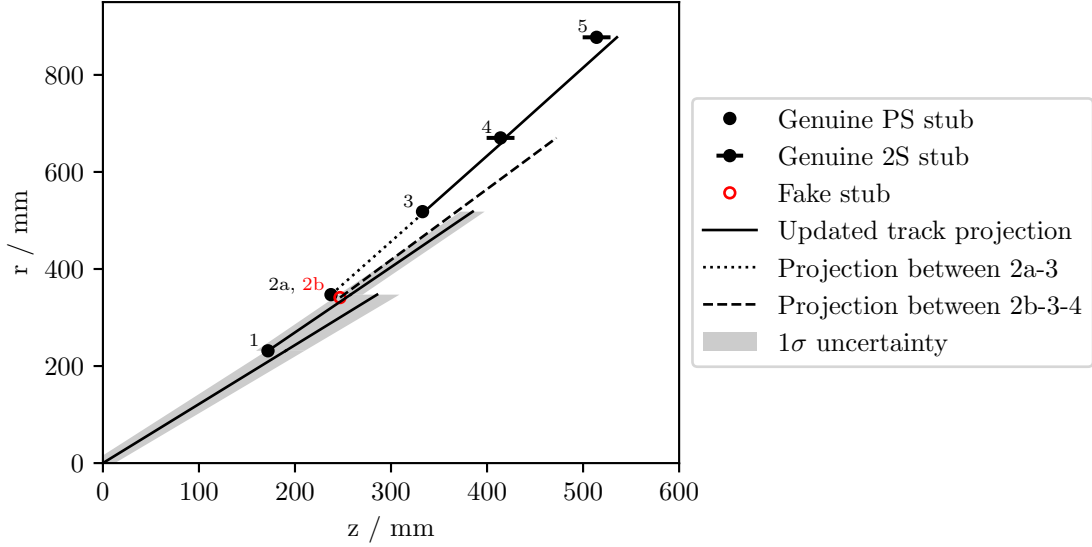
FIGURE 5.4. An example of the Kalman filter fitting procedure for an HT candidate in the barrel, shown in the r - z plane [56]. Genuine stubs are those associated with the same simulated charged particle, and fake stubs are those which are not. Line segments represent the fitted track trajectory at that point of the fit, updating with increasing radius, with the shaded area around the line showing one standard deviation of the track parameter estimate. Dashed track segments highlight the different result after fitting with stub 2a or 2b. The state that includes stub 2b is rejected after propagation to stub 4, due to failing a \chi^2 cut in two consecutive layers.
