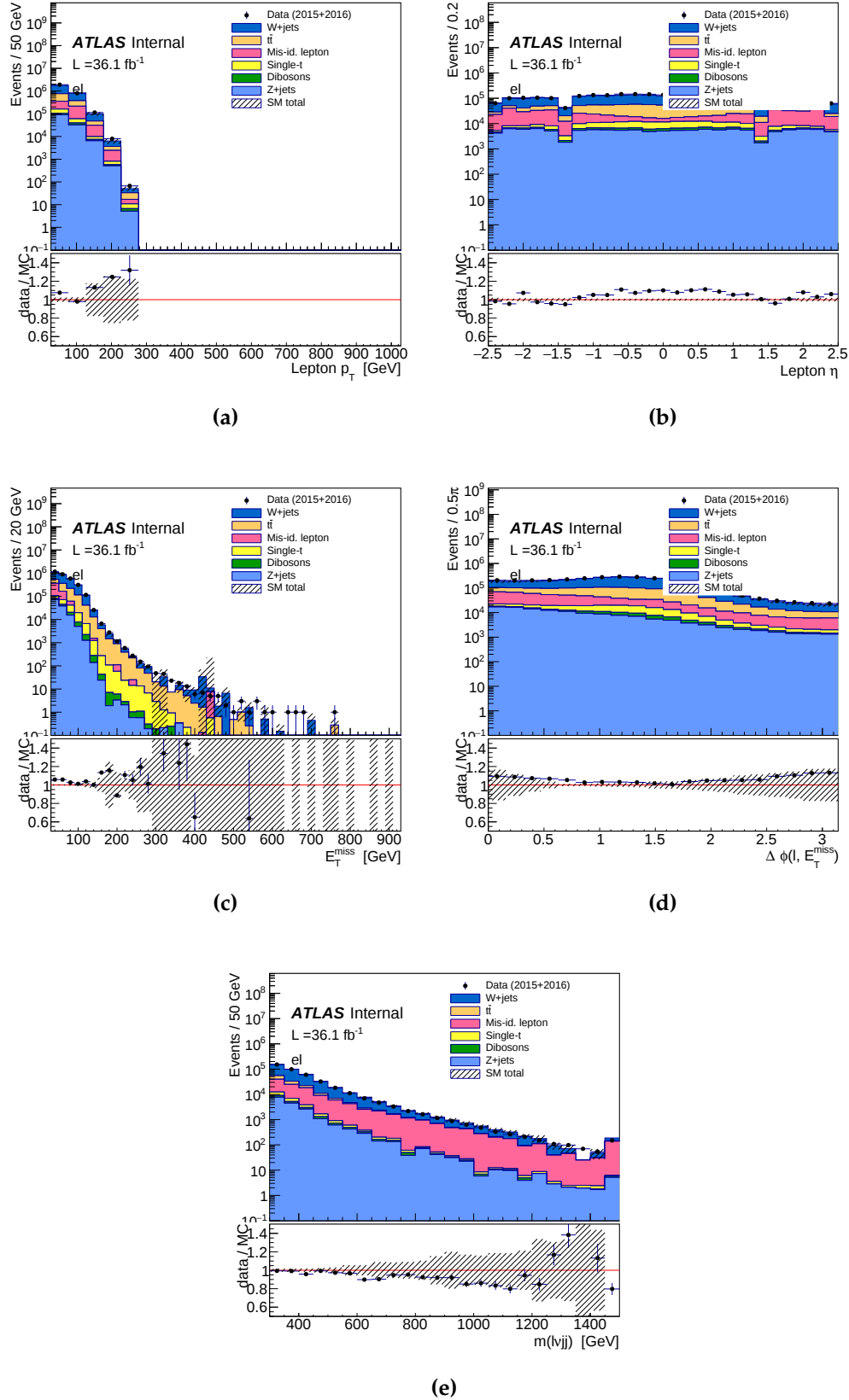
Figure 3.21.: The distribution of lepton p_T , \eta , E_T^{\text{miss}} , \Delta\phi(\ell, E_T^{\text{miss}}) , and m_{WV} in validation region with p_T(l\nu) < 150 \text{ GeV} in electron channel with multijet background
