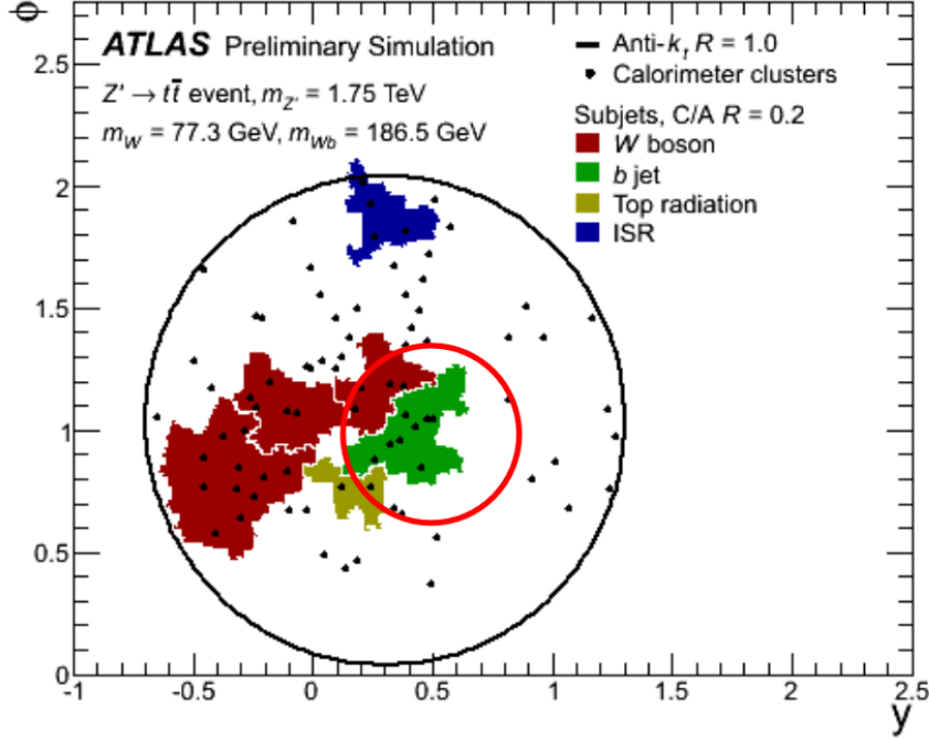
Figure 6.7.: The comparison of the Run 2 (red circle) and Run 3 (black circle) L1Calo jet ROIs for an HVT Z' \rightarrow t\bar{t} event. The Z' boson was given a high mass, so the two top quarks were highly boosted and got close to each other. They would form a large-R jet in the offline reconstruction [126].
