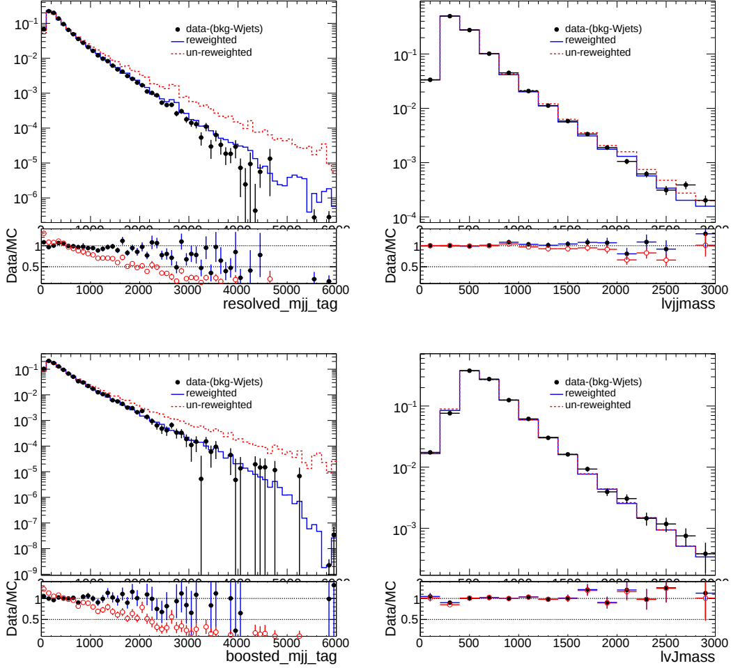
Figure 5.10.: Comparison of m^{VBS} (as resolved_mjj in the plots) and m_{VV} (as lvjjmass in resolved plots and lvJmass in boosted plots) distributions before and after the m^{VBS} reweighting for events in the resolved (top) and boosted (bottom) W+jets control regions
