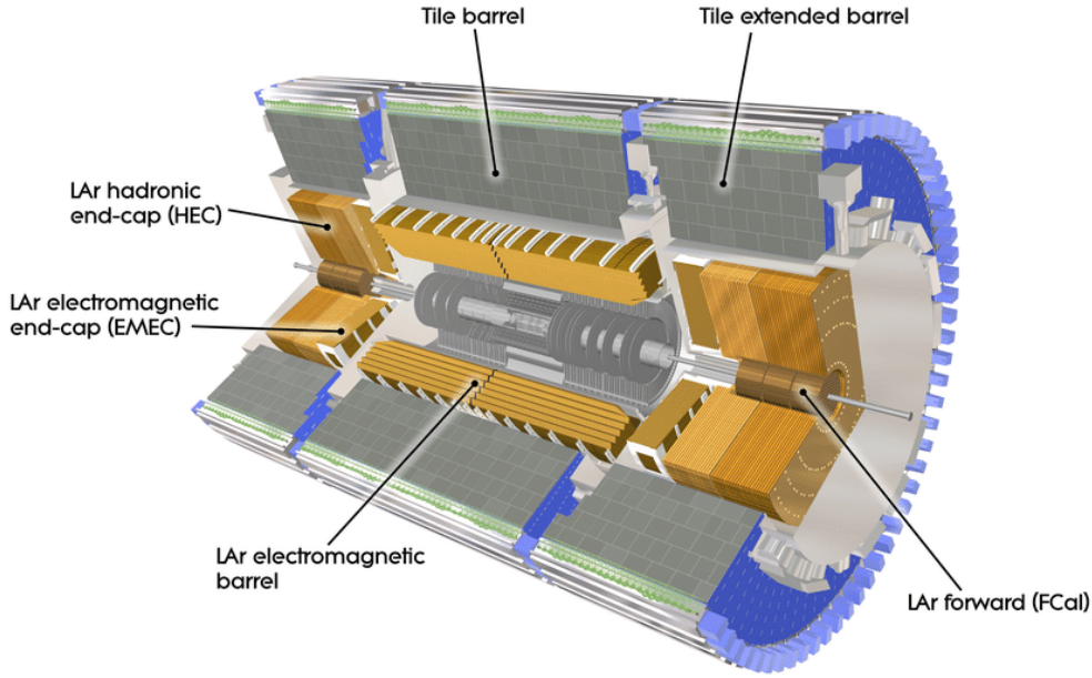
Figure 2.9.: The calorimeter system of the ATLAS detector from [?]
