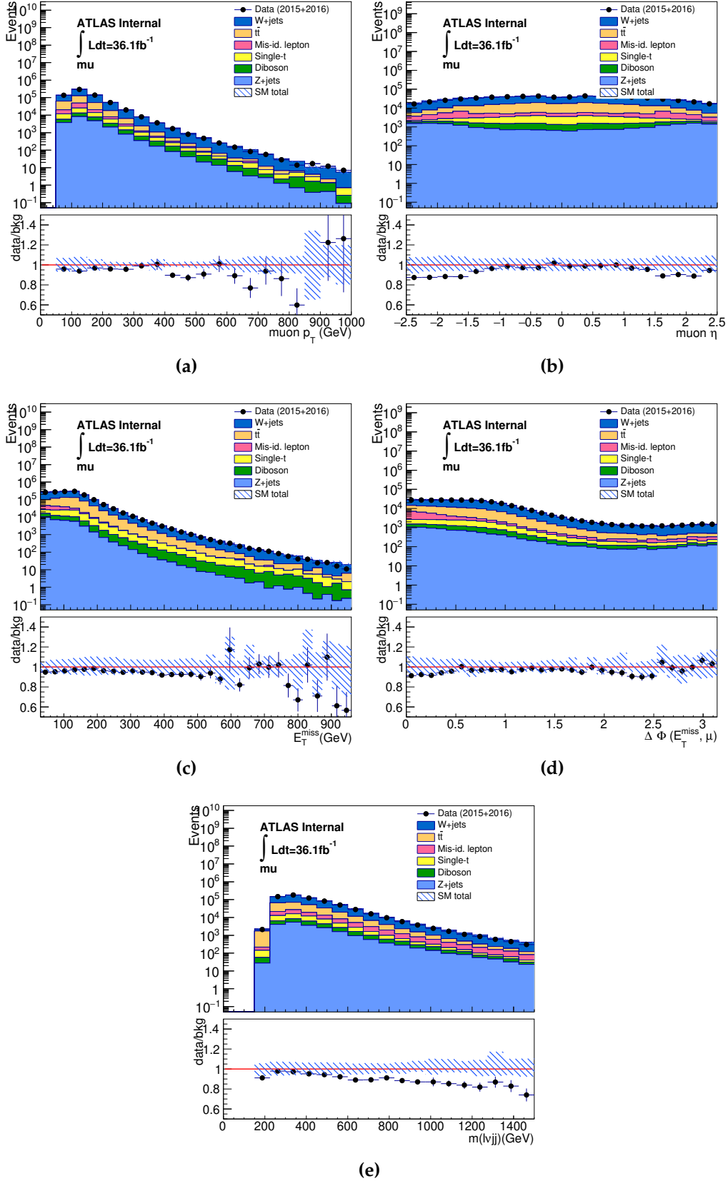
Figure 3.22.: The distribution of lepton p_T , \eta , E_T^{miss} , \Delta\phi(\ell, E_T^{miss}) , and m_{WV} in validation region with p_T(l\nu) > 150\text{GeV} in muon channel with multijet background
