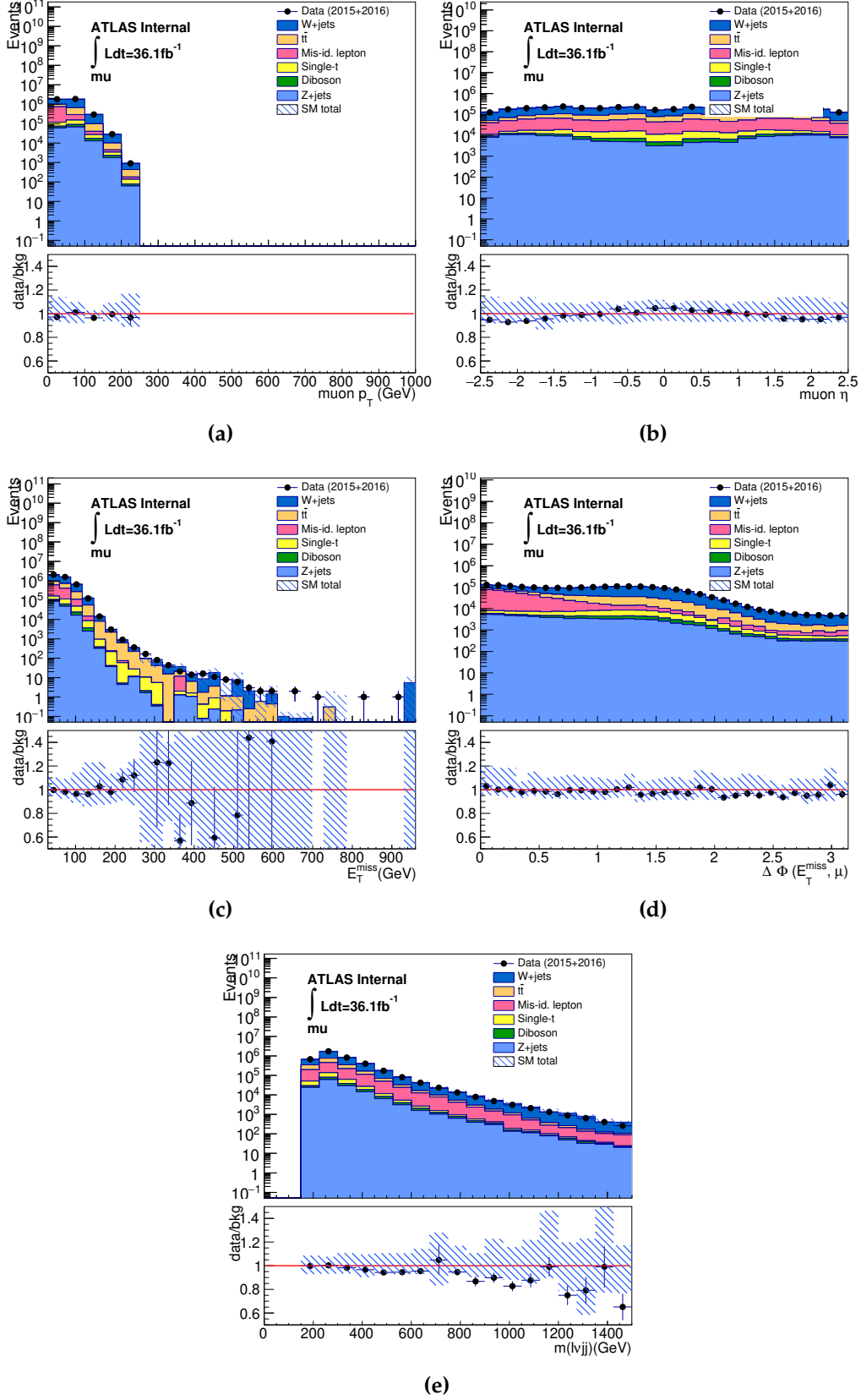
Figure 3.23.: The distribution of lepton p_T , \eta , E_T^{miss} , \Delta\phi(\ell, E_T^{miss}) , and m_{WV} in validation region with p_T(l\nu) < 150\text{GeV} in muon channel with multijet background
