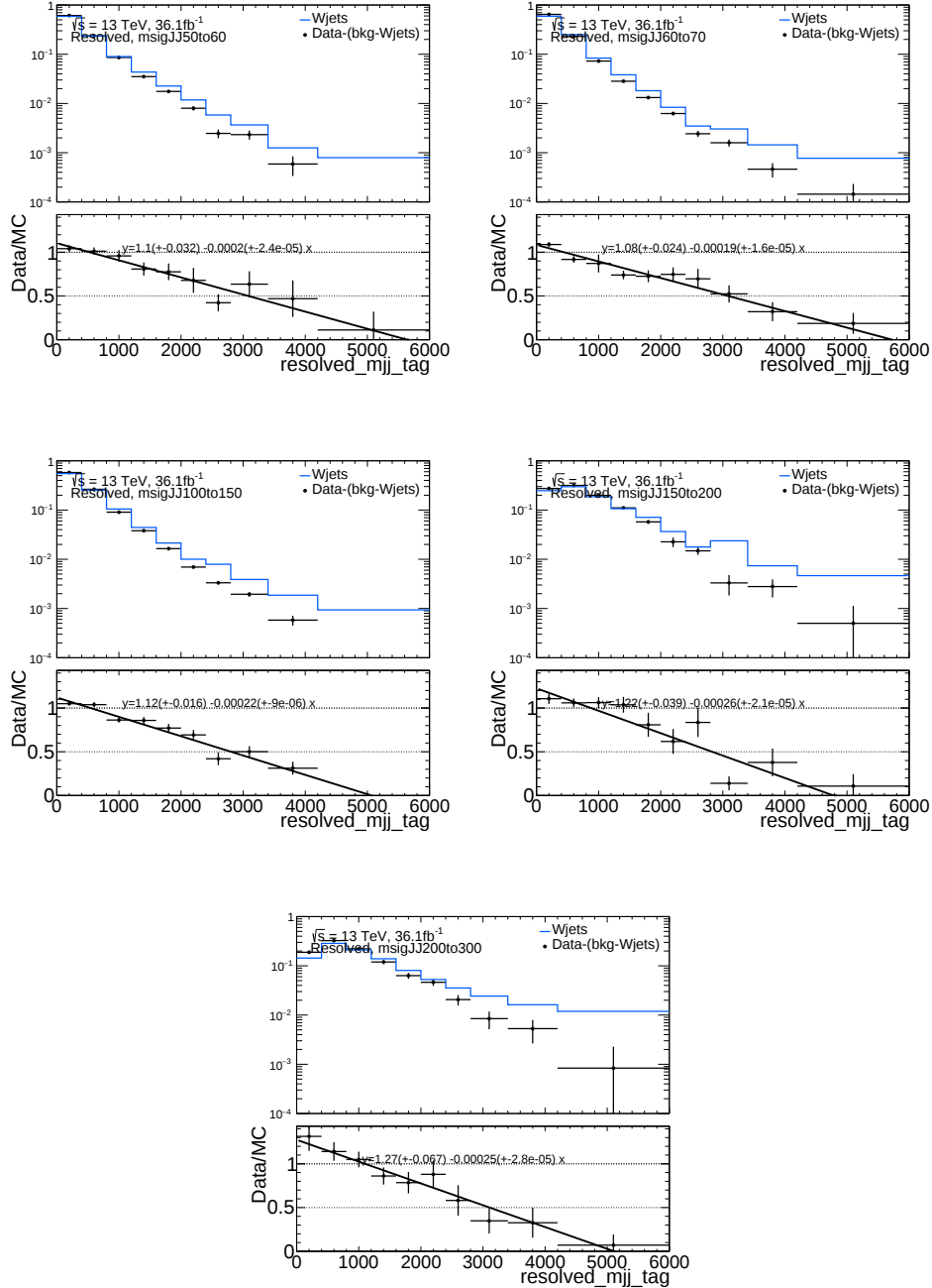
Figure 5.8.: Fit of m^{VBS} (as \text{resolved\_m\_jj} in the plots) slope in W+jets resolved CRs, in different slices of m_{jj}^V .
