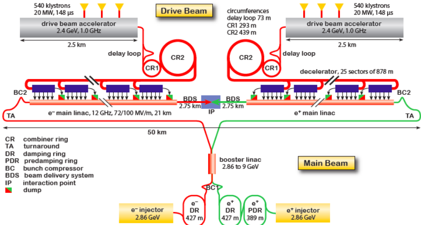
Figure 1.1: CLIC layout at \sqrt{s} = 3 TeV.
