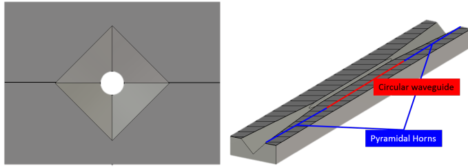
Figure 3.1: DUT: circular waveguide and two pyramidal horns. Left: Front view. Right: Perspective view of longitudinal cut.
