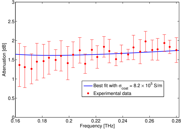
Figure 3.28: Attenuation on the NEG coated slab of 3.68 \mu\text{m} : averaged experimental data (red dots) and best fit curve (blue). The value of reduced \chi^2 = 0.36 .
