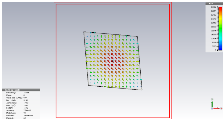
Figure 3.37: Second mode in propagation for diagonal waveguides 62 mm long with an error of 5° on the angle of the aperture.
