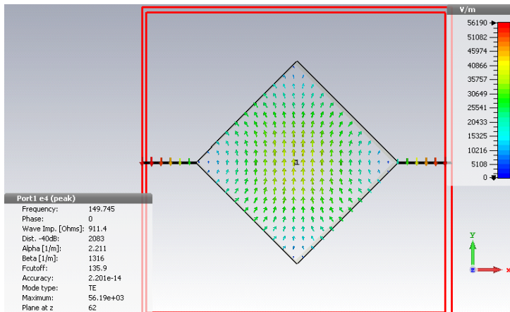
Figure 3.34: Mode passing through the diagonal waveguide 62 mm long with a gap of 10\text{ }\mu\text{m} between the two shells.
