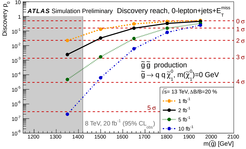
Figure 3.12: Discovery p_0 values as a function of the gluino mass in the gluino-pair production models at a given integrated luminosity of 1, 2, 5, or 10 fb -1 (from inner to outer lines) with a hypothesis of 20% uncertainties on the total background prediction. For each integrated luminosity scenario, one baseline signal region is optimised for one target signal point with a hypothesis of 20% uncertainties on the total background prediction.
