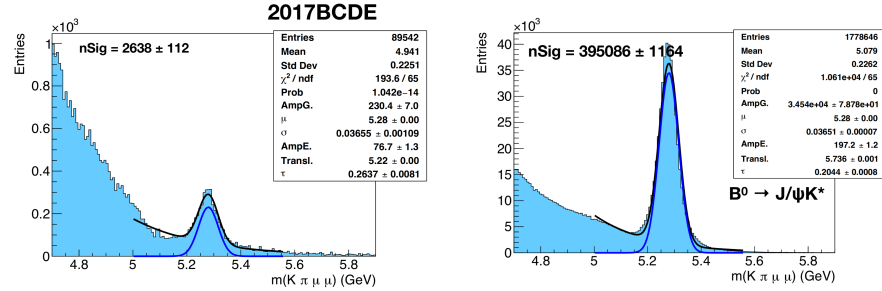
Figure 9.2: Distribution of the candidate- B^0 invariant mass of a partial 2017 dataset, corresponding to 28\text{ fb}^{-1} , for the signal (left) and J/\psi\ q^2 regions. The selection criteria applied to the dataset are described in Section 9.1.1. The rough fits are performed with a pdf obtained from the sum of a Gaussian and an exponential function.
