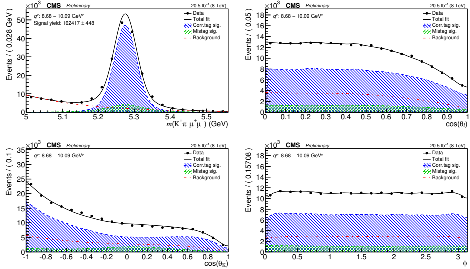
Figure 6.26: The fitting results of the control channel J/\psi on data. The plots show the projections of the fitting results on three different angular variables: B^0 mass, \cos \theta_l , \cos \theta_K and \phi .
