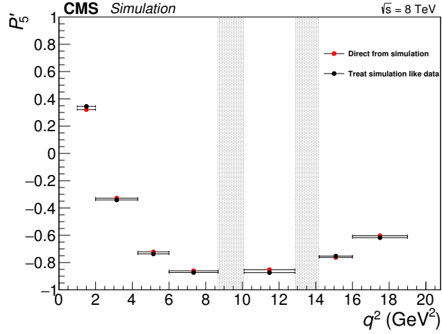
Figure 6.12: Results for the P'_5 parameter from the reconstruction-level fit (black) and from the generator-level fit (red), for each q^2 bin. The vertical shaded regions correspond to the q^2 bins dedicated to the J/\psi and \psi' control channels.
