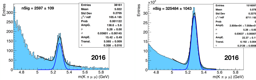
Figure 9.1: Distribution of the candidate- B^0 invariant mass of the 2016 dataset, for the signal (left) and J/\psi (right) q^2 regions. The selection criteria applied to the dataset are described in Section 9.1.1. The rough fits are performed with a pdf obtained from the sum of a Gaussian and an exponential function.
