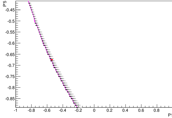
Figure 1.7: Physical boundaries of the negative P_5' sector of q^2 bin 5. Accordingly to the description in Sec. 1.2.3, the magenta line is the boundary of the P-wave physical region and the set of grey-scale lines are the boundaries of the total-PDF physical region, for different A_s^5 values (black for f = -1 , lightest grey for f = 1 ).
