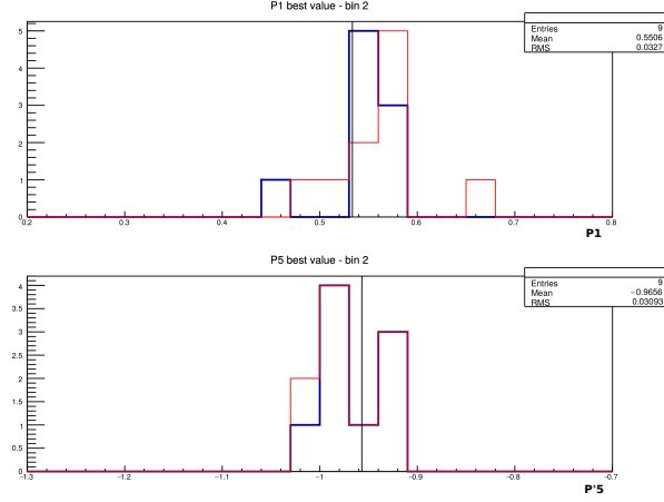
Figure 7.4: Distributions of the best-fit values of the fits performed, in q^2 bin 2, on the high-statistics pseudo-experiments used to compute the systematic uncertainty for the fixed parameters, as described in Section 7.8. The blue (red) histogram is the distribution of the results of the fit with fixed (floating) F_L, F_s, A_s parameters. The black line marks the input value used to generate the pseudo-experiments. Top: results for P_1 . Bottom: results for P_5' .
