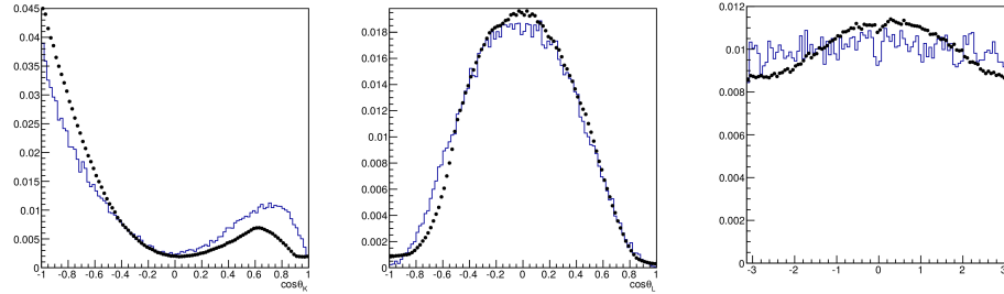
Figure 5.5: Comparison of the reconstructed and selected MC event distributions (histogram) with generated event distributions (dots) weighted with the efficiency, parameterised as in Equation 5.3 with parabolic interpolation of the two-dimension efficiency functions. Both the distributions and the efficiency refer to right-tagged events in q^2 bin 1.
