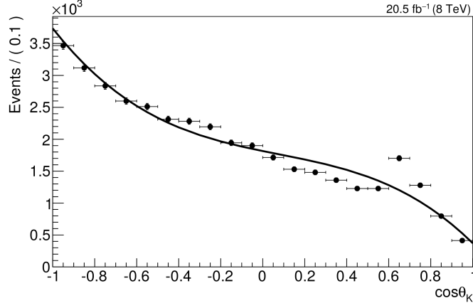
Figure 6.21: Distribution of the \cos\theta_K variable in mass sidebands of the B^0 \rightarrow J/\psi K^{*0} control channel and the background pdf projection.
