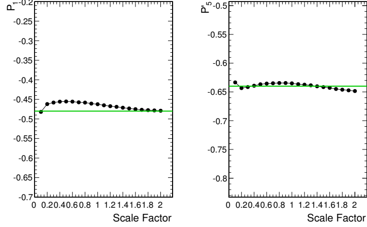
Figure 7.11: Comparison between the position of the absolute maximum of the likelihood (green line) and the results of the bi-variate Gaussian fit, as a function of the fit range (black dots), for the P_1 (left) and P'_5 (right) parameters, in q^2 bin 3.
