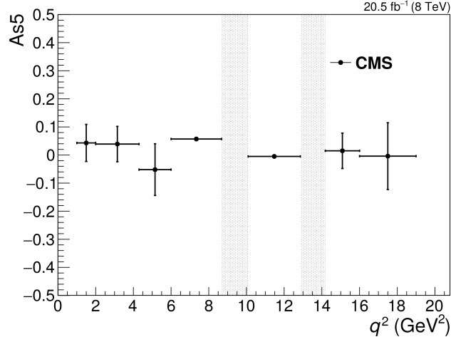
Figure 8.11: Fit results of the A_S^5 angular parameter versus q^2 . Only the statistical uncertainties are shown. The vertical shaded regions correspond to the J/\psi and \psi' resonances.
