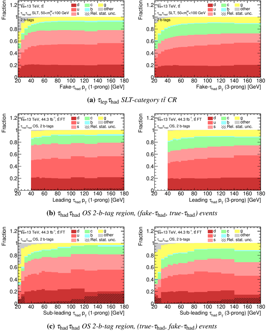
Figure B.1. Composition of the fake- \tau_{\text{had}} origin between the t\bar{t} FR CR ( \tau_{\text{lep}} \tau_{\text{had}} SLT OS 2-b-tag region with 50 \text{ GeV} < m_T^W < 100 \text{ GeV} ) (top) and the \tau_{\text{had}} \tau_{\text{had}} OS 2-b-tag region for the events where the leading \tau_{\text{had}} candidate is fake (middle) and for the events where the sub-leading \tau_{\text{had}} candidate is fake (bottom), shown separately for 1-prong (3-prong) on the left-hand (right-hand) side.
