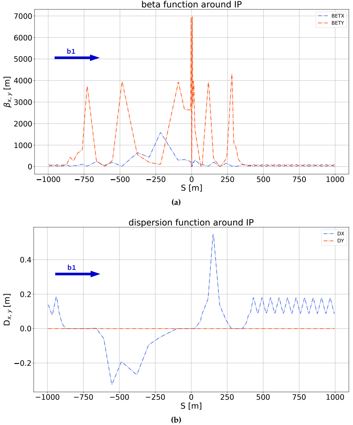
Figure 3.5: FCC-ee interaction region optics at \sqrt{s} = 100 GeV, within \pm 1 km around the interaction point ( S = 0 m). The beam direction is indicated by a blue arrow. This example demonstrates the asymmetry in the optics upstream and downstream of the interaction point. (a) horizontal and vertical beta function. The change of rather regular oscillations into an irregular pattern is a result of the asymmetry, required to reduce the critical energies of upstream dipole magnets. (b) dispersion function, showing how the horizontal dispersion is reduced to 0 at the experiment ( S = 0 m).
