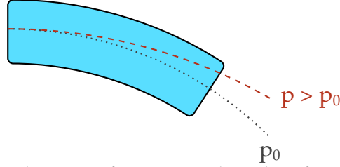
Figure 2.7: Trajectory through a dipole magnet for two particles. The reference particle ( p_0 ) would follow the design orbit, while a particle with positive momentum offset ( p > p_0 ) is less deflected in the bend, following a longer orbit.
