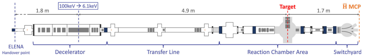
Figure 7.1: Scheme of the GBAR \bar{p}/\bar{\text{H}} beam line as of 2022, adapted from Reference [44]
