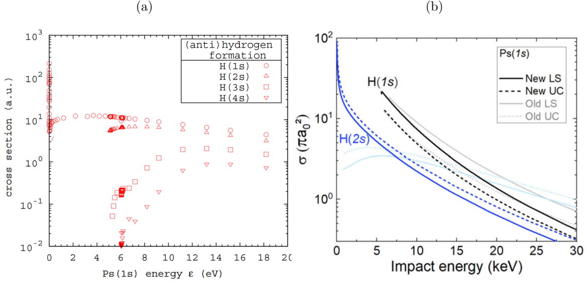
Figure 2.2: Theoretical cross-sections of (a) \bar{\text{H}} atom formation in low-lying excited state via the first reaction shown in Equation (2.1), adapted from Reference [45], and (b) \bar{\text{H}}^+ ion formation via the second reaction shown in Equation (2.2) assuming \bar{\text{H}}(1\text{s}) and \bar{\text{H}}(2\text{s}) incident on Ps(1S), adapted from Reference [49]
