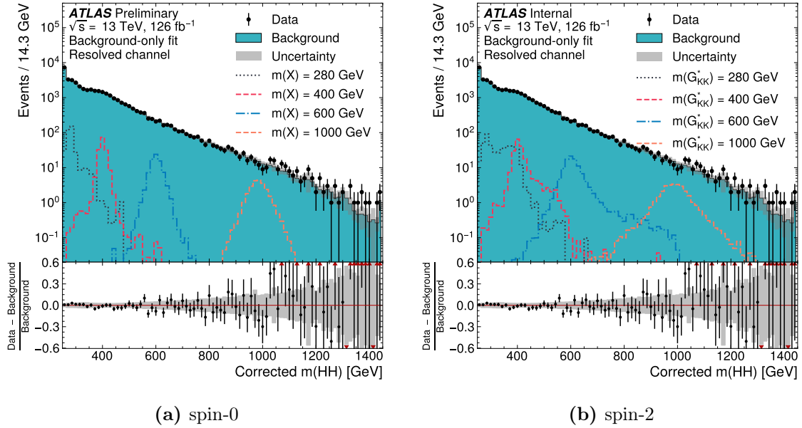
Figure 10.1.: Resonant search m_{HH}^{cor} signal region distributions. The background estimate is compared to the observed data after a background-only profile likelihood fit, which are in agreement with each other except for the high mass tail region. a) Shows the data along with the benchmark spin-0 signal samples for a few resonance masses. b) Shows the same resonance mass points but of the spin-2 benchmark signal instead.
