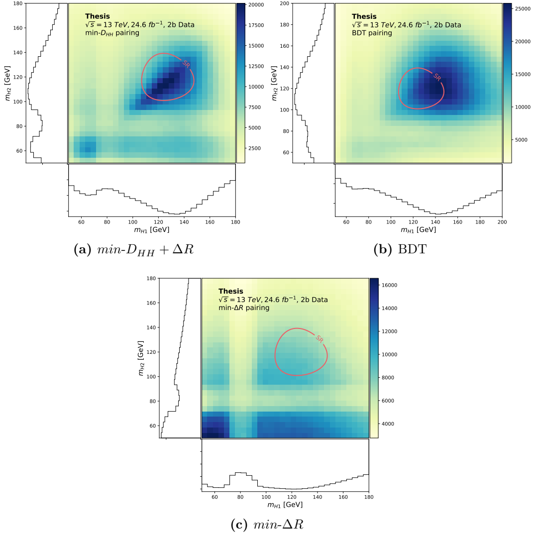
Figure 7.5.: m_{H1} - m_{H2} massplane of the 2b category with the three different pairing methods. The ring indicates the boundary of the signal region. The deficiencies seen as a stripes that are centered at about m_{H1} = m_{H2} = 80 GeV are due to the top veto. These massplanes were formed by using only data available from 2016, which is 24.6 \text{ fb}^{-1} of integrated luminosity. The \min-D_{HH} + \Delta R pairing method results in a significant amount of sculpting that peaks in the centre of the signal region. The BDT pairing method lessens the amount of sculpting while the \min-\Delta R pairing method completely eradicates it.
