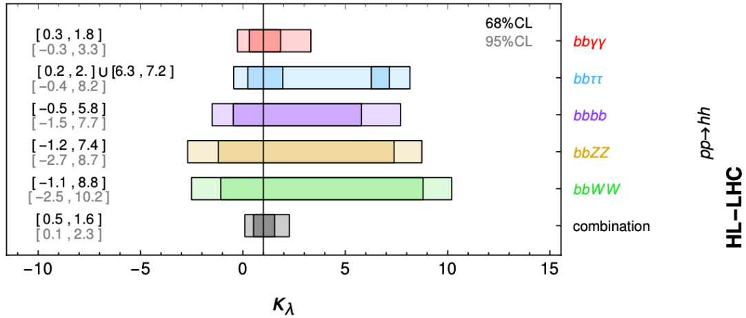
Figure 2.13.: Combined ATLAS and CMS High Luminosity LHC (HL-LHC) projections on the Higgs self-coupling \kappa_\lambda assuming a luminosity of 3000 \text{ fb}^{-1} at \sqrt{s} = 14 TeV. The projections are made using the early Run-2 searches as a baseline. The projections indicate that the \kappa_\lambda can be constrained to values between \kappa_\lambda \in [0.1, 2.3] at 95% CL. Constraining the \kappa_\lambda parameter down to these values can help exclude a number of BSM models. Figure edited from [33].
