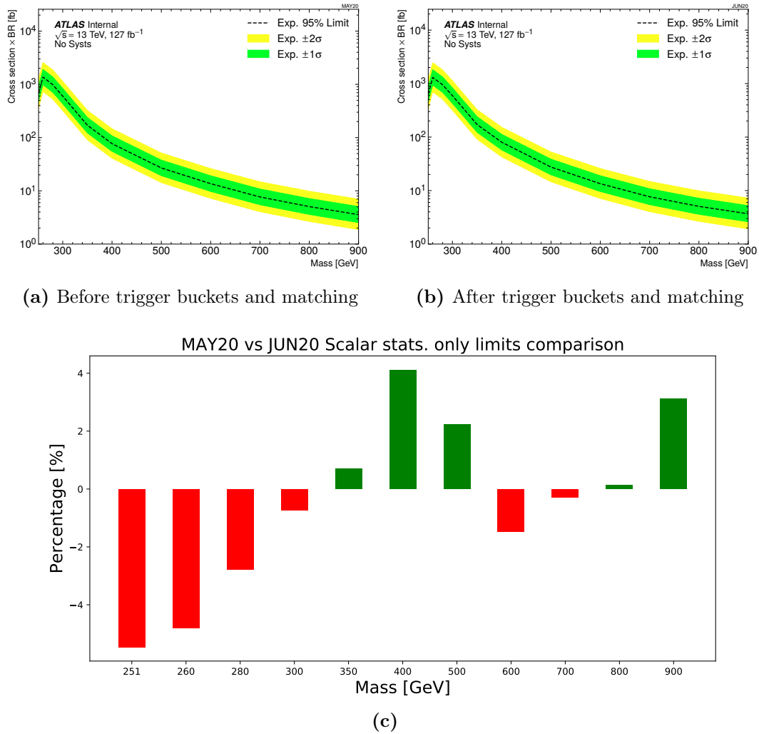
Figure 9.6.: Expected confidence level limits on cross-section of pp \rightarrow X \rightarrow b\bar{b}b\bar{b} with only statistical uncertainties included. These limits ignore the application of scale factors to correct the signal prediction. a) Shows the expected limits before trigger bucketing and matching. b) Shows the expected limits after both trigger bucketing and matching have been applied. This also excludes data taken in 2015. The offline selections of the trigger buckets used in the resonant search are shown in Table 9.6. c) Shows the percentage difference between the limits shown in a) and b).
