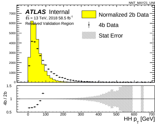
(c) Before Reweighting
