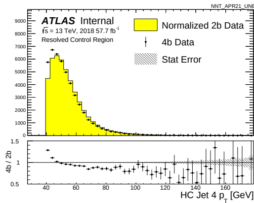
(a) Before Reweighting
