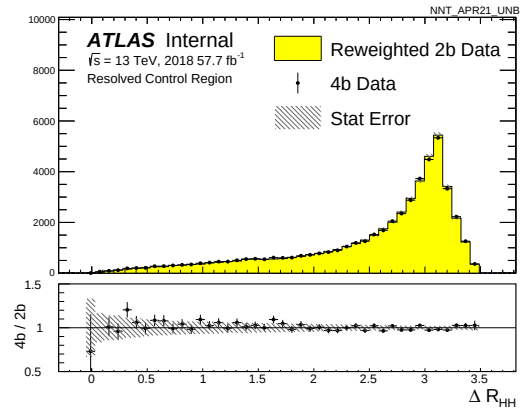
(b) After Reweighting
