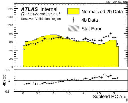
(c) Before Reweighting
