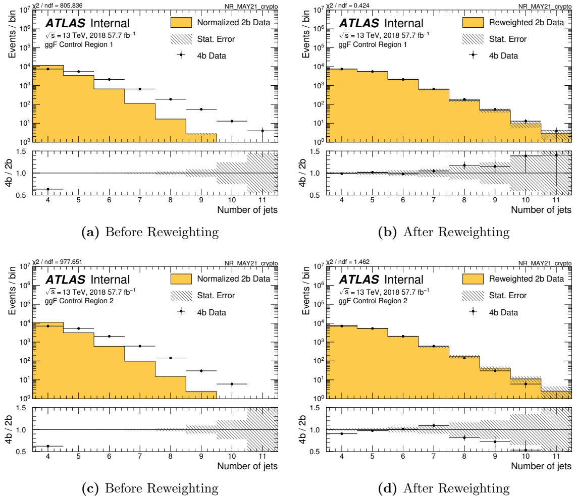
Figure 8.15.: Non-resonant njets distributions before and after reweighting, in both CR1 and CR2 kinematic regions.
