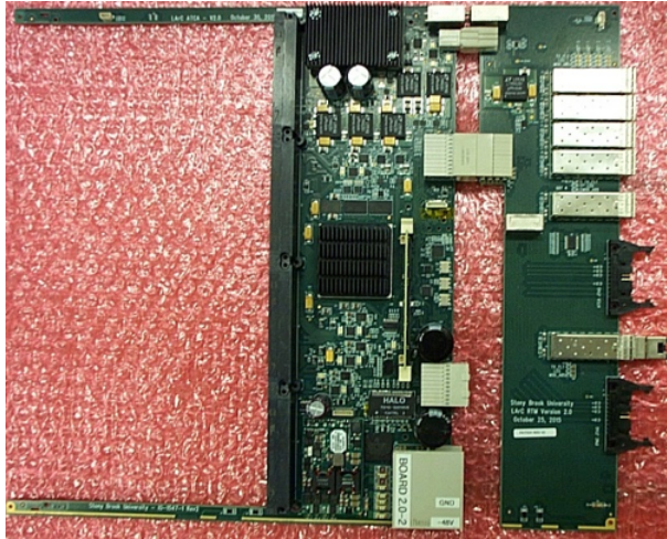
Figure 4.13: Carrier board.
