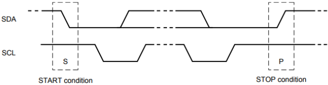
Figure 5.32: I2C start and stop conditions [111].
