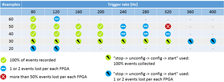
Figure 5.50: Percentage of events successfully recorded for various number of samples and different trigger rates.
