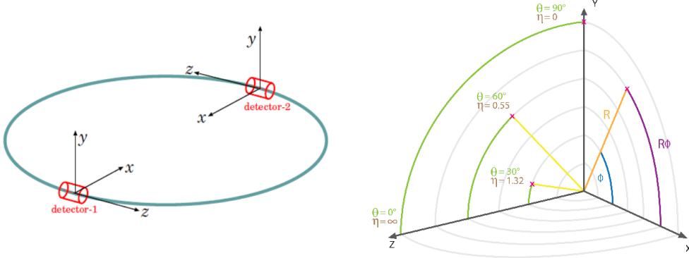
Figure 2.2: Common coordinate system used in the LHC experiments.
