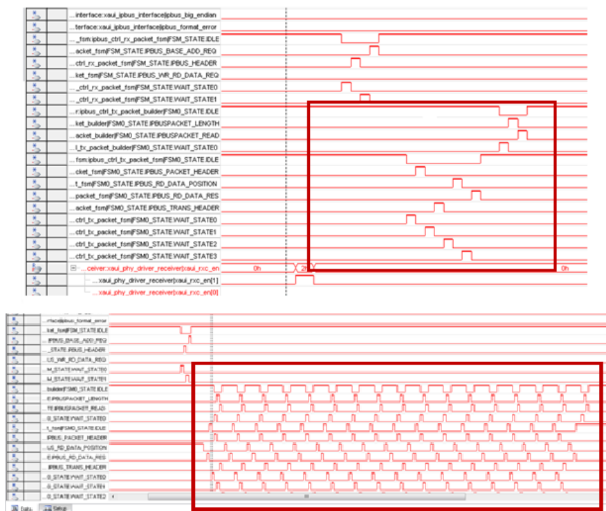
Figure 5.49: Good behaviour (top) and bad behaviour (bottom) of the state machine handling the IPbus requests.
