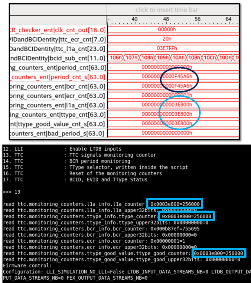
Figure 6.31: Calibration run taken with TDAQ partition: 256000 events at 6.5 kHz delivered. SignalTap tool (top) and firmware registers (bottom) pictures show the correct behaviour of the TTC firmware block: the number of BCRs received and BCR with good periodicity are matching (dark blue) as well as the number of L1A, TType and TType with expected value (light blue).
