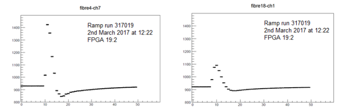
Figure 5.47: Pulse from a ramp run (317019) collected after applying the latency correction. Two channels connected to FPGA 19:2 are shown.
