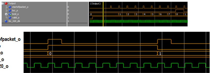
Figure 6.18: IStage simulation details: the top picture shows the simulation of the protocol towards the IStage block. The second picture is a zoom around the BCR event.
