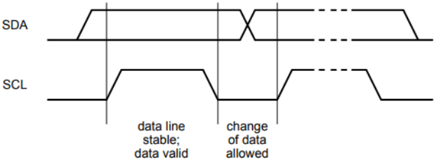
Figure 5.31: Bit transfer on the I2C bus [111].
