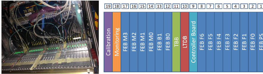
Figure 5.9: Left: LAr front-end crate, sitting on the detector, where the two LTDBs are placed. Right: slot assignments for the new EMB baseplane, used in the demonstrator crate.
