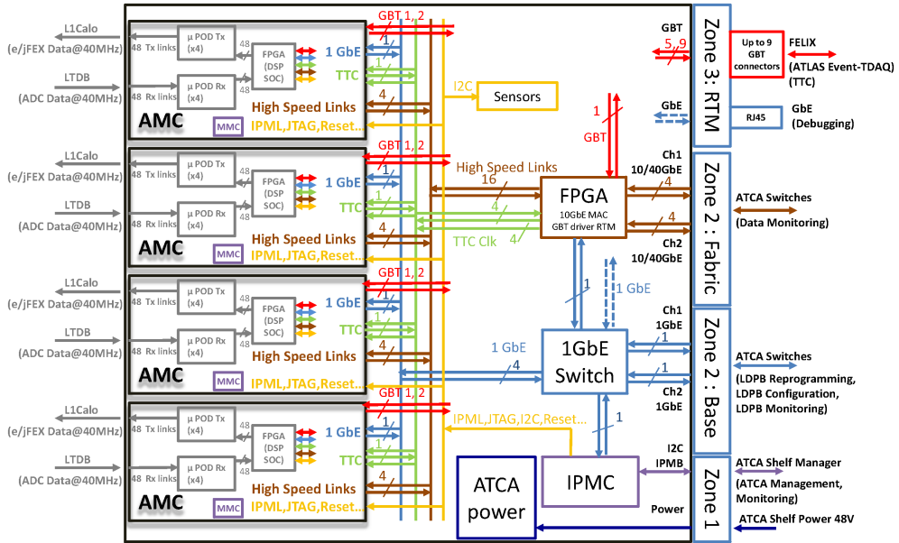
Figure 4.12: Schematic view of a Carrier board [85].
