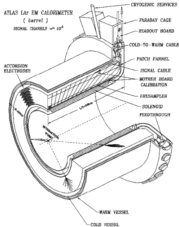
Figure 3.4: Barrel cryostat [35].
