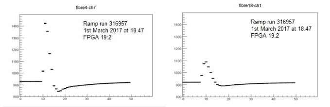
Figure 5.46: Pulse from a ramp run (316957) collected after applying the latency correction. Two channels connected to FPGA 19:2 are shown.
