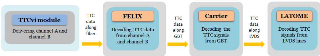
Figure 6.9: TTC chain in EMF.
