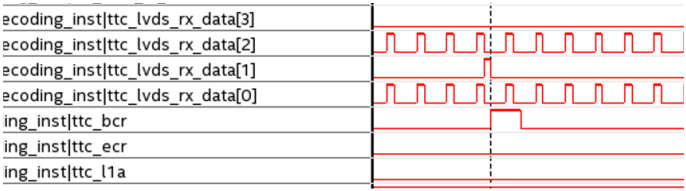
Figure 6.22: BCR detection and decoding in the TTC top level. The four LVDS lines (lvds_rx_data) with the synchronization pattern on the LVDS line 0, the channel B idle on the LVDS line 2 and the BCR on the LVDS line 1 are visible.
