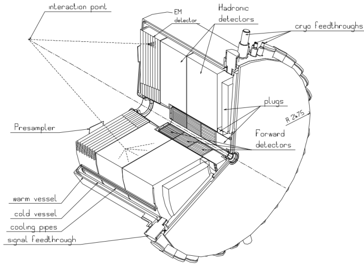
Figure 3.6: End-cap cryostat [35].
