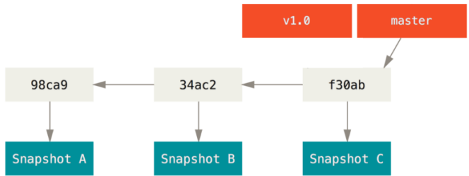
Figure B.3: Example of branches development and commits (snapshots) in git: in this figure a new branch is created from the master [124].
