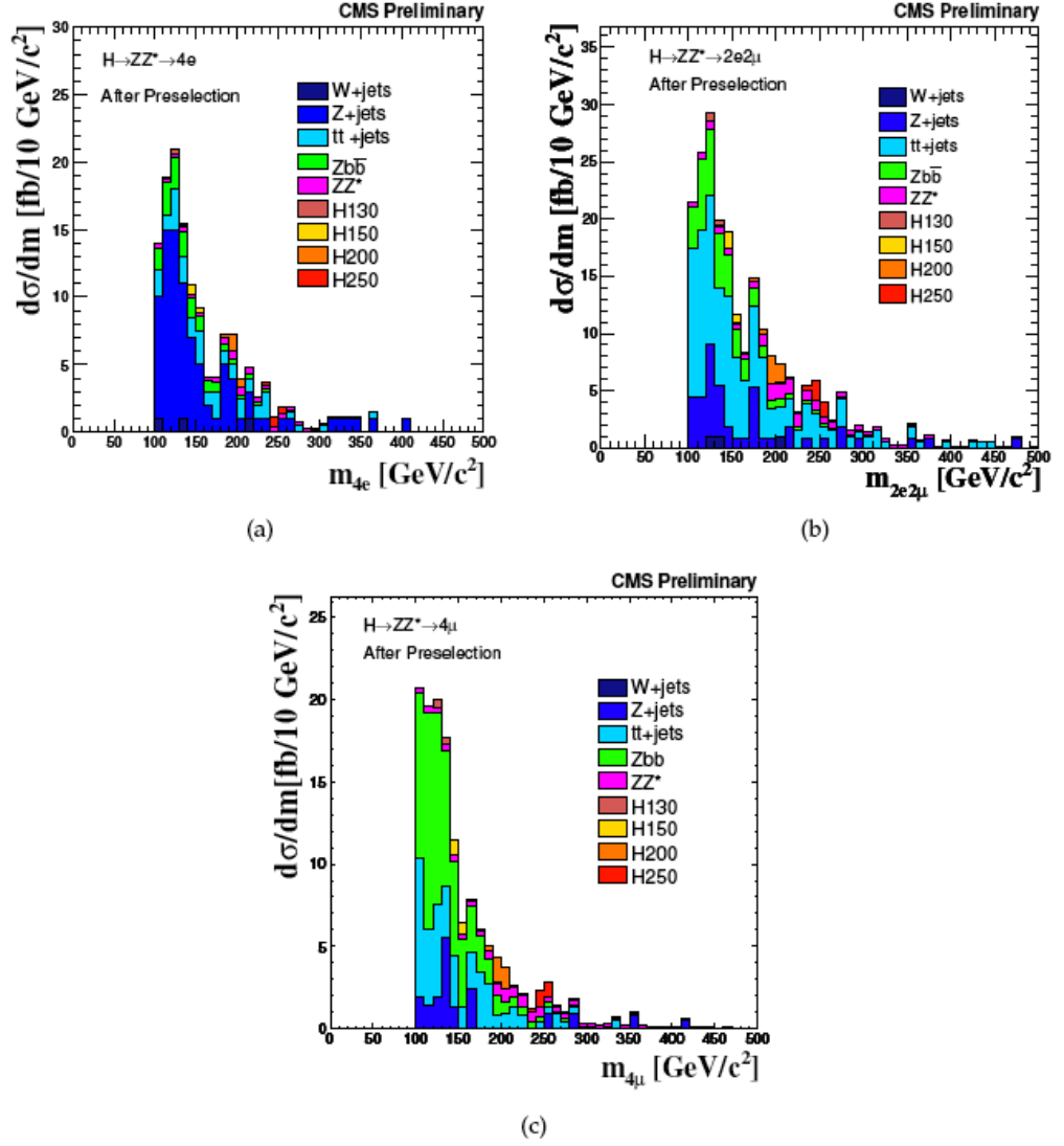
Figure 3.8: Four-lepton invariant mass after pre-selection[55] with cumulative backgrounds and H \rightarrow ZZ^* \rightarrow 4\ell signal events together for different m_H hypothesis in the (a) 4e^- , (b) 2e^- 2\mu^- and (c) 4\mu^- channel.
