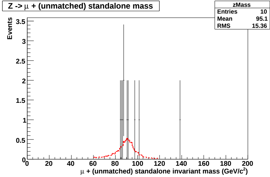
(b) 10 pb -1
