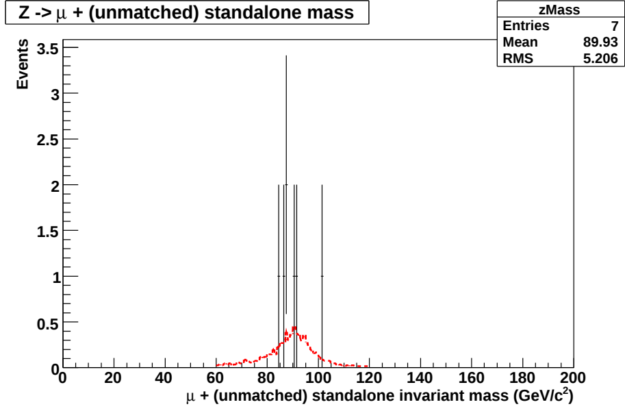
(a) 5 pb -1
