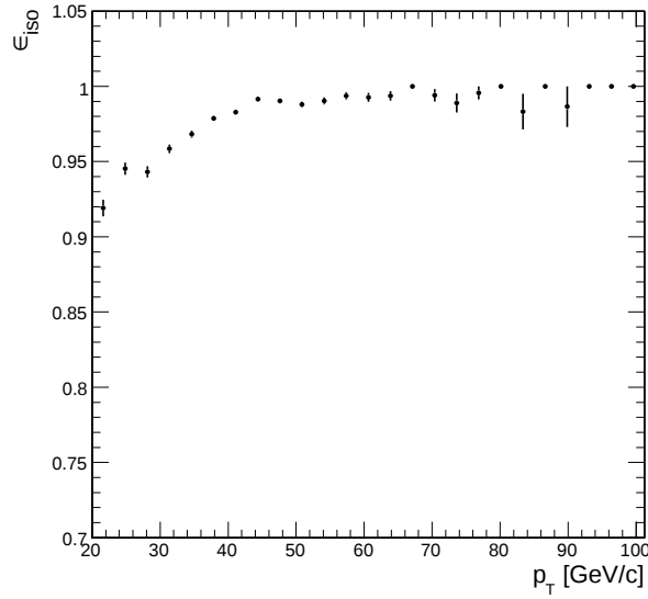
Figure 4.27: Isolation efficiency, for relative isolation selection, with respect to muon p_T .
