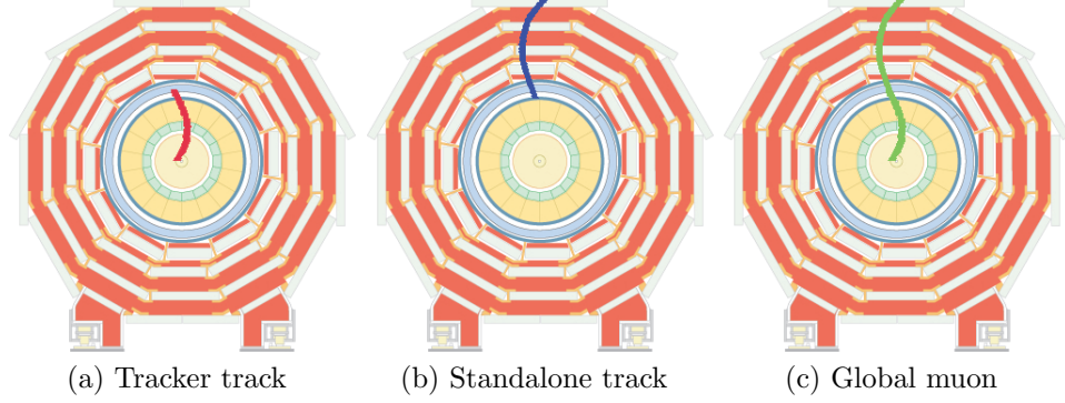
Figure 4.4: Muon candidates reconstruction classification: (a) tracker track, p_T , (b) standalone track and (c) global muon.
