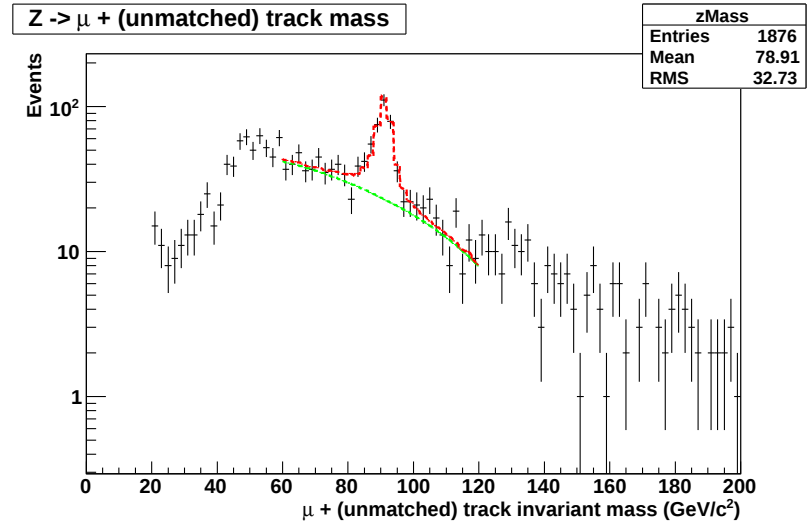
Figure 4.11: Fit curve superimposed to the invariant mass histogram of Z_{\mu t} candidates for a sample corresponding to an integrated luminosity of 45\text{ pb}^{-1} .
