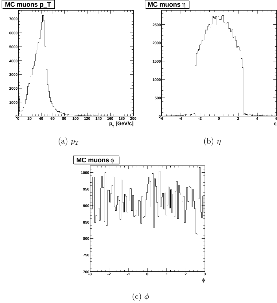
Figure 4.3: Distribution of kinematic quantities of Monte Carlo muons coming from Z decay: (a) transvers momentum, p_T , (b) pseudorapidity \eta and (c) azimuthal angle \phi .
