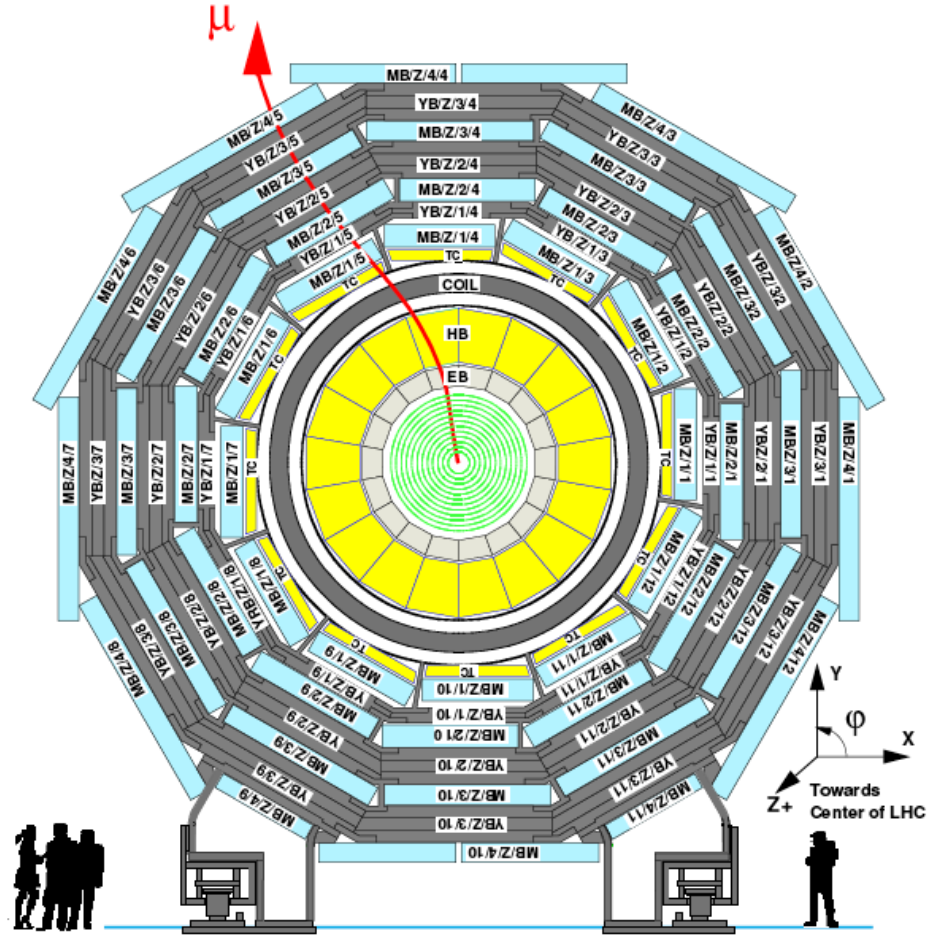
Figure 2.16: Layout of the CMS barrel muon DT chambers in one of the 5 wheels. Each wheel is divided into 12 sectors, each covering a 30^\circ azimuthal angle, and composed of 4 stations.
