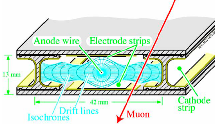
Figure 2.15: Schematic view of a drift cell. The electrons, coming from the gas ionization due to the passage of a muon, drift towards the wire anode. The voltages applied to the electrodes are +3600\text{V} for wires, +1800\text{V} for strips, and -1200\text{V} for cathodes.
