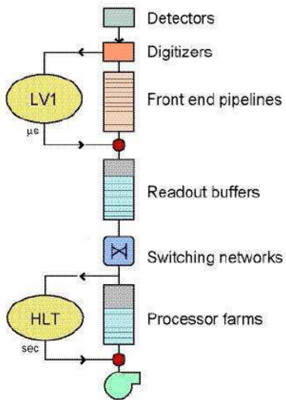
Figure 2.19: Data Flow in the Trigger/DAQ system.
