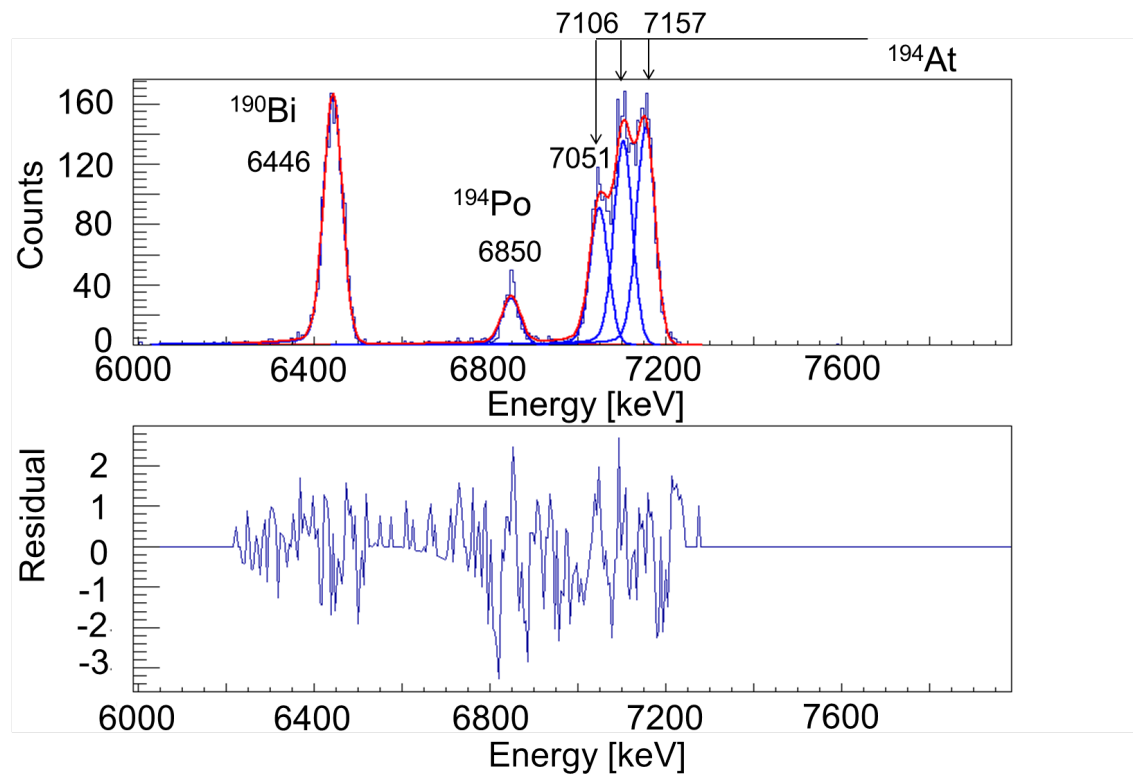
Figure 8.2: Fit of the ^{194}\text{At} \alpha -decay spectrum with the energies of the peaks marked.
