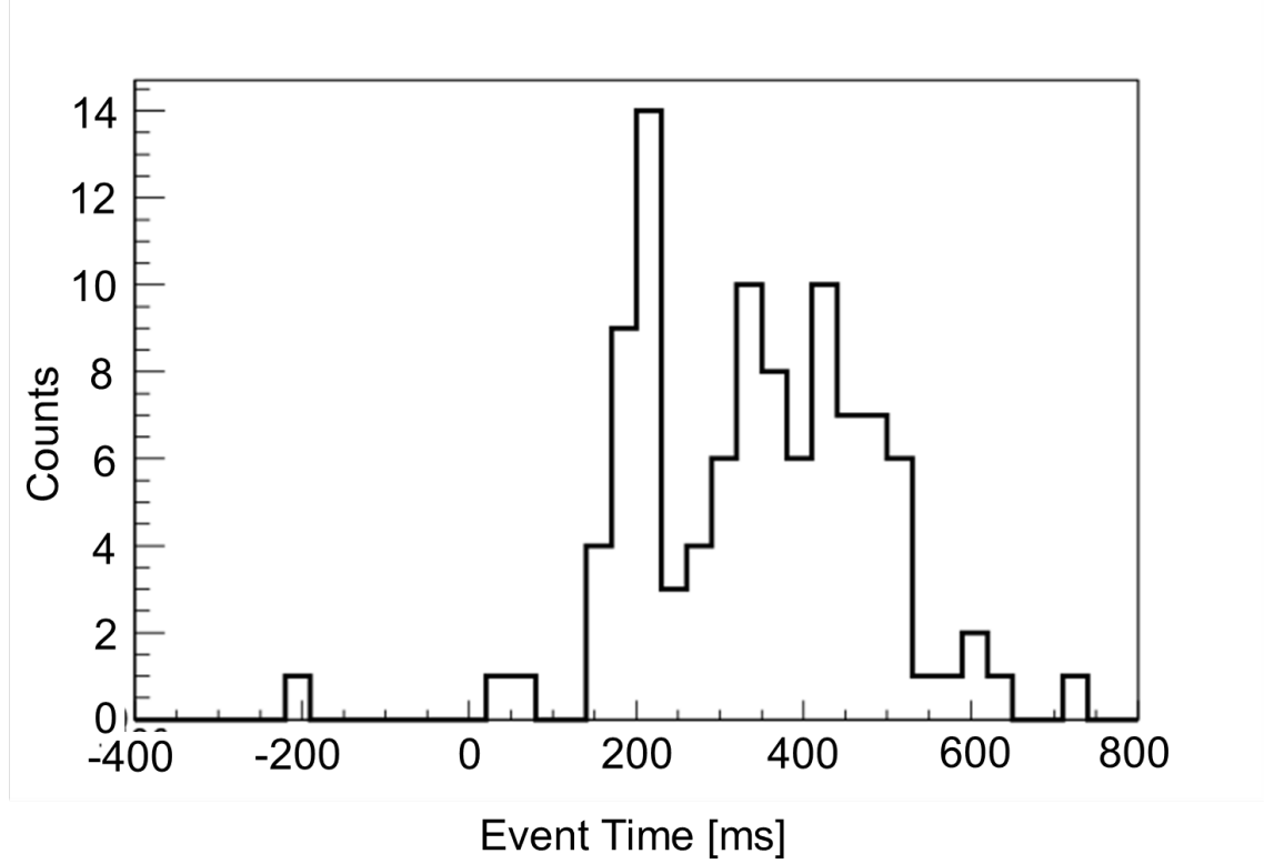
Figure 6.5: X ray timing structure of the lower energy area in coincidence with the fine structure peaks. It can be seen that the structure is not as well defined.
