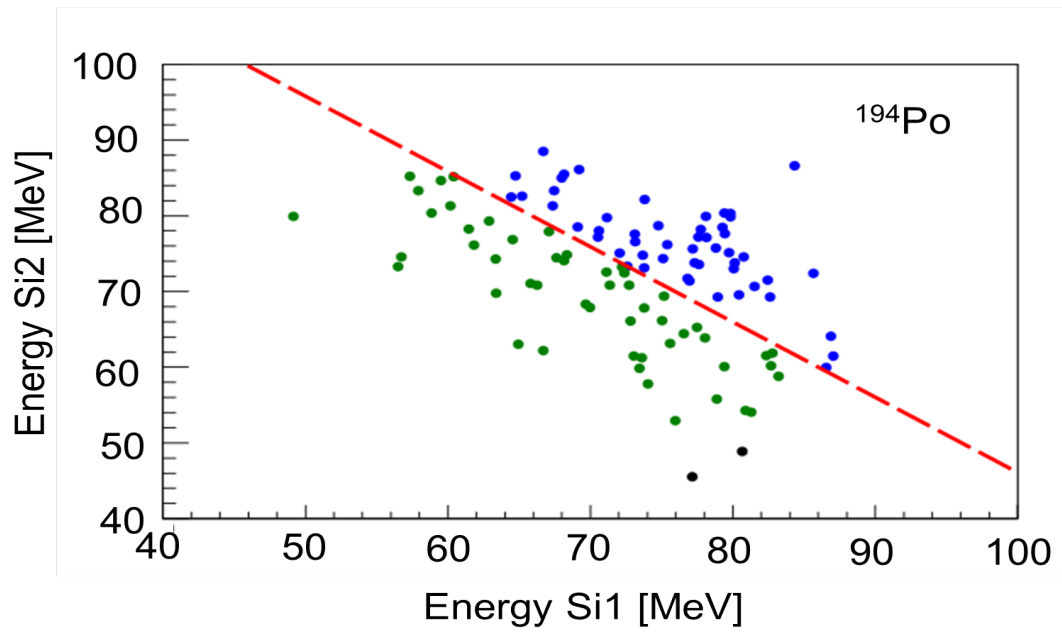
Figure 9.2: 2D coincidence plot for ^{194}\text{Po} which when compared to ^{180}\text{Hg} and ^{196}\text{Po} , is much more similar to the latter.
