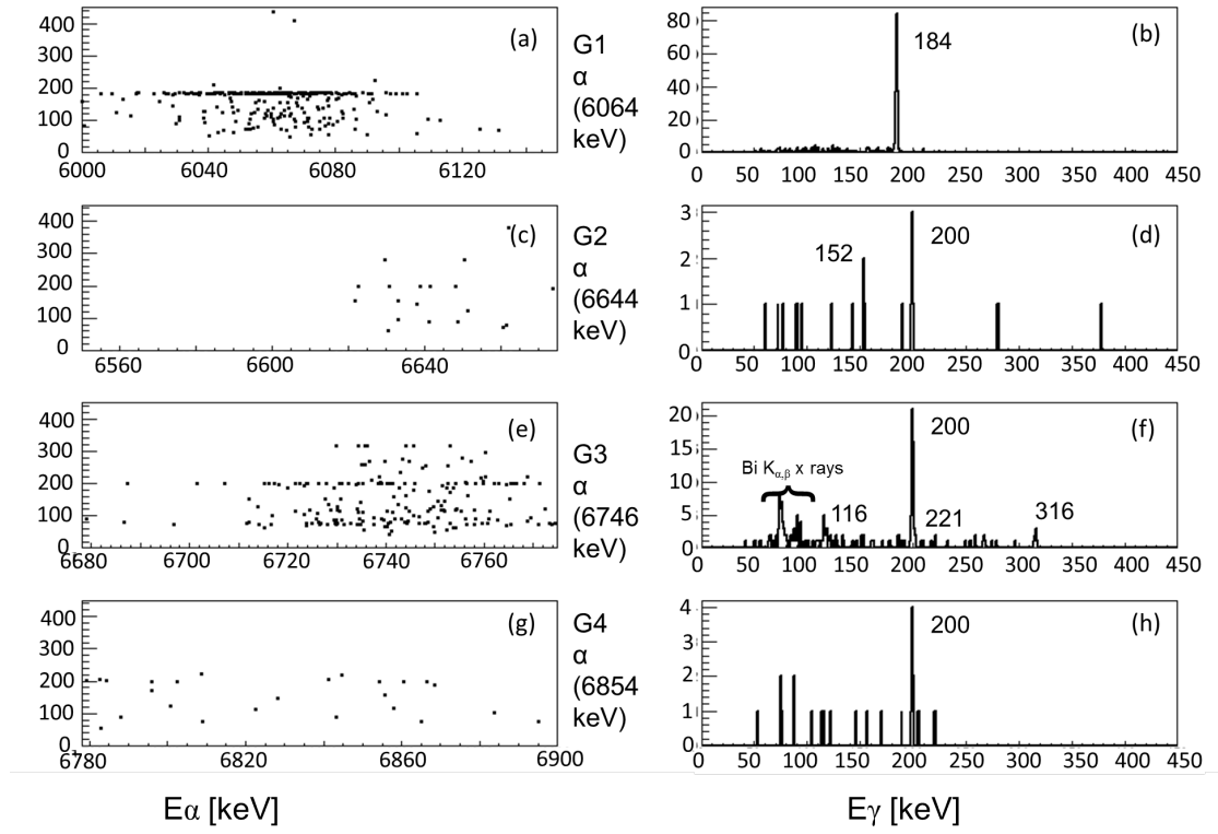
Figure 6.6: Comparison of the \alpha - \gamma coincidences and \gamma projection of ^{192}\text{Bi} and the three \alpha decay fine structure peaks.
