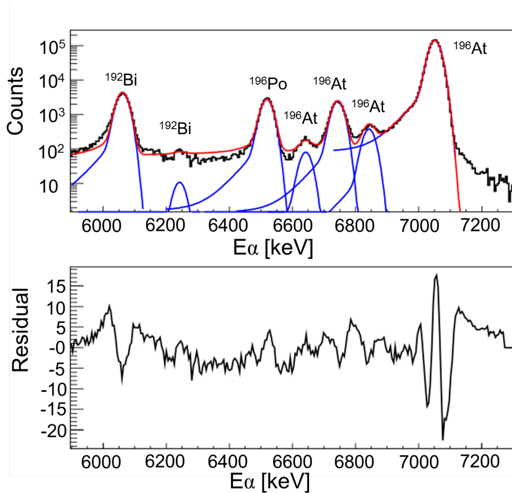
Figure 4.1: \alpha -decay energy spectrum for ^{196}\text{At} taken at HRS showing the tails fitting procedure that was used. This spectrum uses all 13 run files from the first set of data files. A similar plot is shown in Fig. 6.1 (b), but for only the first 6 run files as will be explained.
