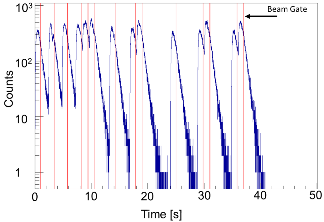
Figure 6.9: Timing structure used for determining ^{196}\text{At} half-life. This plot is an accumulation of all SCs within a file, providing they have the same SC pattern. The red line marks where the beam gate closes. At this point it is known that no more implantation can be occurring and it is only decay. This gives a starting point for the exponential fit of the decay.
