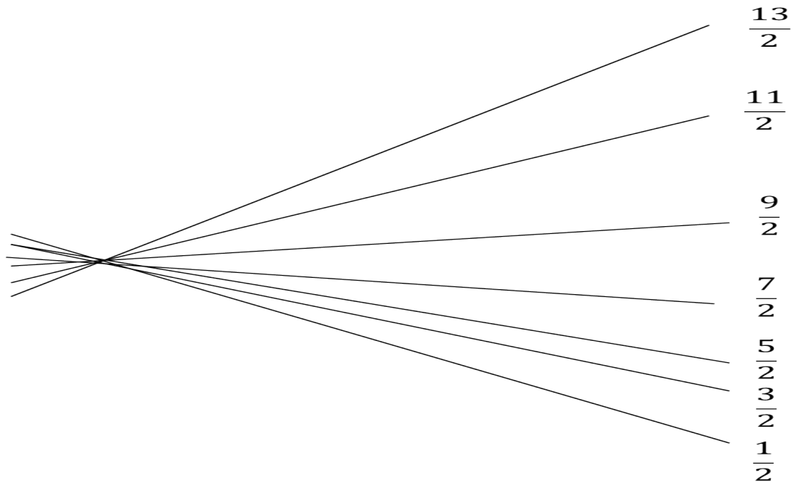
Figure 2.7: Diagram of second simplification of Nilsson model [62].
