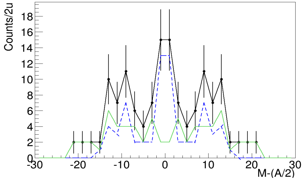
Figure F.2: 2n fission fragment mass distribution. The high TKE is a symmetric mass distribution while the low TKE is an asymmetric mass distribution.
