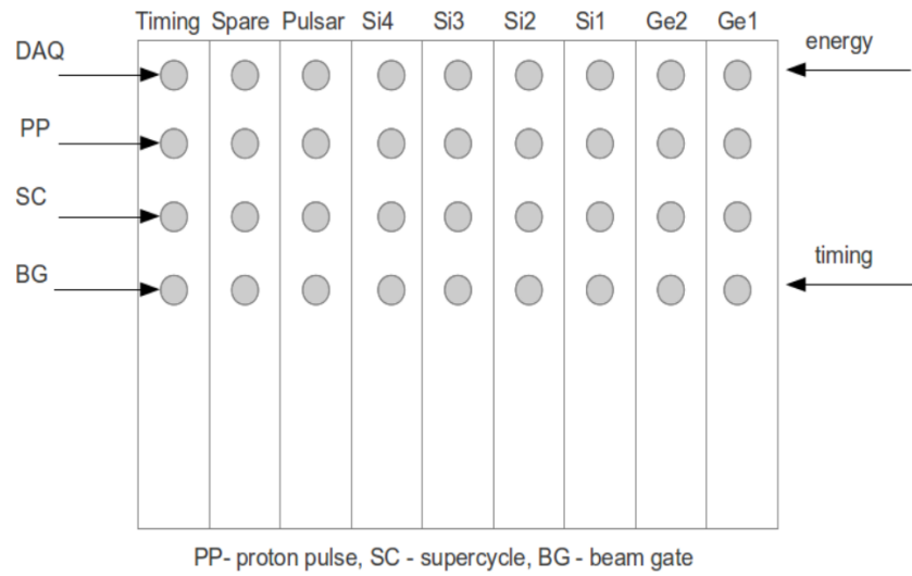
(b) DGF set-up for the 2012 run
