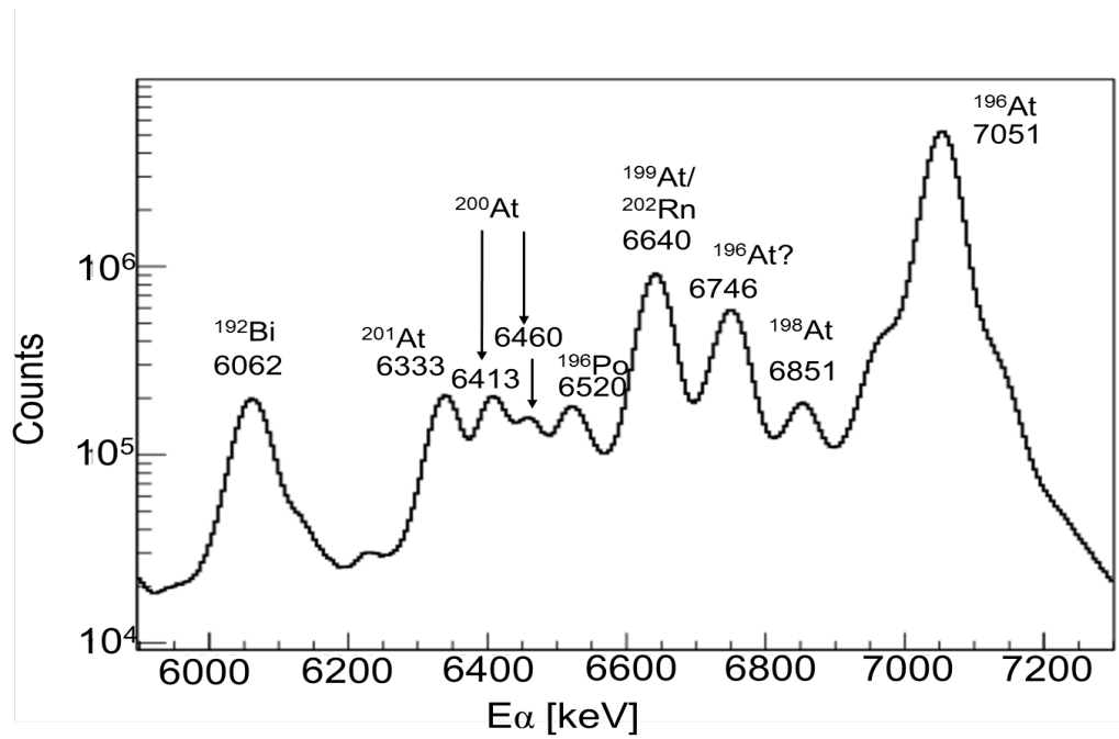
Figure A.2: \alpha -decay energy spectrum from GPS. It can be seen that there is contamination from other astatine masses.
