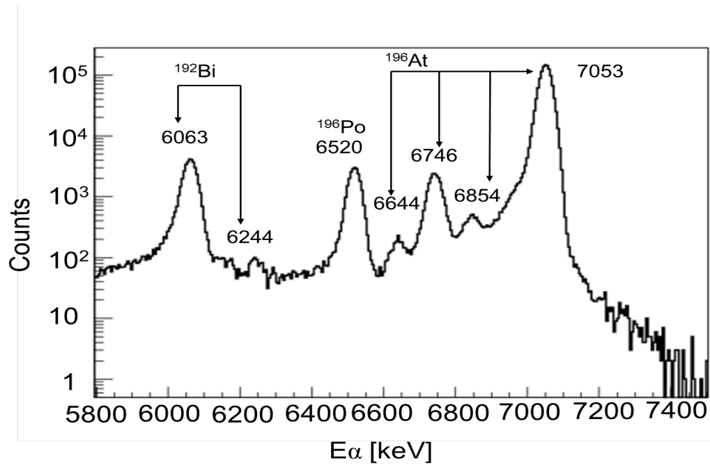
Figure A.1: Alpha decay energy spectrum of ^{196}\text{At} . Marked on the plot are the energies and identities of each of the peaks.
