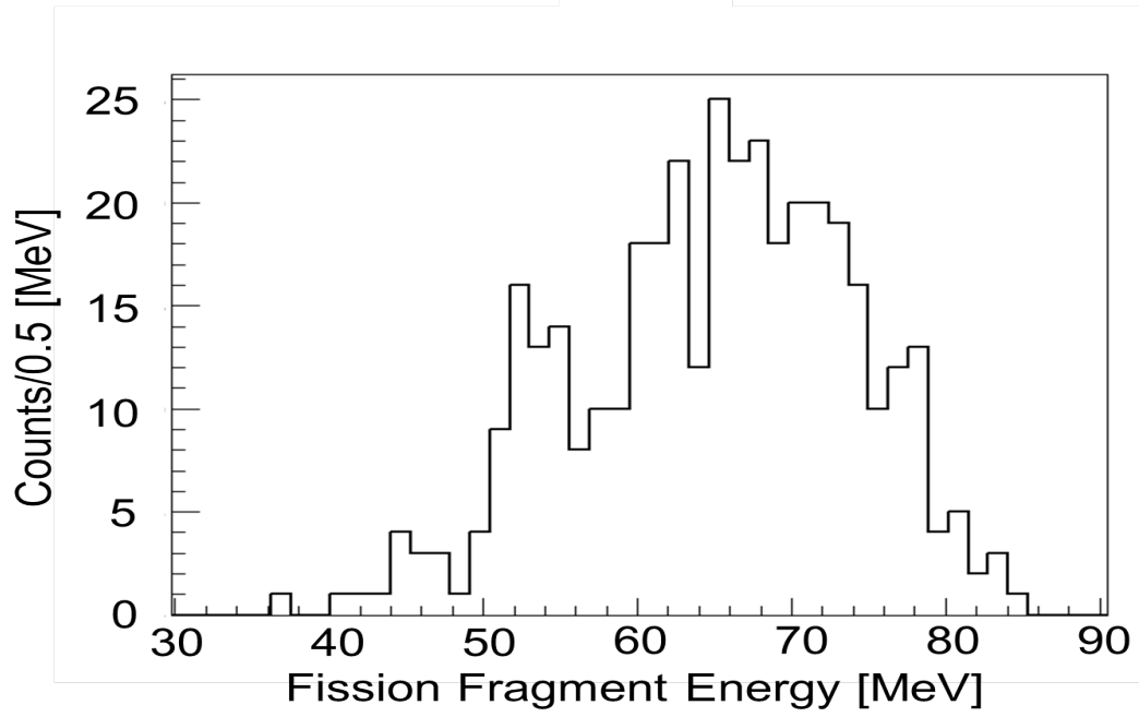
Figure 9.1: ^{194}\text{At} fission events energy spectrum showing the combined events from Si1 and Si2.
