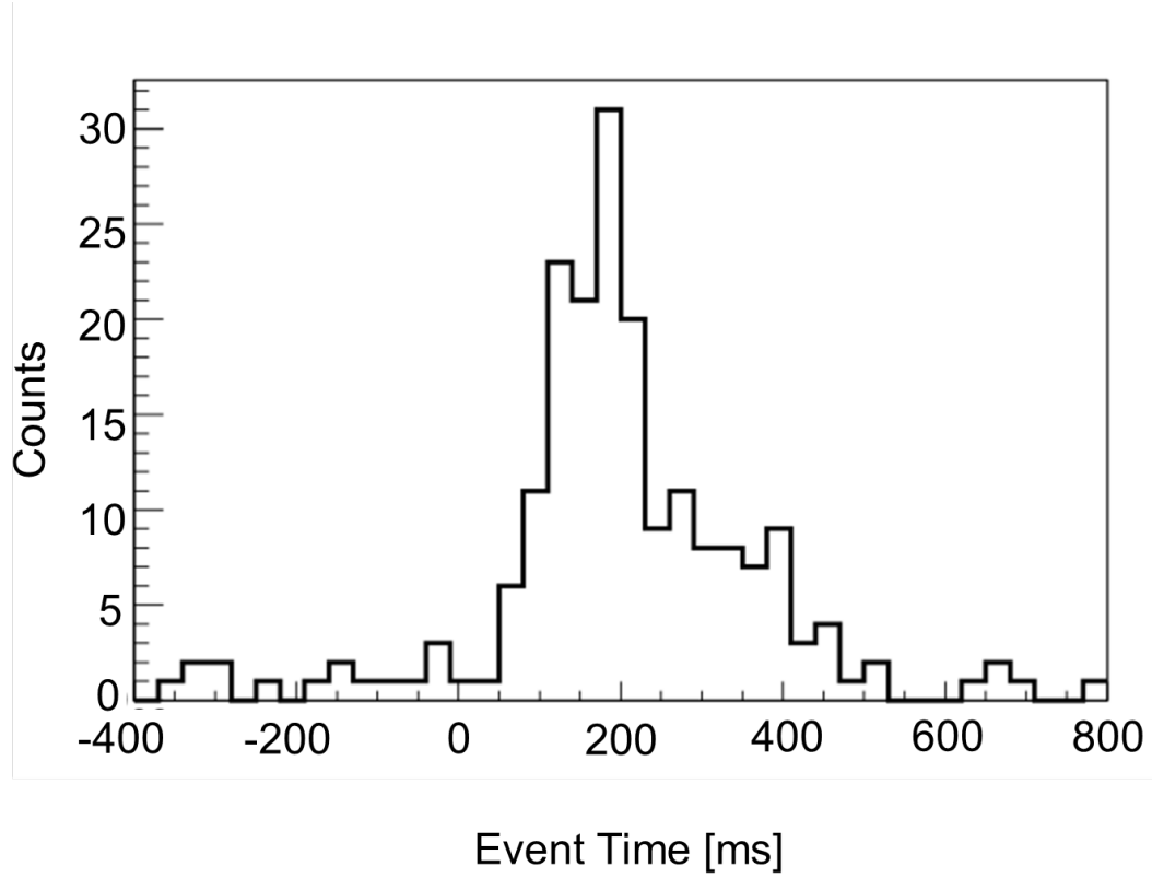
Figure 6.4: Timing structure of the \gamma rays associated with the fine structure peaks. It can be seen that the timing has a peak value after which the peak falls away as time increases.
