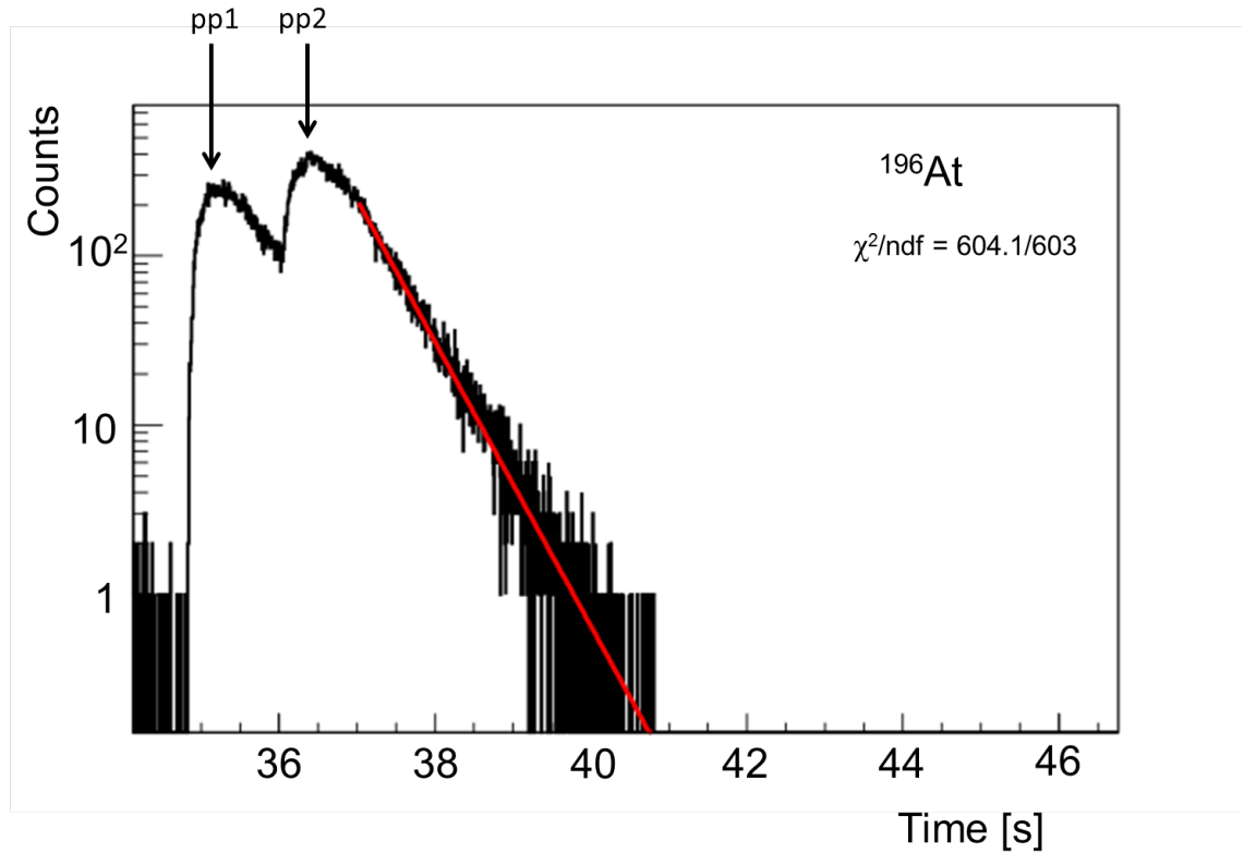
Figure 6.10: The time distribution for the 7053-keV \alpha decay of ^{196}\text{At} , following the implantation during two consecutive proton pulses PP1 and PP2, separated by 1.2 seconds. The “decay part” of the time distribution within the time interval of 2.4–6 s was fitted with an exponential function, resulting in a value of T_{1/2}(^{196}\text{At}) = 358(5) ms. The data from Si1 and Si2 were used.
