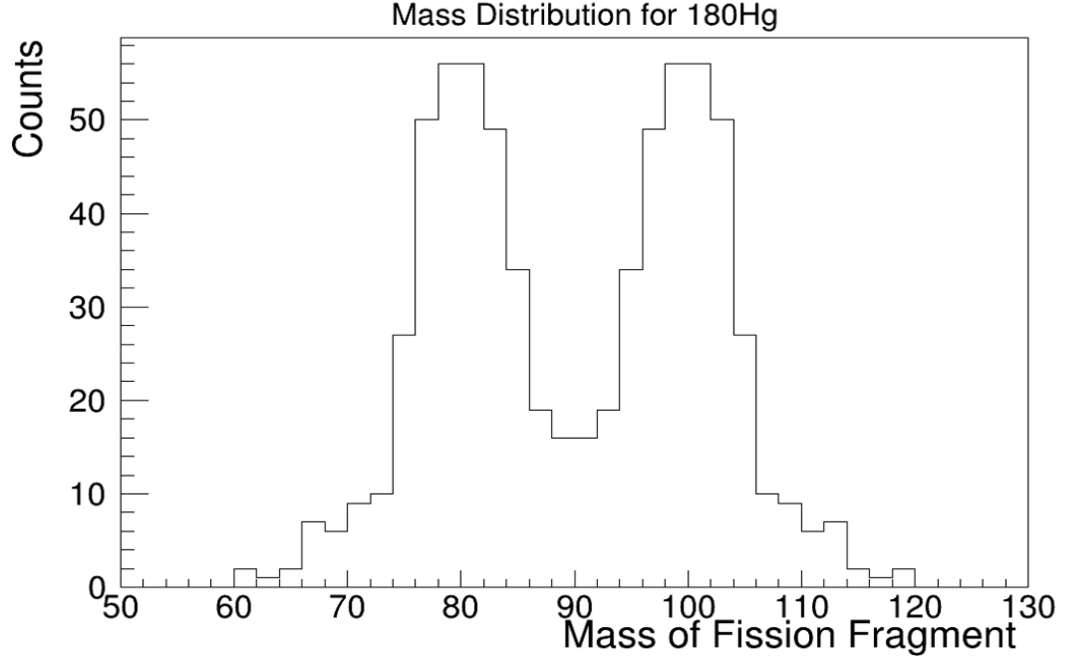
Figure 2.14: Asymmetric mass distribution of ^{180}\text{Hg} (adapted from [28]). ^{180}\text{Hg} was expected to fission symmetrically.
