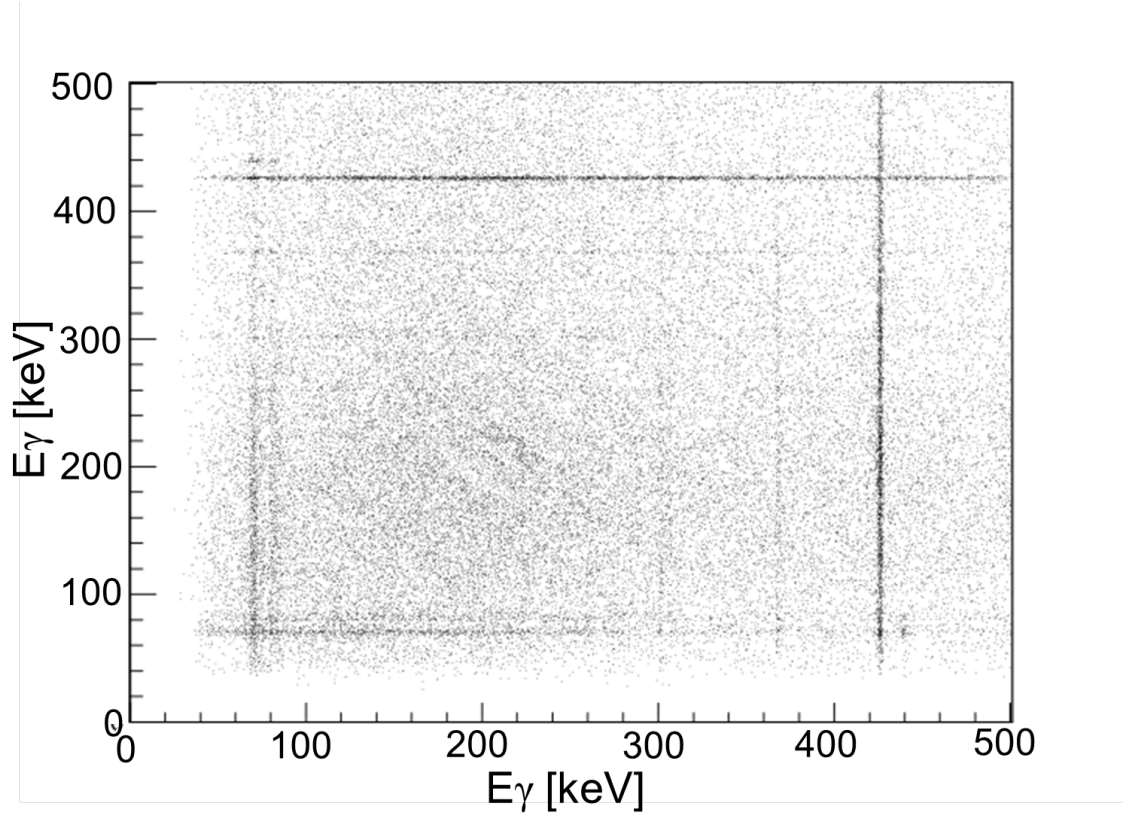
Figure 6.2: 2D \gamma-\gamma matrix of Ge1 against Ge2 used to determine if any coincidences could be seen. This was drawn by plotting all events in Ge1 against all events in Ge2. Due to no time conditions being applied, this made it difficult to see any coincidences.
