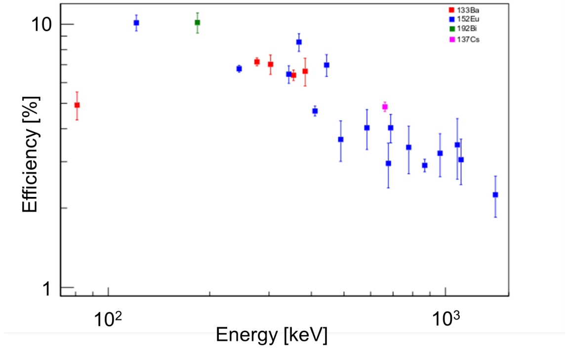
Figure 4.2: Resultant efficiency curve from plotting the efficiencies of the main \gamma transitions of the different calibration sources. Four calibration sources were used as indicated by the different colours. The four sources were a combination of three standard sources, ^{133}\text{Ba} , ^{152}\text{Eu} and ^{137}\text{Cs} and an experimental data point from ^{192}\text{Bi} .
