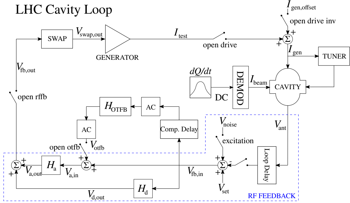
Figure 4.2: Block diagram of the LHC cavity loop model as it is implemented in BLonD.
