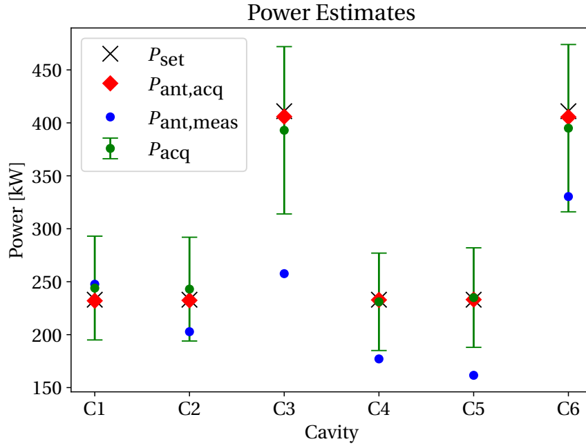
Figure 3.7: The data in Table 3.10 visualized. Note that the standard deviation of P_{\text{ant,acq}} and P_{\text{ant,meas}} were so small compared to that of P_{\text{acq}} that they are plotted as points.
