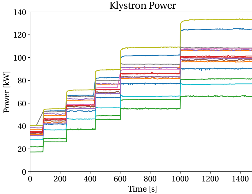
Figure 4.7: Measured forward klystron power from a ramp of the RF voltage from 7 MV to 12 MV in steps of 1 MV. Each step in the power signals in the plot correspond to a step in total RF voltage.
