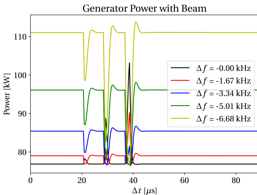
Figure 4.9: RF power for 12+36+72 bunches in the LHC with the OTFB open. The trace with a detuning of -6.68 kHz corresponds to optimum half-detuning value.
