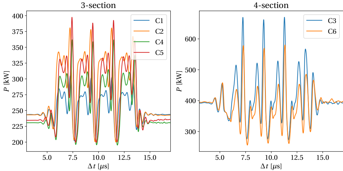
Figure 3.8: The power signal from acquisitions of each cavity. The average is taken for each cavity over 23 turns and 3 acquisitions.
