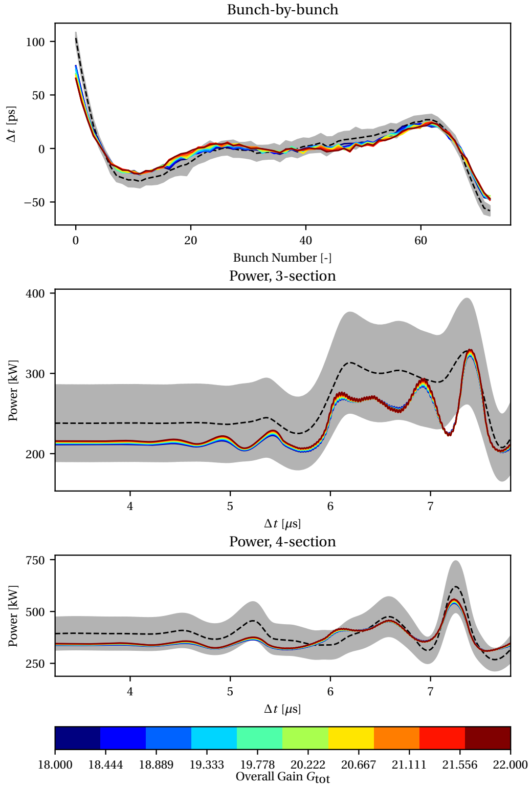
Figure D.1: Scan of the OTFB gain with all other simulation parameters equal to the baseline case except the transmitter gain G_{\text{tx}} . The resonant frequency of the TWCs were equal to the value that was initially designed (see Table 3.13).
