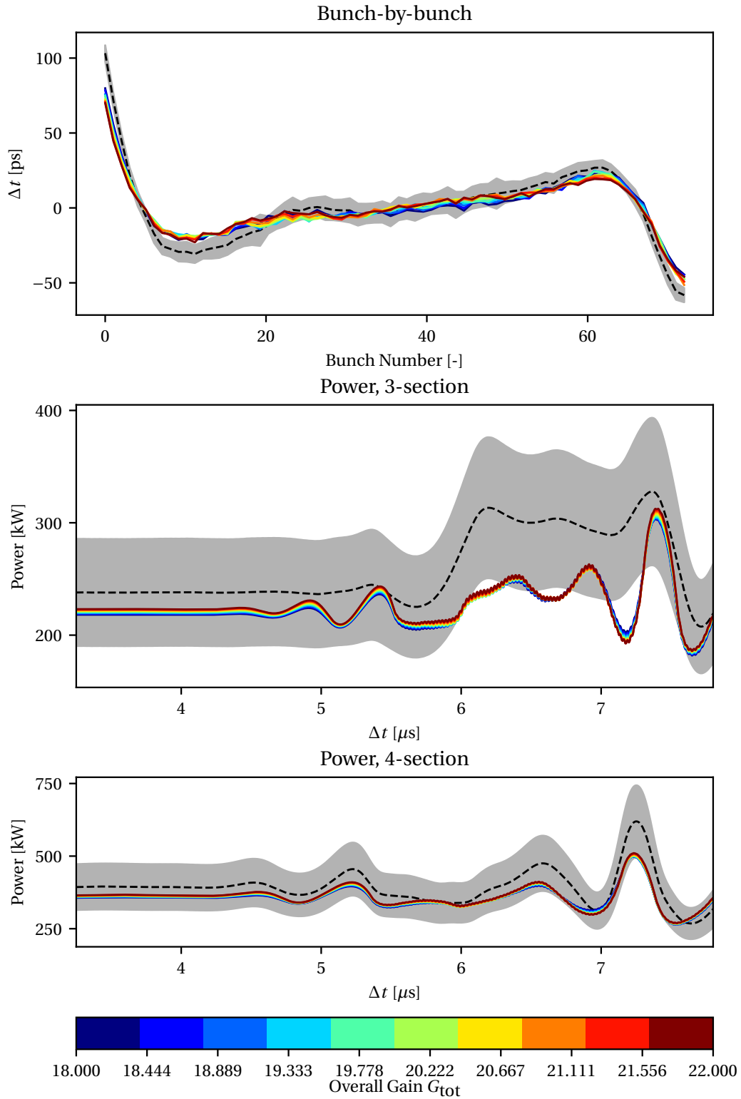
Figure D.2: Scan of the OTFB gain with all other simulation parameters equal to the baseline case except the transmitter gain G_{\text{tx}} . The resonant frequency of the TWCs were equal to the measured value in 2018 (see Table 3.13).
