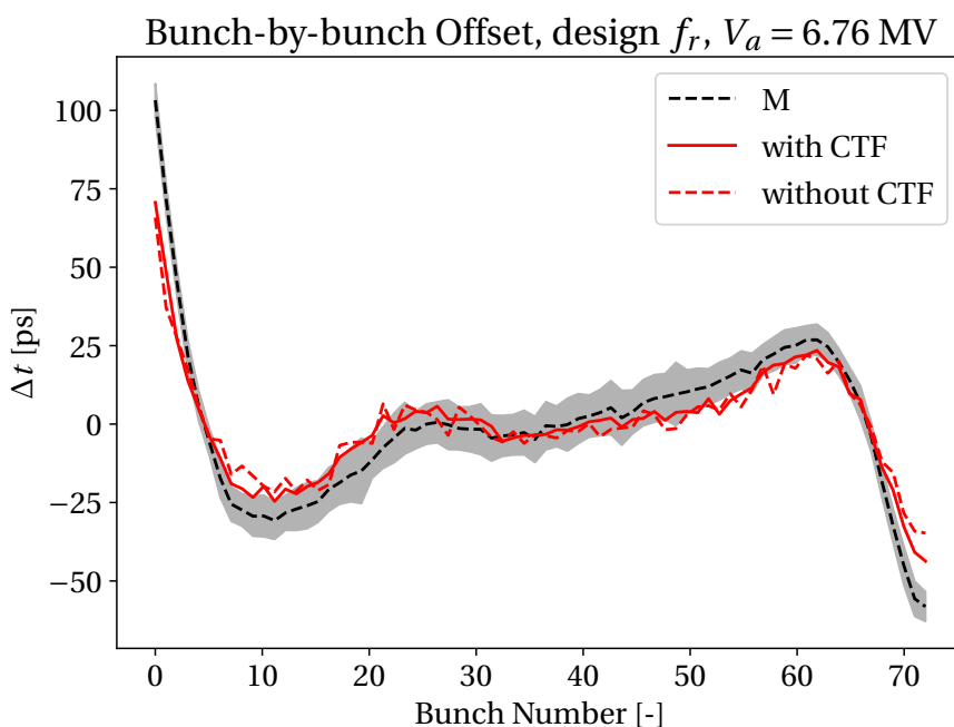
Figure 3.19: Bunch-by-bunch offset of the first batch in a simulation with V_{\text{ant}} = 6.76 MV and TWCs with their original design resonant frequencies. The full red trace is with the cable transfer function (CTF) and the dashed red trace is without.
