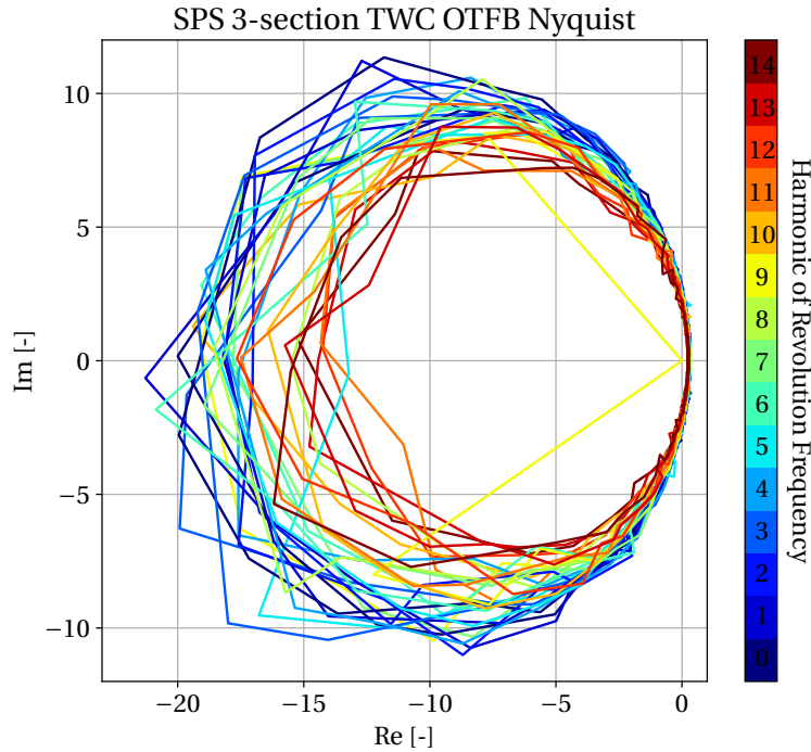
Figure 3.13: Nyquist plot of the 3-section TWC OTFB open loop response. The resonant frequency of the TWC was at 200.038 MHz.
