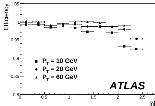
Figure 4.3: Track reconstruction efficiency as a function of |\eta| obtained on single electrons.
