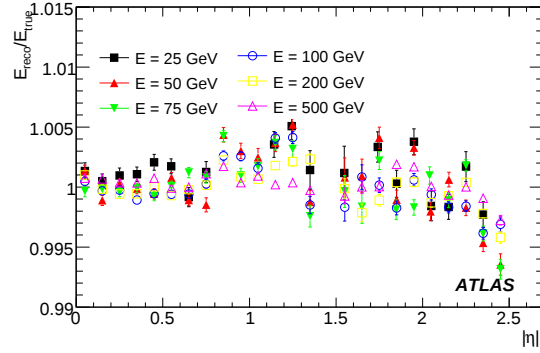
Figure 4.14: Linearity of the energy measurements for electrons as a function of |\eta| for different energies [81].
