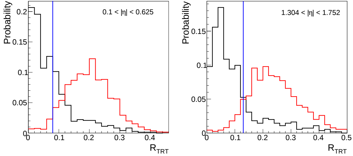
Figure 4.22: Distributions of R_{\text{TRT}} for signal electrons found in SUSY events (red) and fake electrons found in di-jet events (black). On the left-side, candidates with 0.1 < |\eta| < 0.625 are selected while, on the right-side, candidates with 1.304 < |\eta| < 1.752 . For the signal, candidates are selected after the tight set of cuts has been applied except for cuts on the TRT. For the background, no identification cut were applied in order to conserve significant statistics. The blue line indicates the chosen value for the lower cut on R_{\text{TRT}} for the corresponding |\eta| bin.
