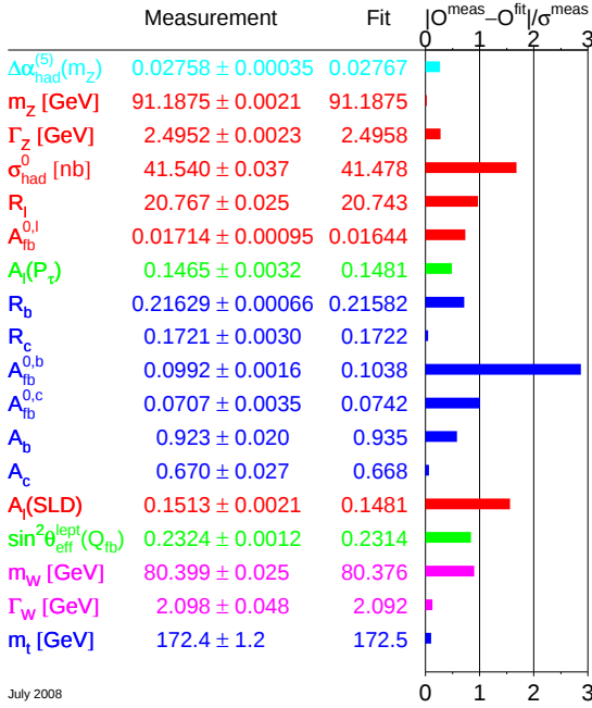
Figure 1: Latest agreements between the predicted values of some electroweak observables and their measurements [10].
