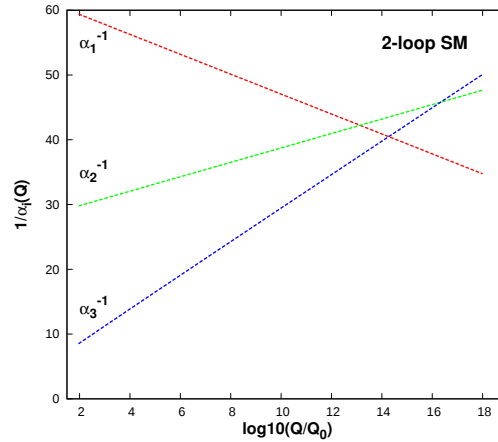
Figure 1.1: Running of the SM gauge couplings as a function of the renormalization scale Q for Q_0 = m_Z .
