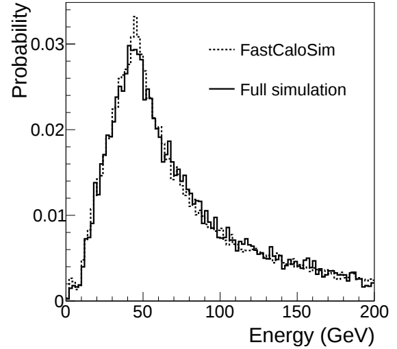
Figure 5.5: Energy spectra of electrons in Z \rightarrow ee events obtained with the Fast Calorimeter Simulation package or with the standard full simulation of the detector.
