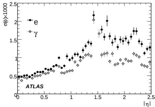
Figure 4.12: Expected \phi -position resolution as a function of |\eta| for electrons and photons with an energy of 100 GeV [81].
