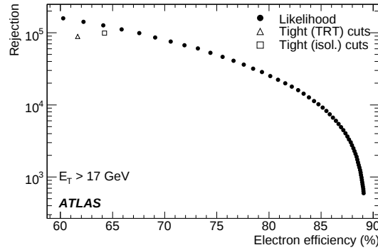
Figure 4.31: Jet rejection versus isolated electron efficiency obtained with a likelihood method (full circles) compared to the results from the two sets of tight cuts (open triangle and open square) [81].
