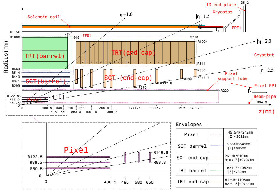
Figure 3.3: Plan view of a quarter of the ATLAS tracking detector.
