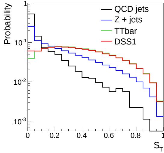
Figure 5.7: Distribution of the transverse sphericity for SUSY DSS1 events and SM processes.
