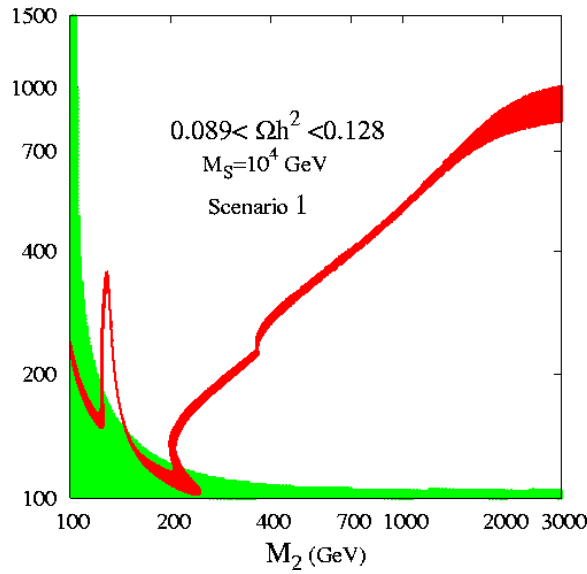
Figure 5.3: Regions of the (\mu, M_2) space allowed by WMAP constraints (red) and excluded by direct searches (green) [110]. The following parameters were used : m_S = 10^4 GeV, \tan \beta = 30 and gaugino masses are universal at the GUT scale.
