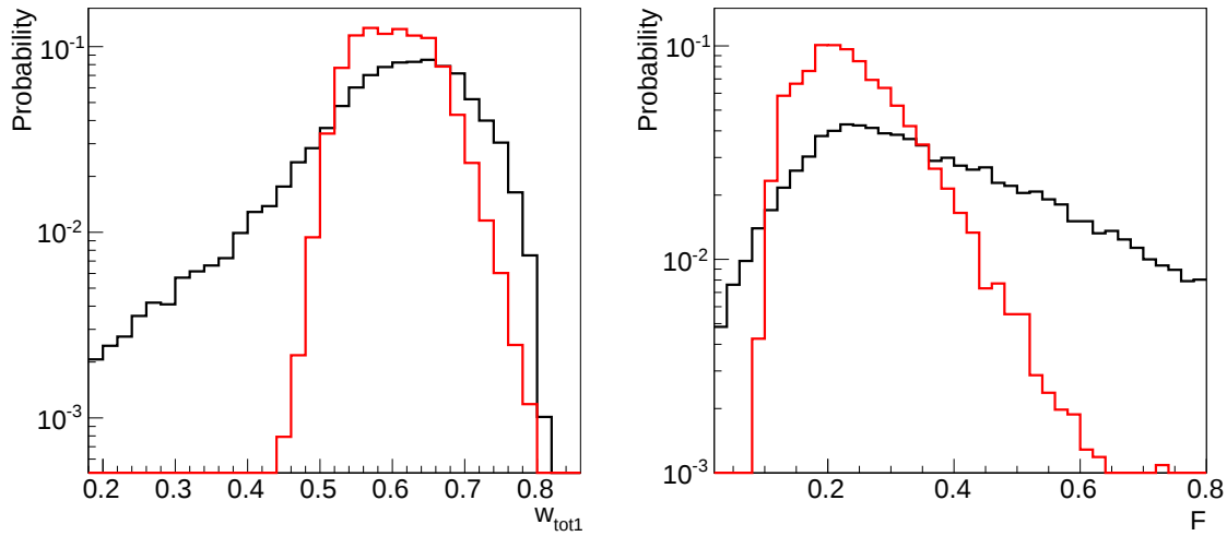
Figure 4.19: Left : distribution of the shower width in the first layer of the EM calorimeter for signal (red) and background (black). Right : distribution of the core shower shape in the first layer of the EM calorimeter for signal (red) and background (black).
