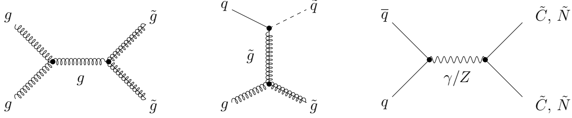
Figure 2.3: Typical processes contributing to the production of supersymmetry at the LHC.
