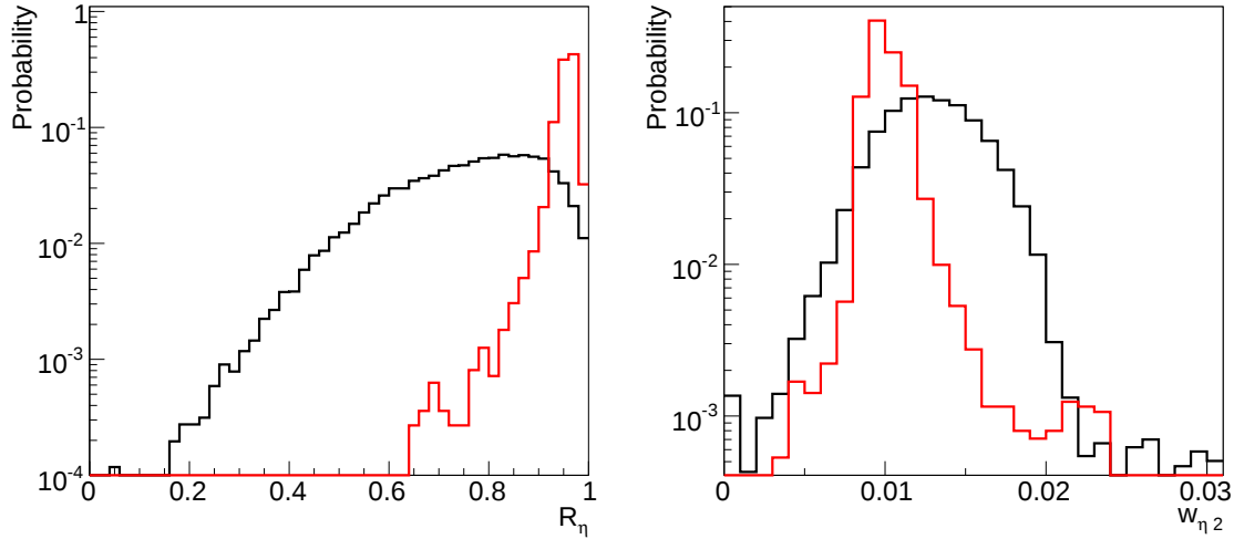
Figure 4.16: Left : distribution of the lateral shower shape in the second sampling of the EM calorimeter for signal (red) and background (black). Right : distribution of the weighted shower width in the second layer for signal (red) and background (black).
