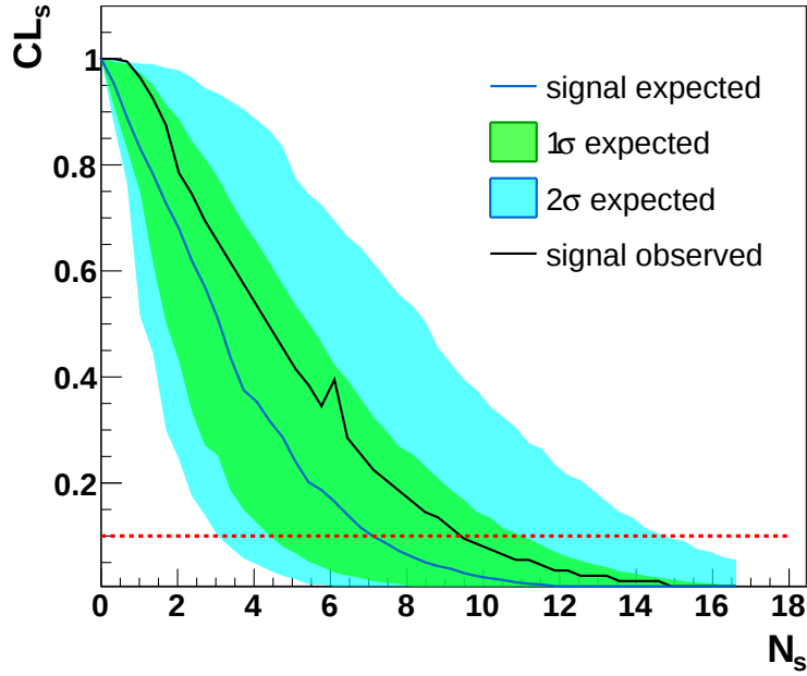
FIGURE 17.1: Two dimensional distribution of CL_s versus N_s for the expected and observed upper limits in the low-momentum sideband region 10–15 GeV/ c . The number of expected background events is 11.1^{+5.5}_{-5.8} while 14 events are observed in the data after all the signal selection. The CL_s results of the data (black line) are compared to the expected fluctuations in absence of a signal. The band of the expected limit is obtained from a combination of MC simulation and data single-photon efficiencies. The green (light blue) area is defined as having a statistical coverage of 34% (47.5%) on either side from the statistical median. The red dashed line corresponds to set the limit at 90% CL ( CL_s = 1 - CL = 0.1 ).
