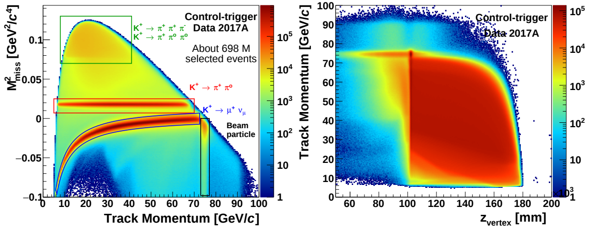
FIGURE 10.3: Left: Squared missing mass versus track momentum for the events passing the single-track selection. The momenta of the track and of the kaon are measured by the STRAW and GTK, respectively. The pion mass hypothesis is assumed for the STRAW 4-momentum. Right: Longitudinal position of the vertex versus STRAW track momentum for the events passing the single-track selection. The 75 GeV/c component is due to elastic scattering of beam particles with material upstream of the GTK3 station ( \simeq 102 m). The enhancement around the GTK3 longitudinal position spanning the whole momentum range is due to inelastic interactions of beam particles in the last GTK station. Correctly reconstructed kaon decays populate the region downstream the GTK3 station.
