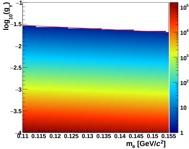
FIGURE 19.6: Lifetime of the ALP particle (in ns) according to Equations (A.3) and (A.4), as a function of \log_{10}(g_Y) and of the ALP mass. The red line corresponds to ALP lifetimes of 2 ns.
