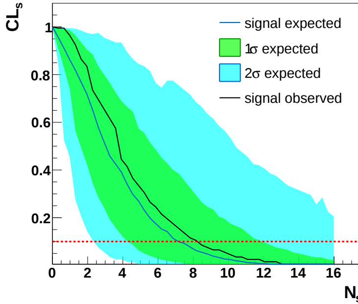
FIGURE 19.2: Two dimensional distribution of CL_s versus N_s for the expected and observed upper limits for the signal events in the \pi^+ momentum range 25–40 GeV/ c . The number of expected background events is 10^{+22}_{-8} while 12 events are observed in the data after the signal selection. The CL_s results of the data (black line) is compared to the expected fluctuations in absence of signal (blue line). The band of the expected limit is obtained from a combination of MC simulation and data single-photon efficiencies. The green (light blue) area is defined as having a statistical coverage of 34% (47.5%) on either side from the statistical median. The red dashed line corresponds to set the limit at 90% CL ( CL_s = 1 - CL = 0.1 ).
