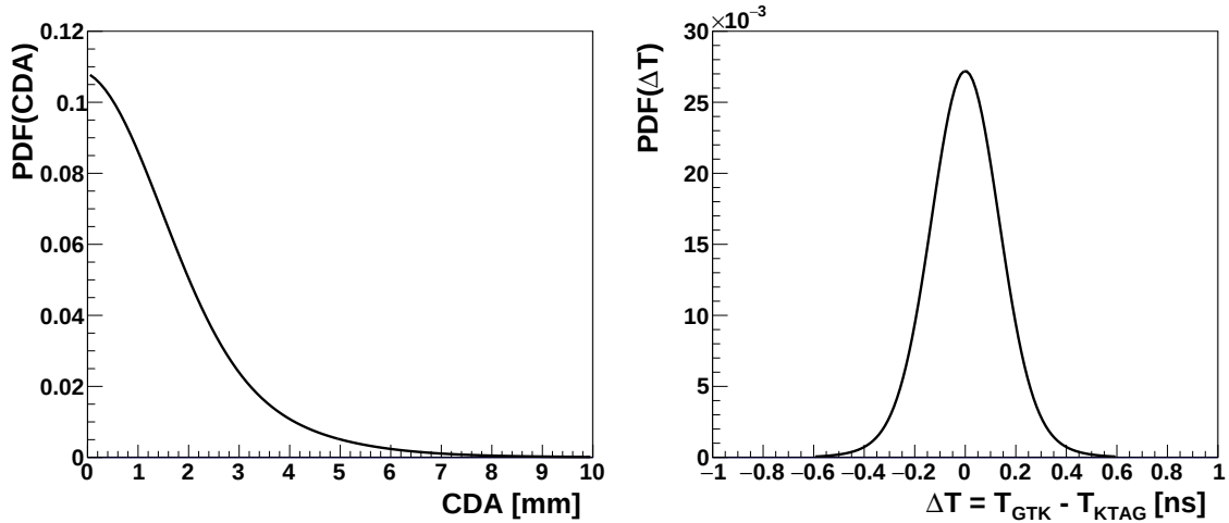
FIGURE 10.2: Left: Distribution of \text{PDF}(\text{CDA}) defined in Equation (10.7). Right: Distribution of \text{PDF}(\Delta T) defined in Equation (10.8).
