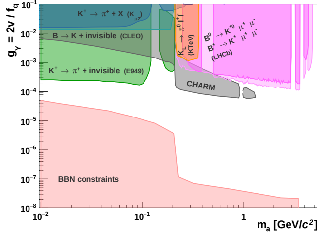
FIGURE 2.3: Search for an axion-like particle a according to the BC10 model of Reference [43]. The contributions from K^+ \rightarrow \pi^+ + \text{invisible} (E949 experiment [52, 53]), K^+ \rightarrow \pi^+ X ( K_{\mu 2} experiment [54]), B \rightarrow K + \text{invisible} (CLEO experiment [55]), the search for visible a decays (CHARM experiment [56]), K_L \rightarrow \pi^0 \ell^+ \ell^- (KTeV experiment [57]), B \rightarrow K^{(*)} \mu^+ \mu^- decays (LHCb experiment [58–60]) and constraints from the Big Bang nucleosynthesis are shown. Picture reproduced from Reference [43].
