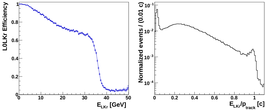
FIGURE 12.1: Left: L0LKr efficiency as a function of the energy deposited in the LKr calorimeter by the \pi^+ track. Right: Ratio of the energy released in the LKr calorimeter over the STRAW track momentum for \pi^+ particle derived from K^+ \rightarrow \pi^+ \pi^- \pi^+ decays [154].
