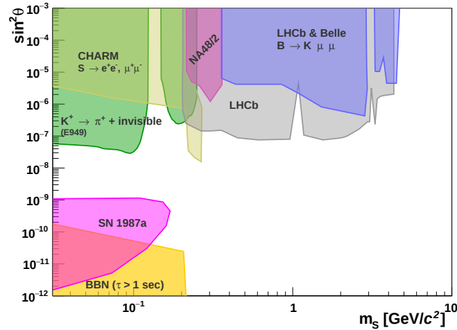
FIGURE 2.4: Search for a dark scalar S according to the BC4 model of Reference [43]. The contributions from K^+ \rightarrow \pi^+ + \text{invisible} (E949 experiment [63]), the search for visible S decays (CHARM experiment [56, 64]), K \rightarrow \pi \mu \mu (NA48/2 experiment [65]), B \rightarrow K \mu \mu (LHCb [59, 60] and Belle [66] experiments), astrophysical constraints (SN1987a [67–70]) and constraints from the Big Bang nucleosynthesis are shown. Picture reproduced from Reference [43].
