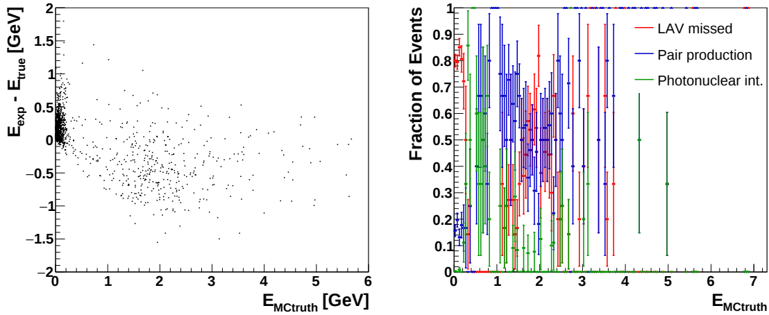
FIGURE 13.6: MC events flagged as inefficient, when probing the LAV detector to evaluate \epsilon_{\text{MC}}^{\text{TP}} . Left: Difference between the expected and true energy of the probed photon versus the true energy. Right: Fractional contribution to the inefficiency for the three categories defined in the text as a function of the true energy of the probed photon.
