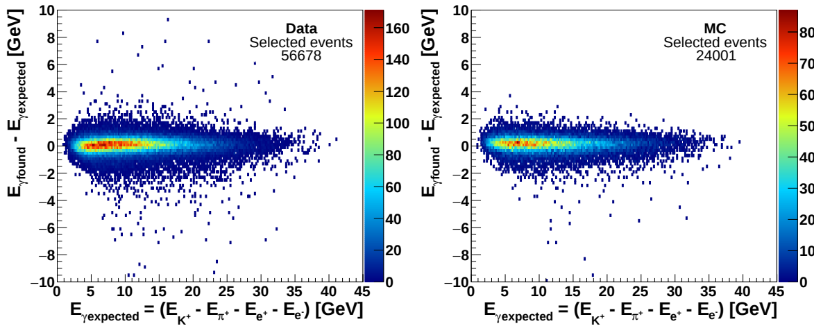
FIGURE 14.2: Difference between expected and reconstructed LKr photon energy as function of the expected energy (computed with the charged particle 4-momenta) for selected K_{2\pi_D} events in data (left) and MC (right).
