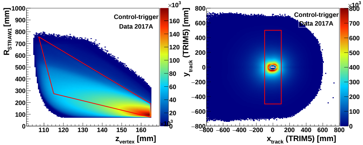
FIGURE 10.4: Left: Distribution of the STRAW track transverse distance with respect to the beam-line at STRAW chamber 1 versus the longitudinal position of kaon-track vertex. The selected events are those inside the red lines. Right: Distribution of the extrapolated STRAW track position at the TRIM5 magnet mid plane ( z_{\text{TRIM5}} = 101.8 m). The rejected events are those inside the red box.
