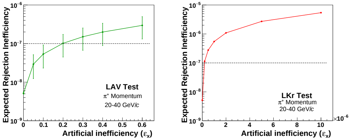
FIGURE 17.3: An artificial single-photon and a global inefficiencies \epsilon_x are introduced, one at a time, for the LAV ( left ) and LKr ( right ) respectively, and the expected \pi^0 rejection inefficiency is re-computed as \epsilon_x varies. Regions in which the expected rejection inefficiency is of \mathcal{O}(10^{-7}) or greater can now be cross-checked with the data. For \epsilon_x = 0 a \pi^0 rejection inefficiency of about 5 \times 10^{-9} is obtained according to the procedure described in Chapter 14. The momentum region between 20–40 GeV/c is used for this test.
