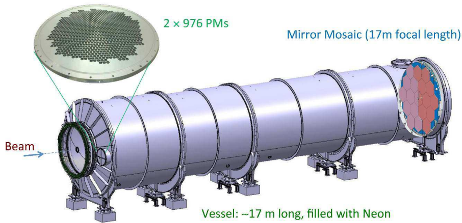
FIGURE 6.5: Layout of the RICH detector [104]. The vessel, 17 m long, is filled with neon gas at atmospheric pressure. The mirror mosaic and the photomultiplier flanges are visible in the downstream and upstream parts of the vessel, respectively.
