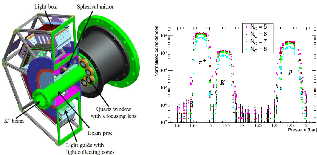
FIGURE 6.2: Left: Upstream part of the KTAG detector [104]. The emitted Cherenkov light exits the radiator gas through 8 quartz windows and then is focused on the light boxes. Right: Pressure scan of the N 2 gas at the nominal diaphragm aperture of 1.5 mm [104]. At 1.75 bar the presence of a kaon is required with at least 5 sectors in coincidence.
