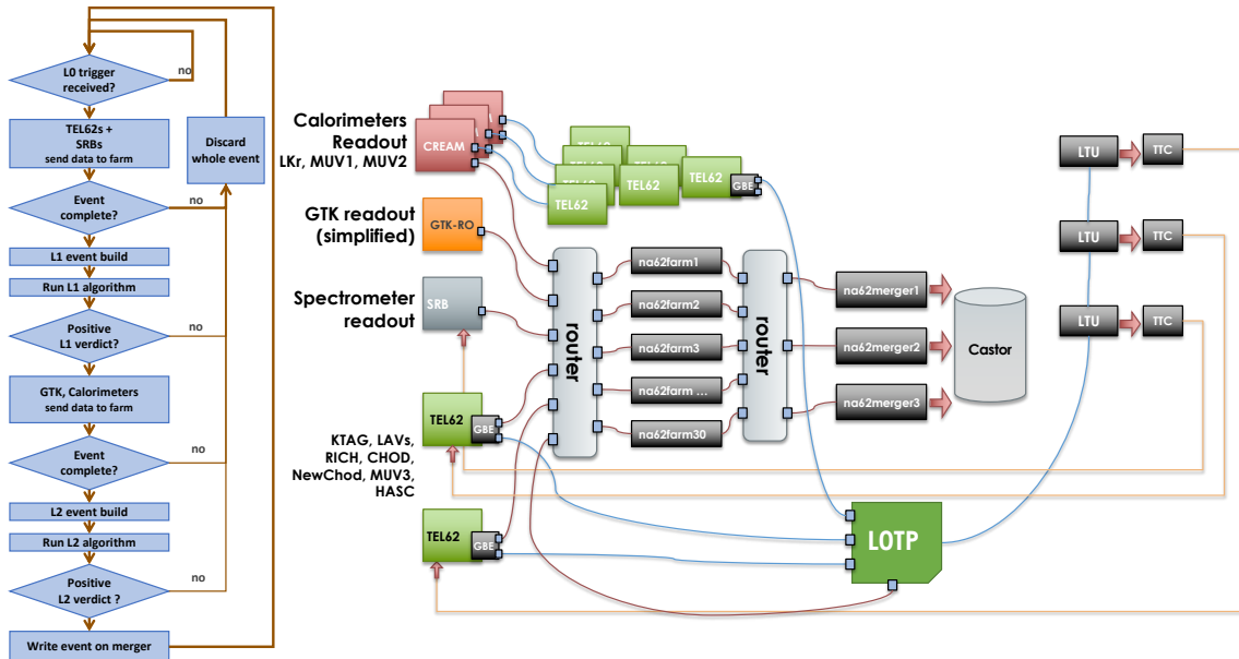
FIGURE 6.12: Data flow and overview of the unified trigger and data acquisition system [119].
