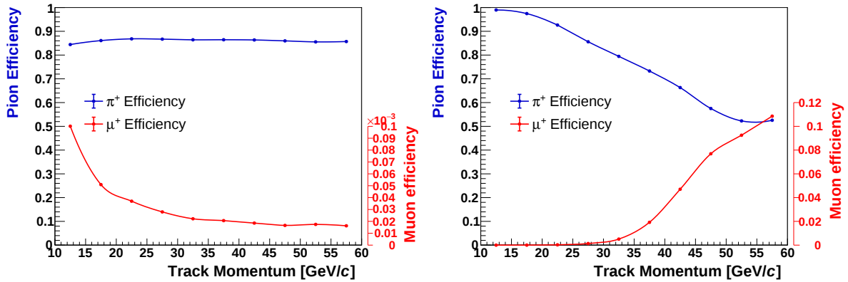
FIGURE 10.6: Left: Efficiency for the calorimetric-based pion-identification criteria detailed in the text, for \pi^+ and \mu^+ . Right: Efficiency for the RICH-based pion-identification criteria detailed in the text, for \pi^+ and \mu^+ .
