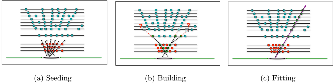
Figure 5.5: Illustration of the three steps of the CMS track reconstruction [166].
