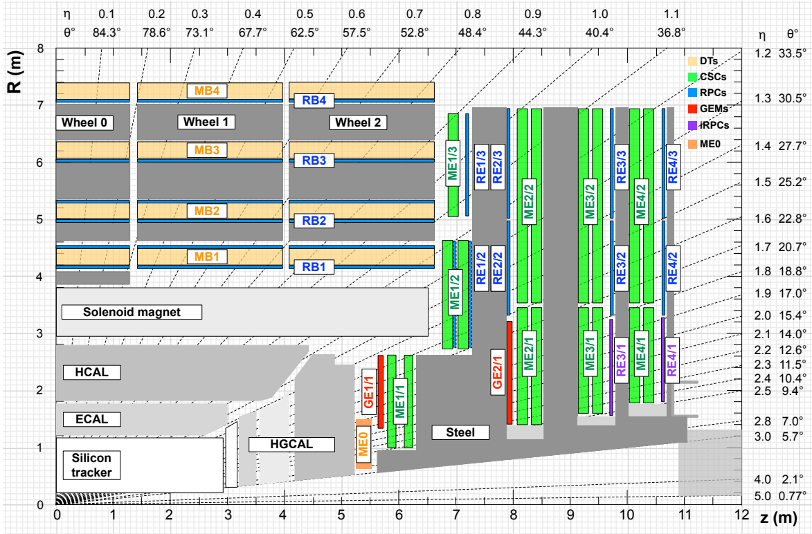
Figure 4.10: One-quarter section of the CMS detector in r - z view, featuring the four DT stations in the barrel (MB1–MB4, in orange), the four CSC stations in the endcap (ME1–ME4, in green), and the RPC stations (in blue). The Phase-II upgrades, some of them discussed below (RE3/1, RE4/1, GE1/1, GE2/1, ME0), are also included. MB = DT = Drift Tubes, ME = CSC = Cathode Strip Chambers, RB and RE = RPC = Resistive Plate Chambers, GE and ME0 = GEM = Gas Electron Multiplier, and iRPCs = improved RPC chambers) [124].
