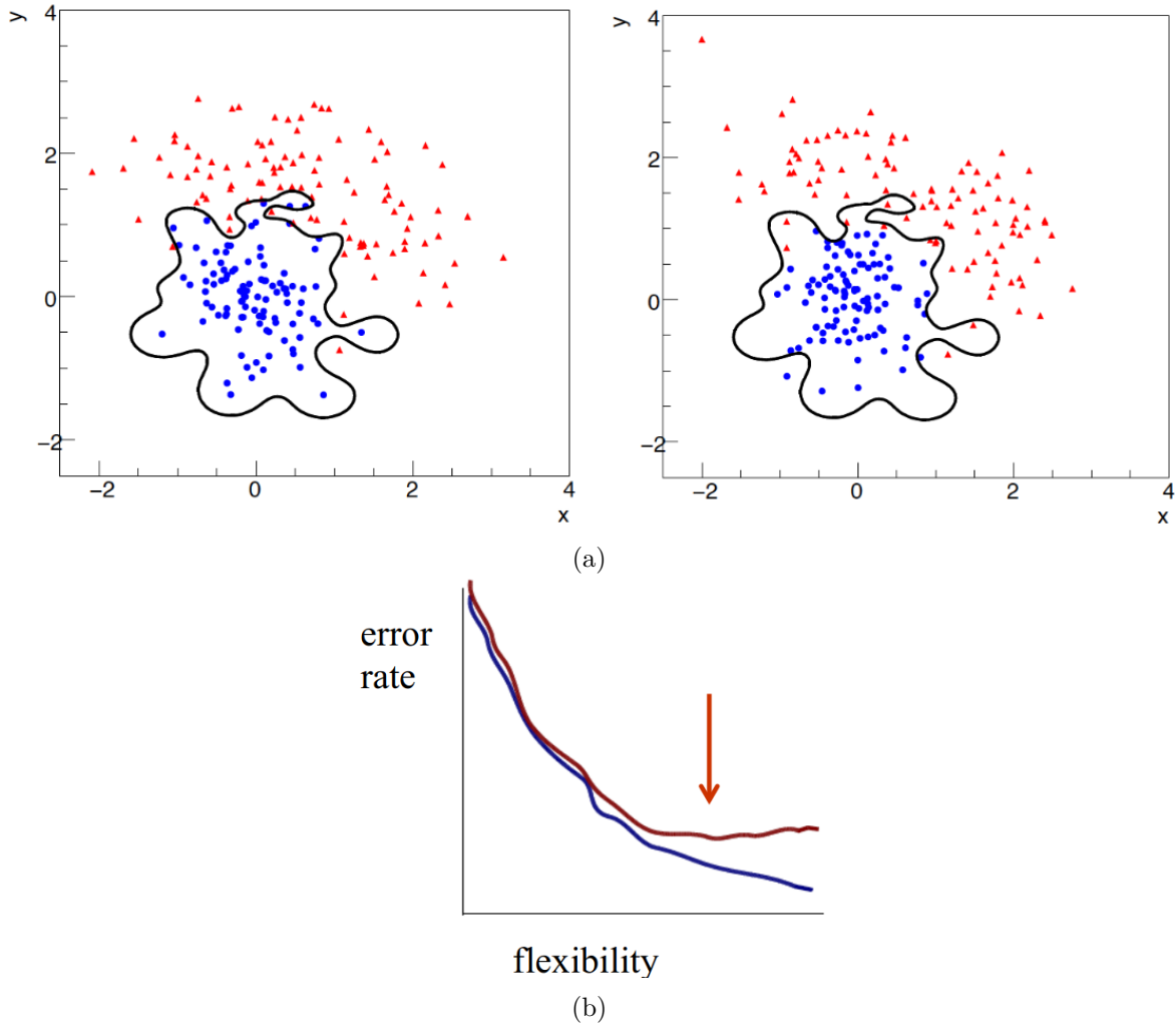
Figure 6.11: a) Performance of an overtrained classifier in the training sample (left) and in an independent test sample (right). b) Overtraining monitoring: error rate as a function of the model flexibility for the training sample (blue) and the test sample (red). The red arrow indicates the optimum point of flexibility at minimum error rate for the test sample. The increase in error rate for the test sample indicates overtraining [190].
