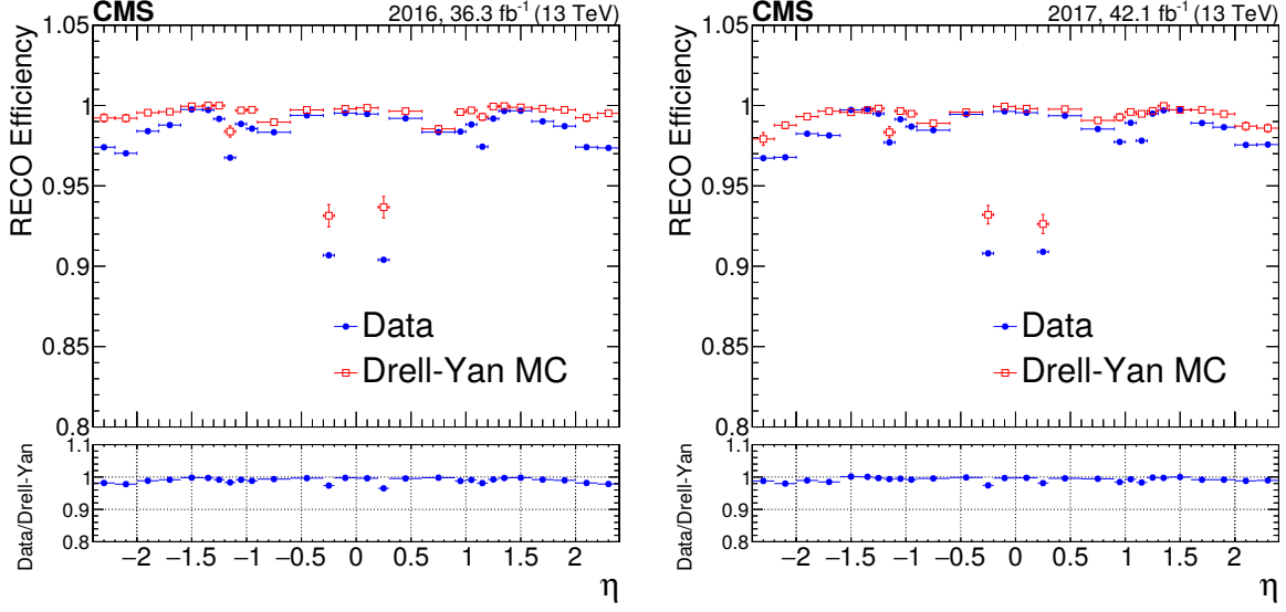
Figure 5.8: Standalone muon reconstruction efficiency as a function of the muon pseudorapidity for the 2016 (left) and 2017 (right) datasets. Data points are shown in blue, while the empty squares in red correspond to simulation [168].
