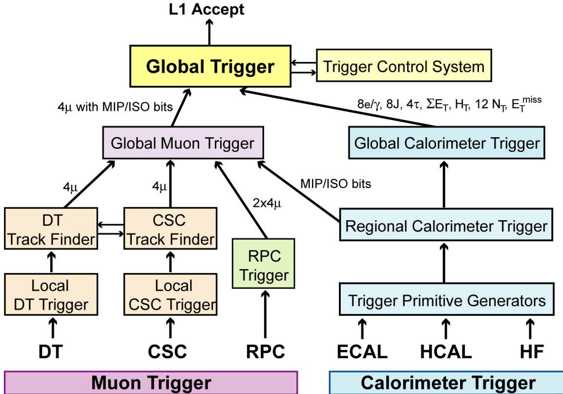
Figure 4.11: Architecture of the L1 trigger [27].
