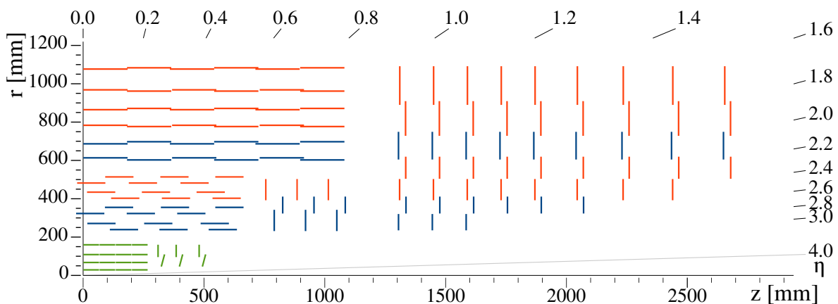
Figure 4.6: One quarter section of the Phase-I CMS tracking system in r - z view. The pixel detector is shown in green, single-sided strip modules in red and double-sided strip modules in blue [111].
