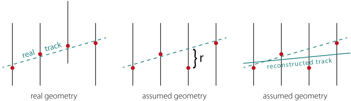
Figure C.2: Sketch representing the effect in the track reconstruction of an incorrect assumption on the position of one module. [230].
