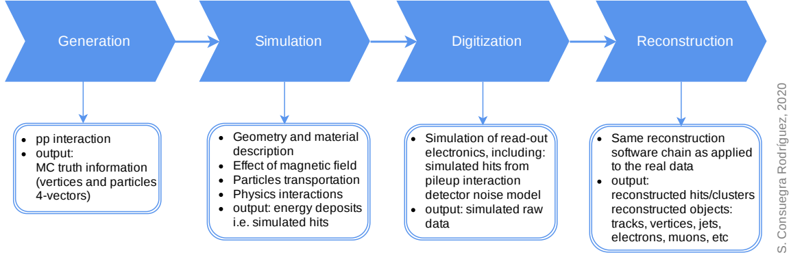
Figure 5.1: CMS simulation workflow.
