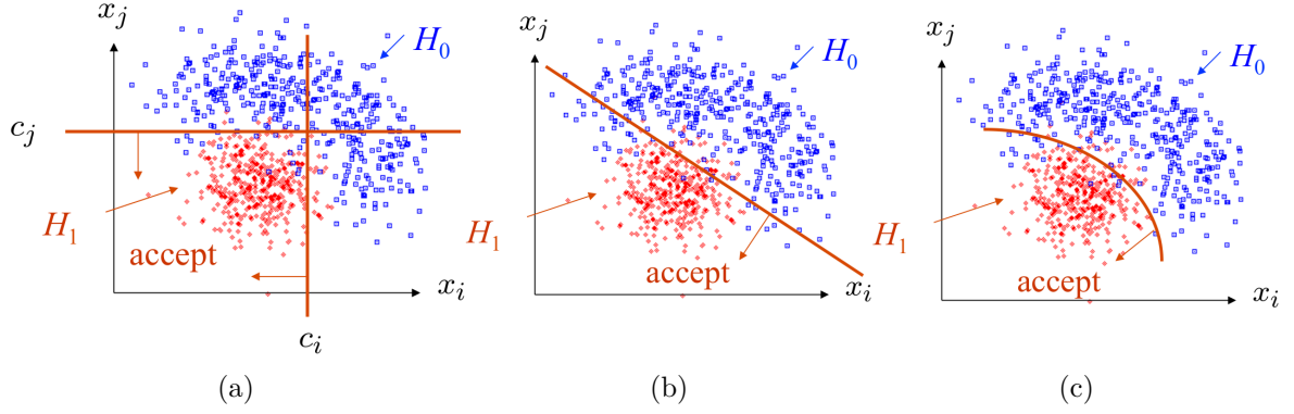
Figure 6.3: Visualization of decision boundaries. a) cut based decision boundary b) linear decision boundary c) non-linear decision boundary [190].
