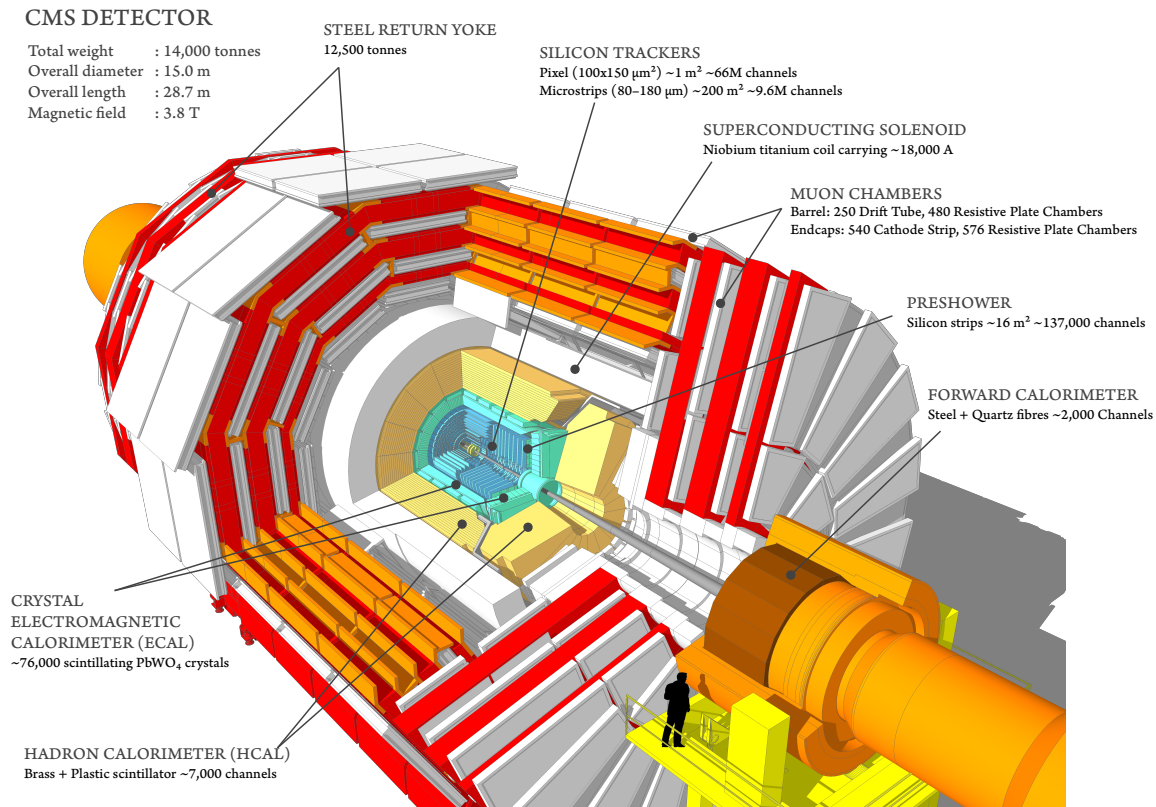
Figure 4.4: Sectional view of the CMS detector. [104].
