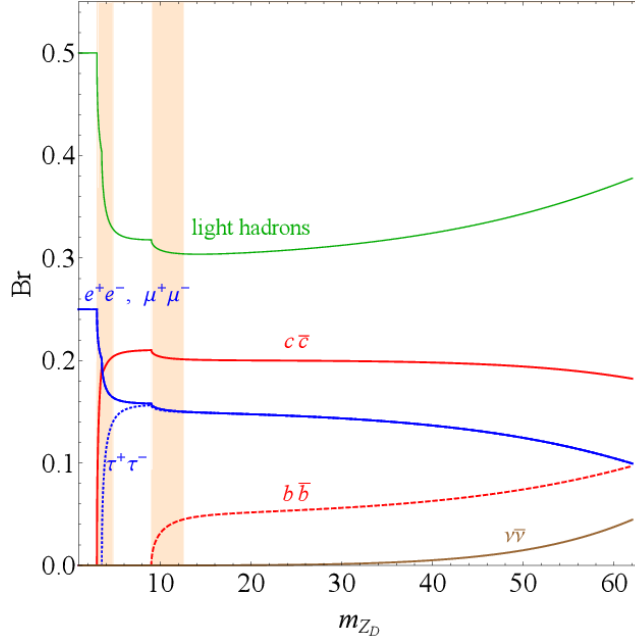
Figure 3.3: Branching ratios for dark photon decay at leading order and without QCD corrections from Ref. [26]. The label light hadrons refers to hadrons containing only up, down, and strange quarks. Decays of the dark photon to the dark sector are assumed to be kinematically forbidden. The simple theoretical calculations are probably invalidated in the shaded regions, due to missing threshold effects and QCD corrections, as well as the presence of hadronic resonances in these regions.
