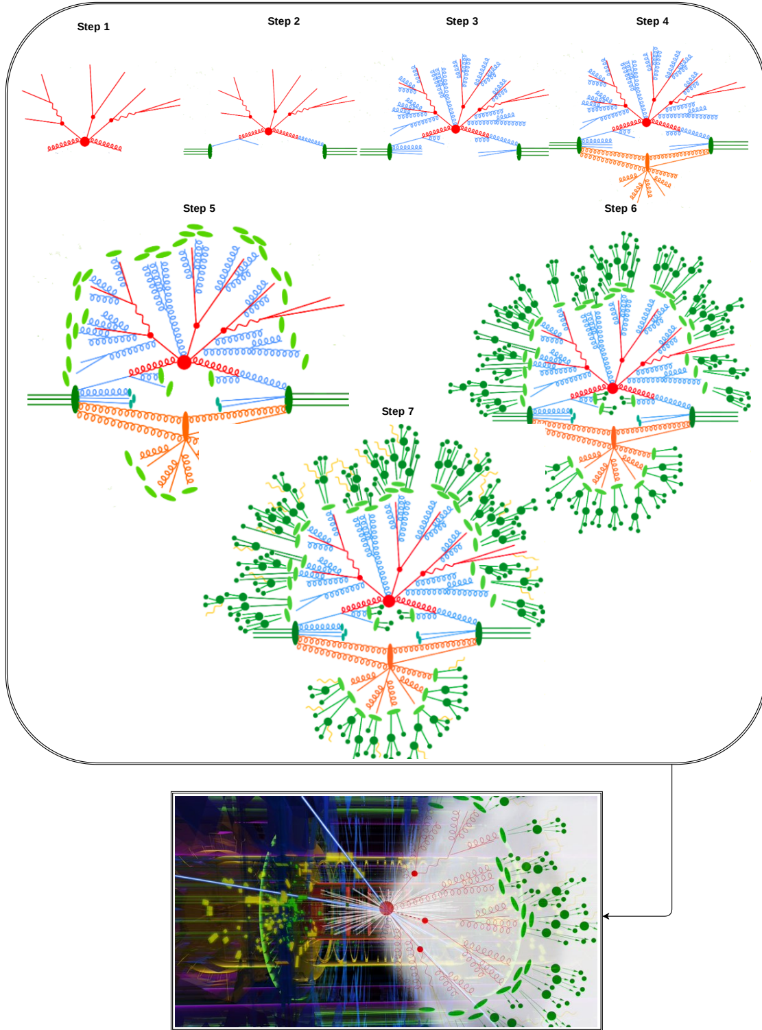
Figure 5.2: Overview of the event generation chain. Step 1: Hard scatter (red), matrix elements from first principles. Step 2: Incoming partons from the parton distribution functions (PDFs). Step 3: Radiative corrections, Initial State Radiation (ISR) and Final State Radiation (FSR) (blue). Step 4: Multi Parton Interaction (MPI) (orange). Step 5: Hadronization (light green). Step 6: Hadron decays from unstable resonances to final-state particles (dark green). Step 7: Photon radiation (occurs at any stage), QED corrections (yellow) [150,151].
