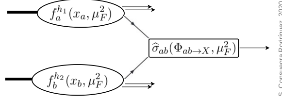
Figure 5.3: Schematic representation of a primary hard process.
