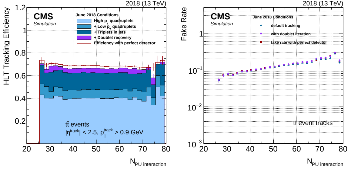
Figure 5.7: Tracking efficiency (left) and misreconstruction rate (right) as a function of the number of pileup interactions. The contributions to the total efficiency resulting from different tracking iterations are shown in different colors. The performance that would be achieved with a perfect detector is shown as a red line (left) and squares (right) [167].
