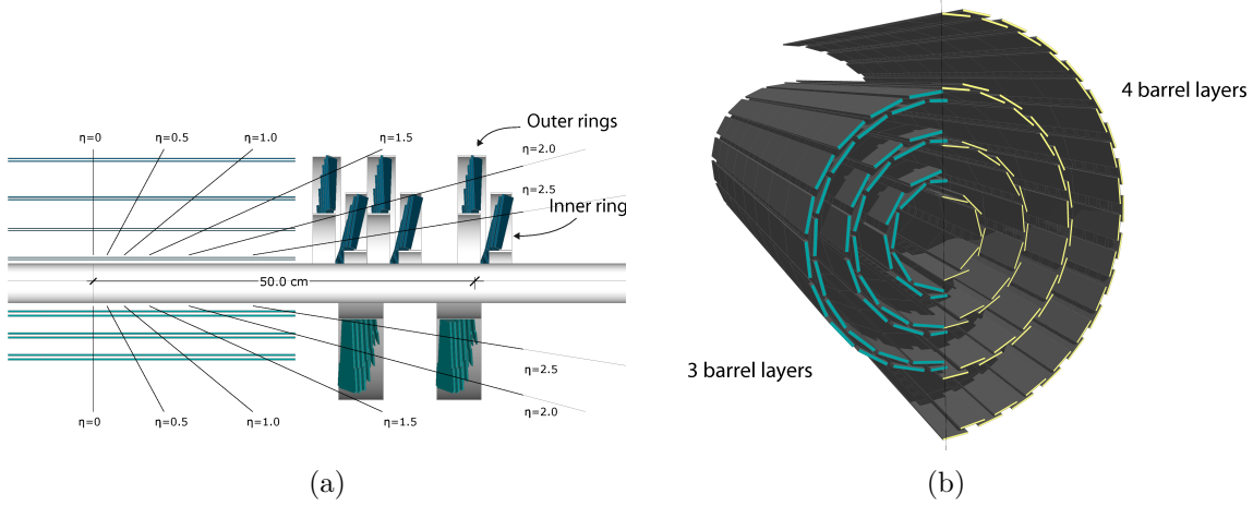
Figure 4.7: a) Comparison of conceptual layout and hit coverage as a function of pseudorapidity for the Phase-0 (bottom) and Phase-I (top) pixel detector. b) Transverse view comparing the original three-layer geometry (blue) with the upgraded four-layer geometry (yellow) of the pixel detector [113].
