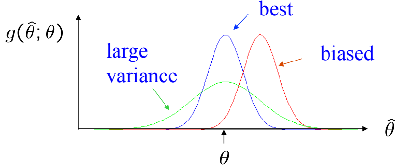
Figure 6.1: Distribution of a sampling pdf g(\hat{\theta}; \theta) as a function of the estimator \hat{\theta} . The estimator is: unbiased (in blue), biased (in red), and has a large variance (in green) [190].
