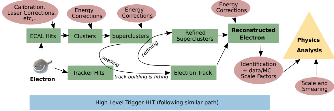
Figure 5.11: Simplified overview of CMS electron reconstruction workflow [169].
