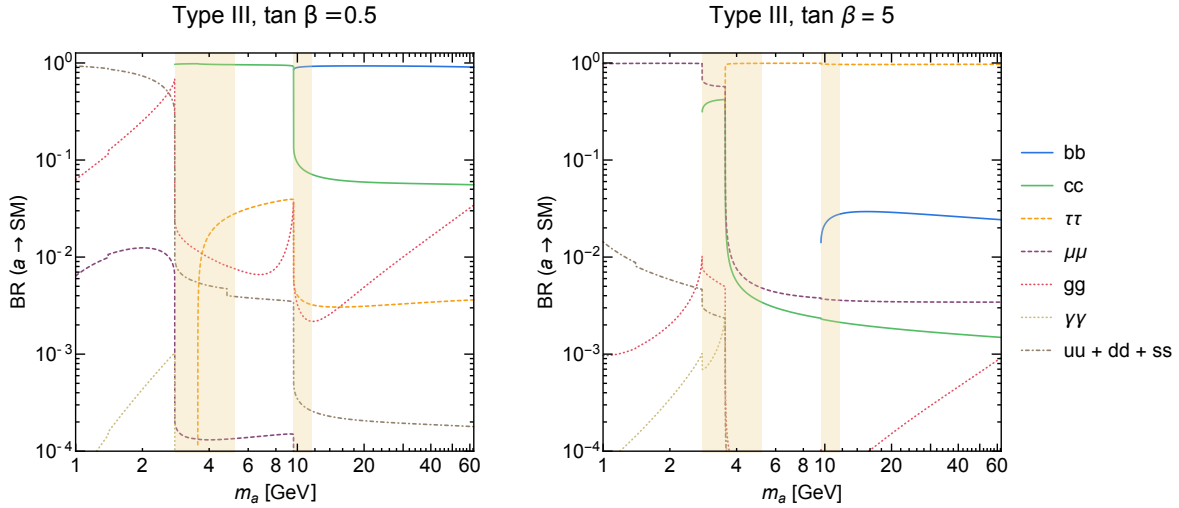
Figure 3.1: Branching ratios of a singlet-like pseudoscalar in the 2HDM+S for Type III Yukawa couplings. Decays to quarkonia probably invalidate theoretical calculations in the shaded regions [26].
