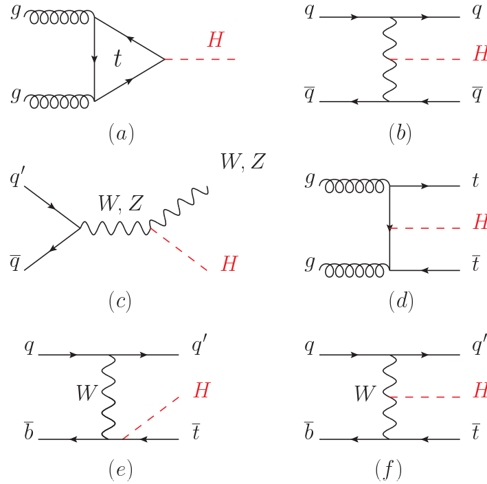
Figure 2.2: The main leading order Feynman diagrams contributing to the Higgs boson production: (a) gluon fusion, (b) Vector-boson fusion, (c) Higgs-strahlung (or associated production with a gauge boson), (d) associated production with a pair of top (or bottom) quarks, (e-f) production in association with a single top quark [38].
