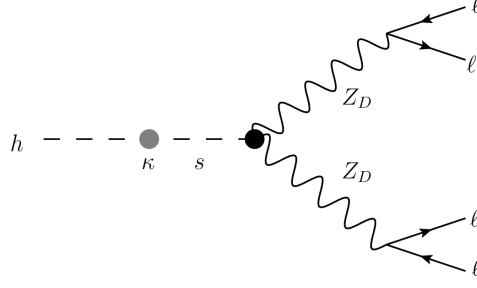
Figure 3.2: Exotic Higgs boson decay to four leptons induced by intermediate dark vector bosons via the Higgs portal, where s is a dark Higgs boson. The Z_D gauge bosons decay to SM particles through kinetic mixing with the hypercharge field or through mass mixing with the Z boson. The HZ_D Z_D vertex factor is proportional to \kappa [50].
