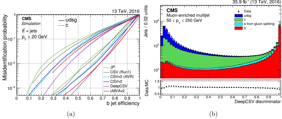
Figure 5.15: a) Misidentification probability for c and light-flavor jets as a function of the b -jet identification efficiency applied to jets in tt events. b) DeepCSV discriminator distribution in data compared to simulation for jets in a muon-enriched multijet sample. The simulation is normalized to the number of entries in data [176].
