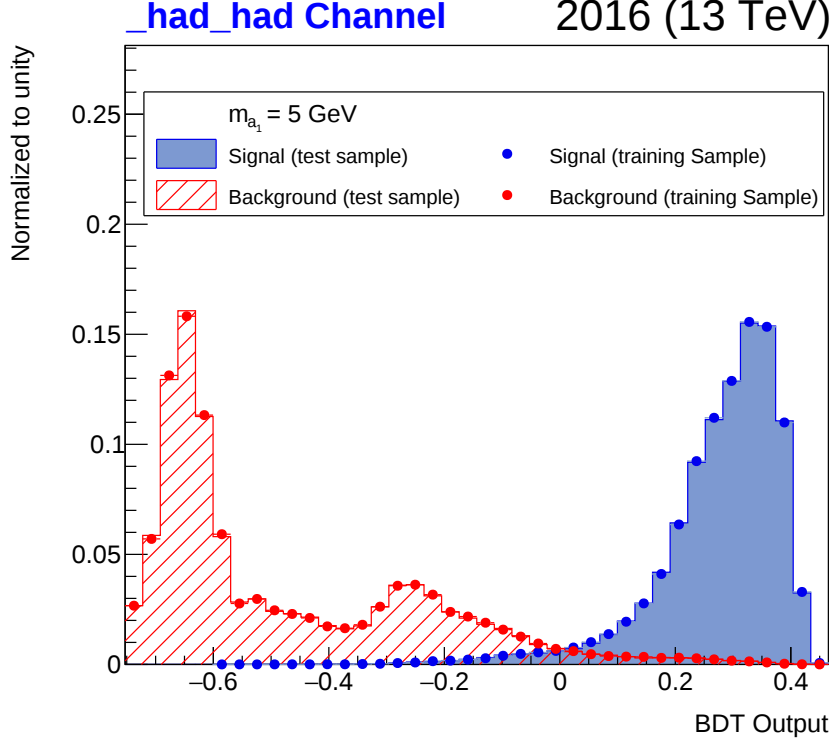
Figure 7.10: Signal and background distributions for the trained classifier. The test (histograms) and training (points with error bars) samples are superimposed for the signal and background classes, to check the overtraining of the classifier. The signal sample corresponds to m_{a_1(Z_D)} = 5 GeV and the training of the classifier is done for the 2016 analysis in the hadron-hadron category.
