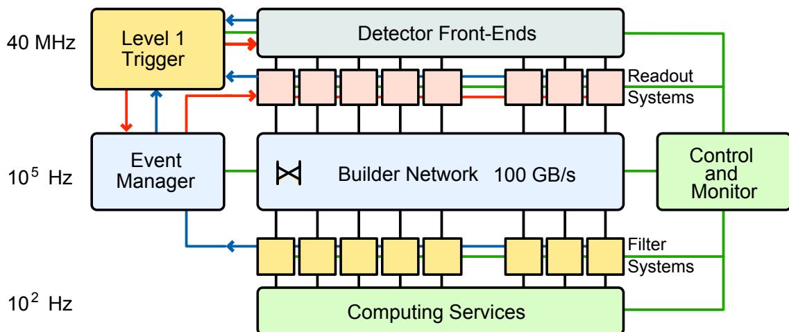
Figure 4.13: Architecture of the DAQ system [27].
