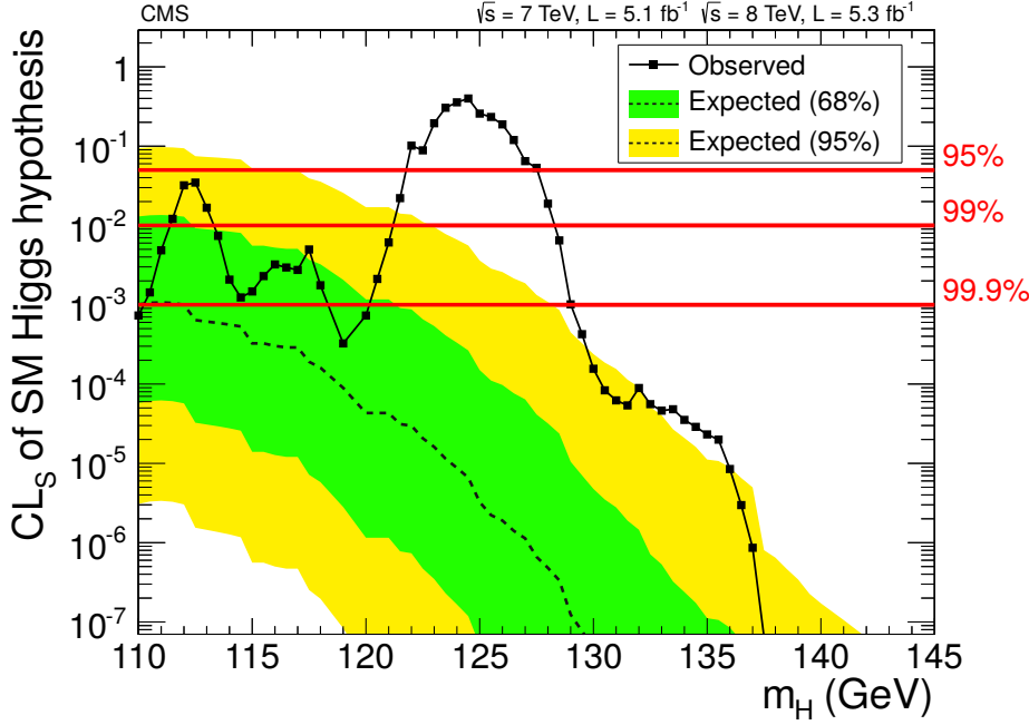
Figure 6.9: The CLs values for the SM Higgs boson hypothesis as a function of the Higgs boson mass in the mass range between 110 and 145 GeV. The expected upper limits are represented by their median (dashed line) and by the 68% (green) and 95% (yellow) CL bands [9].
