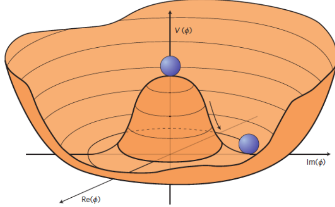
Figure 2.1: Illustration of the Higgs potential for \mu^2 < 0 [39].
