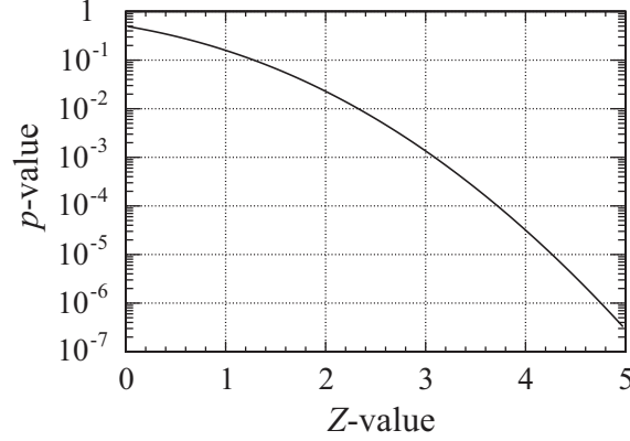
Figure 6.7: One-sided tail probability (p-value) vs. Z-value for a unit Gaussian probability density function [184].
