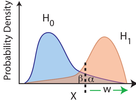
Figure 6.2: Sketch of the distribution of a test statistic under the null and alternative hypotheses. The size \alpha and power \beta of the test are depicted [191].
