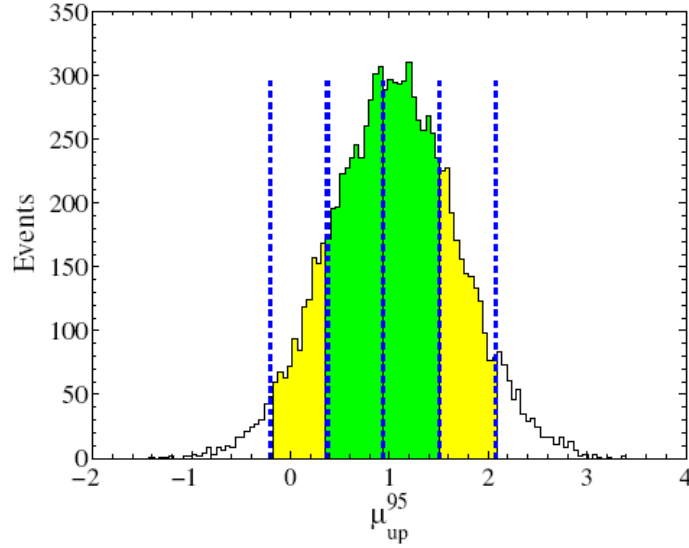
Figure 6.8: Median of \mu_{\text{up}} , 68% and 95% CL bands, for mass point m_H = 95 GeV. The \pm 1\sigma ( 2\sigma ) regions are depicted in green (yellow) [190].
