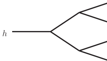
Figure 3.4: The exotic Higgs decay topology h \rightarrow 2 \rightarrow 4 .
