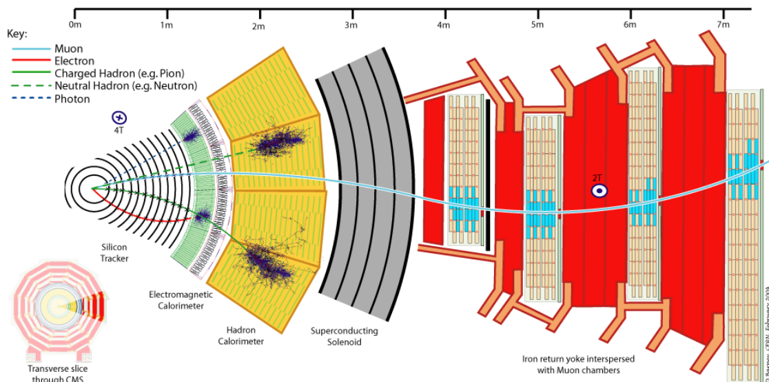
Figure 4.5: Transverse section of the CMS detector illustrating the interaction of the particles in each of the main subdetectors [109].
