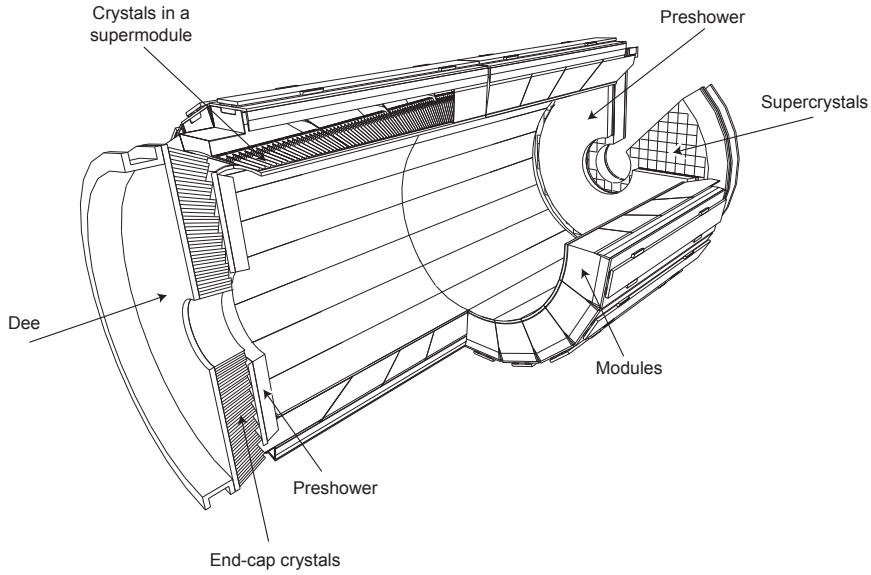
Figure 4.8: Layout of the CMS electromagnetic calorimeter, depicting the barrel, the two endcaps, and the preshower detectors [117].
