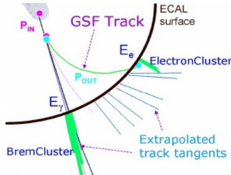
Figure 5.10: Sketch representing the components of CMS electron reconstruction [140].
