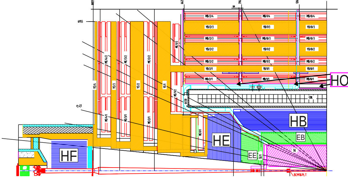
Figure 4.9: One quarter section of the CMS detector in r-z view, showing the location of the HB, HE, HO, and HF subsystems of the HCAL detector [120].
