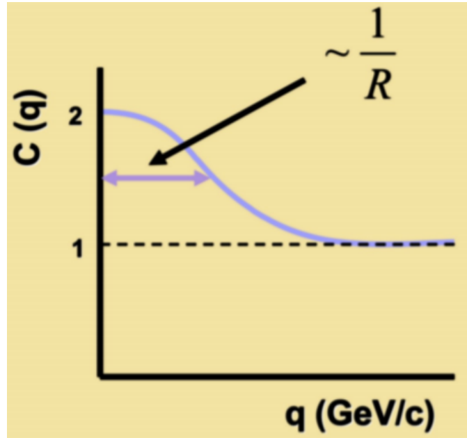
Figure 1.1: The k^* distribution (Image credit: J. Pluta (Warsaw University of Technology))
