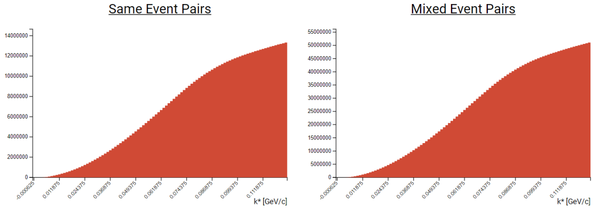
Figure 6.2: Example of the Numerator and Denominator Histograms.
