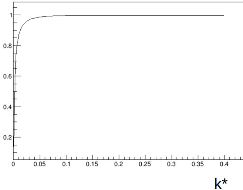
Figure 1.2: An example of the Coulomb function.
