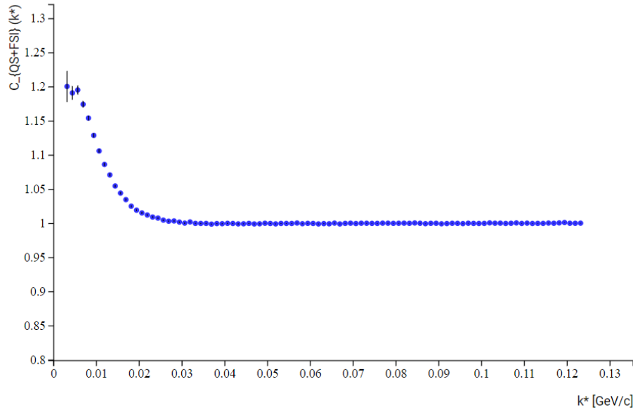
Figure 6.5: An example of the normalized correlation function.
