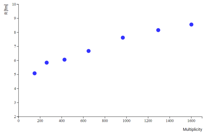
Figure 6.10: An example of the Radii vs Multiplicity plot.
