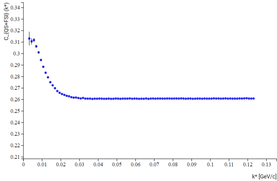
Figure 6.3: An example of the correlation function (Divided Histogram).
