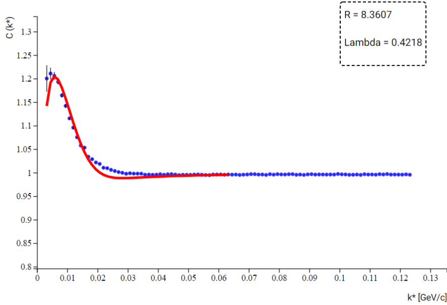
Figure 6.7: An example of a fitted correlation function, with the display of the free parameters.
