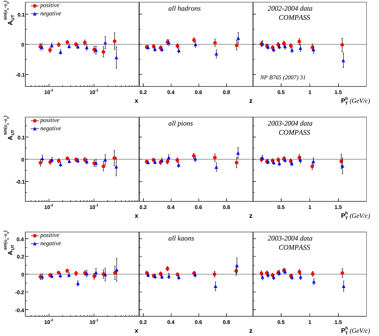
Figure 4.14: Extracted Sivers asymmetry ( A_{UT}^{\sin(\phi_h - \phi_s)} ) for unidentified hadrons (top row), pions (middle row) and kaons (bottom row) as a function of x , z and P_T^h
