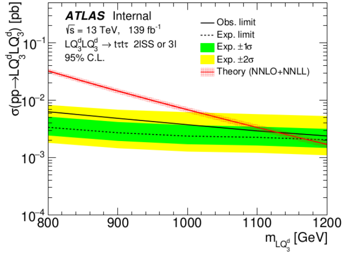
Figure 3.5: The 95% confidence level observed and expected upper limit in 2lSS \text{ or } 3l + \geq 1\tau_{had} channel after taking all systematics uncertainties into account [11][12] (Figure 75).
