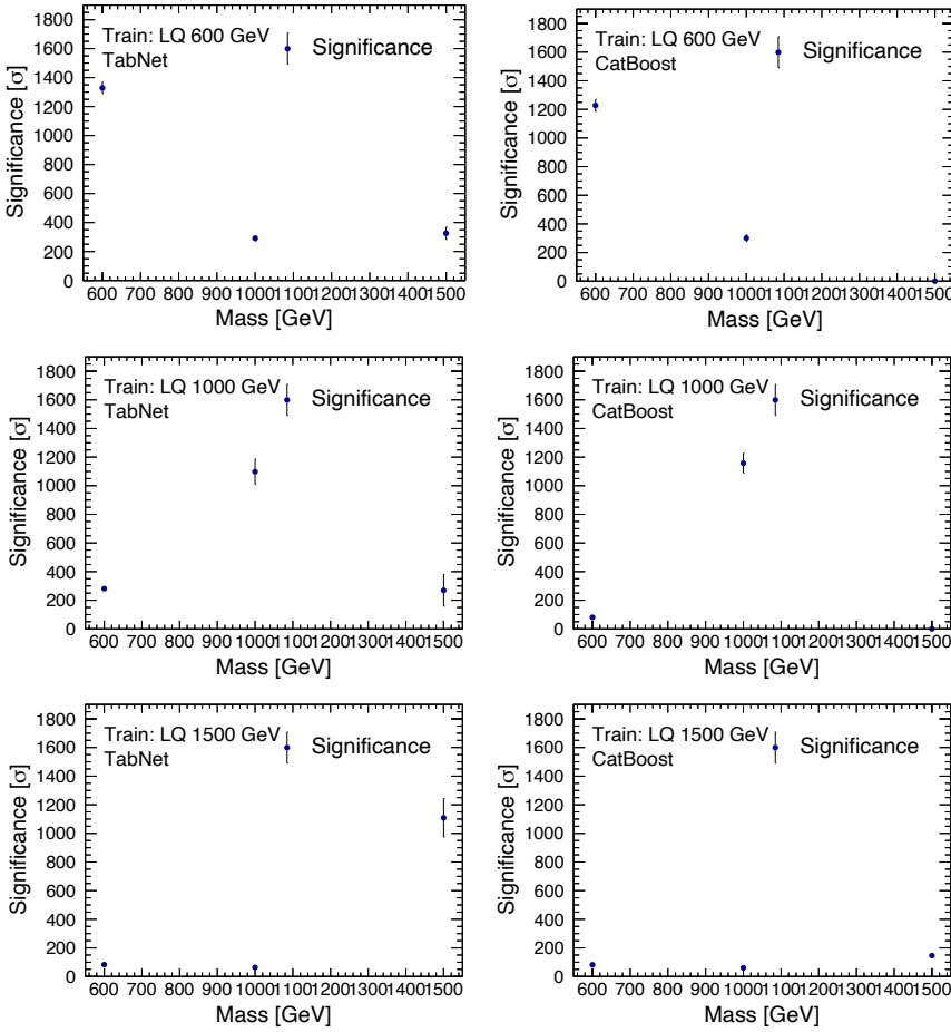
Figure 8.3: CatBoost and TabNet trained on Top: 600 GeV, Middle: 1000 GeV, Bottom: 1500 GeV.
