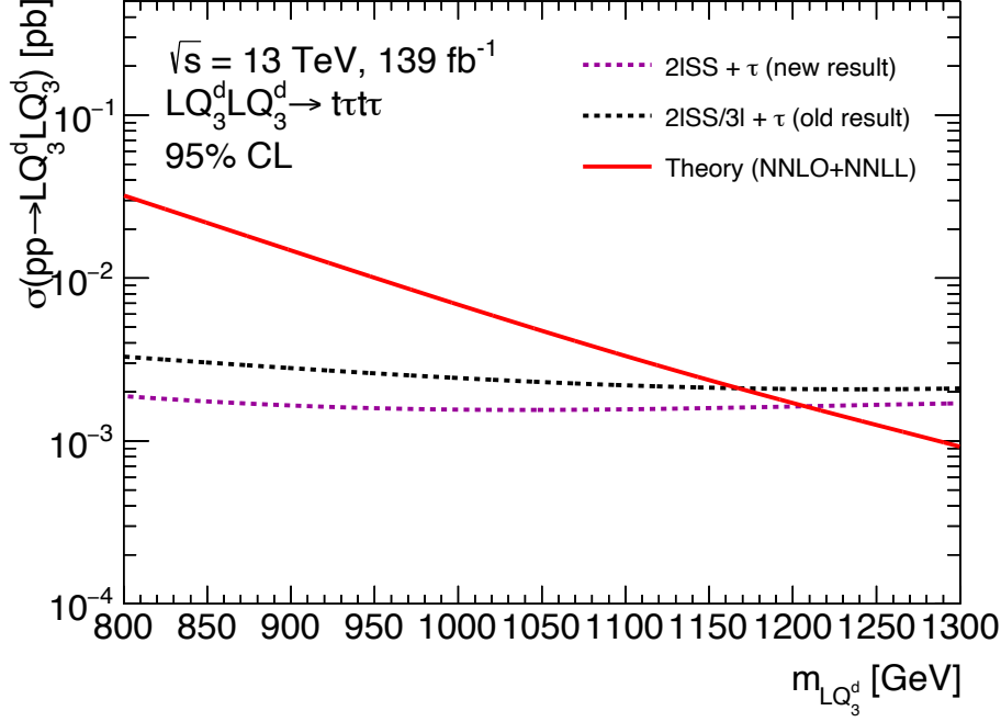
Figure 8.12: Comparison of two \sigma_e . Magenta: new result. Black: previous result [11] and [12] (Figure 75).
