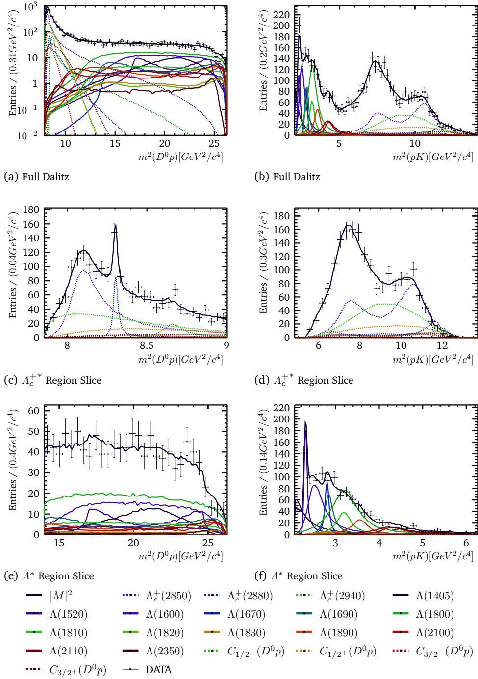
Fig. N.18.: Amplitude fit of all possible \Lambda_c^{+*} and \Lambda^* resonances to the full Dalitz plot. Shown as projection on m_{D^0 p}^2 (left) and on m_{p K}^2 (right). The partial components are shown as their amplitudes squared.
