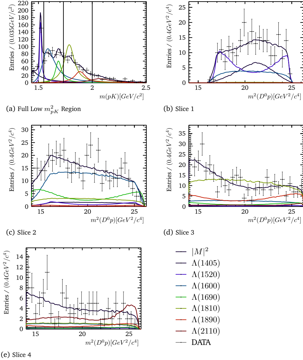
Fig. N.16.: Reduced amplitude fit to the low m_{pK}^2 region. Shown as projection on m_{pK} (a) and on m_{D^0 p}^2 in slices of m_{pK} (b-e). The vertical lines in (a) indicate the slices 1-4 from left to right. The partial amplitudes are shown as their amplitudes squared.
