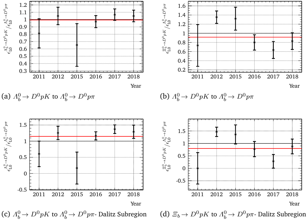
Fig. H.1.: L0 efficiency ratios in the D^0 \rightarrow K^- \pi^+ samples. The red line highlights the luminosity weighted mean ratio. - DATA
