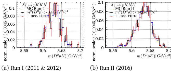
Fig. I.13.: Test of selecting only the \Lambda^* Dalitz subregion and additional acceptance correction for \Lambda_b^0 \rightarrow pK K K MC in m(D^0 p K)
