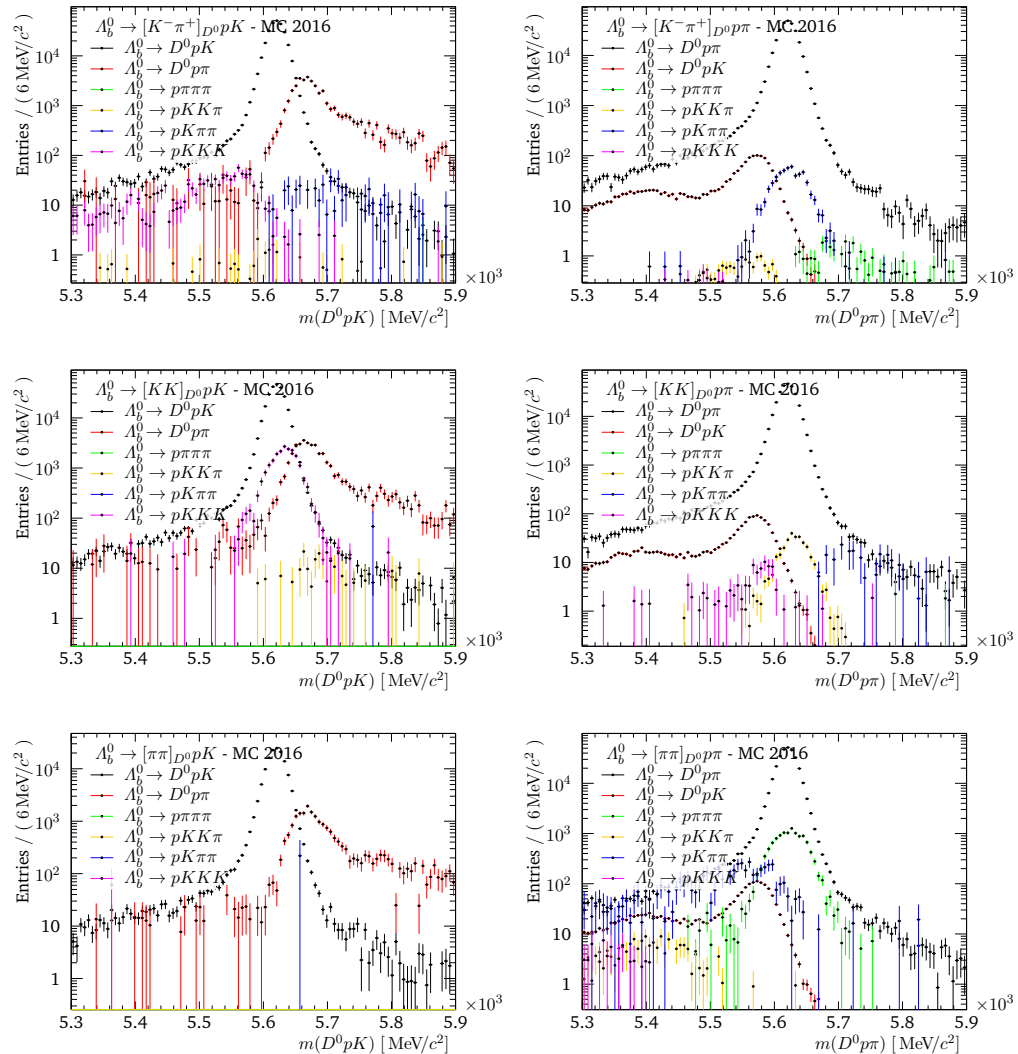
Fig. G.16.: Comparison of different charmless background contributions in m(D^0 ph) with all selections applied and re-normalised to match the A_b^0 \rightarrow D^0 ph reference signal MC. The background MC has been scaled according to their relative scaling factors in table 4.3 - MC 2016
