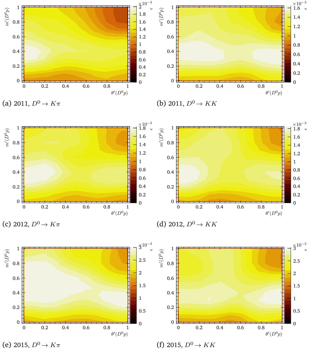
Fig. H.2.: Acceptance across the square Dalitz Plot for the \Lambda_b^0 \rightarrow D^0 p K signal. (1/2)
