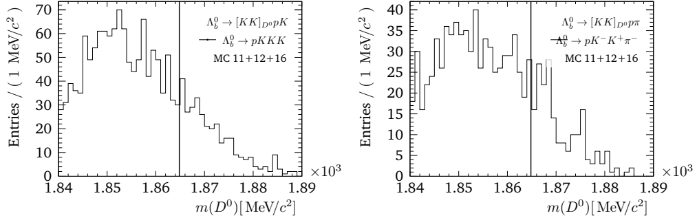
Fig. G.10.: m(D^0) for \Lambda_b^0 \rightarrow pK^-KK (left) in m([KK]_D^0 pK) and \Lambda_b^0 \rightarrow pKK\pi^- (right) in m([KK]_D^0 p\pi) . Both distributions show a shift from the nominal D^0 -mass (vertical line) due to the D^0 -mass constrain of the DTF.
