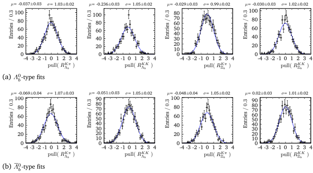
Fig. K.3.: Pull distributions of the measured values from pseudo experiments of the likelihood fits to m(D^0 ph) of the split datasets in the \Lambda^* resonance region ( m^2(D^0 p) > 14 \text{ GeV}^2/c^4 ).
