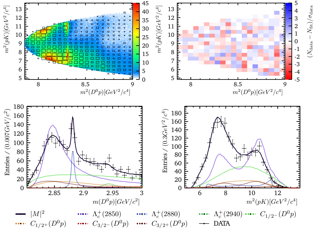
Fig. N.10.: Amplitude fit to the low m_{D^0 p}^2 region, shown in the Dalitz plot with a resolution of 200 \times 200 bins overlayed by DATA in a 20^2 bins box graph (top left) and their pull (top right). The projections on m_{D^0 p} (bottom left) and on m_{pK}^2 (bottom right) are shown. The partial amplitudes are shown as their amplitudes squared.
