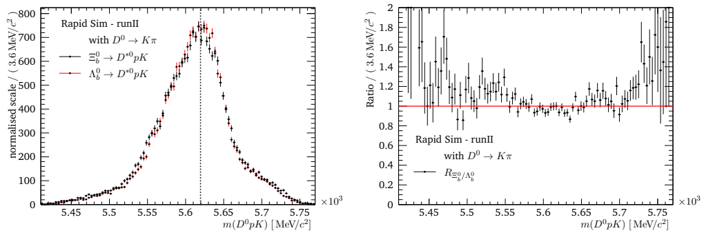
Fig. 4.16.: Distribution of m(D^0 p K) (left) for \Xi_b \rightarrow D^{*0} p K and \Lambda_b^0 \rightarrow D^{*0} p K shifted by |m_{\Xi_b} - m_{\Lambda_b^0}| = 172.5 \pm 0.4 [20]. The nominal \Lambda_b^0 mass is highlighted via a dashed line (left) and the ratio of the histograms is shown (right). - RapidSim Run II
