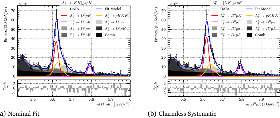
Fig. L.1.: Comparison between the nominal fit and the charmless systematic fit with a free shift value \Delta m_{\text{charmless}} . Both plots show the preliminary fit for the acceptance corrected full phase space.
