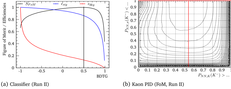
Fig. 4.12.: FoM and Efficiencies for the classifier and kaon PID selection. The chosen cuts values are shown as lines. (Run I in app. F.5)
