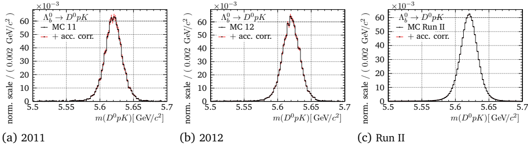
Fig. I.2.: Test of the acceptance correction for \Lambda_b^0 \rightarrow D^0 p K signal MC in m(D^0 p K) .
