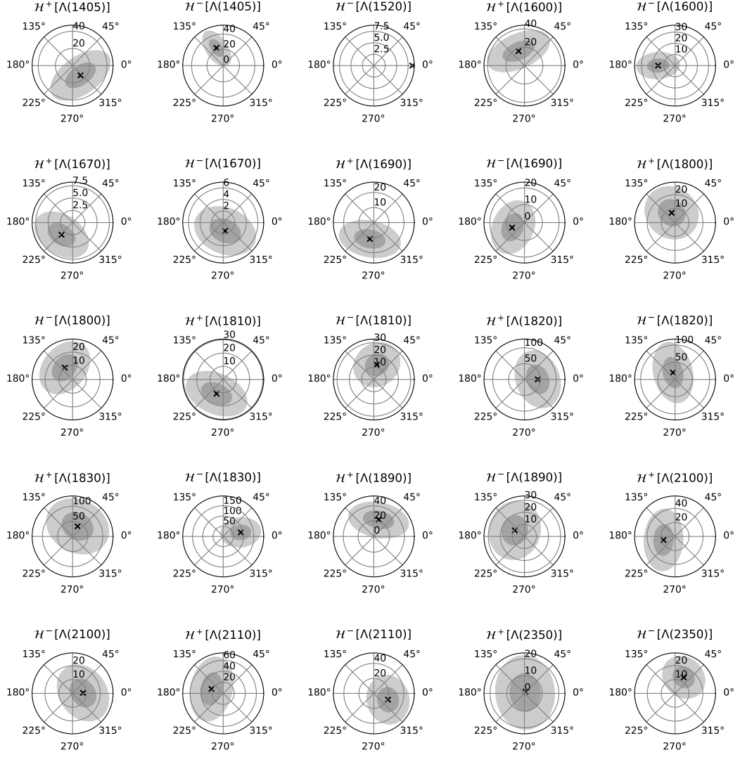
Fig. N.3.: Helicity couplings with their 1\sigma and 2\sigma covariance ellipse found in the fit to the low m_{pK}^2 region in appendix N.3.2.
