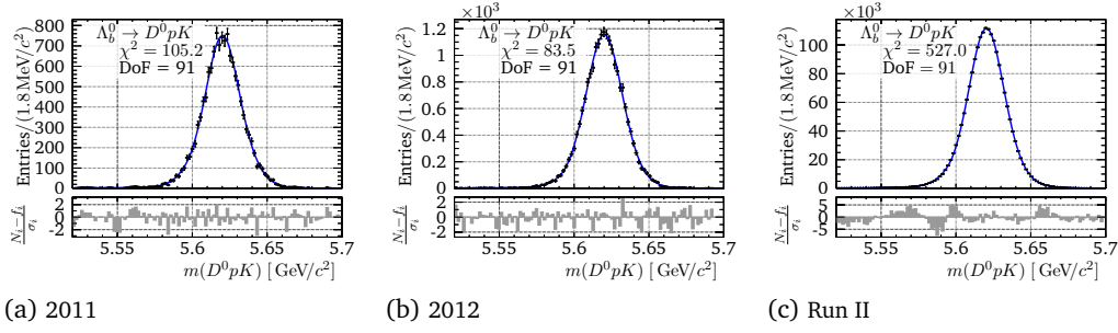
Fig. I.1.: Fit to \Lambda_b^0 \rightarrow D^0 p K signal MC in m(D^0 p K) .
