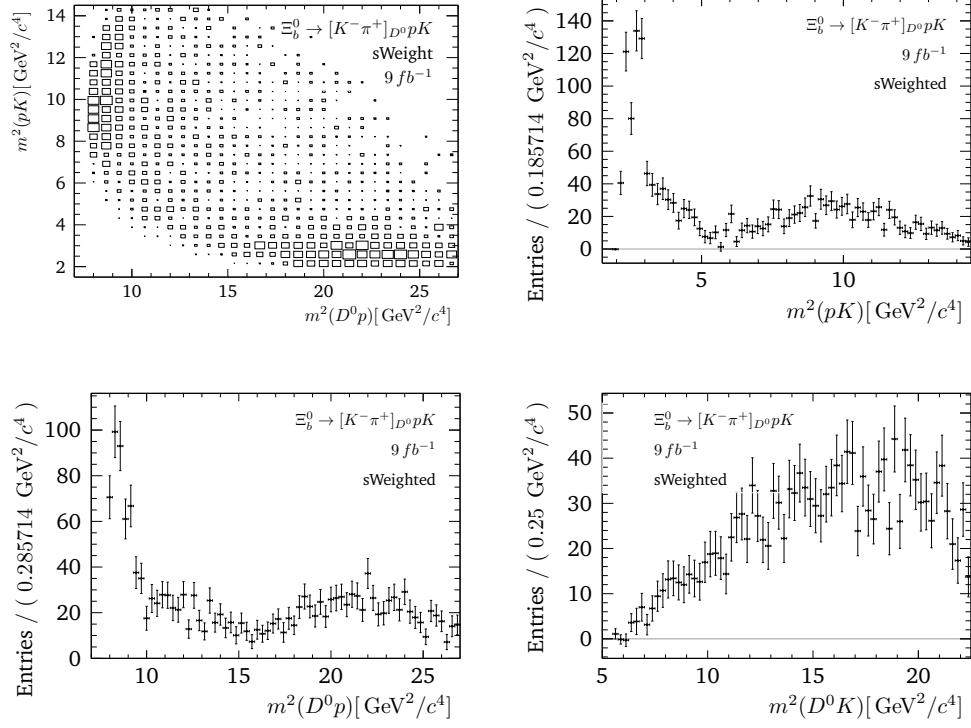
Fig. M.8.: sWeighted and acceptance corrected Dalitz plot of \Xi_b \rightarrow D^0 p K candidates from the D^0 \rightarrow K^- \pi^+ sample (a) and its projections (b-d).
