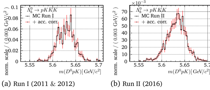
Fig. I.12.: Test of the acceptance correction for \Lambda_b^0 \rightarrow pK K K MC in m(D^0 p K)
