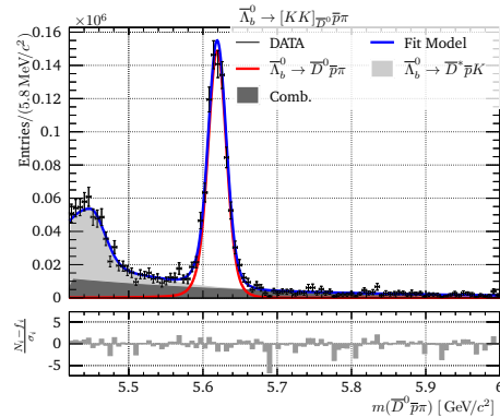
Fig. J.10.: Fits to m(D^0 p K) and m(D^0 p \pi) with acceptance weights and split for the D^0 modes and \Lambda_b^0 -types.
