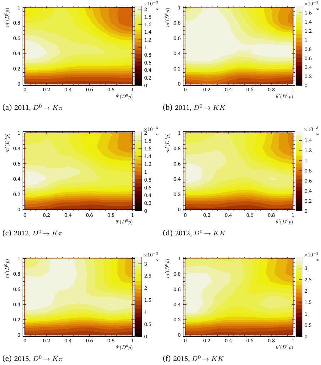
Fig. H.3.: Acceptance across the square Dalitz Plot for the \Lambda_b^0 \rightarrow D^0 p \pi signal. (1/2)
