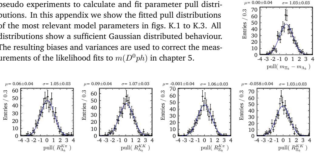
Fig. K.1.: Pull distributions of the measured values from pseudo experiments of the preliminary likelihood fit to m(D^0ph) .
