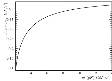
Fig. M.4.: Modified Flaté lineshape width for \Lambda(1405) within the kinematically allowed limits.
