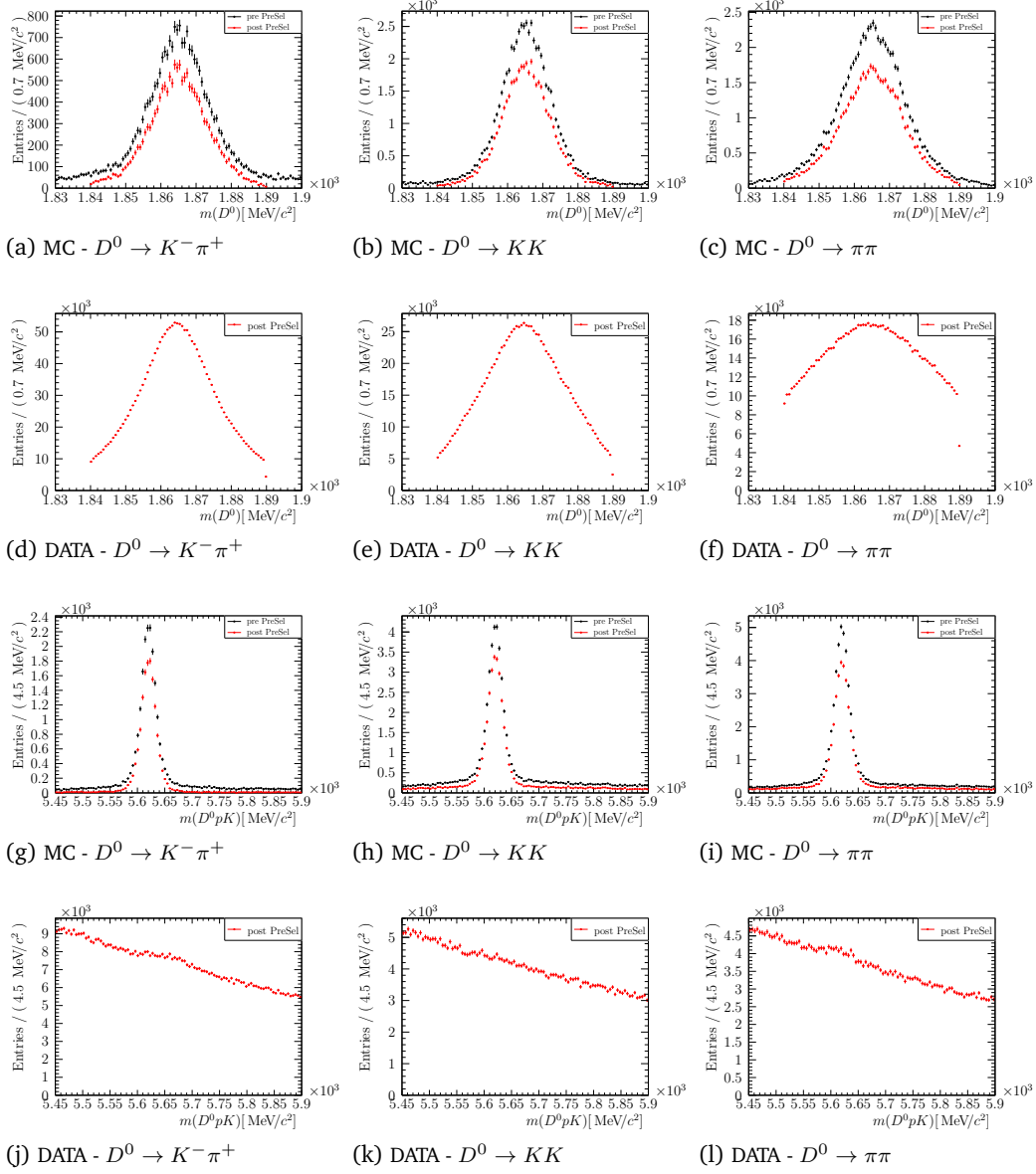
Fig. B.2.: Preselections on DATA and MC ( A_b^0 \rightarrow D^0 p K ) - 2012
