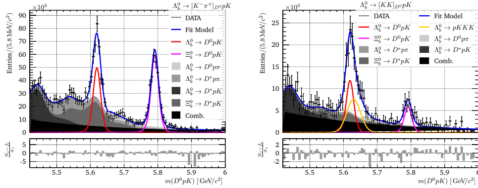
Fig. 5.4.: Fit to m(D^0 p K) and m(D^0 p \pi) with acceptance weights in the \Lambda^* Dalitz subregion ( m^2(D^0 p) > 14 \text{ GeV}^2/c^4 ). Only the m(D^0 p K) distributions of the preliminary fit are shown. All plots are in appendix J.4.
