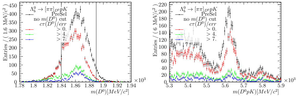
Fig. G.11.: D^0 (left) and \Lambda_b^0 (right) mass comparison for \Lambda_b^0 \rightarrow [\pi\pi]_D^0 pK candidates with strengthened cuts on c\tau/err . The charmless contribution (enhancement to lower D^0 masses) remains in the D^0 mass preselection window. - DATA
