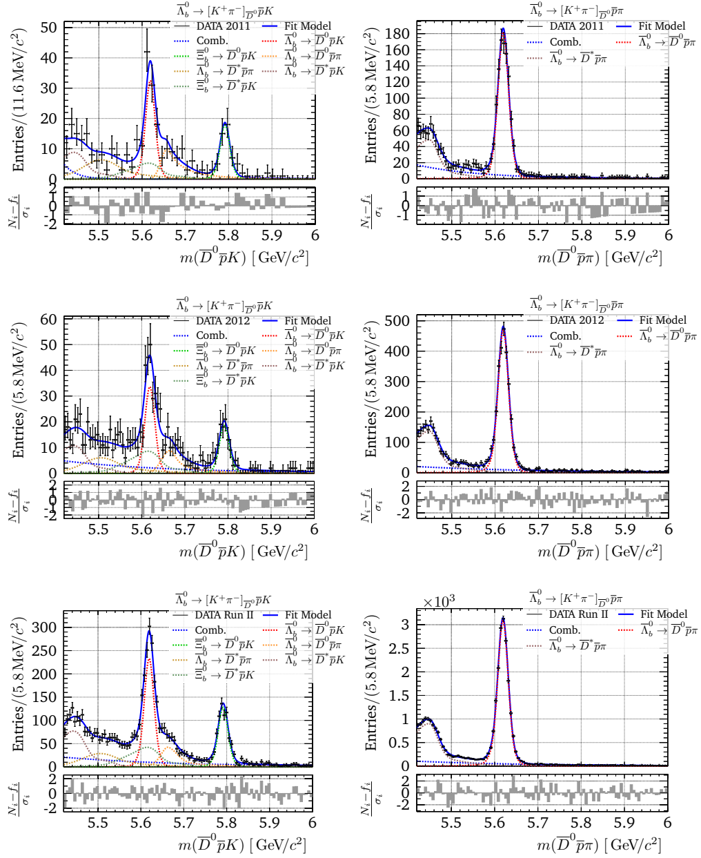
Fig. J.4.: \bar{\Lambda}_b^0 -type fit to m(D^0 p K) and m(D^0 p \pi) with D^0 \rightarrow K^- \pi^+ .
