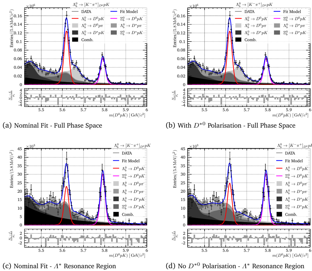
Fig. L.2.: Comparison between the nominal fit and the systematic. The nominal fit in the full phase space assumes no D^{*0} polarisation and the one in the \Lambda^* resonance region allows polarisation. All plots show the \Lambda_b^0 -type fit to the acceptance corrected D^0 \rightarrow K\pi DATA.
