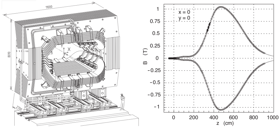
Fig. 3.4.: Scheme of dipole magnet design (left) and magnetic field in z -direction (right) [65].
