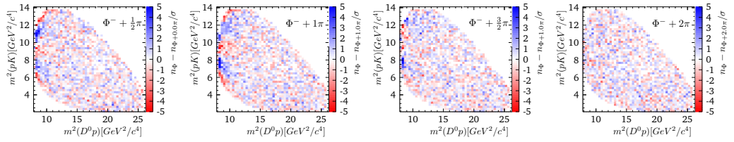
Fig. N.8.: Difference of |M|^2 in 50^2 bins for phase shifts only on \mathcal{H}^- of \Lambda_c^+(2880) .
