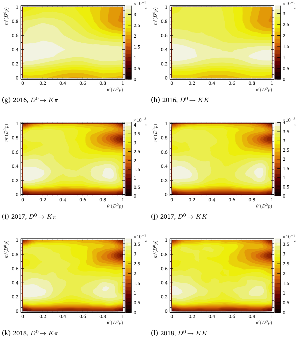
Fig. H.2.: Acceptance across the square Dalitz Plot for the \Lambda_b^0 \rightarrow D^0 p K signal. (2/2)
