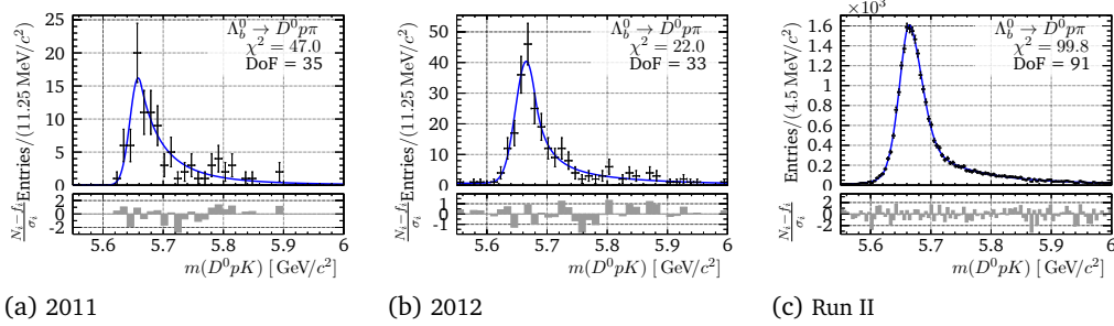
Fig. I.7.: Fit to \Lambda_b^0 \rightarrow D^0 p \pi mis-ID MC in m(D^0 p K)
