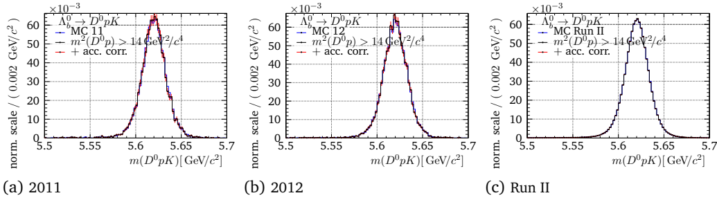
Fig. I.3.: Test of selecting only the \Lambda^* Dalitz subregion and additional acceptance correction for \Lambda_b^0 \rightarrow D^0 p K signal MC in m(D^0 p K) .
