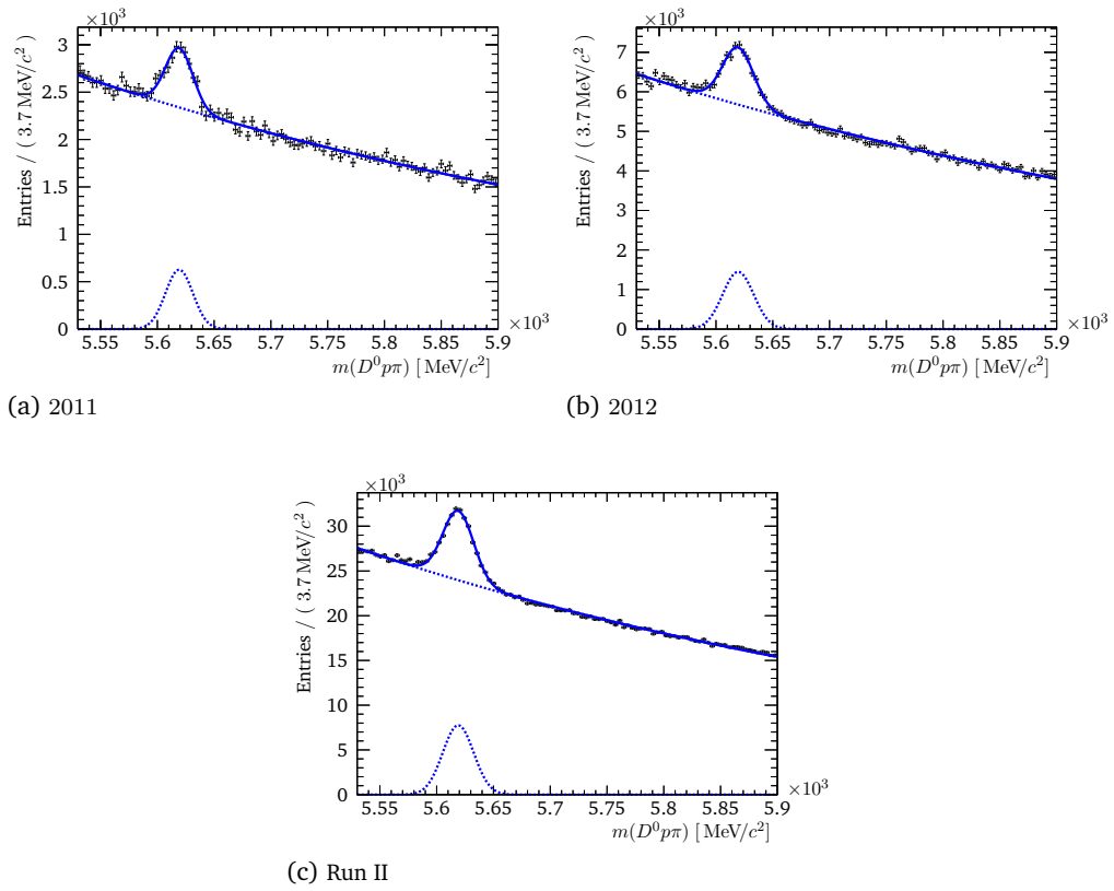
Fig. D.1.: Extended maximum likelihood fit to mass distribution of \Lambda_b^0 \rightarrow D^0 p \pi - DATA
