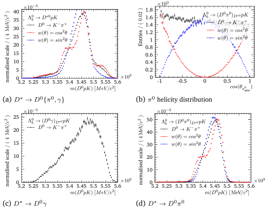
Fig. G.2.: Comparison of m(D^0 p K) distributions for (un)polarised D^{*0} of \Lambda_b^0 \rightarrow D^{*0} p K . They are shown for the channels D^{*0} \rightarrow D^0 \gamma (c), D^{*0} \rightarrow D^0 \pi^0 (d) and both (a). Polarisation is simulated by weighting in the \pi^0 helicity distribution (b). - MC 2018
