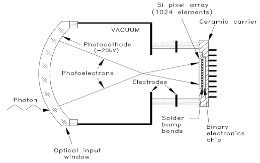
Fig. 3.10.: Schematic of a Hybrid-Photo-Detector [65].
