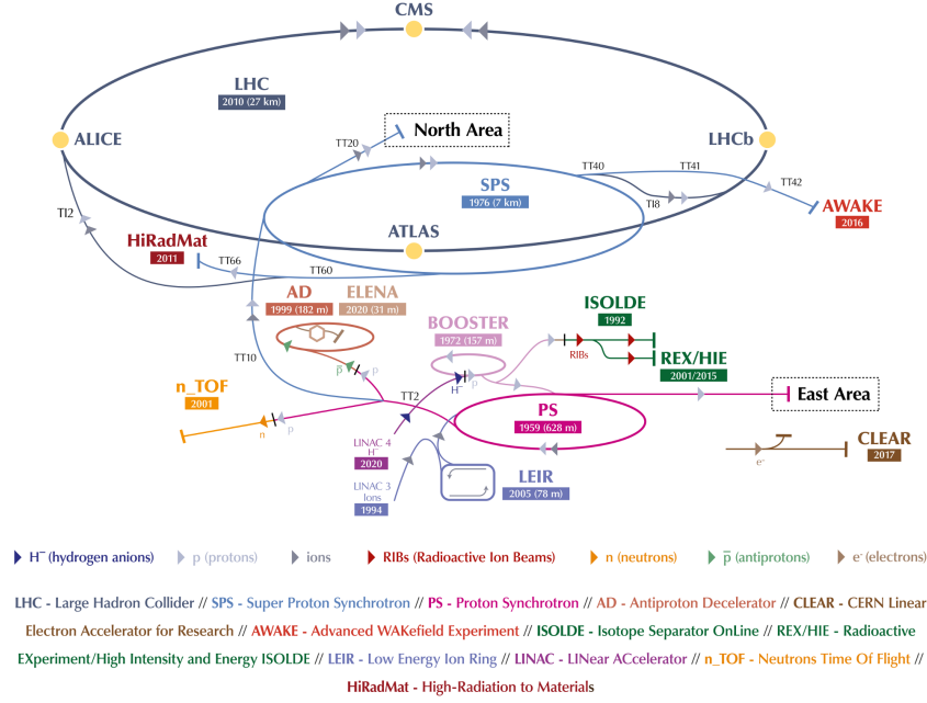
FIGURE 3.1: The CERN accelerator complex and a selection of key facilities and experiments. Figure adapted from [73].
