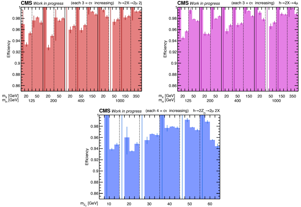
FIGURE 4.30: Efficiencies of the DCA < 15 \text{ cm} requirement in the H \rightarrow 2X \rightarrow 2\mu (top left), H \rightarrow 2X \rightarrow 4\mu (top right), and H \rightarrow 2Z_D \rightarrow 2\mu 2X (bottom) signal samples. The efficiency calculation is based on dimuons that pass the full analysis selection except for the DCA cut.
