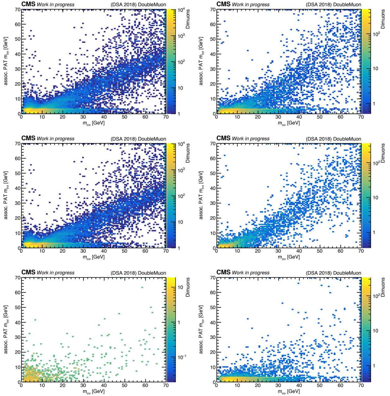
FIGURE 4.48: Comparisons of m_{\mu\mu}^{(DSA)} (horizontally) and m_{\mu\mu}^{(PAT)} (vertically) for DSA-DSA dimuons with both legs associated with PAT muons. The left column shows oppositely-charged dimuons, the right columns equally-charged dimuons. Top row: The full control sample, middle row: a subsample with matching DSA and PAT charges, bottom row: the complementary sample with at least one mismatch between the DSA and associated PAT muons.
