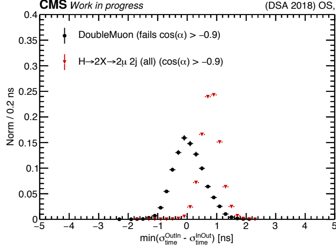
FIGURE 4.29: Normalized distributions of the minimum difference between the uncertainties in the two different time measurements, t_{\text{inside-out}} and t_{\text{outside-in}} in dimuons of the combined H \rightarrow 2X \rightarrow 2\mu signal samples (red) and a 2018 data sample that is enriched in cosmic-ray muons (black). Positive values of the shown variable designate the “inside-out” direction measurement.
