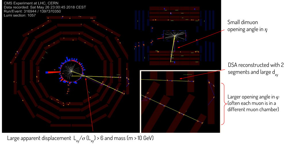
FIGURE 4.35: Event display of a typical low-mass, equal-charge dimuon with L_{xy}/\sigma_{L_{xy}} > 6 . The two distinct DSA muons forming the dimuon are produced in a pp collision and are close-by in the \eta direction (illustrated in the R - z plane in the top right view) but well separated in \phi (illustrated in the x - y plane in the left and bottom right views). The nearly horizontal muon is measured by only two muon segments and, due to its poor track quality, gives rise to a displaced common vertex.
