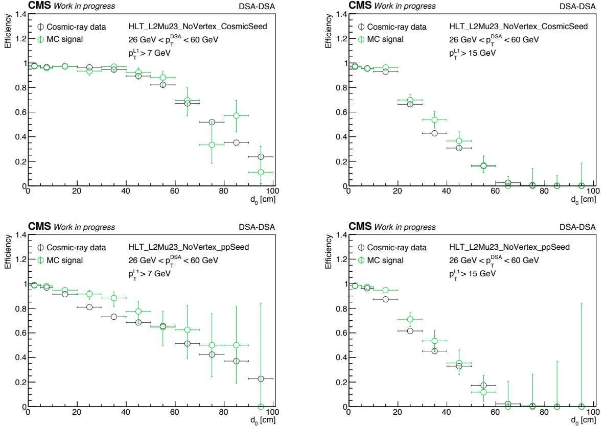
FIGURE 4.13: Efficiencies of the trigger HLT_L2Mu23_NoVertex_CosmicSeed (top) and HLT_L2Mu23_NoVertex_ppSeed (bottom) as functions of d_0 in cosmic-ray data (black) and signal simulation (green). The efficiency calculation is based on events filtered by the corresponding HLT_L2Mu10_NoVertex* path. The additional cuts p_T^{(L1)} > 7 \text{ GeV} (left) and p_T^{(L1)} > 15 \text{ GeV} (right) correspond to the p_T^{(L1)} thresholds used in the 2018 signal triggers.
