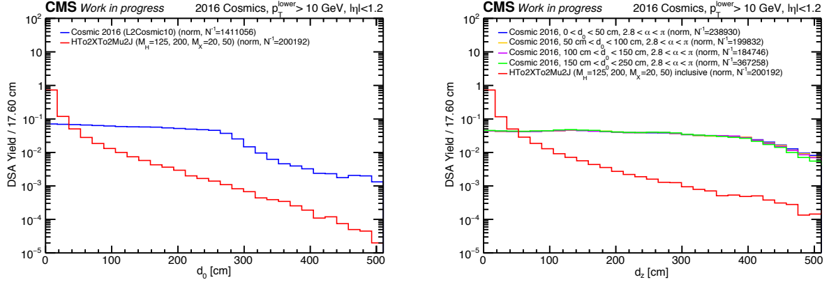
FIGURE 4.2: Distributions of d_0 (left) and d_z (right) for cosmic-ray data (blue) and simulated signal (red). The d_z distribution of cosmic-ray data are shown in several bins of d_0 .
