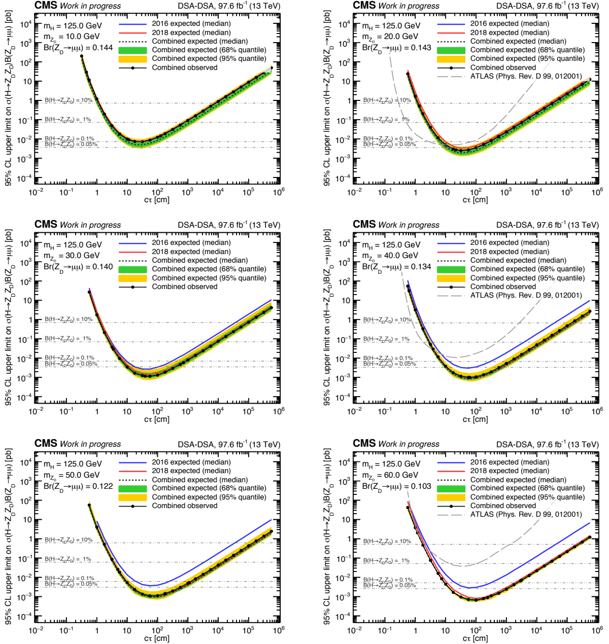
FIGURE 4.61: Expected and observed 95% CL upper limits on \sigma(h \rightarrow Z_D Z_D) \mathcal{B}(Z_D \rightarrow \mu\mu) as a function of c\tau_{Z_D} ranging from m(Z_D) = 10 GeV (top left) to m(Z_D) = 60 GeV (bottom right). The solid blue, solid red, and dashed black lines correspond to the limits obtained with 2016, 2018, and with the combined 2016–2018 data, respectively. The green and yellow bands respectively show the 68% and 95% quantiles for the expected combined limits. The gray horizontal lines correspond to the theoretical predictions for values of \mathcal{B}(h \rightarrow Z_D Z_D) indicated next to the lines. The scenarios for m(Z_D) of 20, 40, and 60 GeV are compared to the expected limits obtained in the ATLAS search for displaced dimuons with 2016 data (dashed gray curves) [64].
