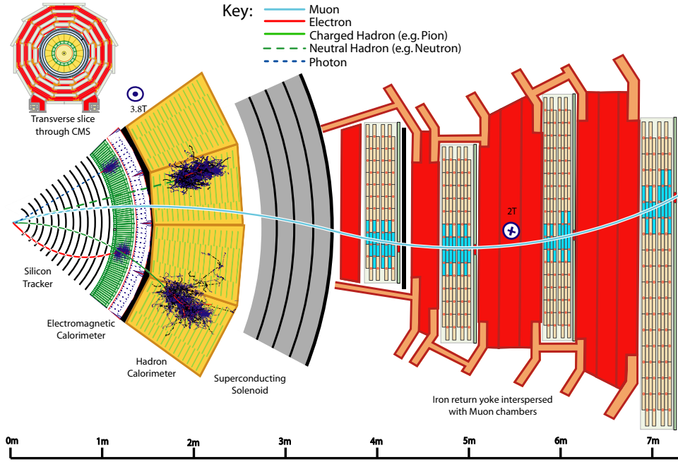
FIGURE 3.7: Interactions of different particle types with the subdetectors of CMS (schematic). The distinct hit/shower patterns across the detector sub-systems are combined in the Particle Flow (PF) algorithm to form hypotheses of stable particles. Figure taken from [90].
