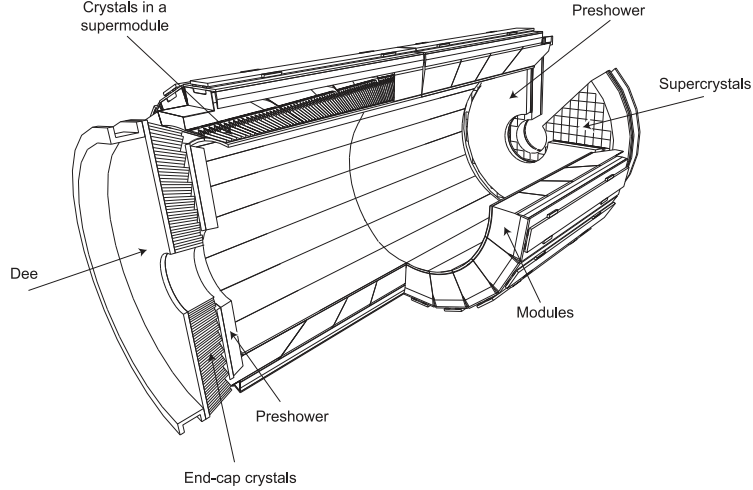
FIGURE 3.5: Schematic drawing of the CMS Electromagnetic Calorimeter (ECAL). Figure taken from [67].
