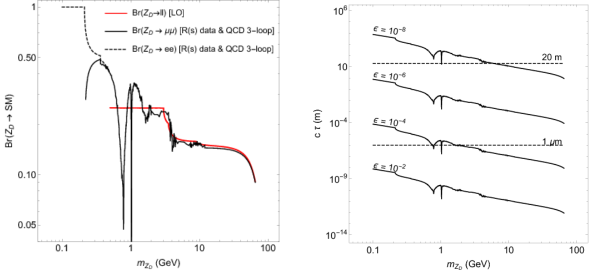
FIGURE 2.5: Left: Branching ratio of Z_D to lepton final-states ( \mu^+\mu^- , e^+e^- , l^+l^- ) as a function of m_{Z_D} . Right: Decay length of Z_D as a function of m_{Z_D} for different values of \varepsilon . Figures taken from [33].
