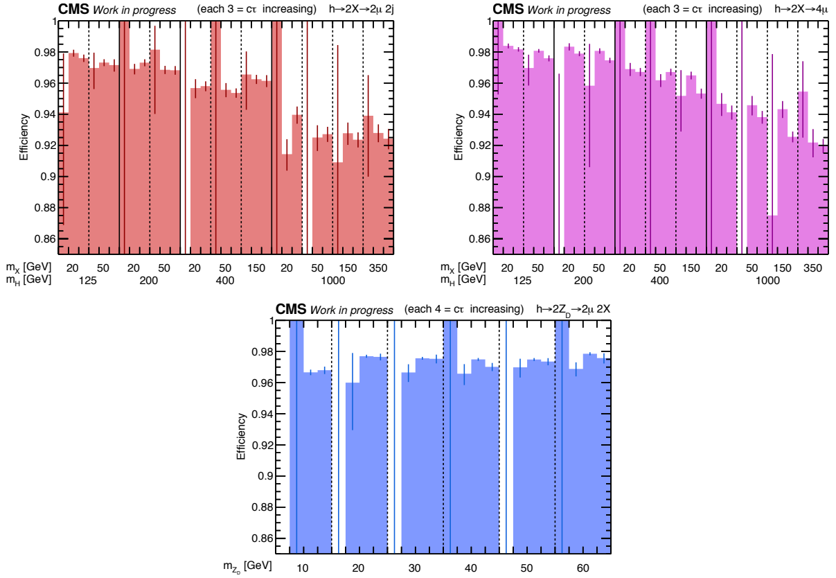
FIGURE 4.31: Efficiencies of the vertex \chi^2/\text{ndof} < 10 requirement in the H \rightarrow 2X \rightarrow 2\mu (top left), H \rightarrow 2X \rightarrow 4\mu (top right), and H \rightarrow 2Z_D \rightarrow 2\mu 2X (bottom) signal samples. The efficiency calculation is based on dimuons that pass the full analysis selection except for the DCA cut.
