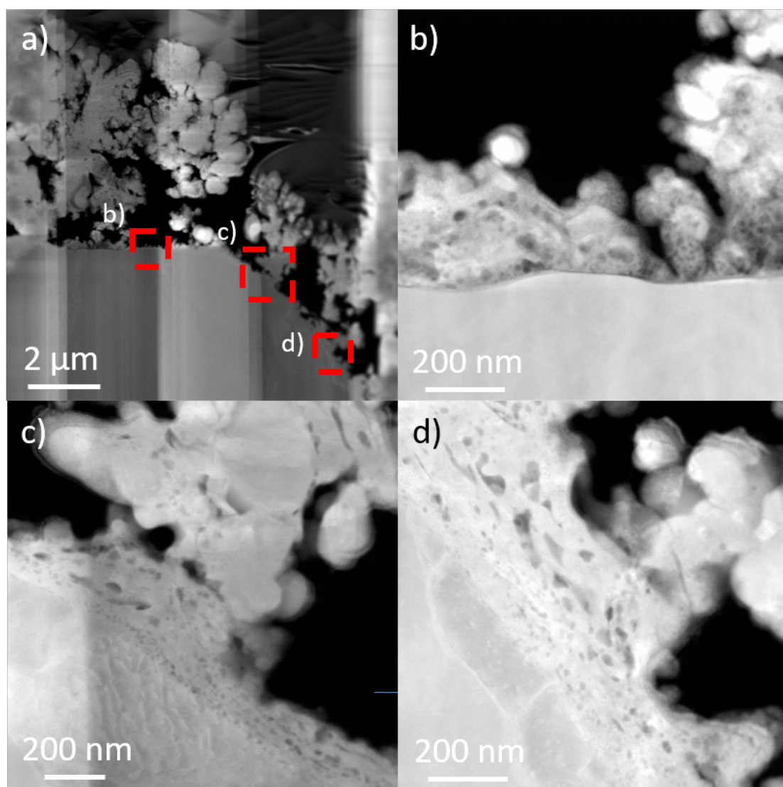
Figure C.11: STEM-HAADF image of a) general view . b) an area irradiated by 0.25 J.cm -2 . c) an area irradiated by 0.55 J.cm -2 . d) an area irradiated by 0.95 J.cm -2 .
