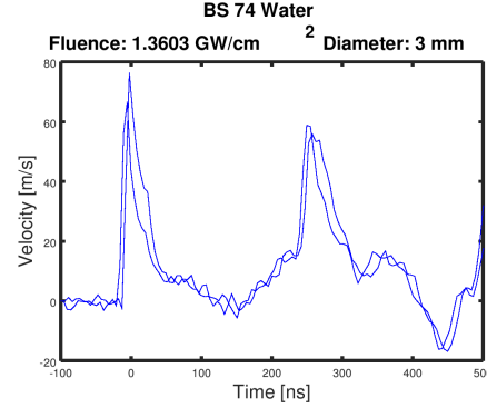
Figure D.55: Comparison of the VISAR measurements on a untreated BS74, with water as confinement media, at the power density of 1.36 \text{ GW.cm}^{-2} .
