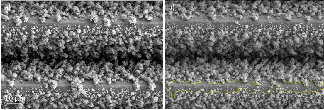
Figure 4.26: SEM top views of the treated surface a) in an area non affected by the laser shock, b) in an area affected by the laser shock (corresponding inertia force of 8.6 \text{ kN.mm}^{-3} ). The yellow line highlights an uncovered area on the groove top.
