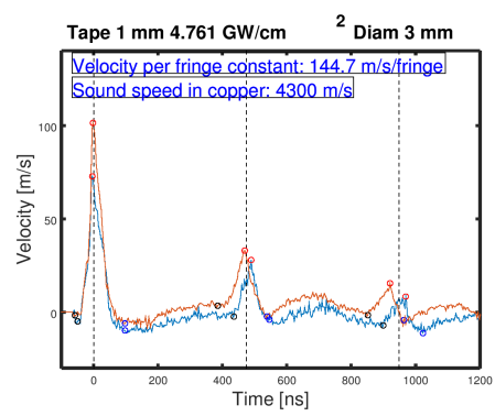
Figure D.23: Comparison of the VISAR measurements on a copper untreated sample of a thickness of 1 mm, with tape as confinement media, at the power density of 4.76 \text{ GW.cm}^{-2} .
