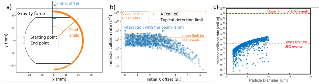
Figure 5.10: a) Sketch of the beam screen. The starting point (blue point) of the macroparticle, before interaction of the proton beam are located on top the flat part of the beam screen, the initial offset of the macroparticles is presented. The orange points are the end point location. Figure from Phillipe BELANGER, Triumf, private communication. b) Inelastic collision rate depending on the initial offset of the macroparticle. The offset is expressed as a function of \sigma_X , beam size characteristic calculated from the emittance \epsilon of the proton beam and the \beta of the magnet, \epsilon = \frac{\sigma^2}{\beta} . Figure from Phillipe BELANGER, Triumf, private communication. c) Inelastic collisions as a function of the particle diameter.
