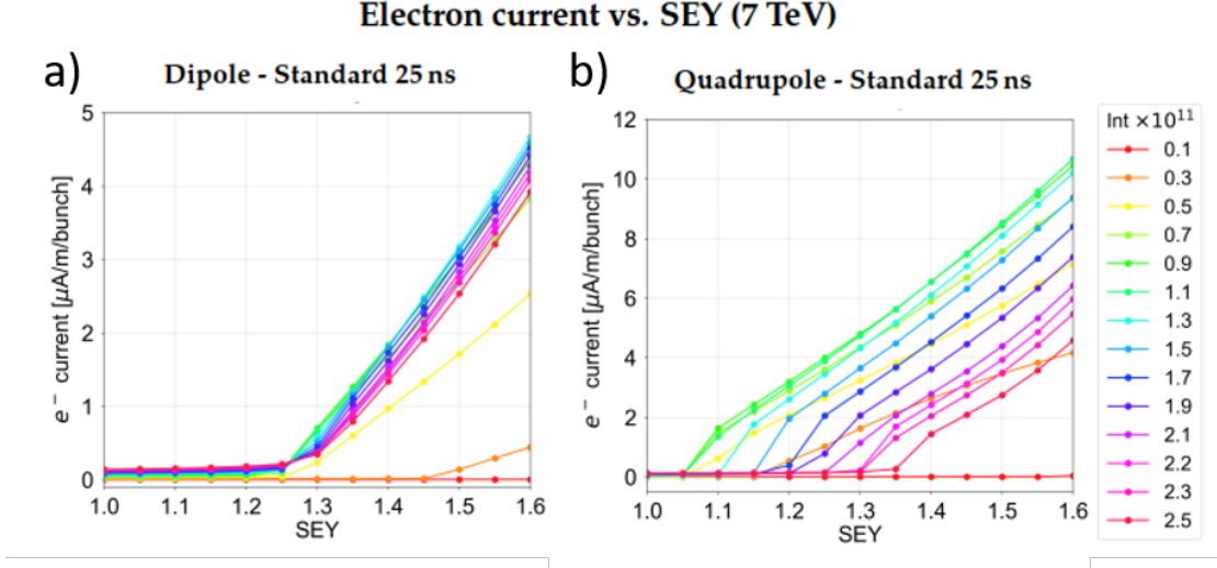
Figure 1.8: Evolution of electron-cloud current as a function of the maximum SEY of beam-pipe surface for LHC arc dipoles (a) and quadrupoles (b), for different bunch intensities. Simulations for 25 ns bunch spacing and 7 TeV beam energy [32].
