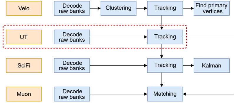
Figure 7.1: Complete High Level Trigger 1 sequence of algorithms at LHCb.
