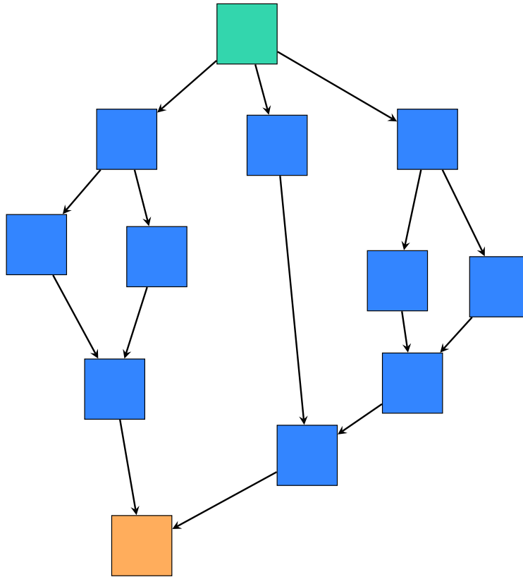
Figure 5.4: Work-span model representation
