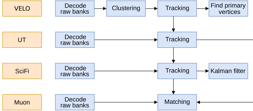
Figure 3.2: Algorithms run in HLT1
