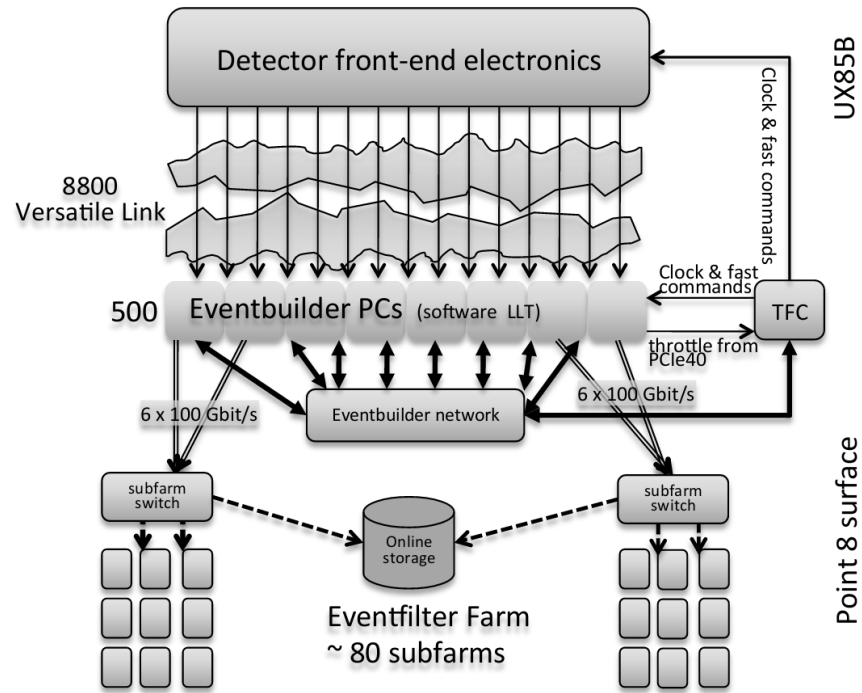
Figure 2.7: Layout of LHCb DAQ. Image from [42]
