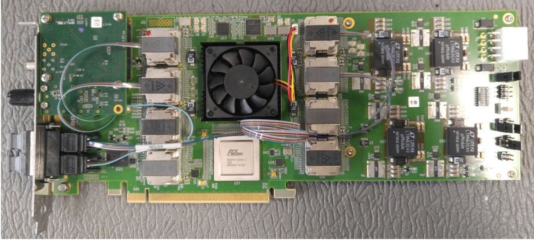
Figure 2.10.: An image of the FLX-712 custom FELIX hardware. Half of the miniPOD fibre optic transceivers are used, corresponding to the 24 of the maximum 48 available links. On the front panel, one MTP24 connector per FELIX device is exposed to the user.
