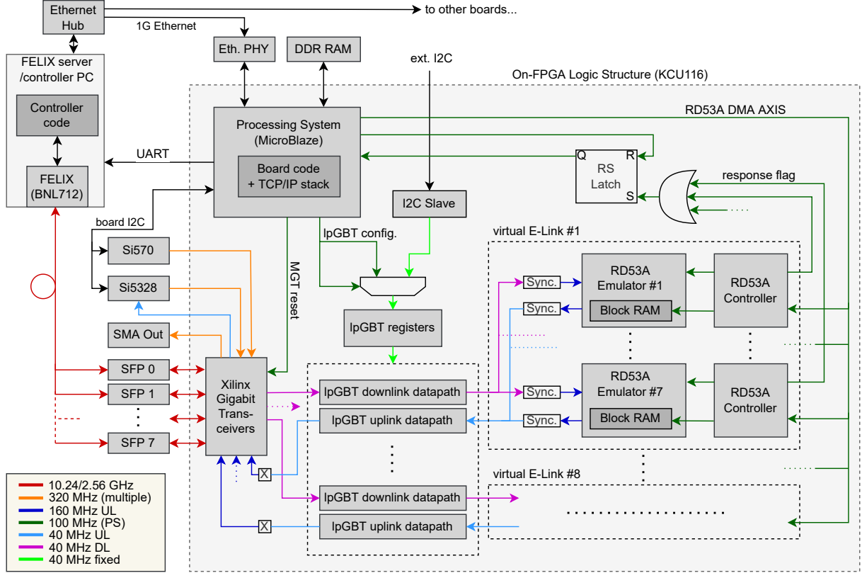
Figure 3.6.: The top-level stress test hardware design and its connections to the FELIX server. The detailed view of the RD53A emulator is already given in Fig. 3.4, and the one for the processing system in Fig. 3.5. The different clock domains are colour-coded. In contrast to the rest, the connections to the SMA Out, Si5328 and Si570 are clock, not data signals.
