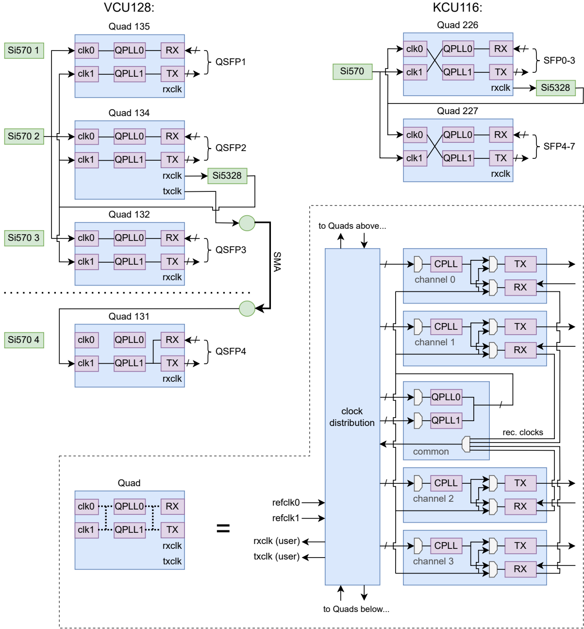
Figure 3.3.: A diagram showing how the MGTs are set up to achieve the required clock recovery scheme for the lpGBT emulator. To save space in the connectivity diagrams, the details of the basic building block, the MGT Quad, are shifted to the legend on the bottom. The MGT Quad diagram is based on [29].
