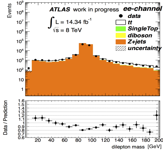
Figure 4.9: The dilepton invariant mass distribution for the ee -channel before E_T^{miss} cut and before the Z p_T reweighting. All simulated samples are normalised to an integrated luminosity of 14.34 \text{ fb}^{-1} .
