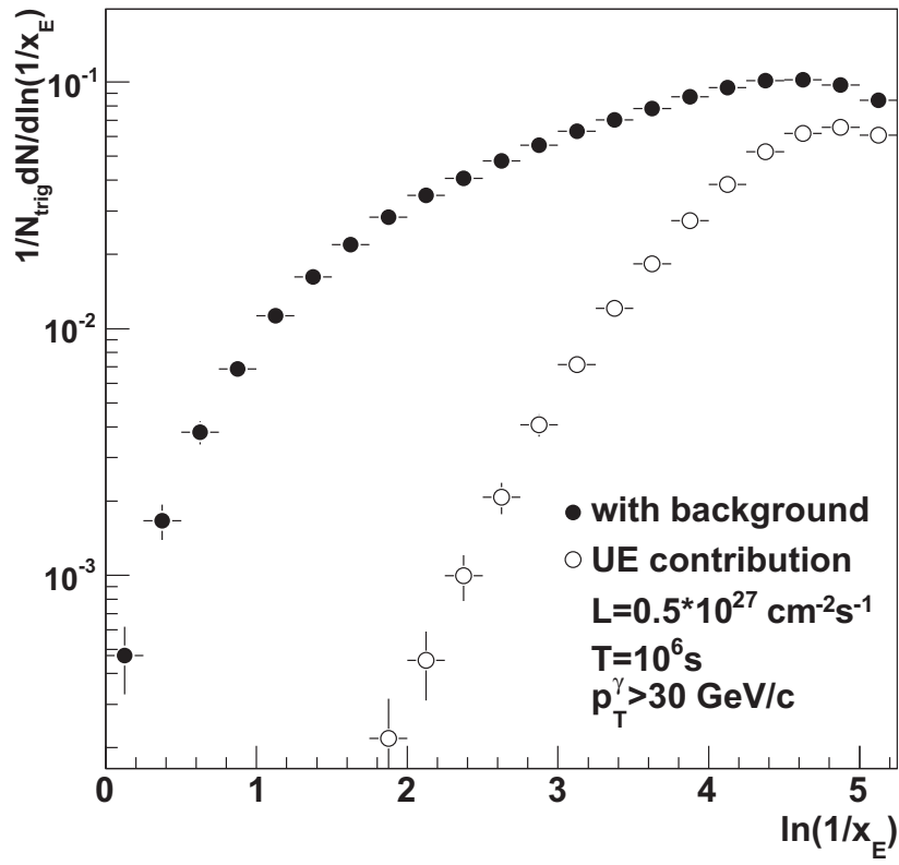
Figure 5.9: Photon-charged hadron correlation spectrum and the contribution from underlying event using photons identified by EMCAL in pp collisions at \sqrt{s} = 5.5 TeV [111].
