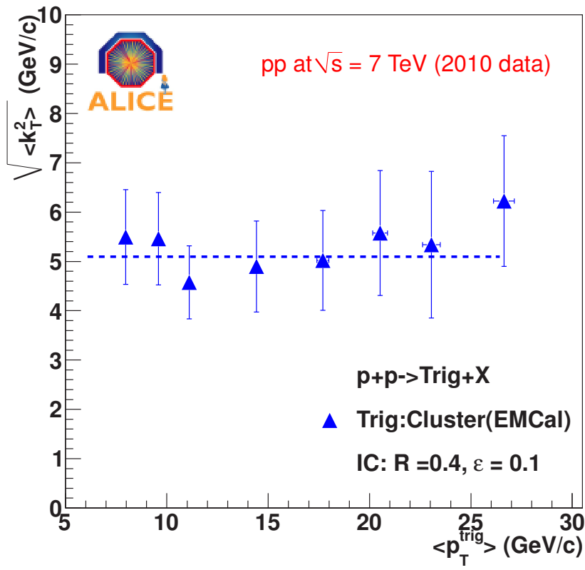
Figure 6.29: \sqrt{\langle k_T^2 \rangle} values evaluated from Eq. 6.6 by obtaining the \sqrt{\langle p_{out}^2 \rangle} values from the fits for isolated cluster triggers from EMCal with p_T^{trig} > 5 GeV/c and p_T^{h^\pm} > 1 GeV/c in pp collisions at \sqrt{s} = 7 TeV.
