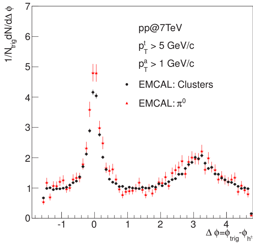
Figure 6.20: Relative azimuthal angle distribution \Delta\phi = \phi_{\text{trig}} - \phi_{h^\pm} for inclusive cluster triggers and \pi^0 triggers in EMCAL with p_T^{\text{trig}} > 5 \text{ GeV/c} and p_T^{h^\pm} > 1 \text{ GeV/c} in pp collisions at \sqrt{s} = 7 \text{ TeV} .
