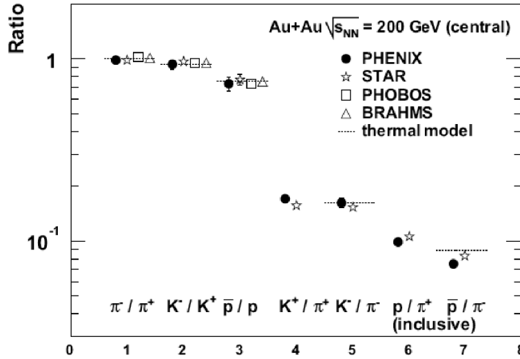
Figure 2.4: Particle ratios [25] in central collisions at \sqrt{s_{NN}} = 200 GeV at mid-rapidity with thermal model prediction [26] compared with PHENIX, PHOBOS, BRAHMS, and STAR.
