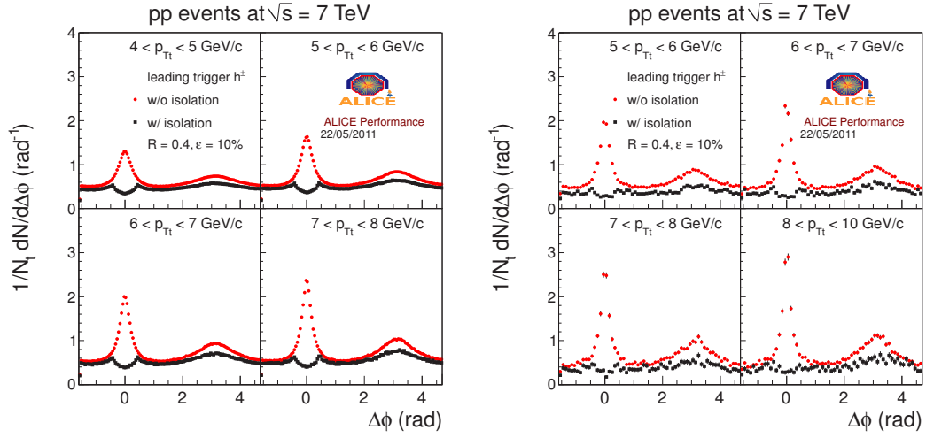
Figure 6.22: Relative azimuthal angle distribution \Delta\phi = \phi_{trig} - \phi_{h\pm} for inclusive charged and cluster triggers with different p_T bins and p_T^{h\pm} > 1 GeV/c in pp collisions at \sqrt{s} = 7 TeV before and after isolation cut (IC) selection: R = 0.4 , \varepsilon = 0.1 .
