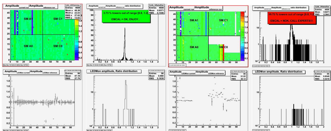
Figure 7.8: the AMORE canvas for EMCAL at P2 DQM station during the data taking from different running period with good data quality (left) and problemable data (right).
