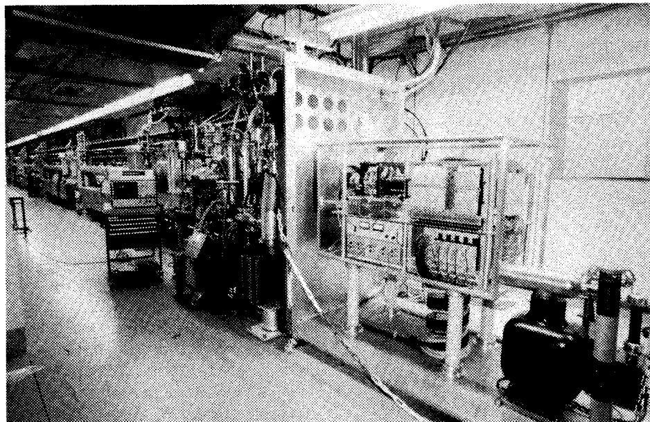
Foreground – The electron gun, bunching system and beam matching section feeding (background) the LEP Injector Linac (LIL)
