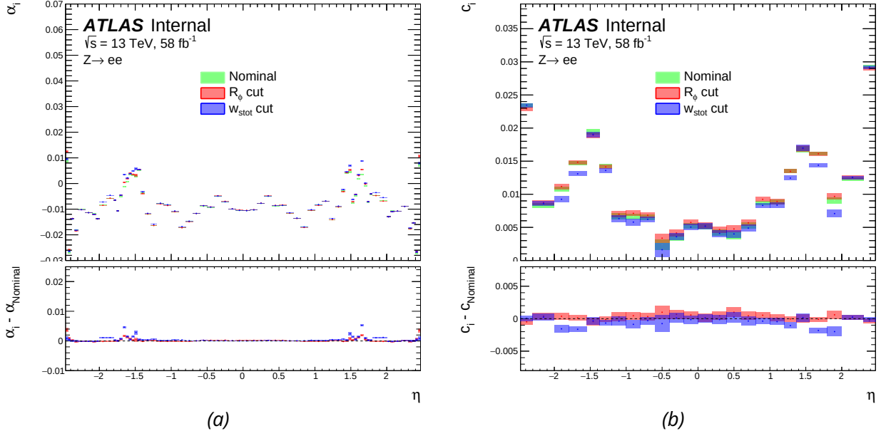
Figure 5.26: Scale factor (a) and constant term (b) obtained with 2018 data using nominal selection, and additional cut on shower shape variables R_\phi and w_{\text{stot}} .
