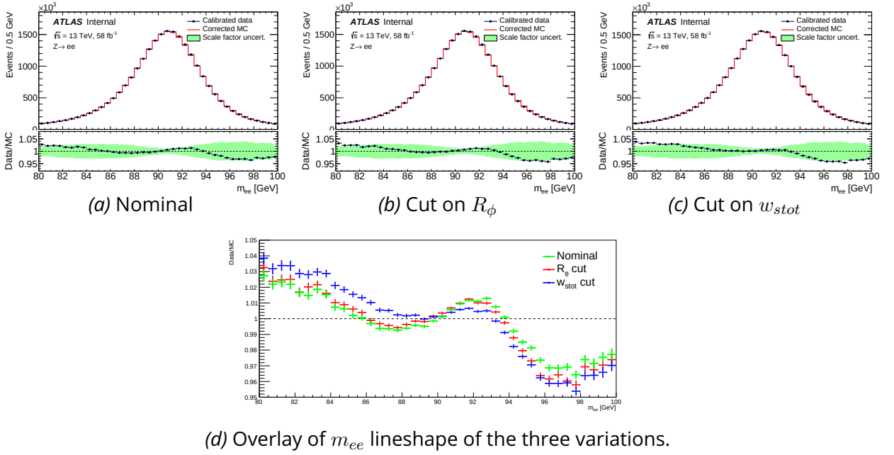
Figure 5.27: Calibrated mass of data 2018 and MC with the nominal selection, and additional cut on shower shape variables R_\phi and w_{\text{stot}} . The mass lineshape is overlapped in the bottom plot. The previous Rel. 21 calibrations are applied.
