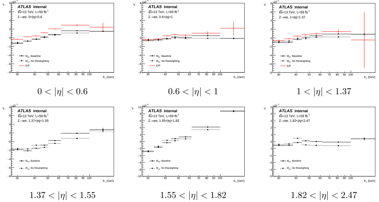
Figure 5.33: Measurement of linearity of LAr calorimeter with Z \rightarrow ee events with and without applying the Z boson p_T reweighting. E/p results are only shown in the barrel, due to its degradation on precision at high \eta . Baseline is the one with reweighted Z momentum.
