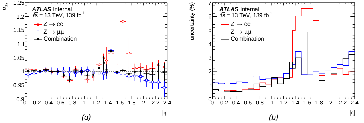
Figure 5.4: Combined E1/E2 scale factors (a) and uncertainties (b) for electron, muon and electron+muon channels[104].
