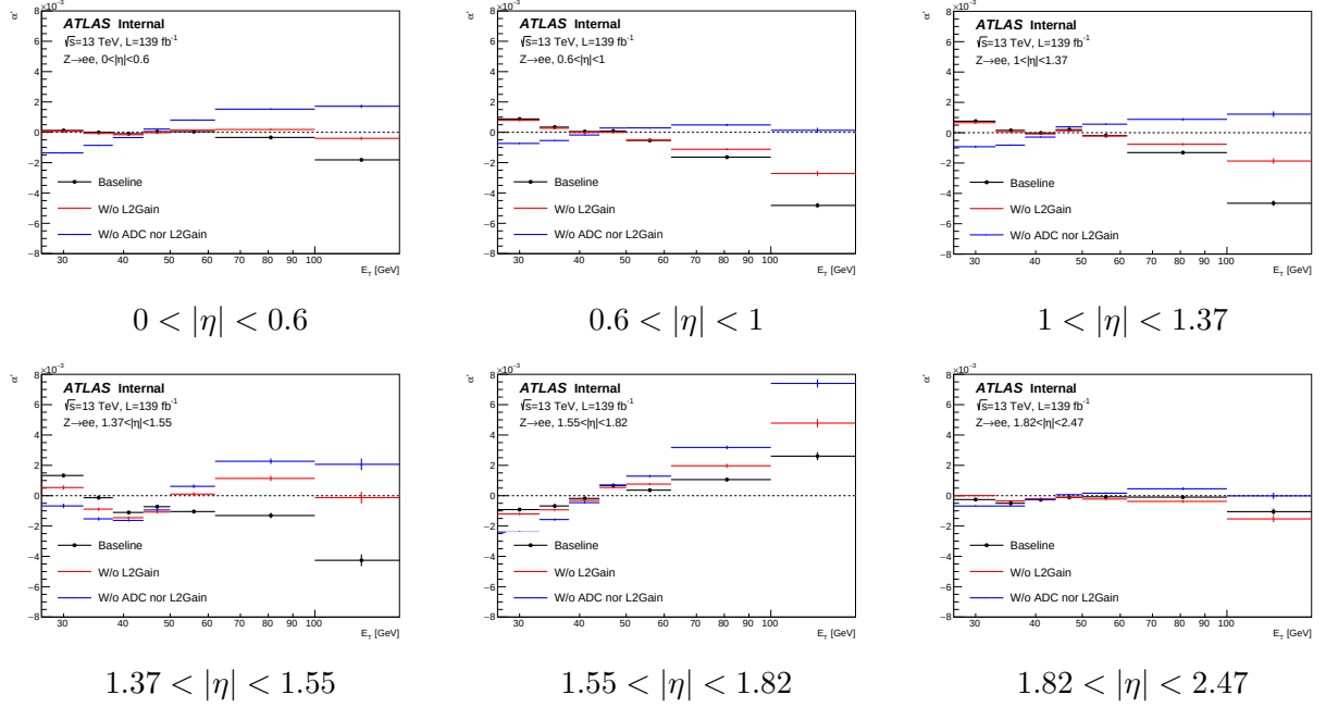
Figure 5.34: Influence of the ADC and L2Gain non-linearity corrections on the measurement of LAr calorimeter linearity with Z \rightarrow ee events. The baseline corresponds to the case with all the uniformity corrections applied. The influence of removing L2Gain is shown by the red curve, and the removal of the summed contribution from both ADC and L2Gain is shown in blue.
