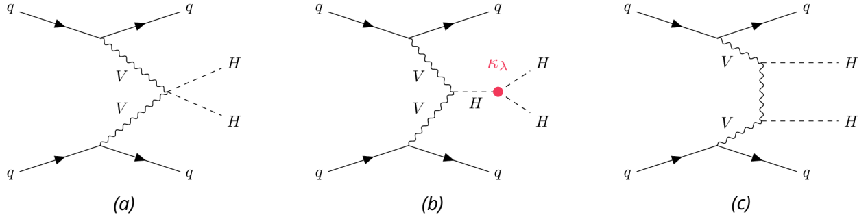
Figure 4.2: Feynman diagrams for the vector boson fusion production processes: (a) VVHH vertex, (b) trilinear coupling, and (c) VVH vertex [57].
