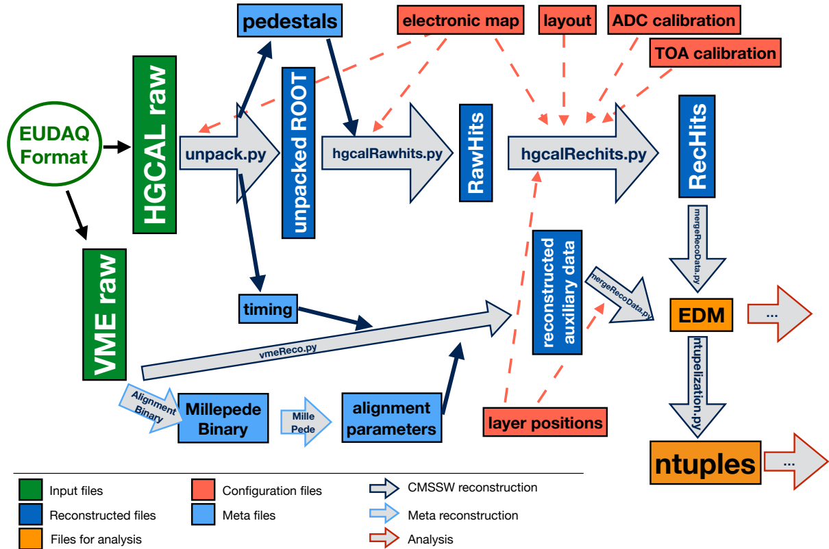
Figure 7.1: Sequence of steps and their dependencies for the reconstruction of the HGCAL prototype's raw data into calorimeter hits ( RecHits ). This data is merged with likewise reconstructed information from beam characterising detectors. Here, the case for the delay wire chambers is illustrated. Reconstructed data are stored in the EDM file format for analysis with CMSSW, or as ntuples for analysis with ROOT. This workflow solution is similarly applied for the DATURA beam telescope data whose reconstruction also proceeds in numerous, interdependent steps.
