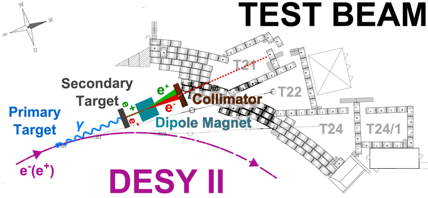
Figure 6.7: Illustration of the test beam generation and the facilities at the DESY II ring accelerator. Figure taken from Ref. [146].
