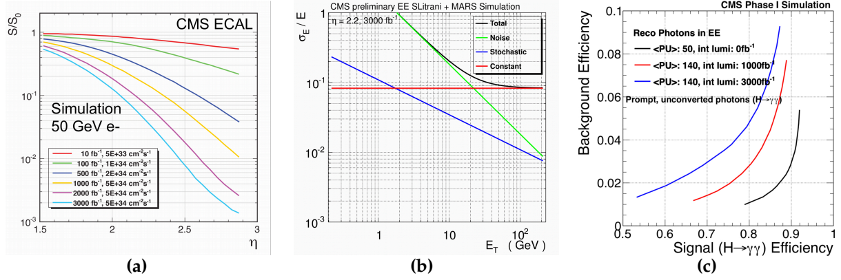
Figure 4.3: (a) Expectation of the relative light output S/S_0 of the ECAL crystals for electron showers of 50 GeV as a function of the pseudorapidity \eta for various ageing conditions, corresponding to different integrated luminosities. (b) The energy resolution including ageing effects at |\eta| = 2.2 after 3000 fb ^{-1} vs. the transverse energy E_T . (c) Selection efficiency for photons from the Higgs boson decay to two photons vs. the background efficiency estimated with the jet in \gamma +jet events for the ECAL Endcap for three MC samples which simulate: unaged detector at the end of Phase-I pile-up conditions, conditions early in HL-LHC operation, end of Phase-II conditions. Figures and their captions are taken from Ref. [105].
