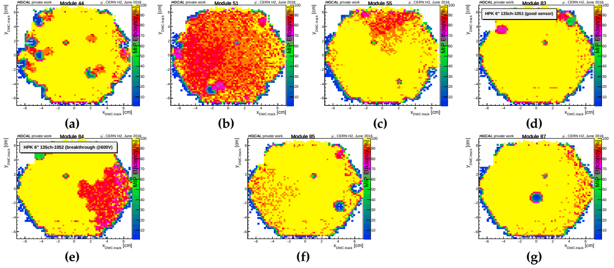
Figure 8.13: MIP detection efficiency maps for 7 of the 28 modules tested within the JUN programme that show a higher degree of inefficiencies compared to the others. The probability to detect a MIP-like hit is colour-coded and is shown in dependency on the impact position inferred from delay wire chamber measurements. Darker colours depict areas with MIP efficiency below 100 %.
