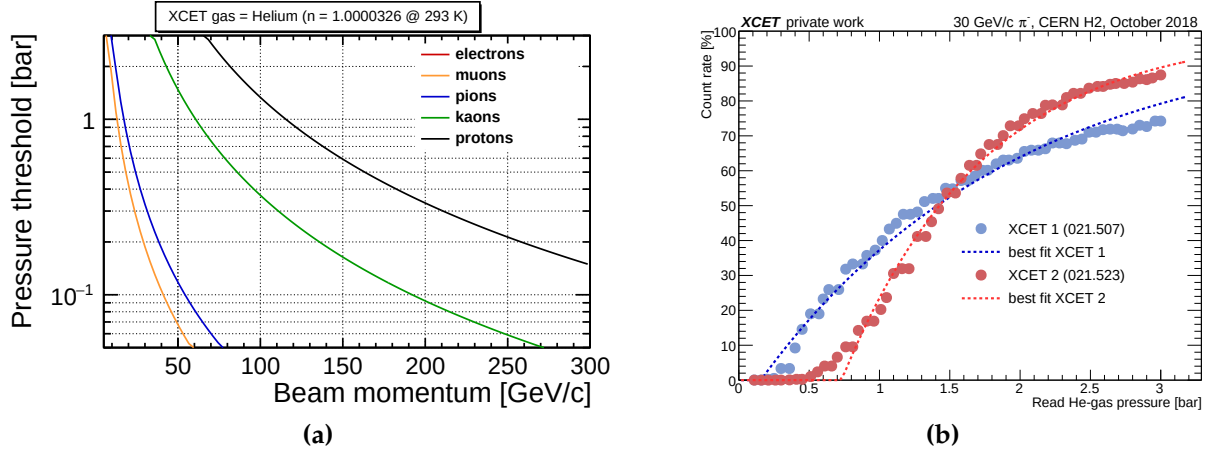
Figure B.1: (a) Theoretical pressure threshold for Helium ( n_0 = 1.0000326 ) for different beam particles and as a function of the beam momentum. (b) Measured count rate of the two XCETs operated during the HGCAL beam test at the H2 beam line at CERN in October 2018 for 30 GeV/c charged pions as a function of the Helium gas pressure. The count rate corresponds to the XCET's detection efficiency as long as particle contamination in the beam can be neglected. It is found that neither of the two curves are described accurately by the theoretically motivated parameterisation in Equation B.13 (best fit).
