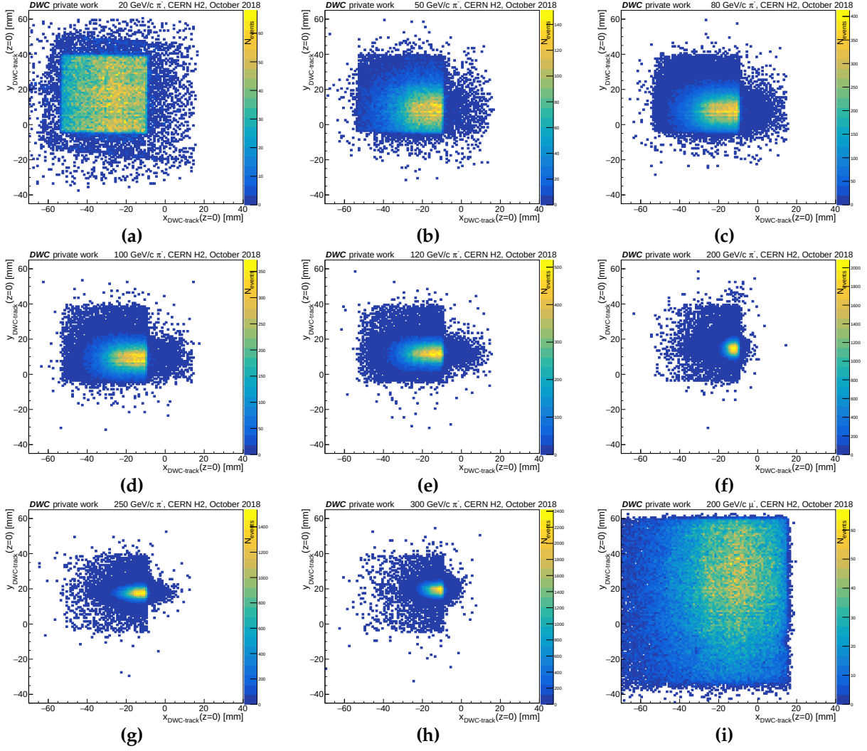
Figure E.2: Transverse beam profiles of incident charged pions and muons measured with the delay wire chamber tracking during the October 2018 HGCAL beam test at the H2 beam line at CERN.
