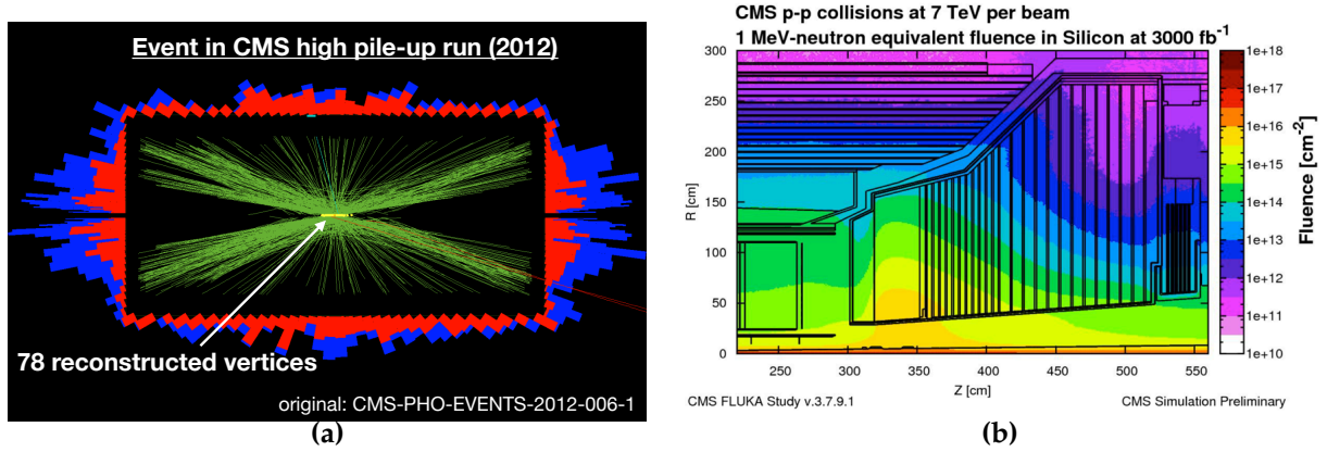
Figure 4.2: (a) Event display of a collision with 78 proton-proton collisions in the same bunch crossing (pile-up) recorded with the CMS detector in 2012. Figure taken and modified from Ref. [107]. (b) Expected fluences in the calorimeter endcap at the end of the HL-LHC's operational lifetime. Figure taken from Ref. [5].
