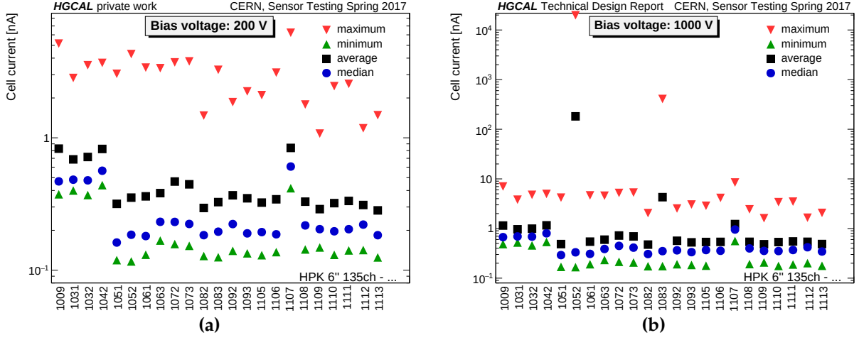
Figure 8.2: Summary of the temperature corrected leakage currents (a) at a bias voltage of 200 V and (b) at 1000 V for all characterised silicon prototype sensors in the IV dataset. The summary includes the leakage currents from cells with full hexagonal geometries only.
