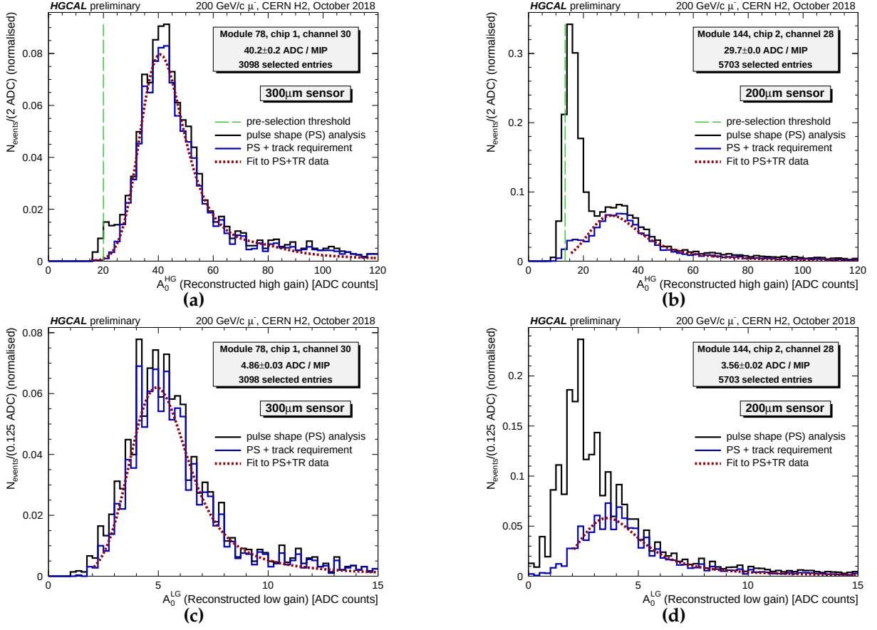
Figure 9.6: Spectra of reconstructed MIP-induced signal amplitudes both (a, b) in high and (c, d) in low gain for two example readout channels due to incident 200 GeV/c muons. Distributions of MIP-selected cells are normalised to unity integral. The inclusive spectra where no selection is applied are scaled likewise. Module 144 consists of a sensor that has a nominal depletion thickness of 200 \mu\text{m} resulting in a lower response compared to the 300 \mu\text{m} sensors, such as in module 78.
