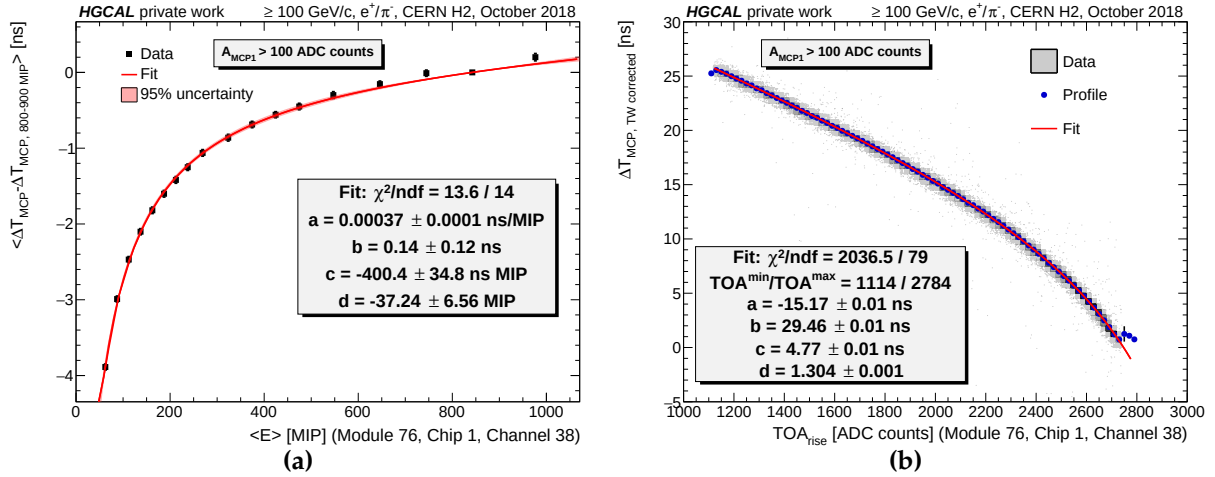
Figure 9.20: (a) Step 3: Quantification of the timewalk correction. The fitted parameters are defined in Equation 7.13. (b) Step 4: Relation between the TOA and the timewalk-corrected time. The fitted parameters are defined in Equation 7.12.
