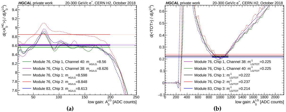
Figure 9.14: (a) Illustration of the spline method applied for the intercalibration of the high and low gain, (b) the low gain and TOT , respectively. These explanatory graphics are made with the O1E dataset, whereas all available data from a given setup were used in the actual calibration. The indicated bands symbolise the 68% uncertainty which is purely statistical and does not include systematic effects.
