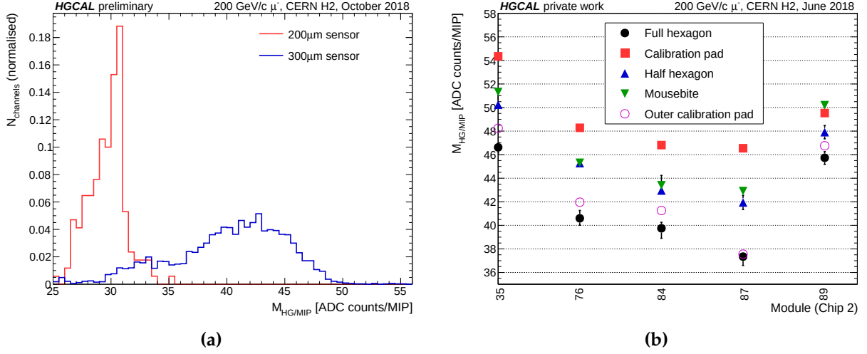
Figure 9.12: (a) Distribution of calibrated high gain MIP calibration constants including only full hexagonal diodes with different sensor thicknesses measured with 200 GeV/c muons. (b) Comparison of the response for different diode geometries.
