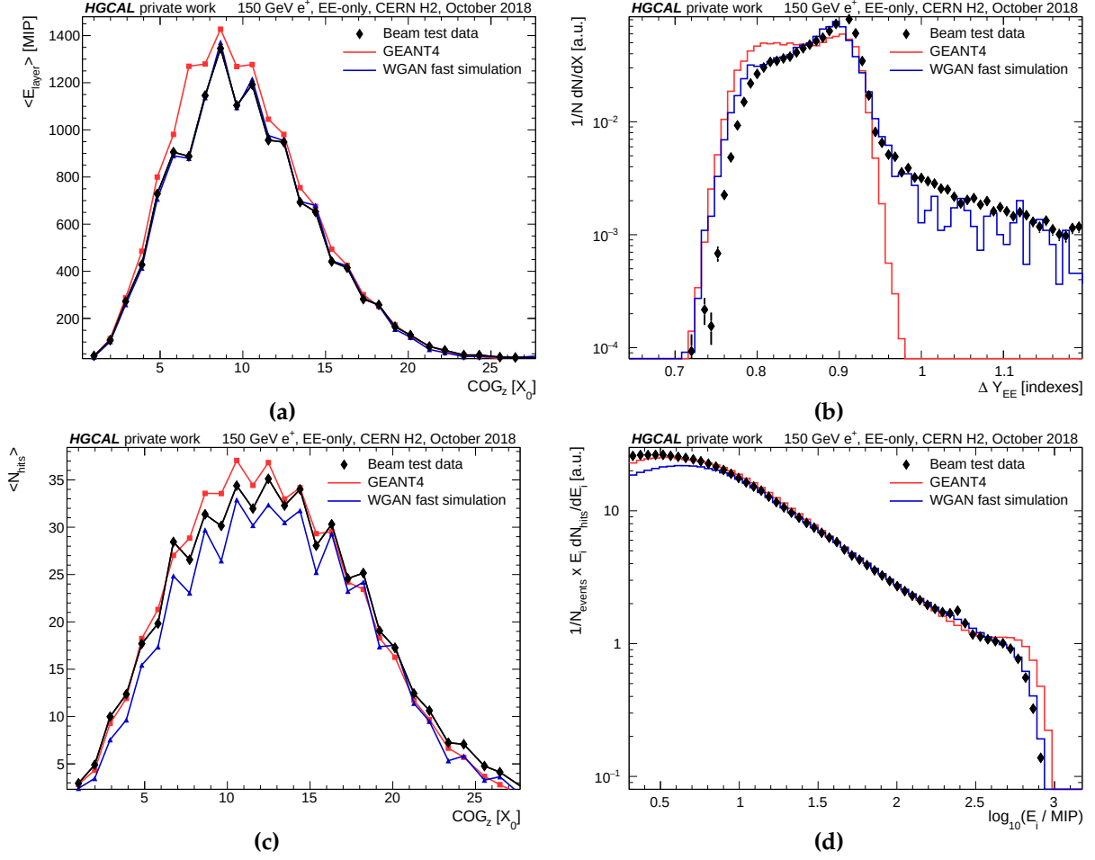
Figure 11.12: Comparison of calorimetric observables due to 150 GeV positrons between the recorded beam test data (black), full GEANT4 simulation with the FTFP_BERT_EMM physics list (red) and fast simulated samples generated by the WGAN (blue). (a) Longitudinal energy profile, (b) transverse shower spread along the y-axis, (c) longitudinal hit profile and (d) energy spectrum of active pixels. Note that the GEANT4 samples in this study incorporate an energy scaling that is different to the one in Equation 9.5. This inconsistency does not alter the interpretation of these graphics as discussed in the text.
