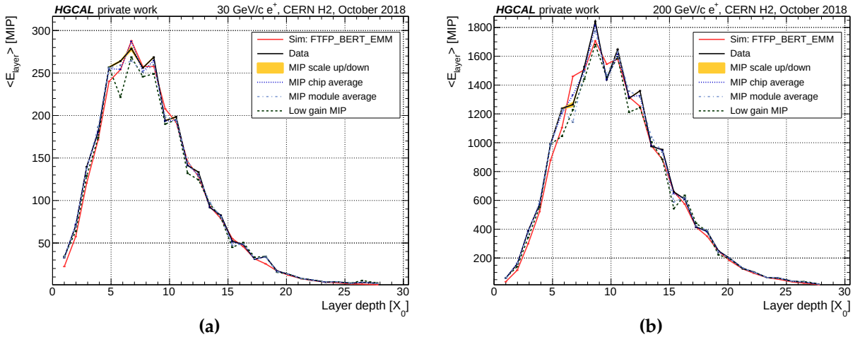
Figure 10.4: Longitudinal shower profiles for electromagnetic showers induced by incident positrons with a momentum of (a) 30 GeV/c and (b) 200 GeV/c.
