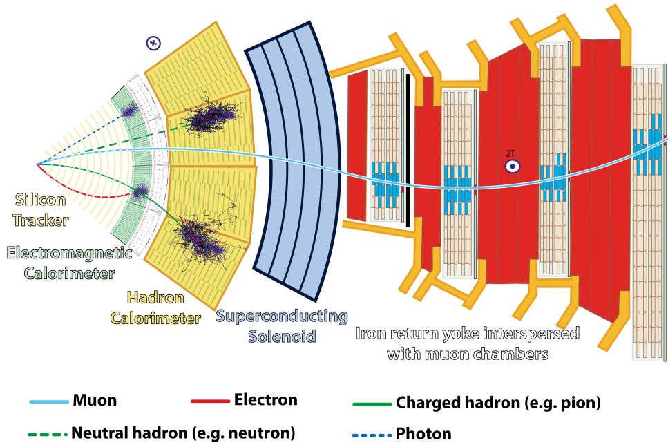
Figure 2.6: Cross section view of the CMS detector and the typical signatures of different particle types therein. The Particle Flow algorithm exploits the measurements from all sub-detectors for the interpretation of the data as physics objects. Figure taken from Ref. [71].
