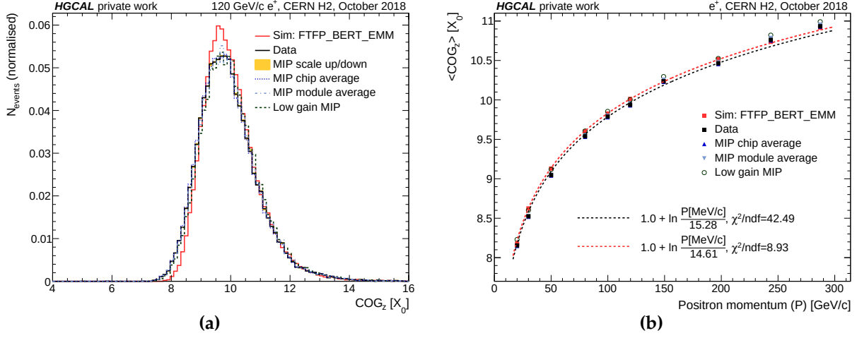
Figure 10.5: (a) Distribution of the longitudinal centre of gravity computed for 120 GeV/c positron-induced showers and (b) the logarithmic dependence of its mean on the incident particle momentum.
