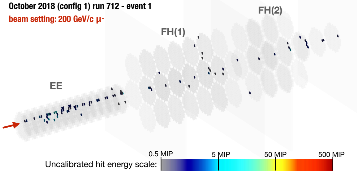
Figure 9.1: Event display of a 200 GeV/c muon traversing the electromagnetic calorimeter (28 layers) and the hadronic calorimeter (12 layers) prototype compartments taken from the O1M dataset. The incoming muon enters the detector from the left-hand side. The HGCAL beam test prototype event display tool [199] was developed as part of this thesis.
