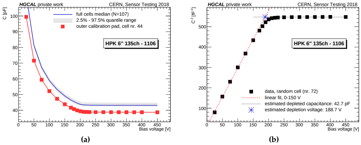
Figure 8.5: (a) Summary of measured CV curves for sensor HPK 6'' 135ch - 1106 after application of the open correction. Only full hexagonal pads are included in this summary. One outer calibration cell (nr. 44) with 8/9 of the full hexagonal cell area is shown in addition. (b) Example estimation of the depletion voltage for a full cell (nr. 72) on sensor HPK 6'' 135ch - 1106.
