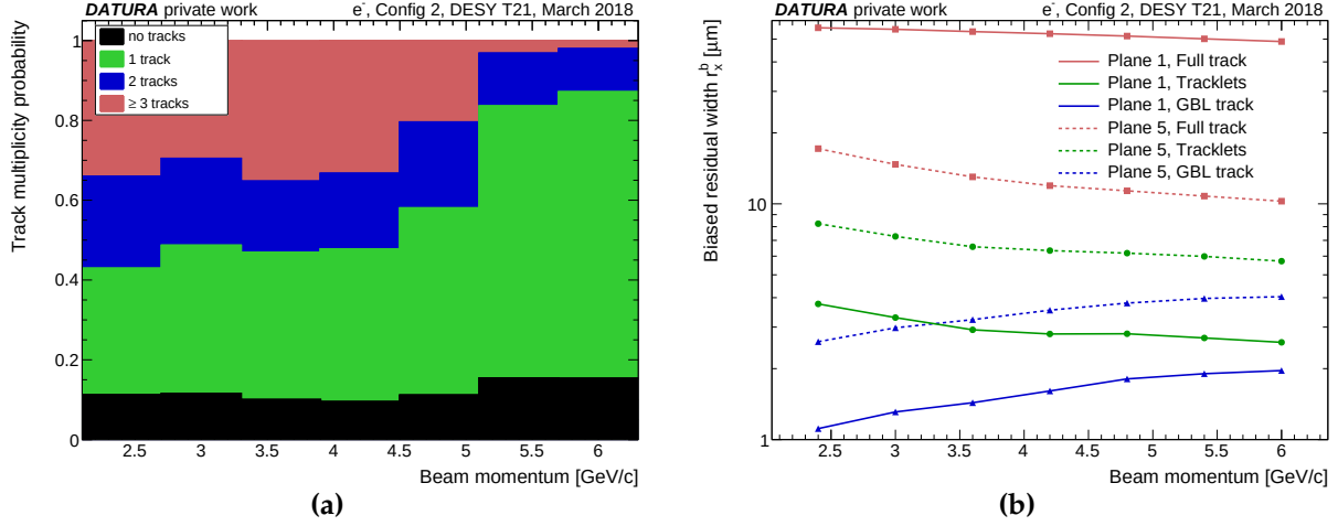
Figure 7.10: (a) Multiplicity of reconstructed tracks with the DATURA beam telescope during the HGCAL beam test at DESY in March 2018. (b) RMS of biased residual distributions for tracklets, full and GBL tracks at planes 1 and 5.
