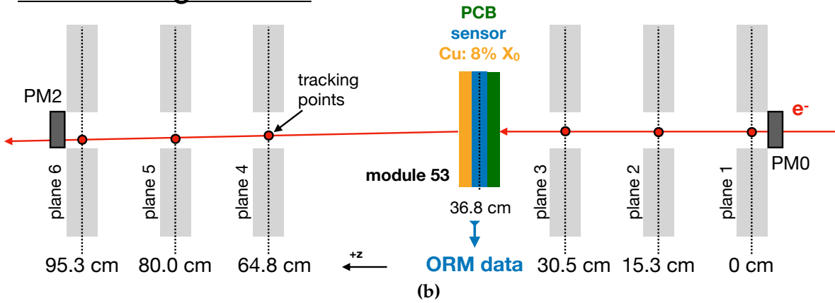
Figure 6.9: Sketch of the two experimental configurations during the HGCal beam test at DESY in March 2018 that are investigated in this work. PM0 and PM2 represent scintillators read out by photomultipliers that were used for triggering. The other two scintillators (PM1 and PM3) were placed in the beam but are not part in the trigger. The "calo-stack" from Fig. 6.8 is not shown.
