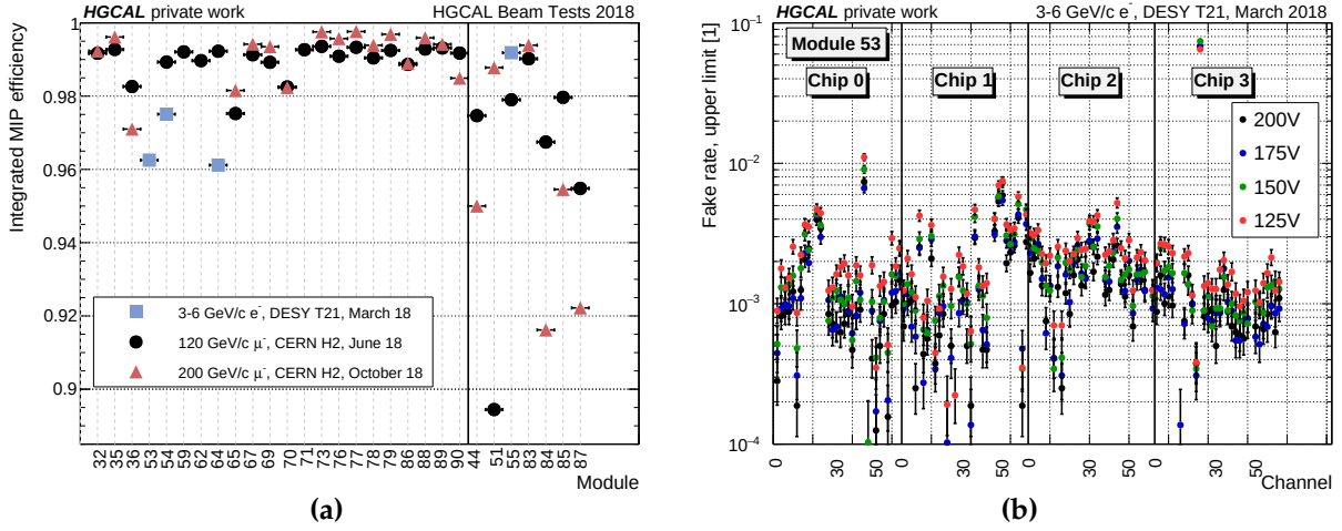
Figure 8.15: (a) Module-integrated efficiency to detect minimum ionising particles for all modules tested in June 2018 ( JUN dataset) and overlaid with the respective results from the other beam test campaigns. (b) Fake rates for different bias voltages and for all channels on module 53 that were outside the beam acceptance during the M1 programme in March 2018 at DESY.
