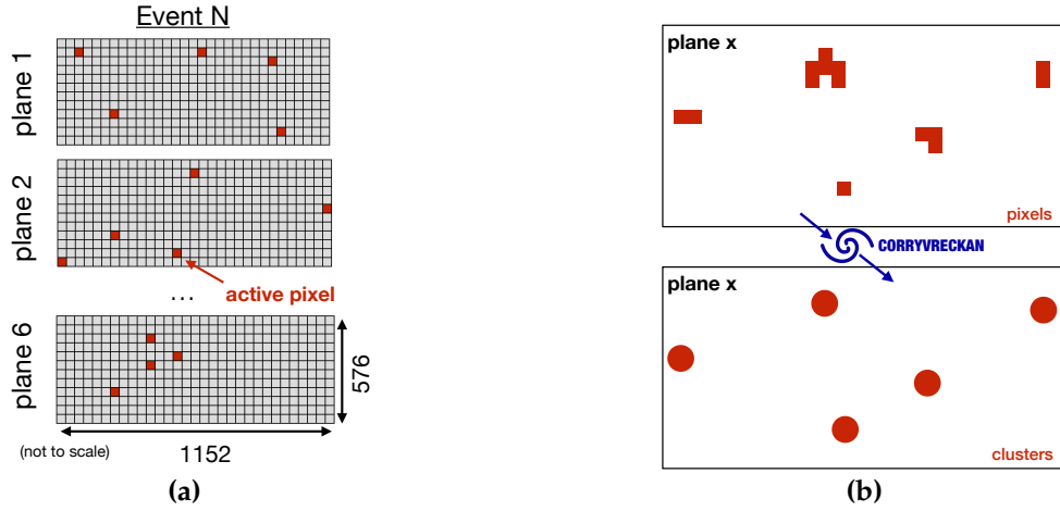
Figure 7.6: (a) Schematic illustration of the DATURA beam telescope's raw data and (b) the pixel clustering provided by CORRYVRECKAN.
