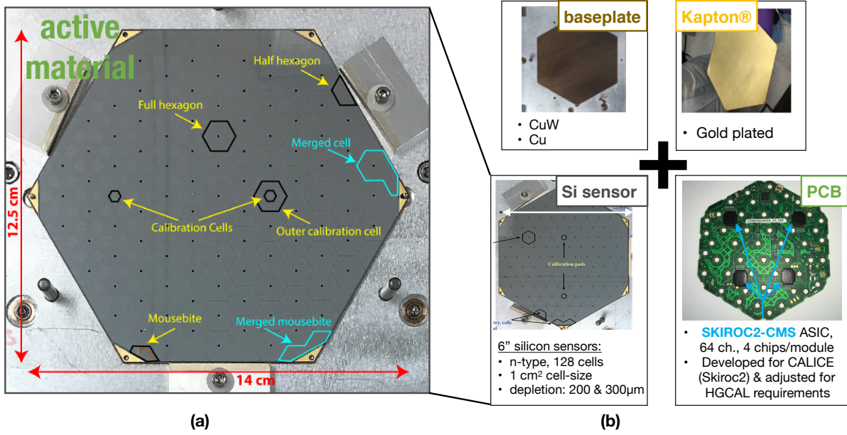
Figure 4.11: (a) Prototype sensor design and different pad geometries. Merged cells were not incorporated into the 2018 modules that are subject in this thesis. (b) Overview on the beam test module assembly in 2018.
