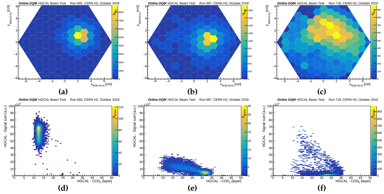
Figure 6.5: Online DQM: (Top) Number of hits of channels with estimated signals above a configurable threshold. (Bottom) Two-dimensional distribution of the summed calorimeter signal and the estimated longitudinal centre of gravity using low gain only. Examples taken from runs with (a, d) 200 GeV/c positrons, (b, e) 50 GeV/c pions and (c, f) 200 GeV/c muons are shown.
