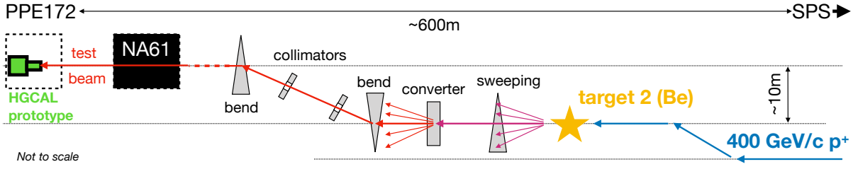
Figure 6.10: Sketch of the H2 beam line operated with electron beam. The length of the beam line from the SPS to the test area (PPE172) amounts to approximately 600 m. It comprises various targets, collimators, di- and quadrupole magnets whose operating parameters can be modified depending on the user-specific requirements to the beam. The NA61 experiment [161] is located in front of PPE172 and adds some amount of passive material to the beam line.
