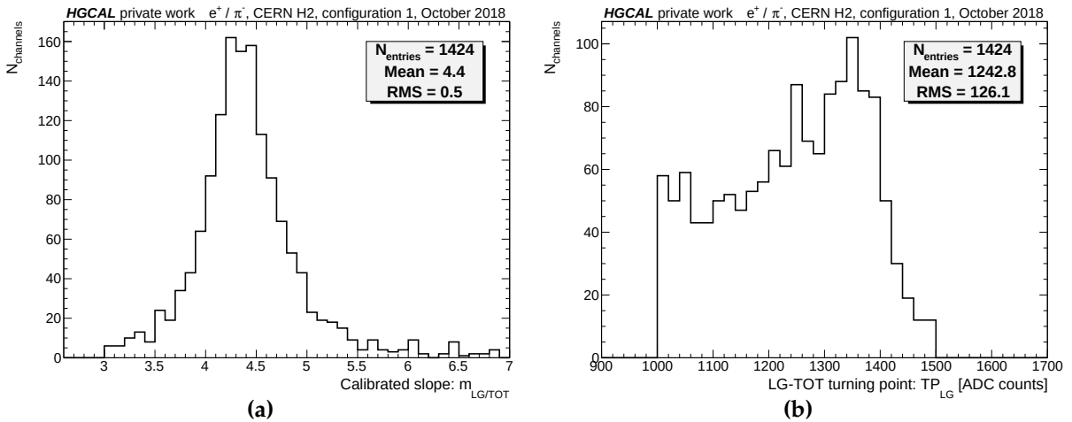
Figure 9.16: Result of the intercalibration of the low gain ADC the time-over-threshold. (a) The slope ( m_{\text{LG}/\text{TOT}} ) and (b) turning points ( TP_{\text{LG}} ) could be derived for only 12% of all channels with the O1E and O1H datasets due to the limited transverse beam spread with high-energetic particle showers.
