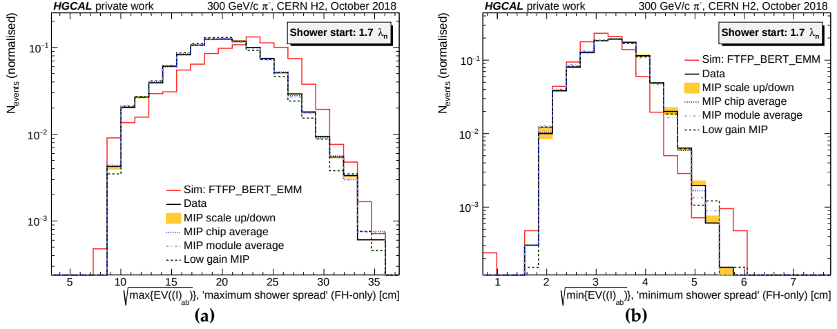
Figure 10.18: (a) Longitudinal and (b) transverse shower spread for 300 GeV/c charged pions where the shower is initiated at the beginning of the FH compartment. The values are derived from a principal component analysis-inspired method, cf. Equation 10.4. Mind the logarithmic scale.
