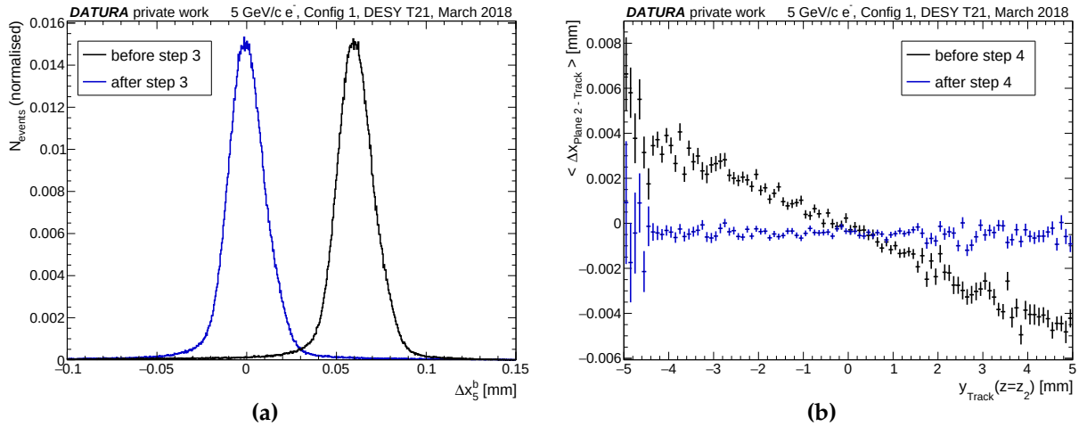
Figure 7.9: Illustration of the telescope plane-to-plane alignment procedures: (a) Effect of alignment step 3 amending relative displacements between the planes. (b) Alignment step 4 correcting the planes' relative rotations along the z-axis.
