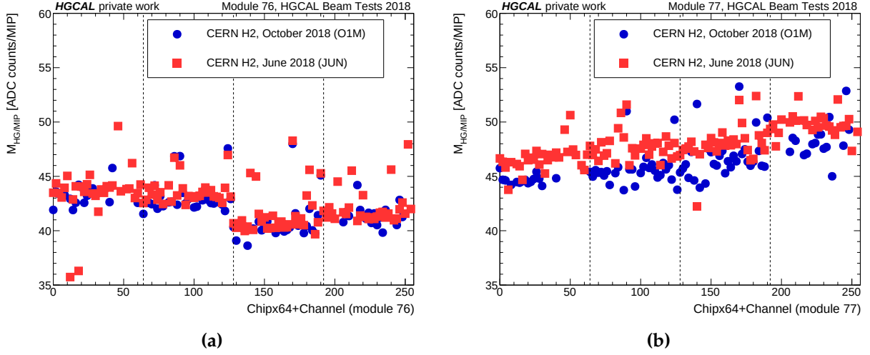
Figure 9.10: Comparison of the calibrated electric response in high gain between the beam test periods in June and in October 2018 ( JUN and O1M datasets) (a) for module 76 and (b) module 77. Statistical error bars are smaller than the marker size. Similar discrepancies like they are shown for module 77 are present for the comparison to the O3 dataset.
