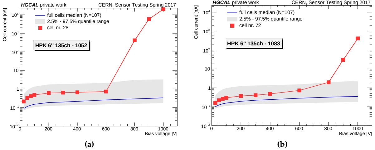
Figure 8.3: Temperature corrected leakage current vs. applied bias voltage (a) for sensor HPK 6'' 135ch - 1052 and (b) sensor HPK 6'' 135ch - 1083. The IV curve for the two single cells with an observed breakthrough are highlighted. Only full hexagonal cells are included in this summary.
