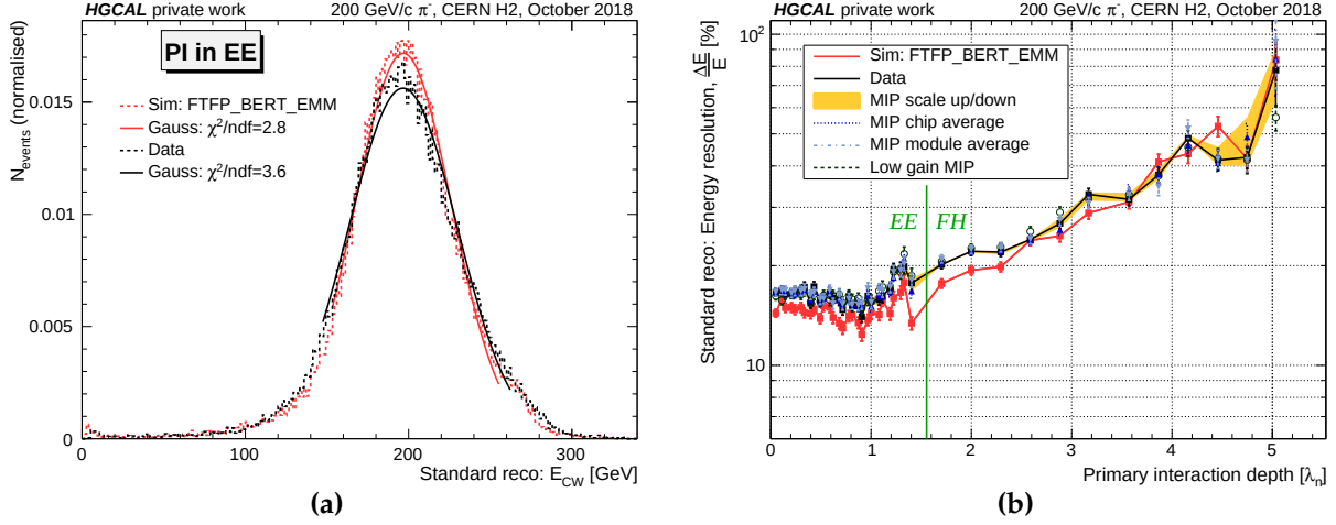
Figure 10.20: (a) Distribution of compartment-weighted energy sums for 200 GeV/c charged pions whose showers are initiated in the EE. The distribution’s core is not accurately described by a Gaussian. (b) Energy resolution estimates for charged pion showers that are initiated at different depths. The increase for showers that are initiated later is due to increasing longitudinal leakage.
