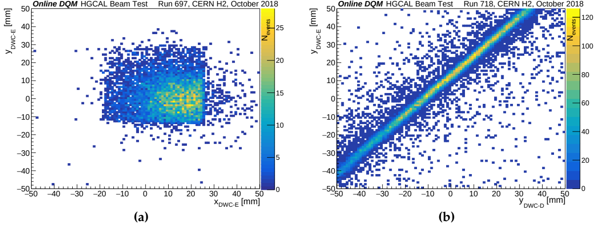
Figure 6.14: (a) Exemplary beam occupancy distribution measured by DWC E and (b) correlation in the y-coordinate determined by DWCs D and E as visualised by the online monitoring during the HGCal prototype beam test in October 2018.
