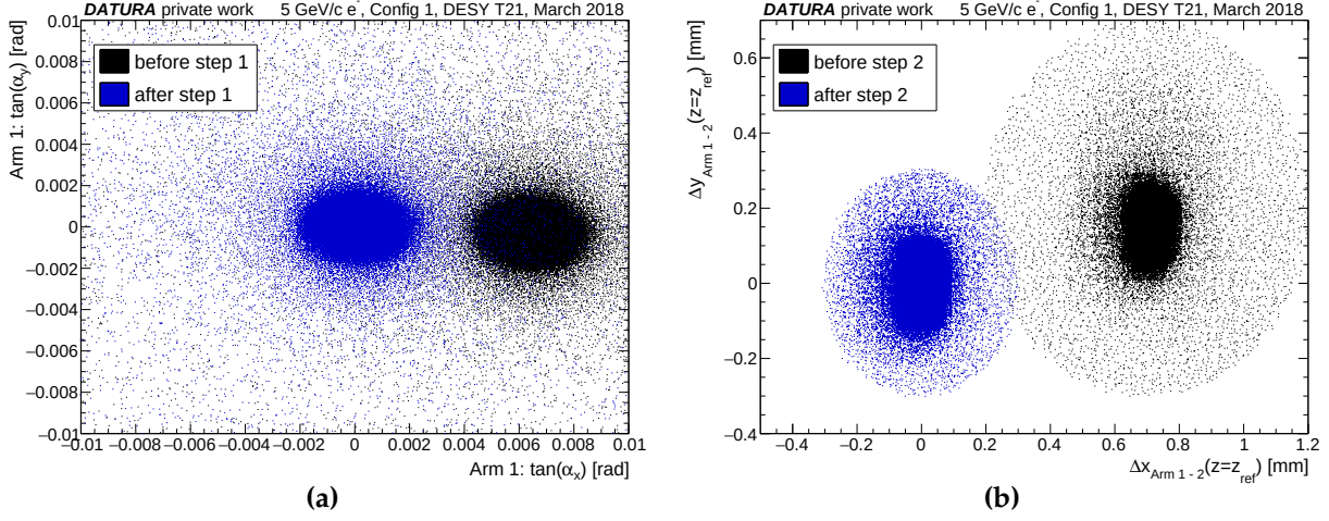
Figure 7.8: Illustration of the telescope arm-to-arm alignment procedures: (a) Effect of alignment step 1 correcting for their different orientations, here shown for arm 1. The tracklet angle is denoted as \alpha_{x(y)} . (b) Alignment step 2 in which the second arm is translated to amend its relative displacement, \Delta x_{\text{Arm 1-2}} ( y analogous), with respect to the first arm.
