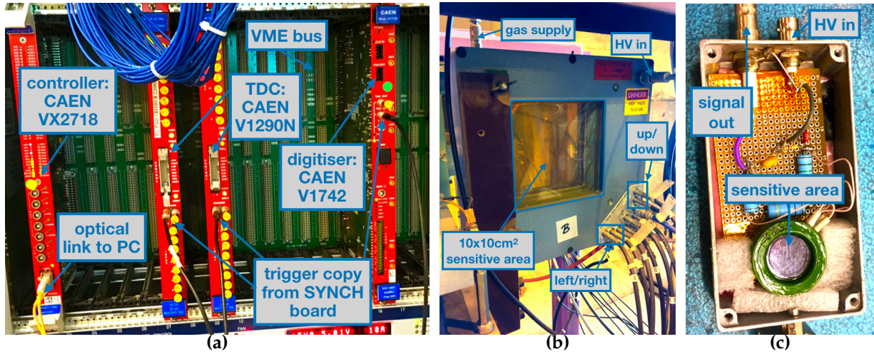
Figure 6.13: (a) VME modules used for the readout of the beam characterising detectors. The CAEN VX2718 controller is the bridge between the modules and the DAQ computer. (b) Representative photograph of (the unused) delay wire chamber B in the PPE172 area. (c) Photograph of one of the two MCPs. During operation, its case is closed to minimise light-induced signal distortions. All photos have been taken during the preparation for the HGCAL prototype test in October 2018.
