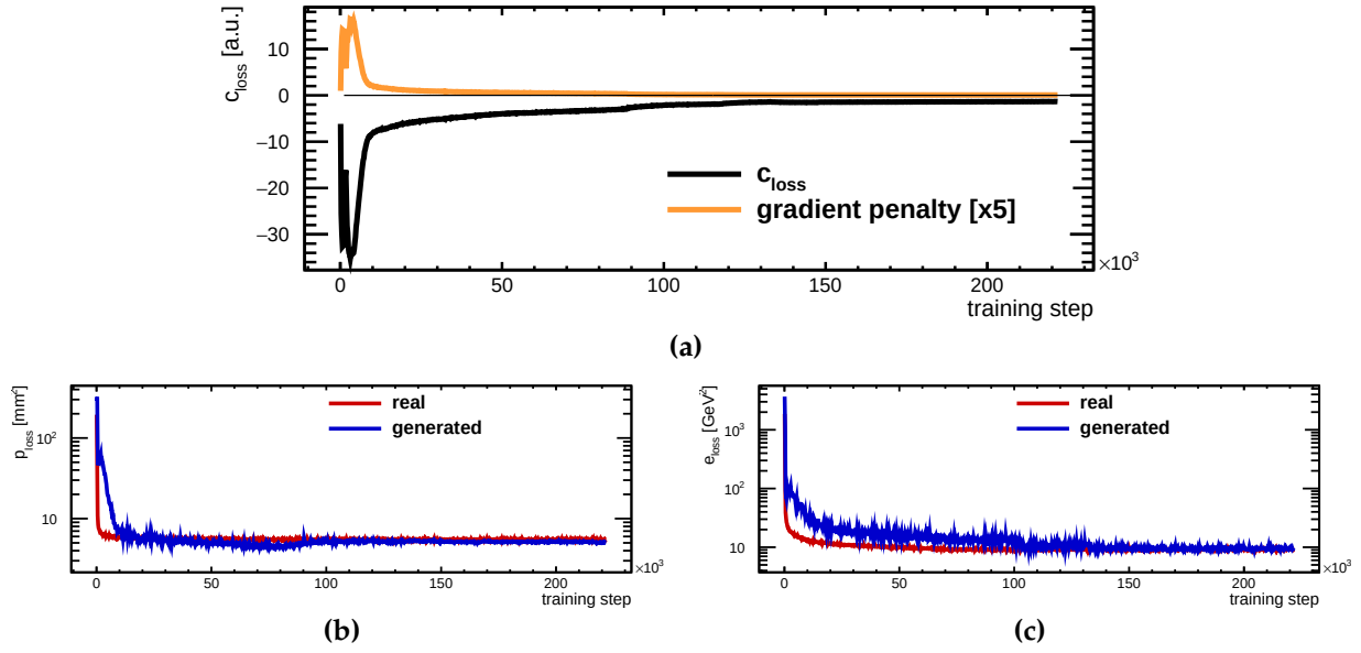
Figure 11.4: (a) Total critic loss c_{\text{loss}} during the training (black) and rescaled gradient penalty (yellow). (b) Loss curves of the constrainer networks during the supervised training for the position regression p_{\text{loss}} and (c) the energy reconstruction e_{\text{loss}} .
