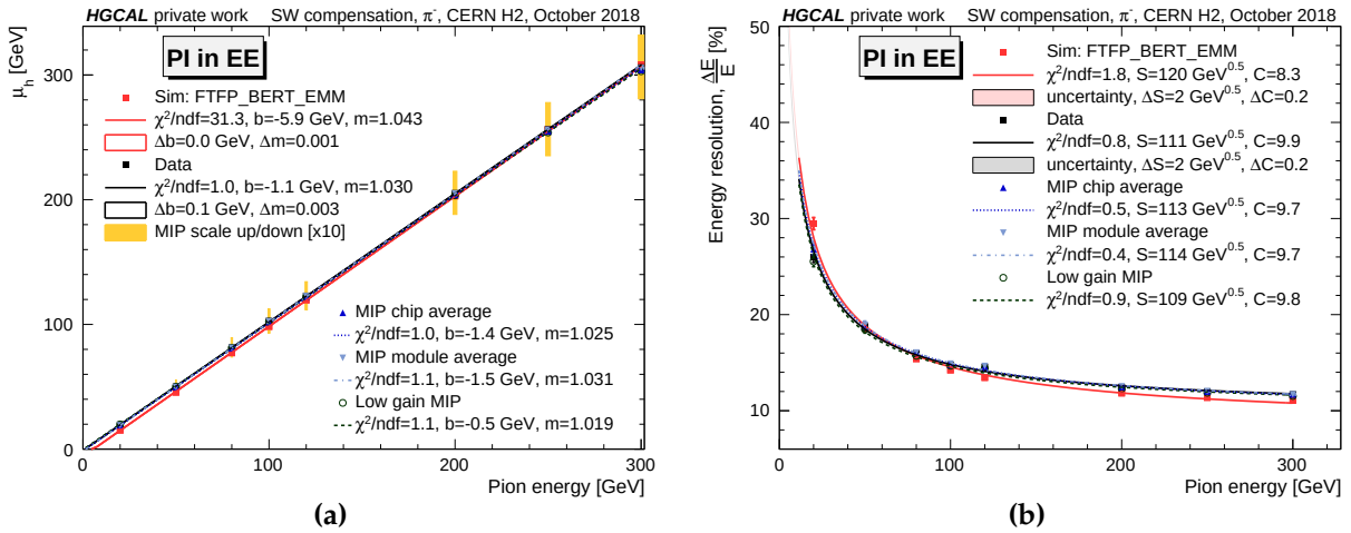
Figure 10.25: (a) Energy linearity and (b) resolution of the HGCAL prototype calorimeter for charged pions with a shower start anywhere inside the EE compartment using a variation of the CALICE inspired, local software compensation. Data from the CALICE AHCAL prototype are not included in these results. The underlying evaluation of the reconstructed shower energy distributions is identical to the procedure in Section 10.2.2.
