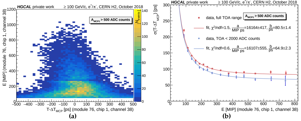
Figure 9.21: Timing resolution for one exemplary readout channel: (a) Distribution of differences between the calibrated TOA timestamp T and the MCP reference time for different reconstructed hit energies. (b) Combined MCP and TOA resolution as a function of the hit energy for TOA values covering the full range and for those restricted to the linear region in the TOA - \Delta T_{\text{MCP}} relationship. The data are well described by the parameterisation in Equation 9.8.
