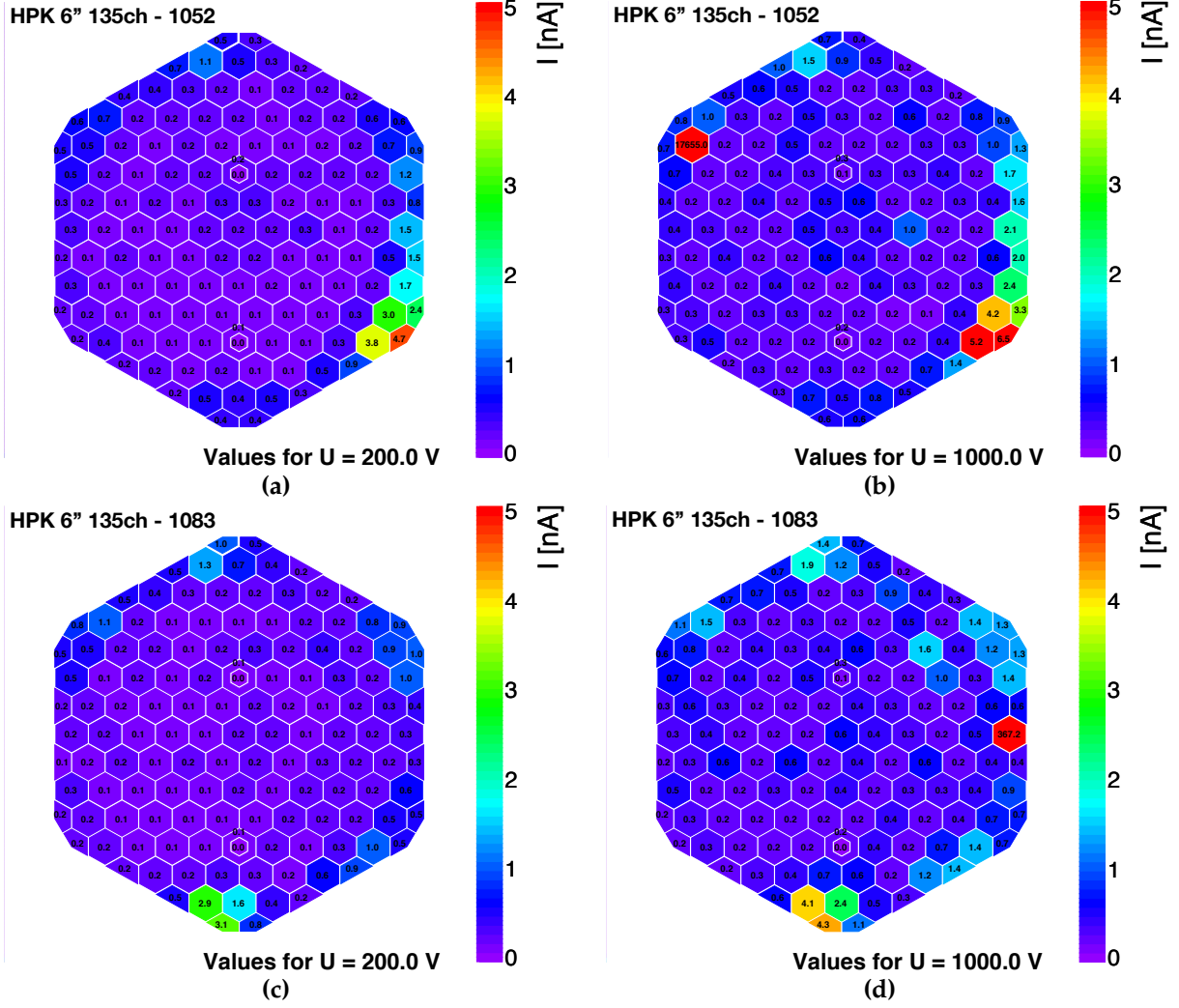
Figure 8.1: Hexplots showing the measured leakage currents of sensor HPK 6'' 135ch - 1052 (a) at an applied bias voltage of 200 V, (b) at 1000 V and (c) for sensor HPK 6'' 135ch - 1083 at 200 V and (d) at 1000 V. Cells with currents above the indicated scale are coloured red. The temperature during the measurements ranged from 21.5–24.5°C. No temperature correction is applied in these graphics.
