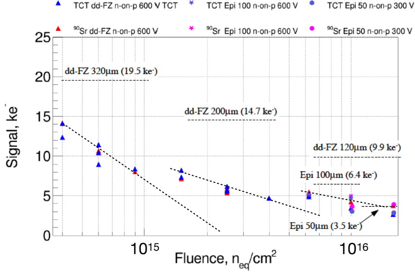
Figure 4.7: Measured signal for different prototype silicon sensors after exposure to a certain neutron fluence. The range of fluences includes the maximum expected exposure after 3000 \text{ fb}^{-1} of integrated luminosity. Figure taken and modified from Ref. [120].
