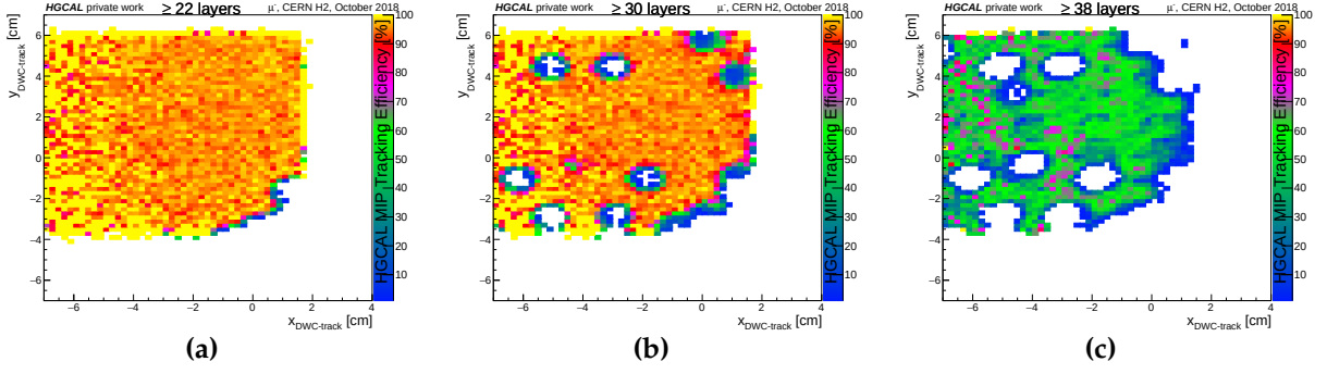
Figure 9.3: Efficiency to reconstruct MIP-like trajectories with the HGCal prototype as a function of the DWC-track extrapolation using the O1M dataset. Shown are the efficiency maps for trajectories with (a) at least 22, (b) 30 and (c) 38 contributing layers.
