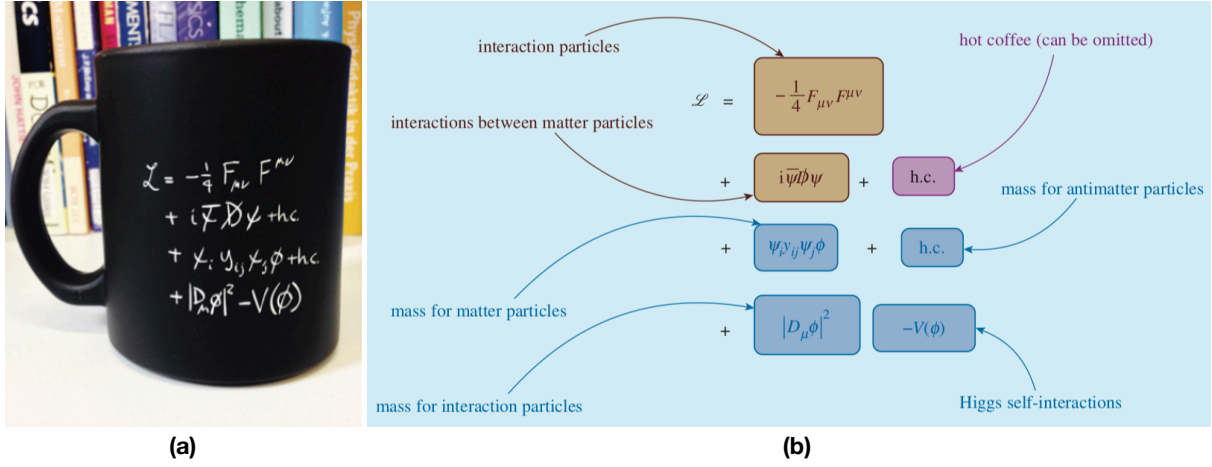
Figure 2.2: (a) Compact version of the SM Lagrangian on a coffee mug. (b) The terms coloured in brown are governed by the electromagnetic, weak, and strong forces, while those that are coloured blue are governed by interactions with the Brout–Englert–Higgs field. Figures and captions taken from Ref. [30].
