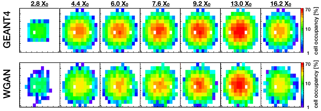
Figure 11.6: (Top) Cell occupancy for 90 GeV electrons simulated using GEANT4 and (bottom generated by the WGAN. Dead pixels and areas outside the sensor acceptance are masked in the generator.
