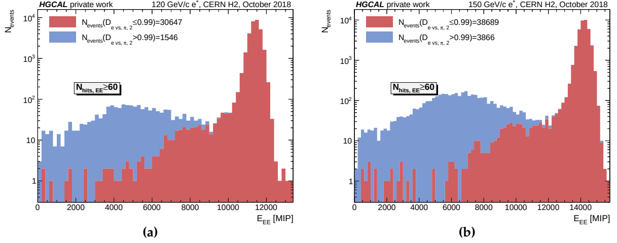
Figure 10.28: Reconstructed energy sum in the EE compartment for (a) 120 GeV/c and (b) 150 GeV/c particles from a run with positrons. Electron-identified contributions are shown in red and pion-identified contributions are blue. Together with the 100 GeV/c sample, these two instances show the relatively highest amount of pion-like signatures inside the EE in the O1E dataset.
