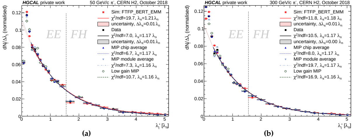
Figure 10.16: Normalised distribution of the depth of identified primary interactions, for (a) 50 GeV/c and (b) 300 GeV/c charged pion-induced showers. The depth is given in units of the nuclear interaction length \lambda_n .
