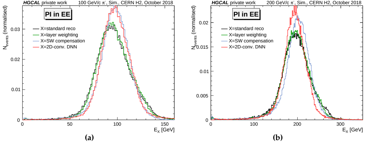
Figure 10.22: Distribution of the computed shower energy with the different energy reconstruction methods discussed in this section (a) for 100 GeV/c charged pions and (b) for 200 GeV/c charged pions. The evaluation is based on simulated charged pions with a shower start anywhere inside the EE compartment.
