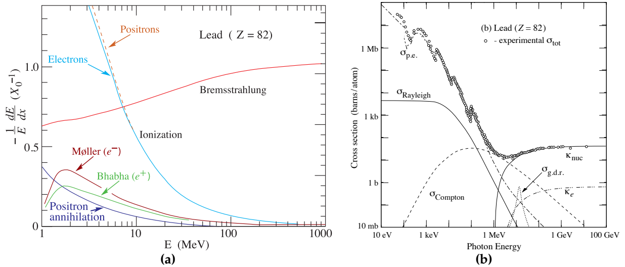
Figure 3.3: (a) The fractional energy loss per radiation length of electrons and positrons in lead as a function of their energy. (b) Cross sections of the photon interactions with lead as a function of the photon energy. The shown processes are Rayleigh scattering ( \sigma_{\text{Rayleigh}} ), the photoelectric effect ( \sigma_{\text{p.e.}} ), Compton scattering ( \sigma_{\text{Compton}} ), pair production by the nucleus ( \kappa_{\text{nuc}} ) and electron fields ( \kappa_e ), as well as photo-nuclear absorption ( \sigma_{\text{g.d.r.}} ). Figures taken from Ref. [16].
