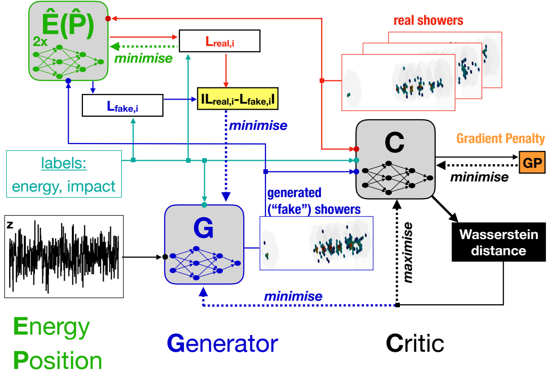
Figure 11.2: Overview of the adversarial WGAN framework for the training of the generator. The critic network C estimates the Wasserstein (=earth mover's) distance between real and generated, i.e. fake, shower images. Two auxiliary networks a_1 = \hat{E} and a_2 = \hat{P} are used in order to assist the incorporation of the initial shower conditions (energy and impact position) into the generation process.
