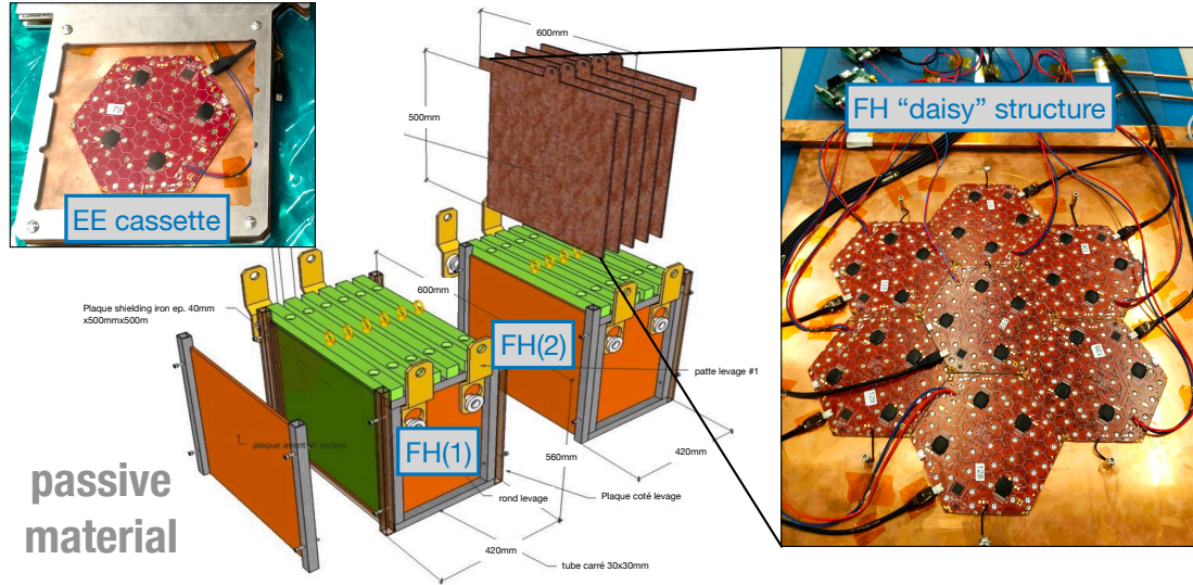
Figure 4.12: Mechanics and structure of the sensitive layers made from the silicon modules forming the HGCAL calorimeter prototypes for the beam tests in 2018. FH(1) and FH(2) denote the mechanically separated hanging file structures that make the FH compartment.
