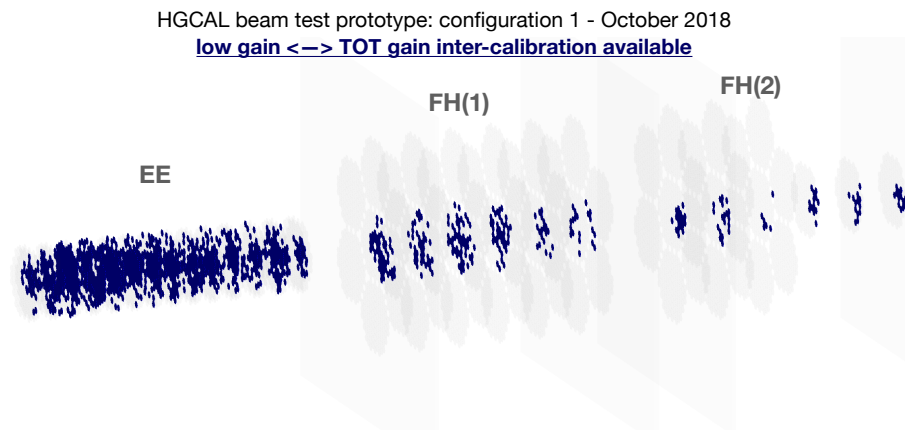
Figure F.3: Location of cells whose low gain vs. TOT could be intercalibrated in the October 2018 HGCAL beam test.
