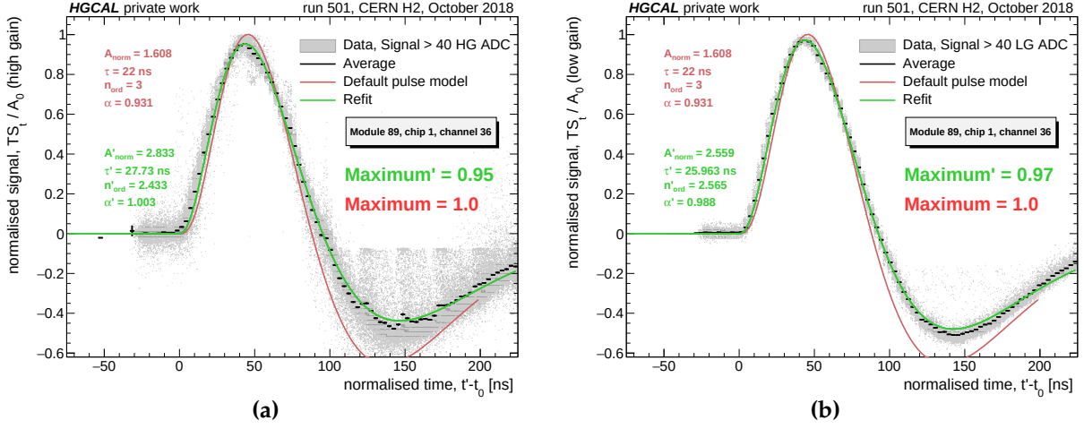
Figure 7.3: Illustration of the pulse fit model used for amplitude reconstruction in a readout channel for (a) the high- and (b) the low-gain ADC. Time samples are normalised by the fitted amplitude and start time for each event as obtained from the default pulse reconstruction fit using the parameterisation illustrated in red. The green curve represents a refit to the average, normalised samples where all parameters are allowed to vary. Its parameters seem to render a better description of the pulse shape incorporating even the undershoot.
