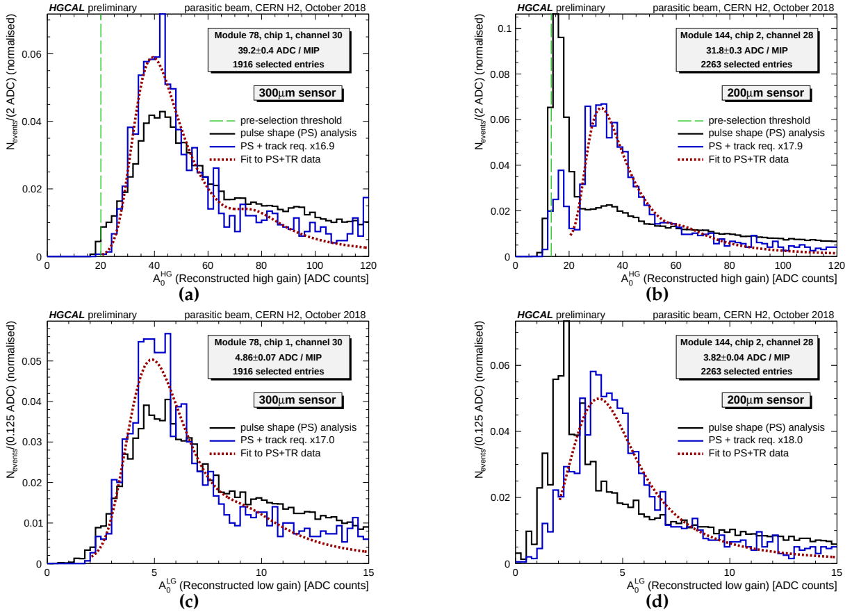
Figure 9.9: (a, b) Spectrum of reconstructed MIP-induced signal amplitudes both in high- and (c, d) in low gain for the two readout channels of Figure 9.6. Hits contributing to a MIP-like track in the data are selected. The inclusive spectra are normalised to unity integral. The selected spectra are scaled accordingly whereby an additional scaling, indicated in the legend, is applied for better visualisation.
