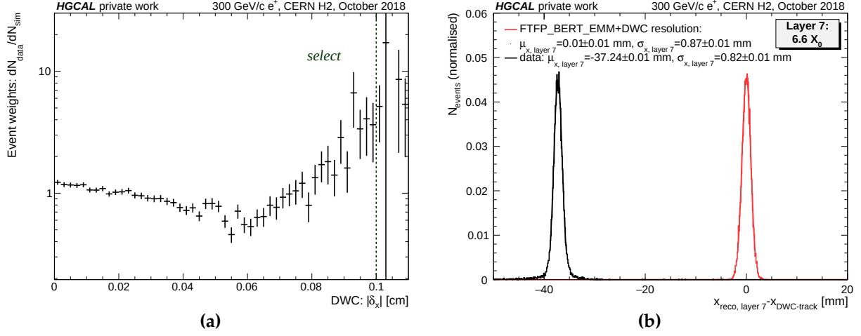
Figure 10.10: (a) Event weights for simulated 300 GeV/c positron samples to incorporate non-Gaussian effects of the DWC's pointing resolution into the simulation. The analysis is restricted to events with |\delta_{x(y)}| < 0.1 cm. (b) Residual distribution of the horizontal shower impact position measured in layer 7 and the DWC extrapolation for incident 300 GeV/c positrons. DWC event weights are applied in the simulation.
