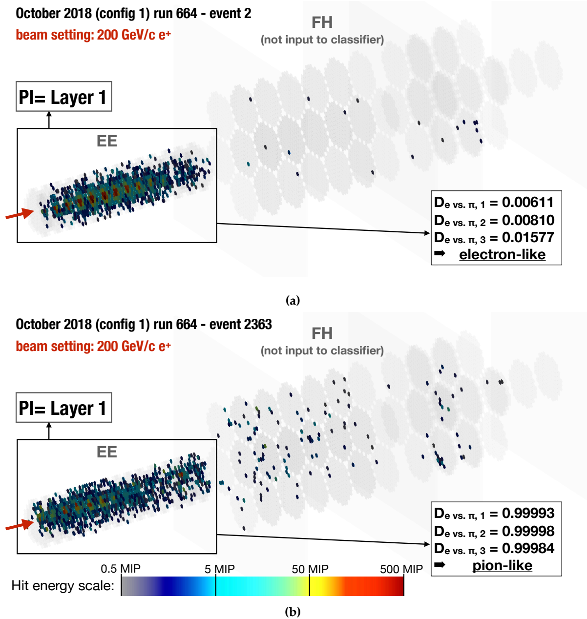
Figure 10.27: Example of (a) an electron-like and (b) a pion-like shower recorded with test beam of positrons. The reconstructed shower start corresponds to the first layer. Only the hits from the EE compartment are input to the DNN classifiers.
