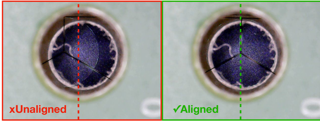
Figure 6.3: Sensor-to-probe-card alignment using the alignment hole and the USB microscope.
