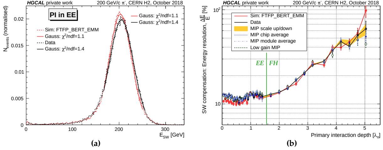
Figure 10.24: (a) Distribution of reconstructed particle energy using software (SW) compensation for 200 GeV/c charged pions. This method compensates for the different response to electromagnetic and hadronic showers. Thus, the core of the distribution becomes more Gaussian with respect to the standard reco. (b) Energy resolution for charged pion showers initiated at different depths. The increase for later showers is due to the limited longitudinal coverage of the HGCAL beam test prototype.
