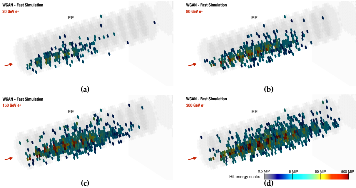
Figure 11.11: Event displays of fast simulated positron-induced electromagnetic showers inside the 28-layer EE prototype calorimeter compartment. The generator network was trained with showers from the O1E dataset.
