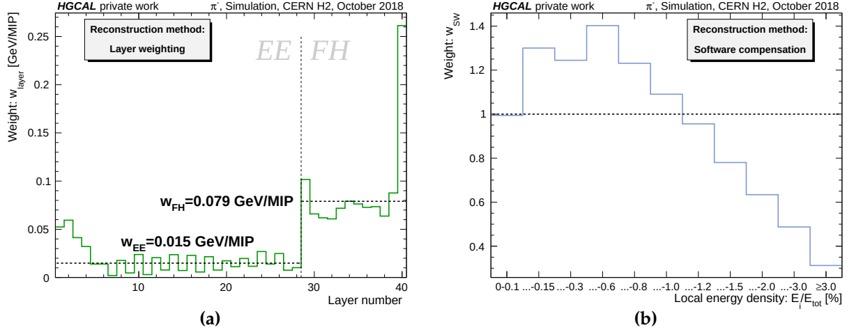
Figure 10.21: (a) Layer weights for the two compartments in comparison to the layer weights obtained in the standard reco (green). (b) Software compensation weights that are determined by a hit's relative contribution to the summed energy of the shower. The values are obtained from the optimisation of Equation 10.24.
