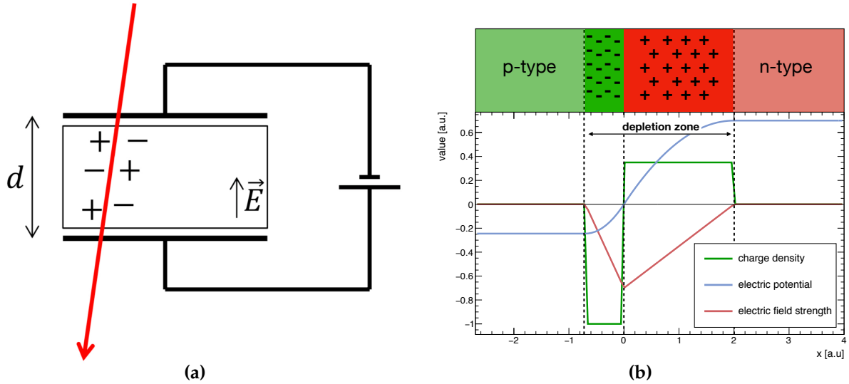
Figure 4.6: (a) Working principle of silicon as an ionisation chamber for particle detection. (b) An instructive model of a pn-junction, as well as the electric potential and field strength therein.
