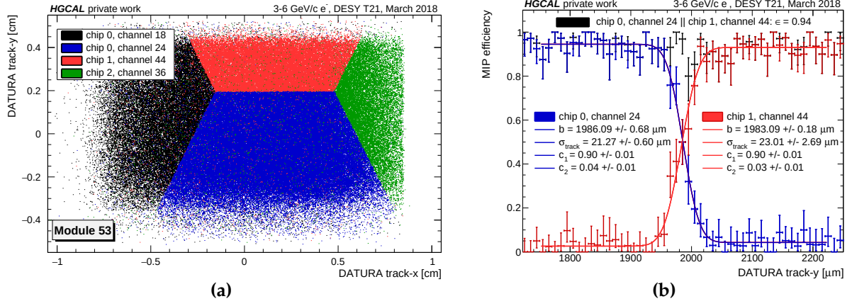
Figure 8.16: (a) DATURA track occupancy of events with one reconstructed trajectory. Entries are colour-coded depending on the simultaneously reconstructed hits. (b) MIP detection efficiency at the horizontal boundary region between channel 44 of chip 1 and channel 24 of chip 0. The physical gap between these diodes is designed 20 \mu\text{m} wide.
