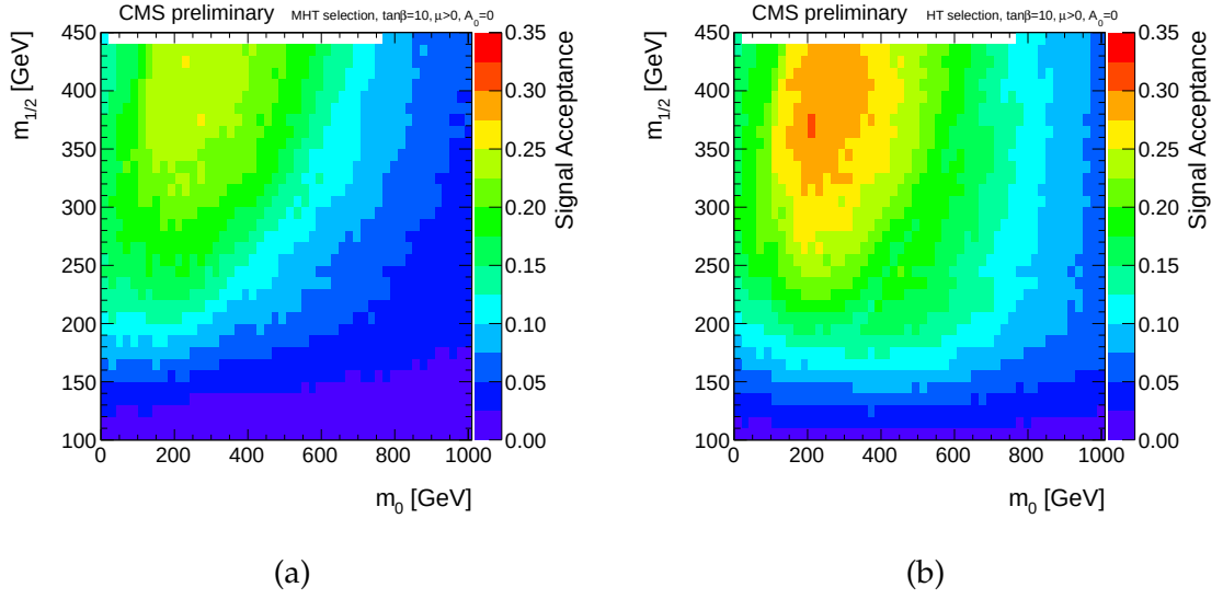
Figure 7.3: The total signal efficiency (selection efficiency times acceptance) is shown in the cMSSM m_0 - m_{1/2} plane for the M_{HT} selection (a) and the H_T selection (b). The other cMSSM parameters are \tan\beta = 10 , \mu > 0 , and A_0 = 0 for both figures. From the paper [1].
