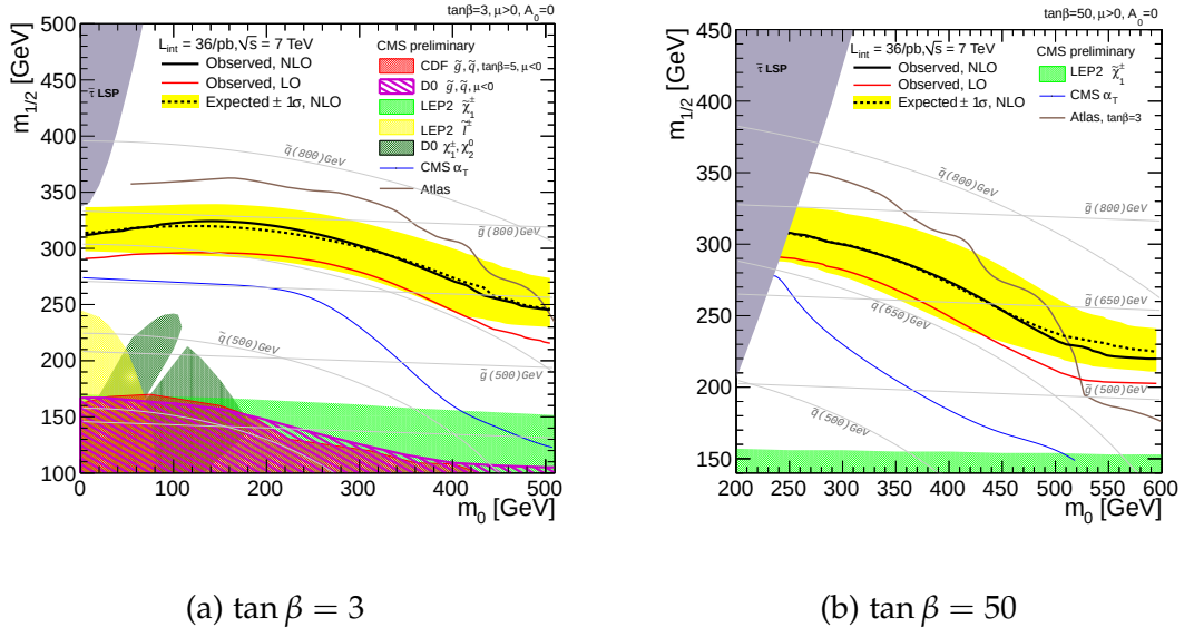
Figure 7.5: The expected and observed 95%CL limits in the cMSSM parameter plane are shown. The figure (a) corresponds to \tan \beta = 3 and (b) corresponds to \tan \beta = 50 . The remaining cMSSM parameters are \mu > 0 , and A_0 = 0 for both figures. From [45].
