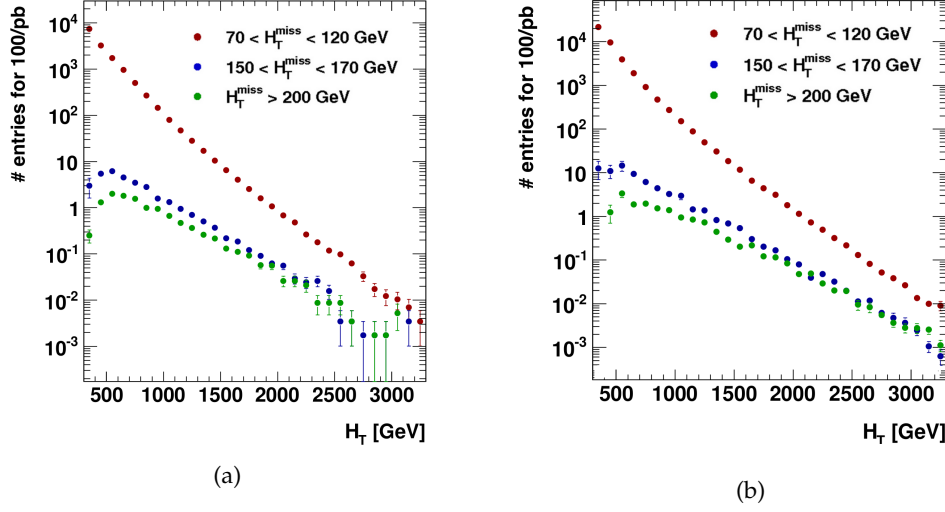
Figure 6.5: Distribution of H_T in three slices of \#H_T for QCD generated with MADGRAPH (a) and PYTHIA (b). The y -axis shows number of entries for 100\text{pb}^{-1} .
