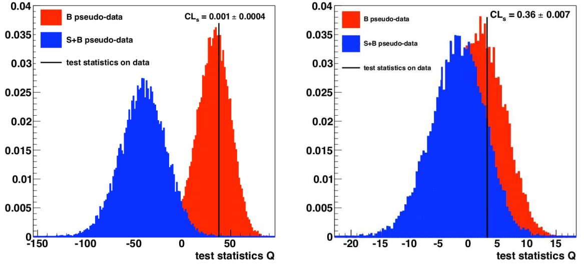
Figure 7.2: Distributions of the test-statistic Q for two different signals in the m_0 - m_{1/2} parameter plane. The precision of the stated CLs values is determined by the finite number of pseudo-experiments (here: 20k for each S + B and B ).
