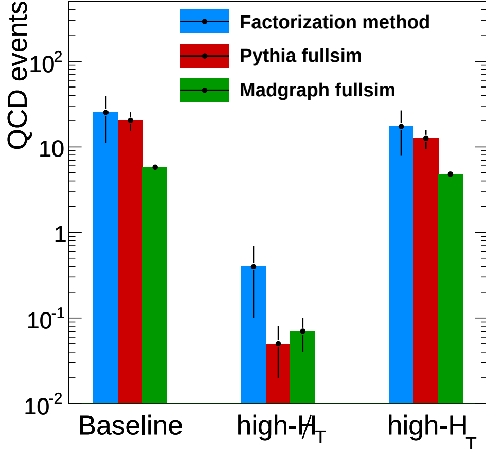
Figure 6.22: Final QCD background prediction for the baseline selection and for the evolved search selections high- \sqrt{s}_T and high- H_T for 36 \text{ pb}^{-1} . The combined result of the factorization method is compared to PYTHIA and MADGRAPH full simulation. The numbers correspond to tab. 6.5.
