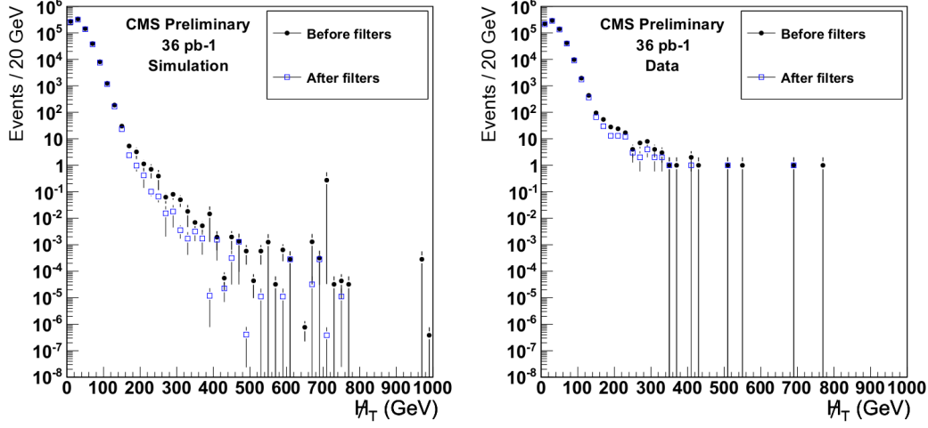
Figure 4.2: Distribution of H_T for the full QCD sample (left) and the full data sample (right), before and after all event filters. The data sample being dominated by electroweak processes with real H_T , it cannot be directly compared to the QCD sample in the high H_T region. From [37].
