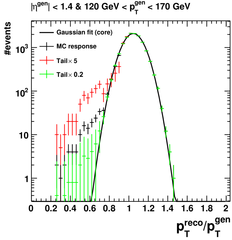
Figure 6.9: Monte Carlo response for jets in one p_{\text{T}}\text{-}\eta bin (QCD PYTHIA). The non-Gaussian tail is added to the core with different scaling factors f = 5 \cdot f_0 and f = 0.2 \cdot f_0 as described in the text.
