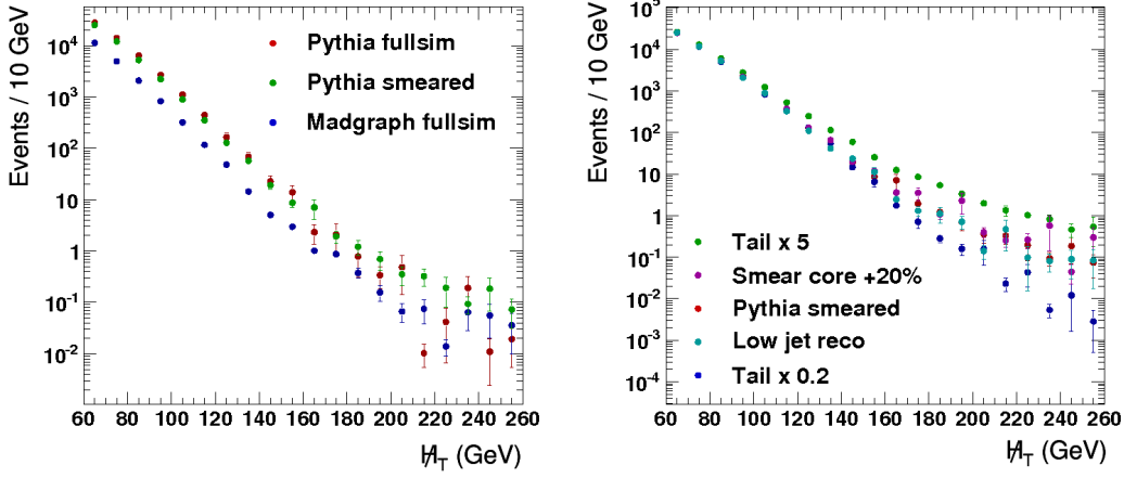
Figure 6.10: \cancel{H}_T distribution after smearing of the generator jets. Left: Comparison of the smeared PYTHIA sample to the full simulation with PYTHIA and MADGRAPH. Right: Different smearing scenarios for the closure test as explained in the text.
