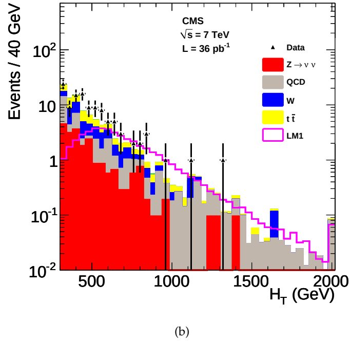
Figure 4.3: M_T and H_T distributions for background and signal with all other cuts from the baseline selection applied. The samples (and sum of SM MC) correspond to tab. 4.2. From the paper [1].
