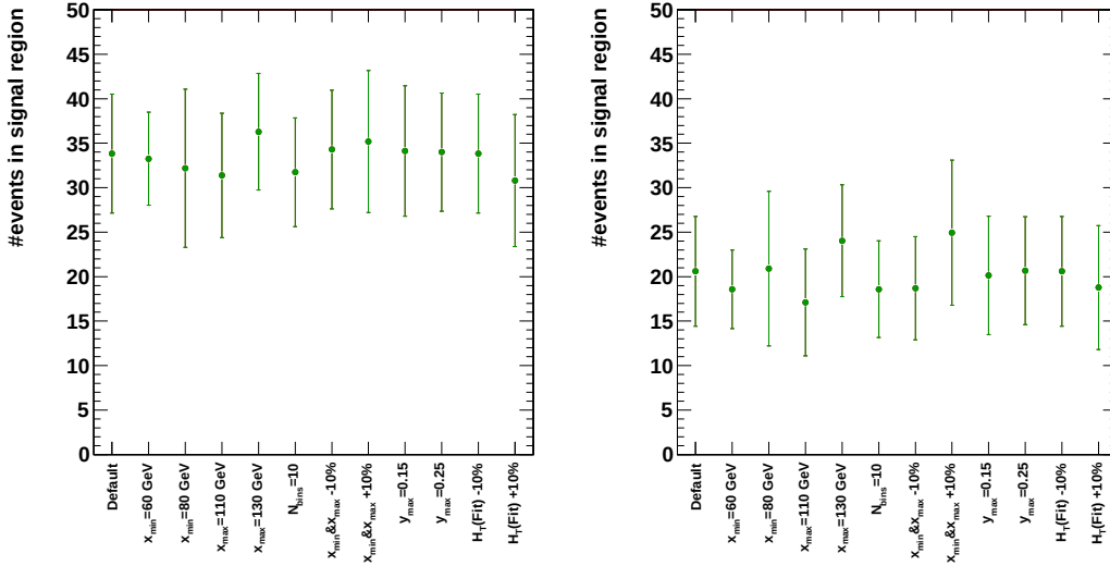
Figure 6.18: Results of the robustness check for data for the exponential extrapolation (left) and the Gaussian model (right). All variations corresponding to the x -axis labels can be found in numbers in tab. 6.3. The statistical errors arise from the error propagation from the fit covariance matrix and the statistics in control region D .
