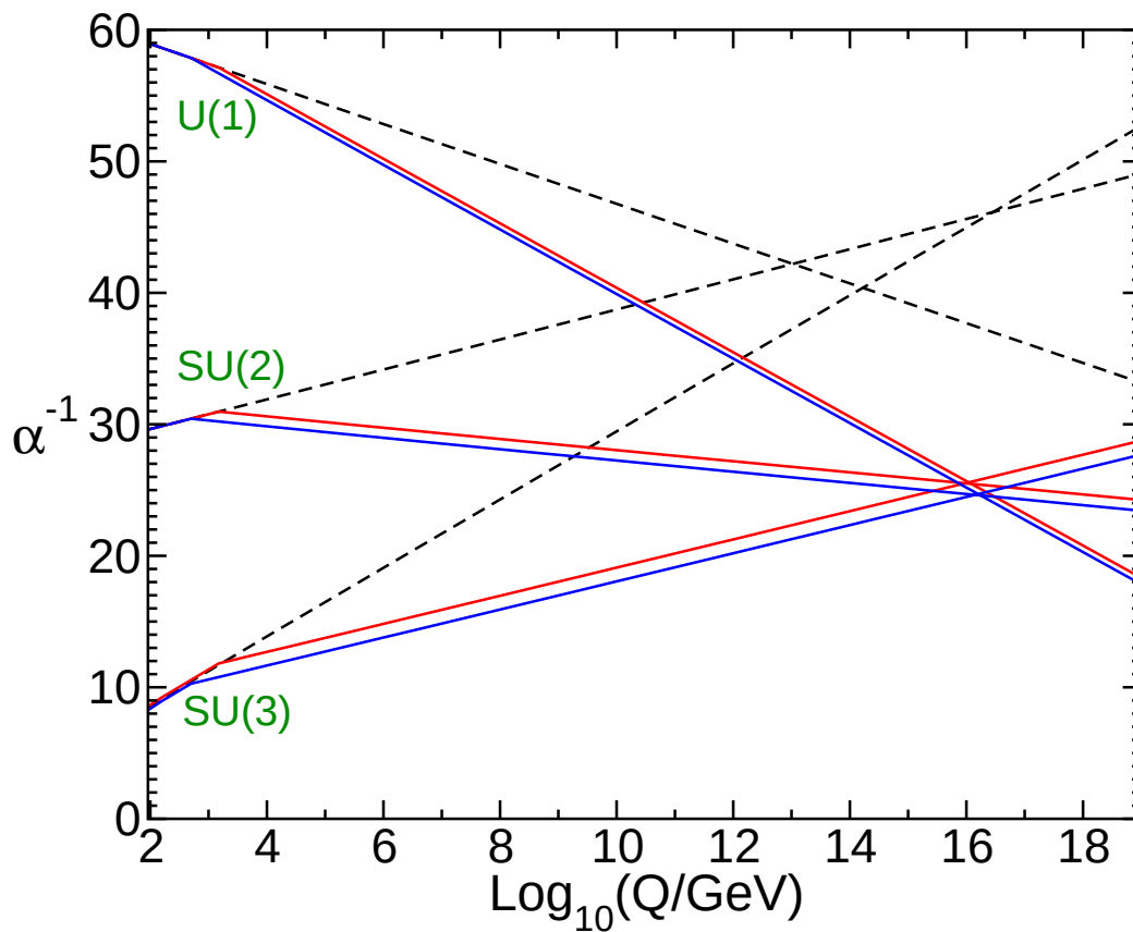
Figure 2.1: Evolution of the inverse gauge couplings of the electroweak interaction ( \alpha_1^{-1} for U(1)_Y and \alpha_2^{-1} for SU(2)_L ) and the strong interaction ( \alpha_3^{-1} ) in the SM (dashed lines) and the MSSM (solid lines). From [8].
