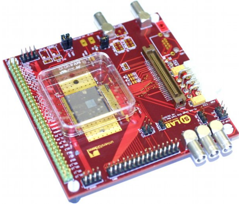
Figure 4.5.: Photograph of an FE-I4A Single Chip Card.
