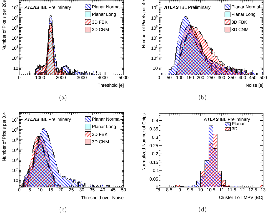
Figure 3.16.: (a) Threshold, (b) threshold noise, (c) threshold over noise distributions per pixel at a module temperature of -12^\circ\text{C} and a threshold calibration target of 1500 e^- . (d) Chip wise time over threshold response for the 14 IBL staves at a module temperature of 20^\circ\text{C} and a threshold calibration target of 3000 e^- [29], [40].
