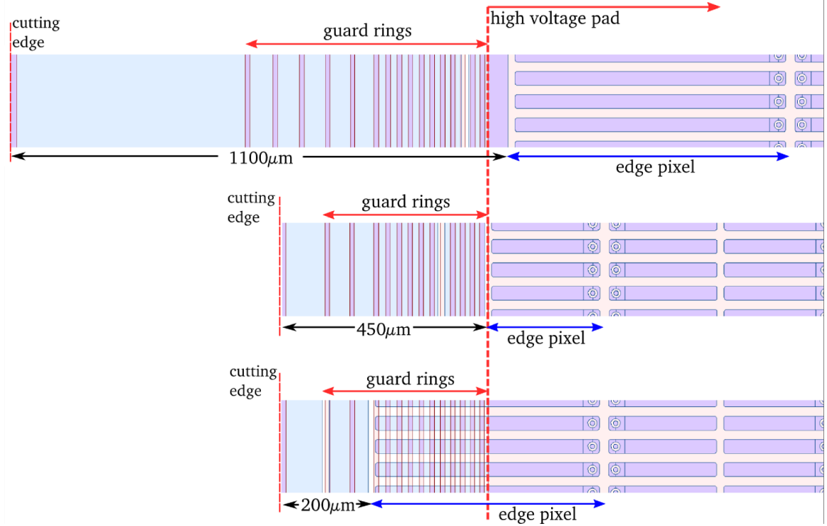
Figure 3.2.: Top view of the sensor edge region of the ATLAS Pixel (top), the conservative (middle) and the slim edge (bottom) IBL design. The \text{n}^+ implantation is seen in blue, the \text{p}^+ implantation in red. By reducing the number of guard rings, narrowing of the safety margin and by extending the edge pixels beyond the high voltage pad, the inactive edge could be reduced from 1100\text{ }\mu\text{m} for the ATLAS Pixel design to ca. 200\text{ }\mu\text{m} for the slim edge IBL design [36].
