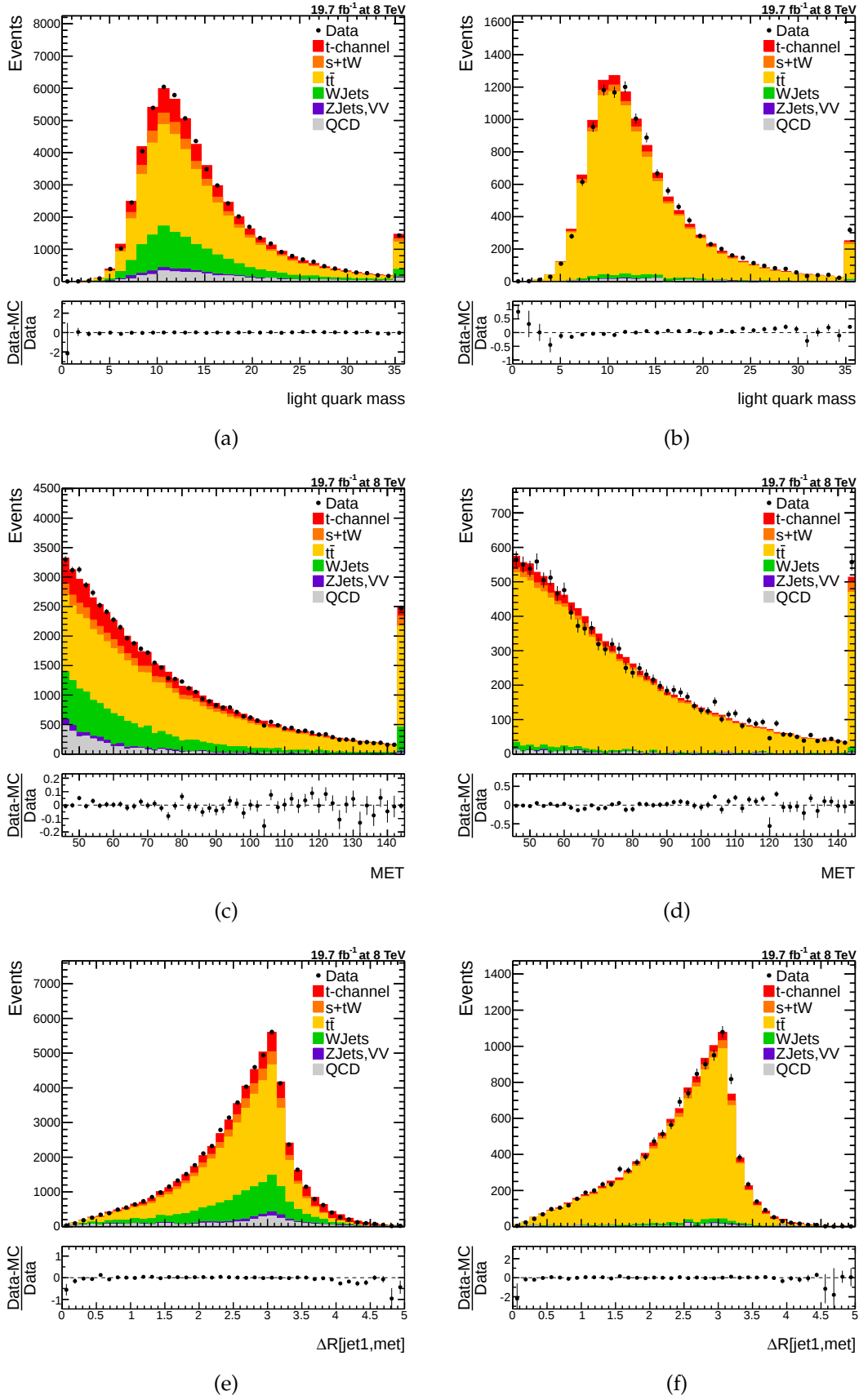
Figure C.11.: Electron channel input variables. m_{lq} , \cancel{E}_T and \Delta R(\text{jet1}, \cancel{E}_T) .
