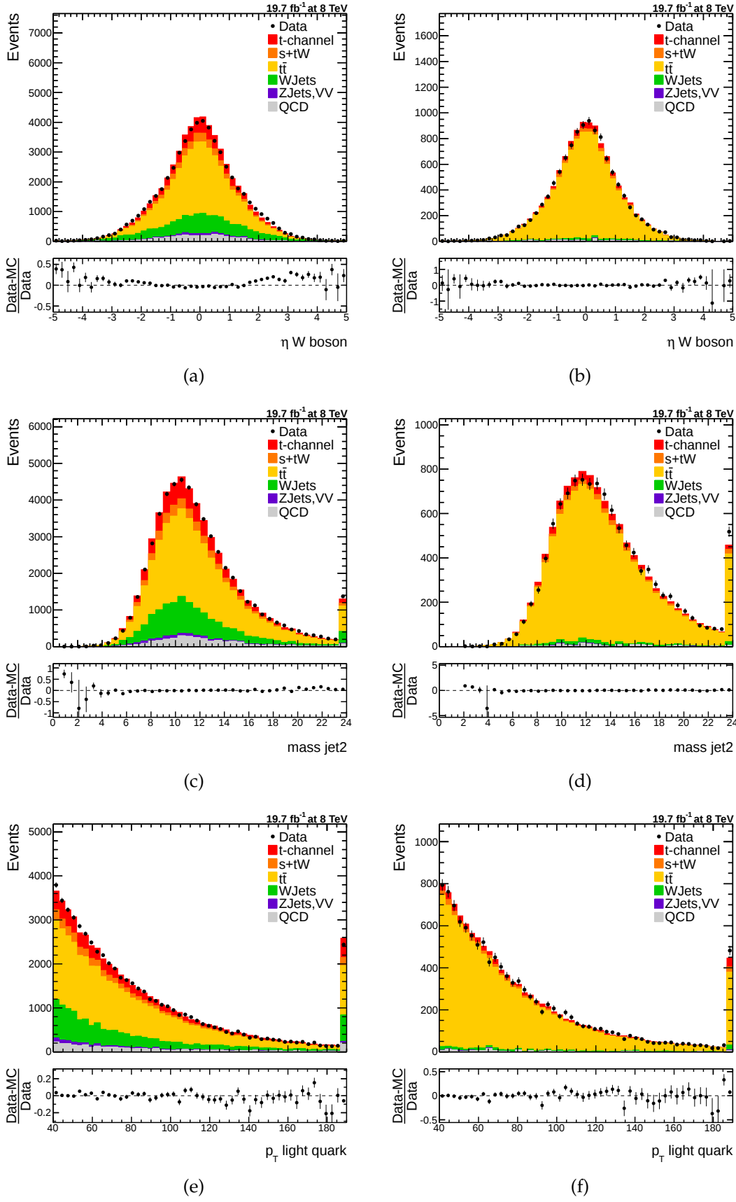
Figure C.9.: Electron channel input variables. \eta_W , m_{\text{jet2}} and p_{T,\text{Lq}} .
