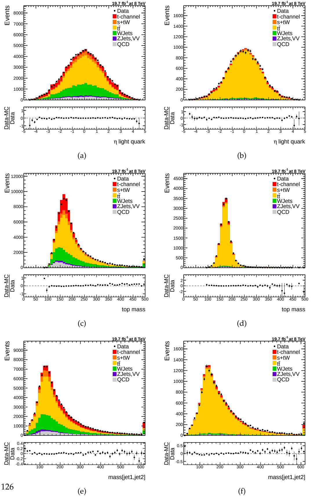
Figure C.1.: Muon channel input variables. \eta_{\text{light quark}} , m_{\ell\nu b} and m_{\text{jet1,jet2}} .
