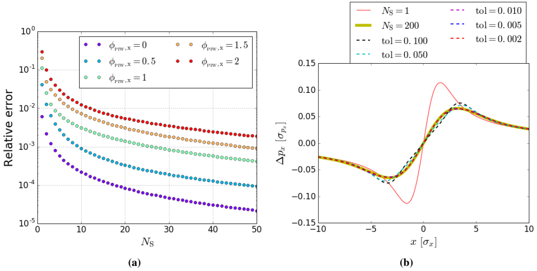
Figure B.5: Dependence on N_S of error in representation of the round beam-beam map. (a) displays the dependence of \text{err}_{N_S} on different values of \phi_{\text{PIW},x} . (b) displays the actual change of p_x for different values of N_S , for particles distributed along the x axis, when \beta_q^* = 40 cm and \phi_{\text{PIW},x} = 2 . The labelled tolerances (in descending order) correspond to N_S = \{3, 4, 13, 22, 48\} .
