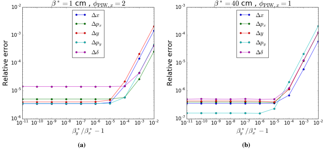
Figure B.2: Relative error between the flat beam-beam map in Hirata's code, as \beta_y^* \rightarrow \beta_x^* , and the round beam-beam map in CABIN, for each coordinate separately. (a) is for \beta_q^* = 1 cm and \phi_{\text{PIW},x} = 2 . (b) is for \beta_q^* = 40 cm and \phi_{\text{PIW},x} = 1 .
