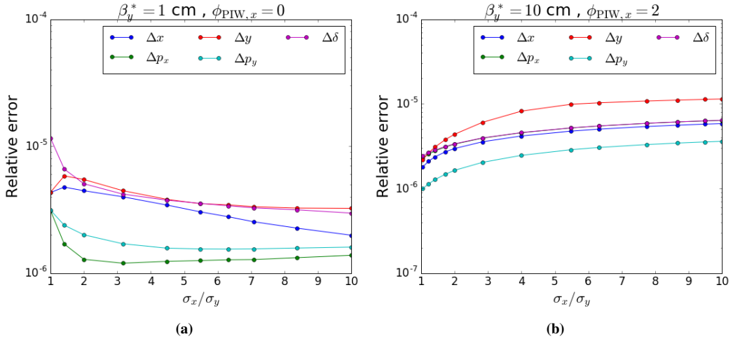
Figure B.3: Relative error between the flat beam-beam map in Hirata's code and CABIN, for different ratios between the two transverse sizes. (a) is for \beta_y^* = 1 cm and \phi_{\text{PIW},x} = 0 . (b) is for \beta_y^* = 10 cm and \phi_{\text{PIW},x} = 2 .
