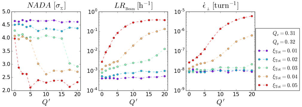
Figure 4.31: Beam quality reduction for multiple combinations of the chromaticity, Q' , and the beam-beam parameter, \xi_{\text{Tot}} , when Q_x = 0.31 , Q_y = 0.32 , \beta_q^* = 4 m and \phi_{\text{PIW}} = 1 . The outputs NADA , LR_{\text{Beam}} and \dot{\epsilon}_{\perp} have been calculated as expressed in Sec. 3.4. The outputs are presented as functions of Q' .
