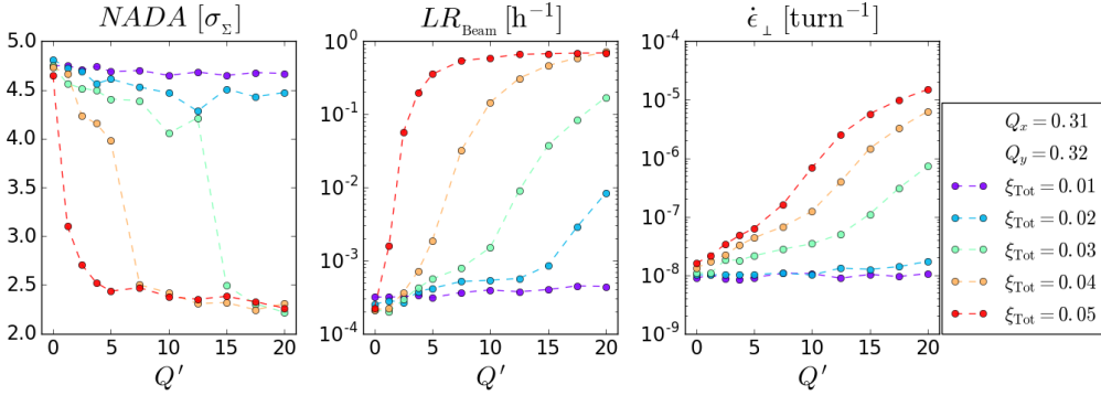
Figure 4.29: Beam quality reduction for multiple combinations of the chromaticity, Q' , and the beam-beam parameter, \xi_{\text{Tot}} , when Q_x = 0.31 , Q_y = 0.32 , \beta_q^* = 4 \text{ m} and \phi_{\text{PW}} = 0 . The outputs NADA , LR_{\text{Beam}} and \epsilon_\perp have been calculated as expressed in Sec. 3.4. The outputs are presented as functions of Q' .
