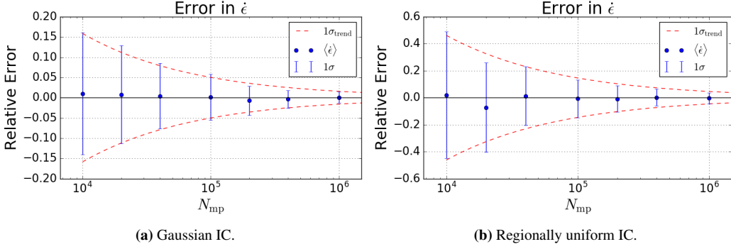
Figure 3.8: Convergence of relative error in measurements of the emittance growth rate, \dot{\epsilon} , for a configuration with only the noise of \Delta = 1 \times 10^{-4} . The relative error has been calculated separately for the Gaussian IC in (a) and the regionally uniform IC in (b).
