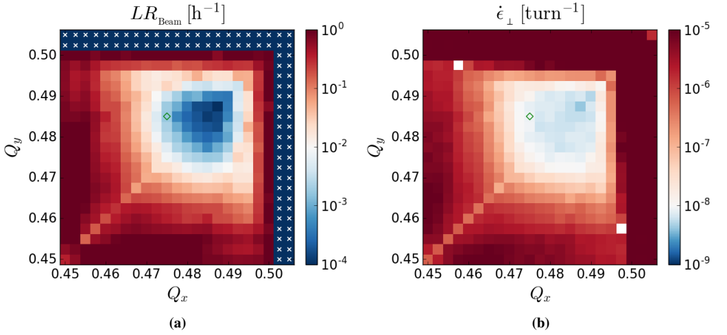
Figure 4.2: Scan in (Q_x, Q_y) space, for \Delta Q_{\text{Tot}}(\phi_{\text{PIW}}) = 0.03 , \beta_q^* = 40 cm, \phi_{\text{PIW}} = 0.9 and Q' = 15 . (a) displays the loss rate per hour and (b) displays the emittance growth rate per turn, calculated as explained in Sec. 3.4. At the working points marked by blue squares with white crosses in (a) , the entire beam was lost before the long-term loss rate could be calculated. The green diamond ( \diamond ) marks a suggested working point in this tune area, (Q_x, Q_y) = (0.475, 0.485) .
