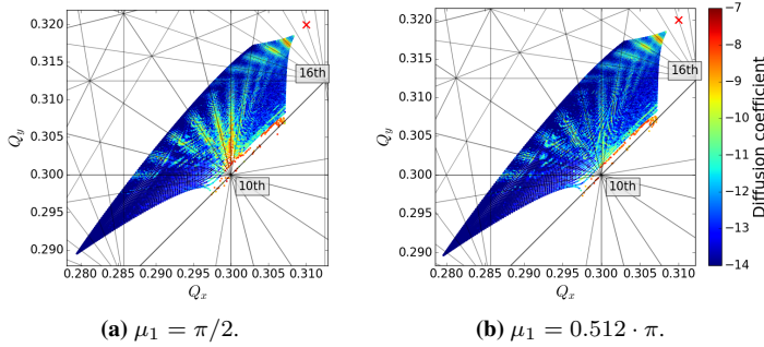
Figure 4.26: FMAs illustrating cancelling of resonances using an intermediate phase advance close to \mu_1 = \pi/2 , for a working point of (Q_x, Q_y) = (0.31, 0.32) , \phi_{\text{PW}} = 0 , Q' = 0 and \xi_{\text{Tot}} = 0.03 . The red cross in each subfigure is the working point in the simulations. Possible resonance lines up to the 16th order have been added, in addition to a few labels meant to guide the reader.
