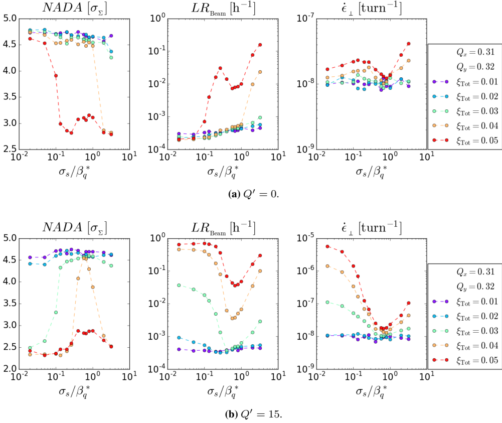
Figure 4.12: Beam quality reduction for different combinations of \beta_q^* and \xi_{\text{Tot}} , when Q_x = 0.31 , Q_y = 0.32 , and \phi_{\text{PW}} = 0 . The outputs NADA , LR_{\text{Beam}} and \dot{\epsilon}_{\perp} have been calculated as expressed in Sec. 3.4 and presented as functions of \sigma_s/\beta_q^* . The chromaticity is Q' = 0 for the scan in (a), and 15 for the scan in (b).
