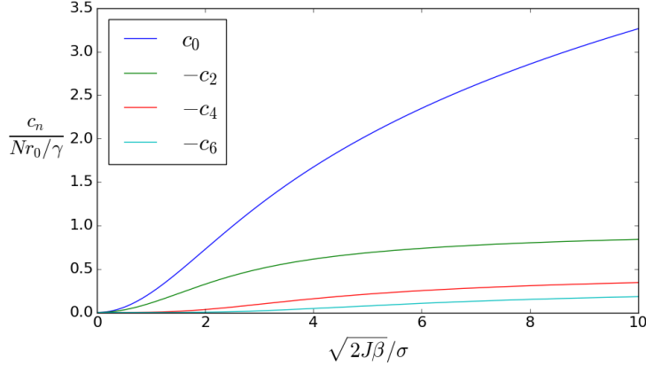
Figure 2.12: Fourier coefficients for the beam-beam potential. The horizontal axis is amplitude in position space in units of the transverse beamsizes \sigma of the strong beam.
