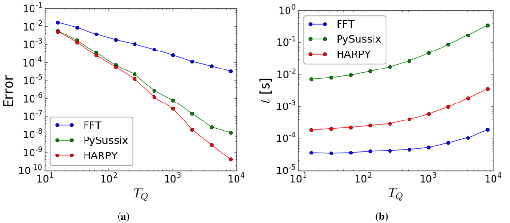
Figure 3.14: Plot comparing the ability of FFT, PySussix [43] and HARPY [45] to calculate tunes. (a) displays the absolute error of the tune calculations. (b) displays the required time to calculate a single tune. T_Q are the number of points used to calculate the tunes, all are powers of 2. 150 tunes have been calculated for each T_Q for each method.
