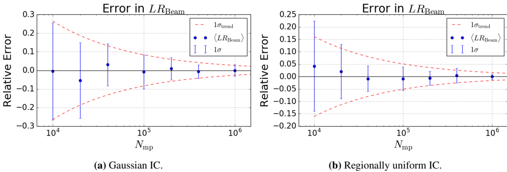
Figure 3.12: Convergence of relative error in measurements of the beam loss rate, LR_{Beam} , for a configuration with (Q_x, Q_y) = (0.31, 0.32) , \Delta = 1 \times 10^{-4} , \xi_{Tot} = 0.03 and Q' = 15 . The relative error has been calculated separately for the Gaussian IC in (a) and the regionally uniform IC in (b).
