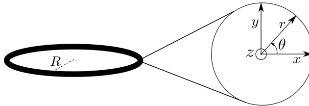
Figure 2.1: Geometry of a large circular collider, in the limit of zero length straight sections and constant beam pipe radius. The transverse plane has its origo in the design orbit, at a radius R from the centre of the collider. Not to scale.
