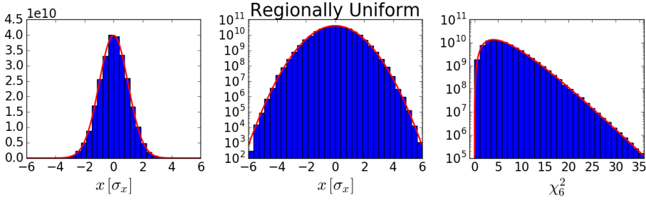
Figure 3.6: Comparison of the regionally uniform initial distribution of N_{\text{mp}} = 1 \times 10^5 macroparticles, with actual Gaussian and \chi^2_6 distributions. The sum of the weight of all particles is N = 1 \times 10^{11} . The first plot from the left displays a histogram of x . The second plot displays the same histogram of x , but with a log-scaled y -axis. The last plot displays a histogram of \chi^2_6 .
