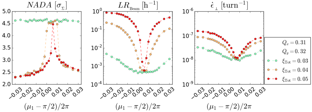
Figure 4.25: Beam quality improvement for intermediate phase advance close to \pi/2 , for different values of \xi_{\text{Tot}} , when Q_x = 0.31 , Q_y = 0.32 , \phi_{\text{PW}} = 0 and Q' = 15 . The outputs NADA , LR_{\text{Beam}} and \dot{\epsilon}_{\perp} have been calculated as expressed in Sec. 3.4. The outputs are presented as functions of the intermediate phase advance.
