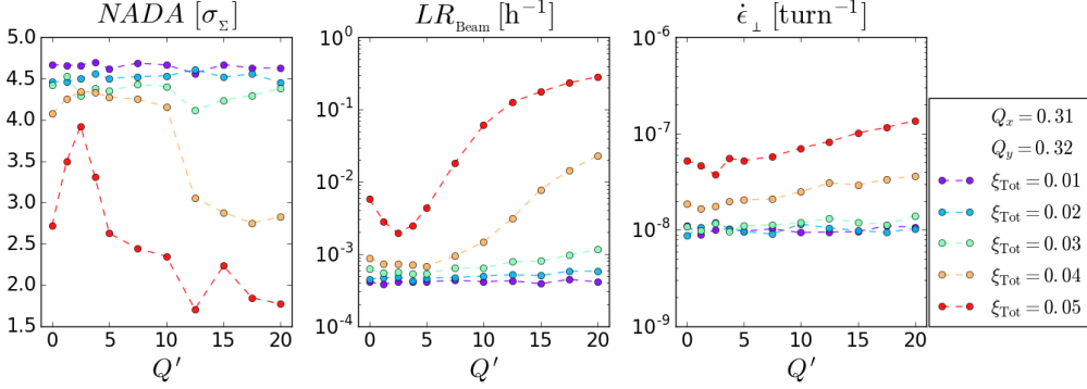
Figure 4.32: Beam quality reduction for multiple combinations of the chromaticity, Q' , and the beam-beam parameter, \xi_{\text{Tot}} , when Q_x = 0.31 , Q_y = 0.32 , \beta_q^* = 12 cm and \phi_{\text{PIW}} = 1 . The outputs NADA , LR_{\text{Beam}} and \epsilon_{\perp} have been calculated as expressed in Sec. 3.4. The outputs are presented as functions of Q' .
