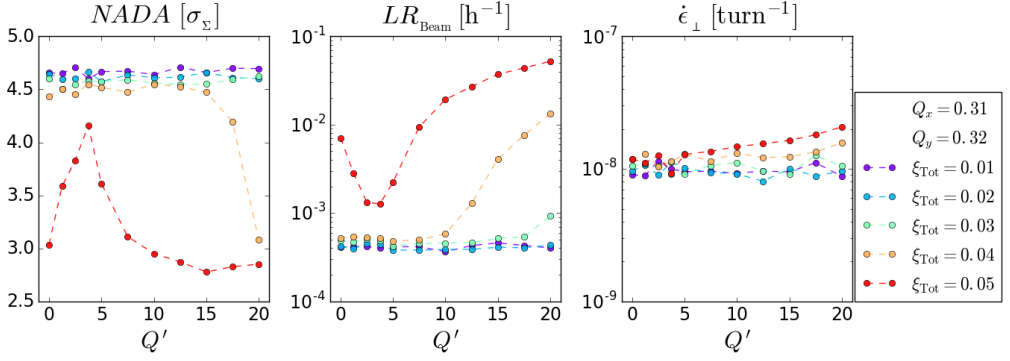
Figure 4.30: Beam quality reduction for multiple combinations of the chromaticity, Q' , and the beam-beam parameter, \xi_{\text{Tot}} , when Q_x = 0.31 , Q_y = 0.32 , \beta_q^* = 12 cm and \phi_{\text{PIW}} = 0 . The outputs NADA , LR_{\text{Beam}} and \dot{\epsilon}_{\perp} have been calculated as expressed in Sec. 3.4. The outputs are presented as functions of Q' .
