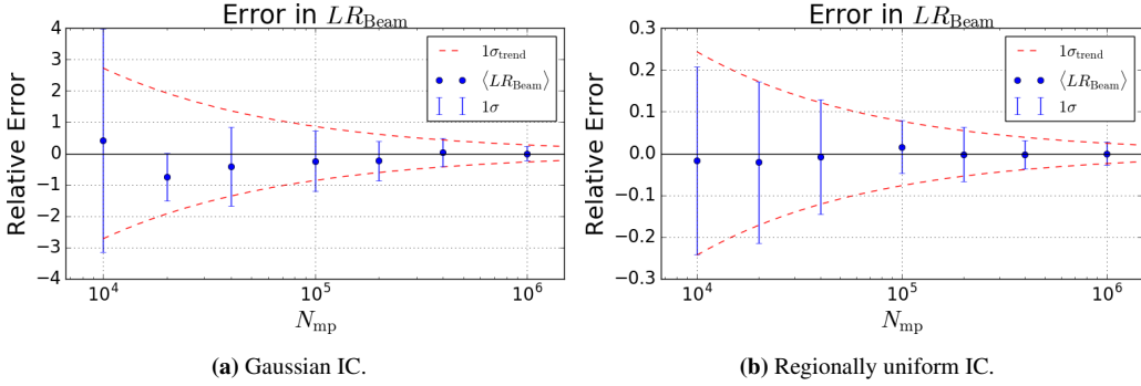
Figure 3.11: Convergence of relative error in measurements of the beam loss rate, LR_{Beam} , for a configuration with a noise of \Delta = 1 \times 10^{-4} only. The relative error has been calculated separately for the Gaussian IC in (a) and the regionally uniform IC in (b).
