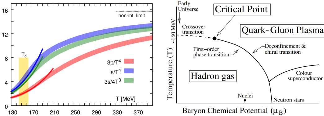
Figure 1.7. Left: Lattice QCD calculations at \mu_B = 0 showing the crossover regime around the critical temperature. The pressure, energy and entropy densities growth reflect an increase in the number of degrees of freedom of the system, which passes from a hadron gas to the deconfined quark and gluons plasma. Image adapted from [21]. Right: QCD phase diagram [22].
