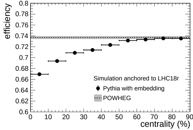
Figure 3.11. Efficiency from embedded proton-proton Pythia-8 simulation as a function of centrality. The comparison with the POWHEG simulation without embedding is added. ★THIS THESIS★
