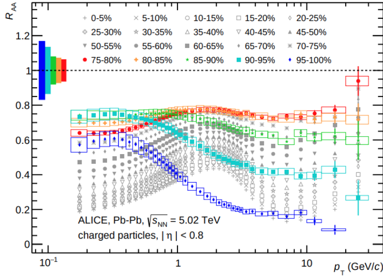
Figure 2.10. Nuclear modification factor for charged particles at midrapidity in Pb-Pb collisions at \sqrt{s_{NN}} = 5.02 TeV [97].
