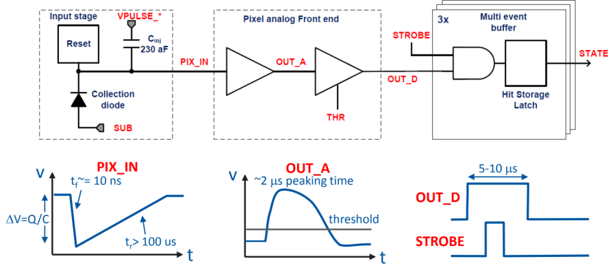
Figure A5. Block diagram of the ALPIDE pixel cell [131].
