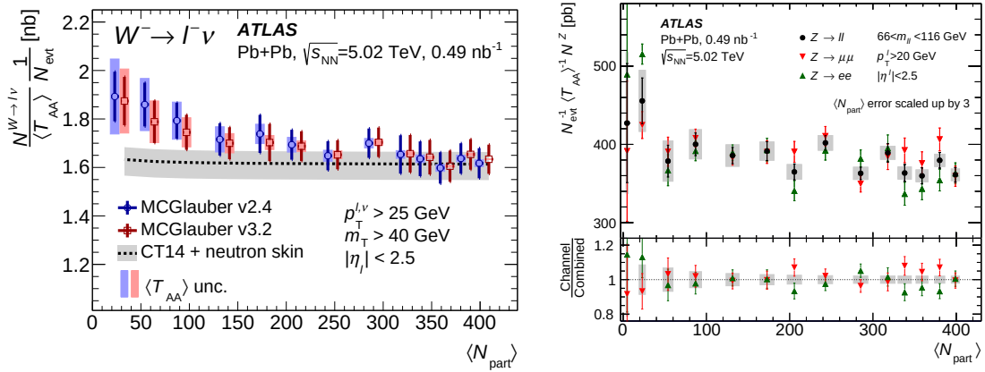
Figure 1.19. W^- (left, [75]) and Z (right, [74]) production yields normalized to the nuclear overlap function \langle T_{AA} \rangle , measured as a function of centrality by ATLAS in Pb-Pb collisions at \sqrt{s_{NN}} = 5.02 \text{ TeV} . The attention should be focused on the enhancement towards more peripheral collisions (lower \langle N_{part} \rangle ). As shown in the papers, the measurements are also systematically above the corresponding EPPS16 predictions.
