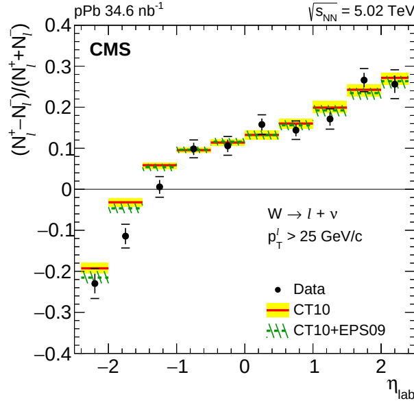
Figure 1.18. Charge asymmetry of muons coming from W boson decay, measured by CMS in p-Pb collisions at \sqrt{s_{NN}} = 5.02 \text{ TeV} [68]. The EPS09 calculations are not flavour-dependent; the deviation from data could be explained as a different nuclear modification of u and d quarks.
