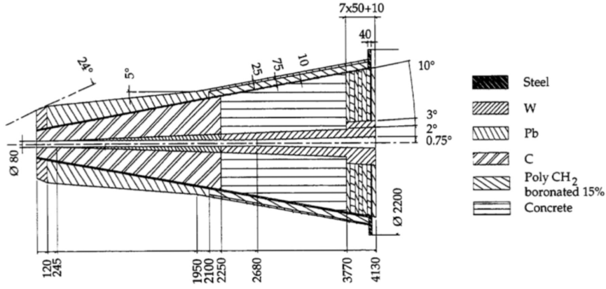
Figure 2.4. The different materials of the front absorber.
