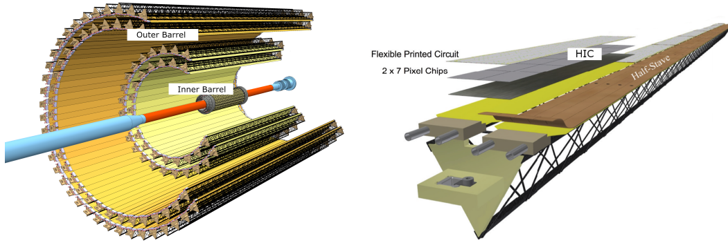
Figure A3. Layout of the new ITS. Left: Geometry of the seven concentric layers arranged in the Inner (layers 0, 1, 2) and Outer (layers 3, 4, 5, 6) Barrel. Right: Outer Barrel stave with exploded view of one of the HICs. Pictures taken from [132] .
