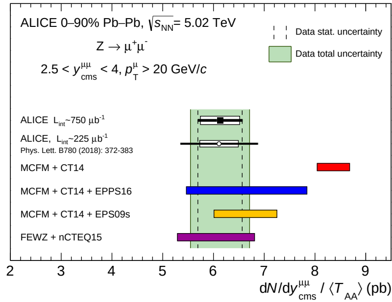
Figure 3.27. Yield of Z/\gamma^* \rightarrow \mu^+ \mu^- normalized by \langle T_{AA} \rangle measured in Pb-Pb collisions at \sqrt{s_{NN}} = 5.02 TeV. The measurement presented in this work is the first data point on the top. The width of vertical dashed band corresponds to the statistical uncertainty, while the filled band is the sum in quadrature of statistical and systematic uncertainties. The colored filled boxes are different theoretical pQCD calculations. The first one (MCFM+CT14) doesn't include nuclear modification to the PDFs and shows a significant deviation from the measurement. (Figure published on [69].)
