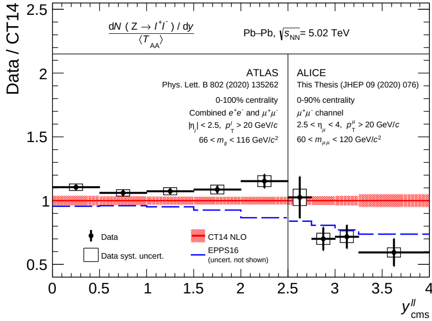
Figure 3.34. Comparison between Z boson normalized yields measured by ATLAS at midrapidity [74] and ALICE at large rapidity in Pb-Pb collisions at \sqrt{s_{\text{NN}}} = 5.02 TeV. pQCD calculations based on CT14 free PDFs are taken as reference for the data/theory ratio. Details on the different fiducial cuts of the two analyses are given inside the figure and in the text. The boxes around unity represent the theoretical uncertainty on CT14 calculations. The uncertainty on the EPPS16/CT14 ratio is not shown. ★THIS THESIS★
