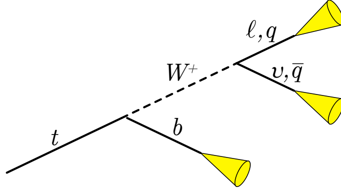
Figure 1: Decay diagram of top quark.
