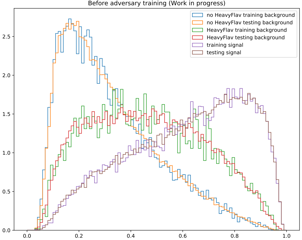
Figure 17: Neural network output distribution before adversary training, normalised.
