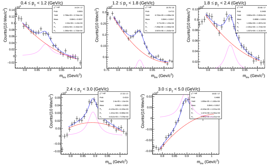
Figure B.12: Invariant mass distribution M_{\pi K} after mixed event background subtraction and fitted with Breit-Wigner + residual background function in centrality class 10–50% for various p_T bins in \cos\theta^* bin 0.8 < \cos\theta^* < 1.0 . Quantization axis is perpendicular to the EP.
