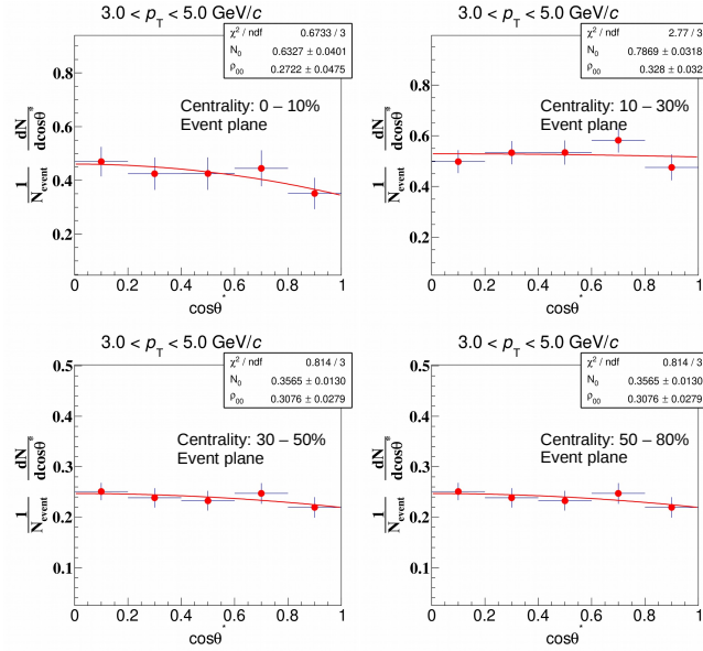
Figure B.49: The efficiency and acceptance corrected \cos\theta^* distribution of K^{*0} decay daughter for 3.0 < p_T < 5.0 GeV/c in different centrality classes of Pb-Pb collisions at \sqrt{s_{NN}} = 2.76 TeV. Measurements are done with respect to normal to the event plane in mid-rapidity.
