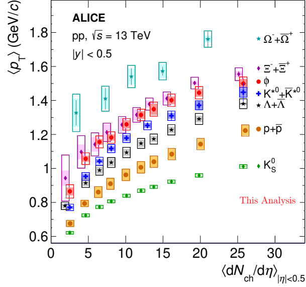
Figure 5.12: \langle p_T \rangle of K_S^0 , p , K^{*0} , \phi , \Lambda , \Xi and \Omega as a function \langle dN_{ch}/d\eta \rangle in pp collisions at \sqrt{s} = 13 TeV [39]. Statistical uncertainties are represented by bars and total systematic uncertainties are represented by boxes. Shaded boxes show the systematic uncertainties that are uncorrelated between multiplicity classes.
