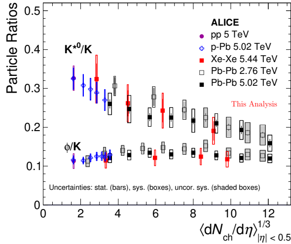
Figure 4.12: K^{*0}/K and \phi/K ratios as a function of \langle dN_{\text{ch}}/d\eta \rangle^{1/3} in pp, p–Pb, Xe–Xe and Pb–Pb collisions [23, 24, 27].
