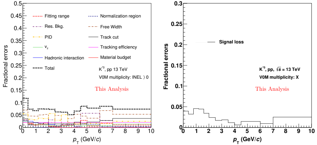
Figure 5.8: Left panel: Systematic uncertainties for K^{*0} in minimum bias pp collisions at \sqrt{s} = 13 TeV. Right panel: Uncertainty due to signal loss correction in 70-100% multiplicity class.
