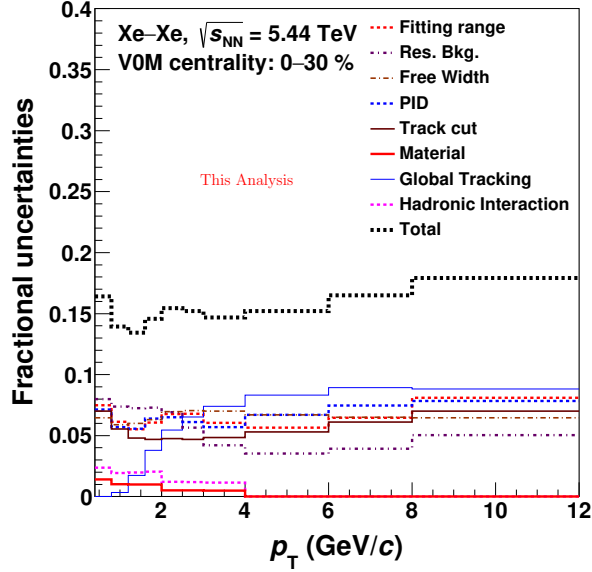
Figure 4.9: Fractional systematic uncertainties from various sources of systematic uncertainties in 0–30% Xe–Xe collisions at \sqrt{s_{\text{NN}}} = 5.44 \text{ TeV} .
