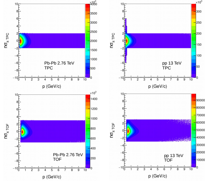
Figure B.2: |n\sigma_{\text{TPC}}| and |n\sigma_{\text{TOF}}| distributions as a function of momentum for selected pion candidates in Pb–Pb collisions at \sqrt{s_{\text{NN}}} = 2.76 TeV and in pp collisions at \sqrt{s} = 13 TeV.
