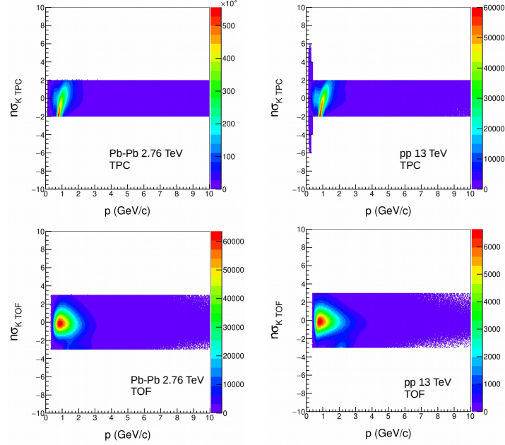
Figure B.3: |n\sigma_{\text{TPC}}| and |n\sigma_{\text{TOF}}| distributions as a function of momentum for selected kaon candidates in Pb–Pb collisions at \sqrt{s_{\text{NN}}} = 2.76 TeV and in pp collisions at \sqrt{s} = 13 TeV.
