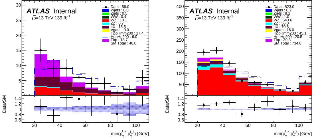
(a) 0 same-flavor-opposite-charge pairs
