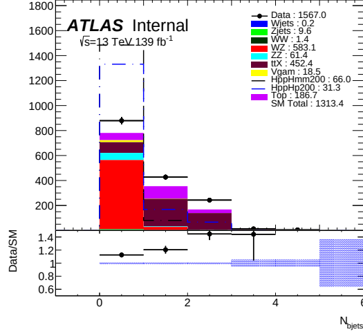
(b) N_{b\text{jets}} distribution (Linear Scale)
