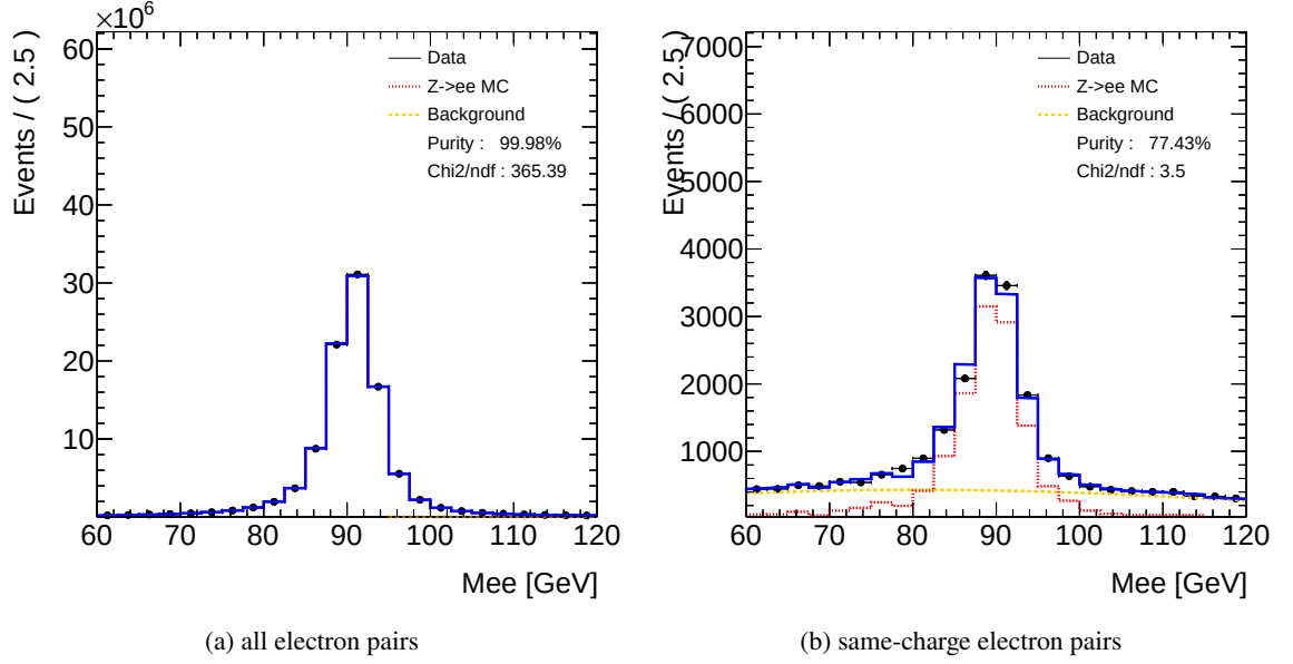
Figure 7.10: SS2L channel. Distributions of the invariant mass of the two signal electron candidates (inclusive p_T and \eta ). Left: all OC+SC events; the signal purity obtained from the fit is 99.98% in central region (80-100 GeV). Right: all SC events; the signal purity obtained from the fit is 77.43% in central region (80-100 GeV). The black dots show the data, the blue dash line is for the fit and the yellow dash line is for the background template.
