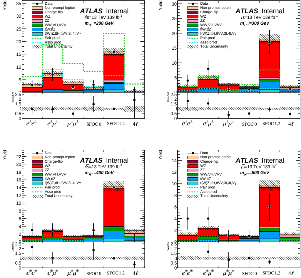
Figure 10.1: 200 GeV - 500 GeV mass point: Signal and background (non-prompt leptons and charge-flip from data-driven estimation) yields in all signal regions. The uncertainty includes all stat. and syst. sources.
