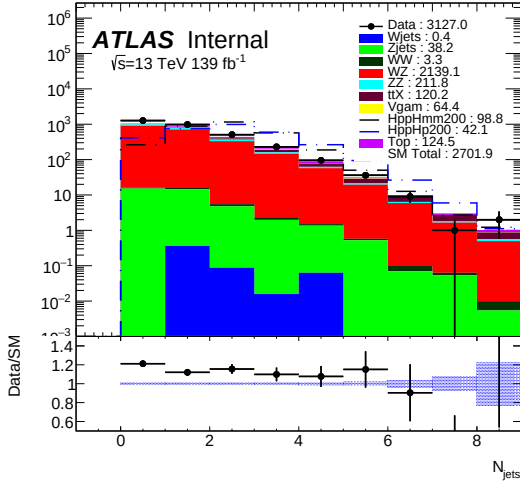
(c) N_{\text{jets}} distribution (Log Scale)
