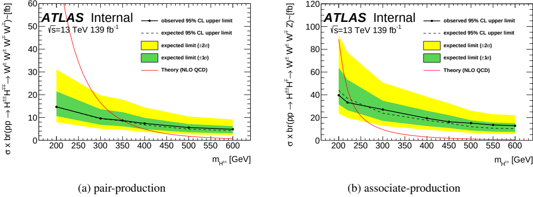
Figure 10.5: Expected and observed limits for the combination of 2\ell^{sc} , 3\ell and 4\ell channels. The benchmark model is observed to be excluded at m_{H^{\pm\pm}} < 350 \text{ GeV} for pair-production and 220 \text{ GeV} for associate-production.
