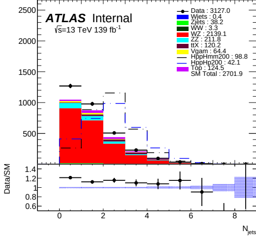
(a) N_{\text{jets}} distribution (Linear Scale)
