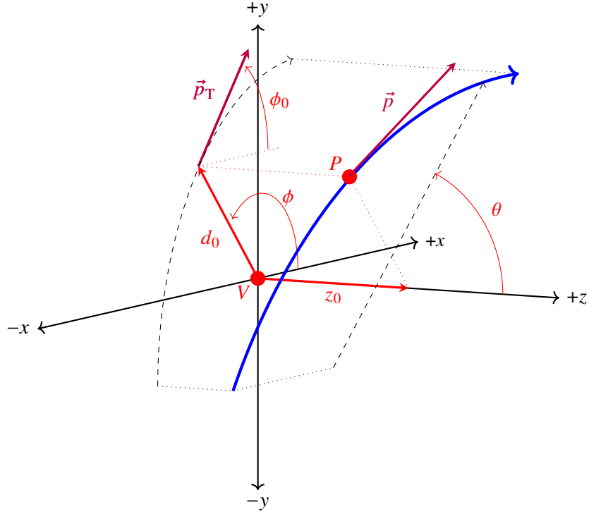
Figure 4.1: Illustration of the five defined track parameters at the perigee. Taken from Ref. [110].
