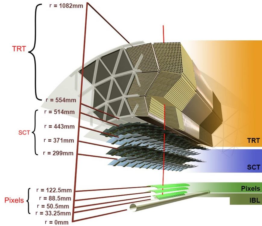
Figure 3.4: Sketch of the barrel region of the ATLAS Inner Detector traversed by a charged track of p_T = 10\text{ GeV} . The beam pipe, the IBL, the Pixel layers, the four cylindrical layers of the SCT and the three layers of TRT barrel modules are shown. Taken from Figure 1 in Ref. [101].
