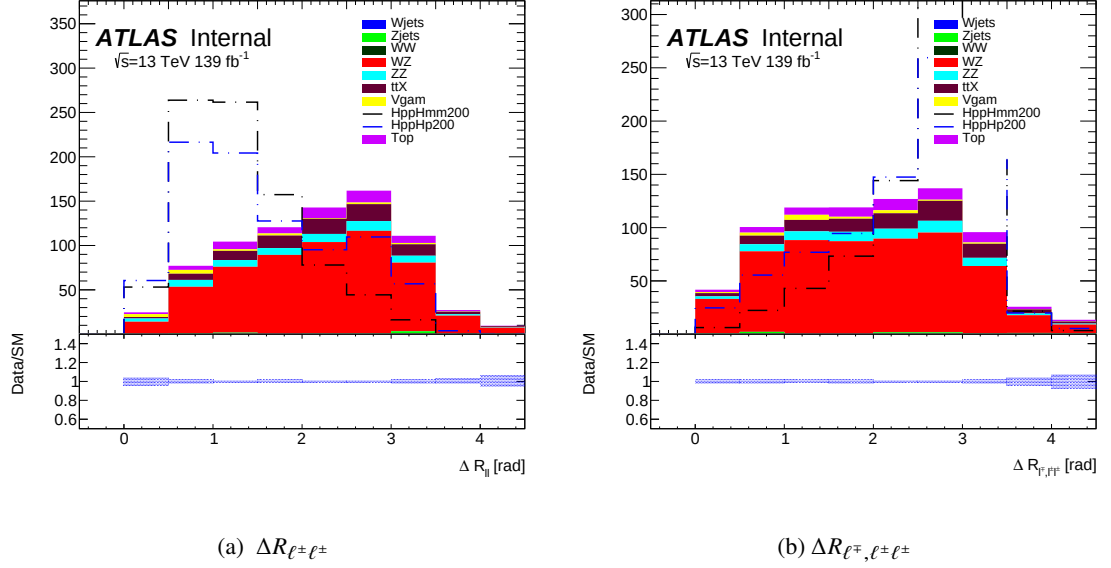
Figure 6.5: 3\ell channel, \Delta R_{\ell^\pm \ell^\pm} and \Delta R_{\ell^\mp, \ell^\pm \ell^\pm} at the event pre-selection stage. Left is the same-charge di-leptons distance in \eta - \phi plane; here the signal tends to be smaller than the SM background. Right is the \eta - \phi distance between opposite-charge lepton and same-charge lepton pair; here the signal tends to become larger than the background. Only the statistical uncertainties are shown. The signal is scaled to the same integral as background MC to have better vision.
