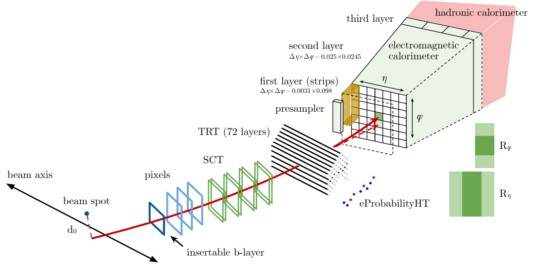
Figure 4.2: A schematic view of the electron reconstruction and identification quantities. The dimensions in this figure are not drawn to scale. Taken from Ref. [119].
