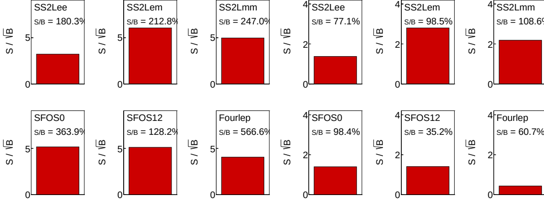
Figure 10.2: m_{H^{++}} = 200 \text{ GeV} signal mass point: The ratio between signal and background (S/B) and the signal significance (S/√B). SFOS0 and SFOS12 are the SFOC0 and SFOC12 channels defined for the 3\ell channel, respectively.
