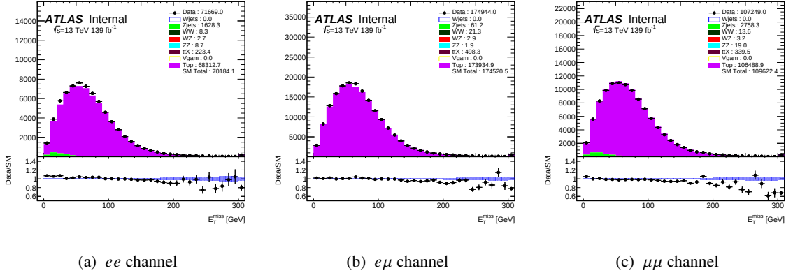
Figure 7.1: E_T^{\text{miss}} of t\bar{t} validation region for ee , e\mu and \mu\mu channels from left to right. Uncertainty is stat only. The non-prompt lepton background is taken from the Monte-Carlo simulations.
