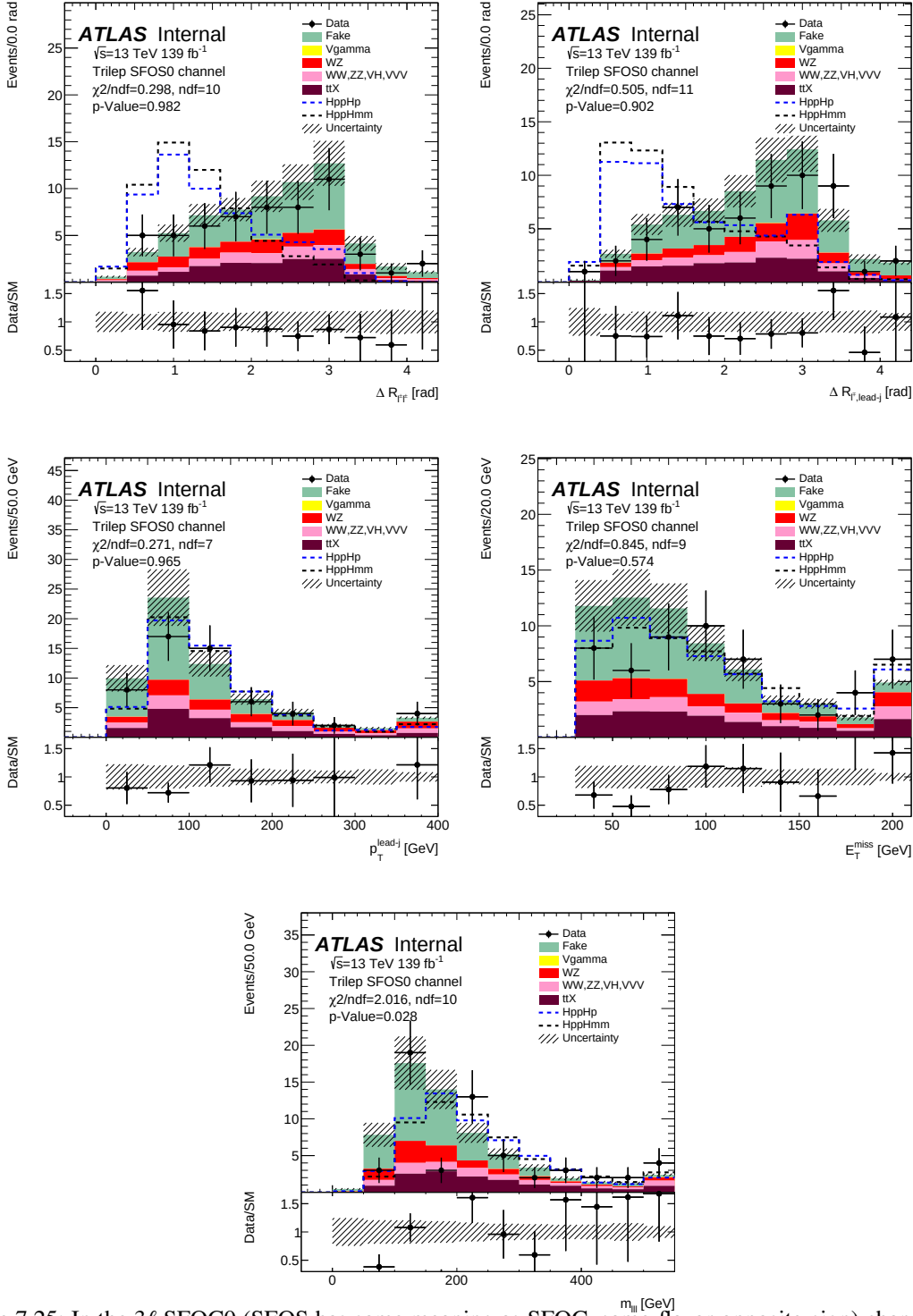
Figure 7.25: In the 3\ell SFOS0 (SFOS has same meaning as SFOC, same-flavor-opposite-sign) channel, the distributions of the 3\ell events included in the pre-selection stage. The variables shown from the left top are the \Delta R between same-sign leptons, \Delta R between the lepton-jet, p_T of the leading lepton, E_T^{miss} and tri-lepton mass. Note that the signal is scaled to data integral. The uncertainty includes the statistic uncertainty and all sources of systematic uncertainties on the background estimation. The non-prompt lepton background is taken from the data-driven method. Two signals points with a mass of 200 GeV are shown.
