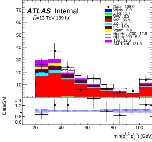
(a) xee channel
