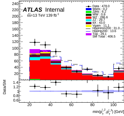
(c) xe\mu channel
