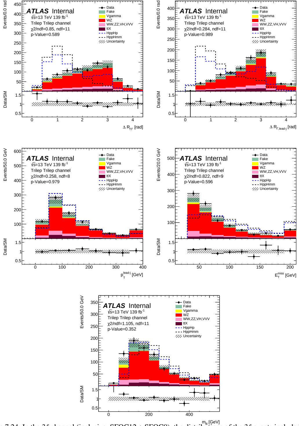
Figure 7.24: In the 3l channel (inclusive, SFOC12 + SFOC0), the distributions of the 3l events included in the pre-selection stage. The variables shown from the left top are the \Delta R between same-sign leptons, \Delta R between the lepton-jet, p_T of the leading lepton, E_T^{miss} and tri-lepton mass. Note that the signal is scaled to data integral. The uncertainty includes the statistic uncertainty and all sources of systematic uncertainties on the background estimation. The non-prompt lepton background is taken from the data-driven method. Two signals points with a mass of 200 GeV are shown.
