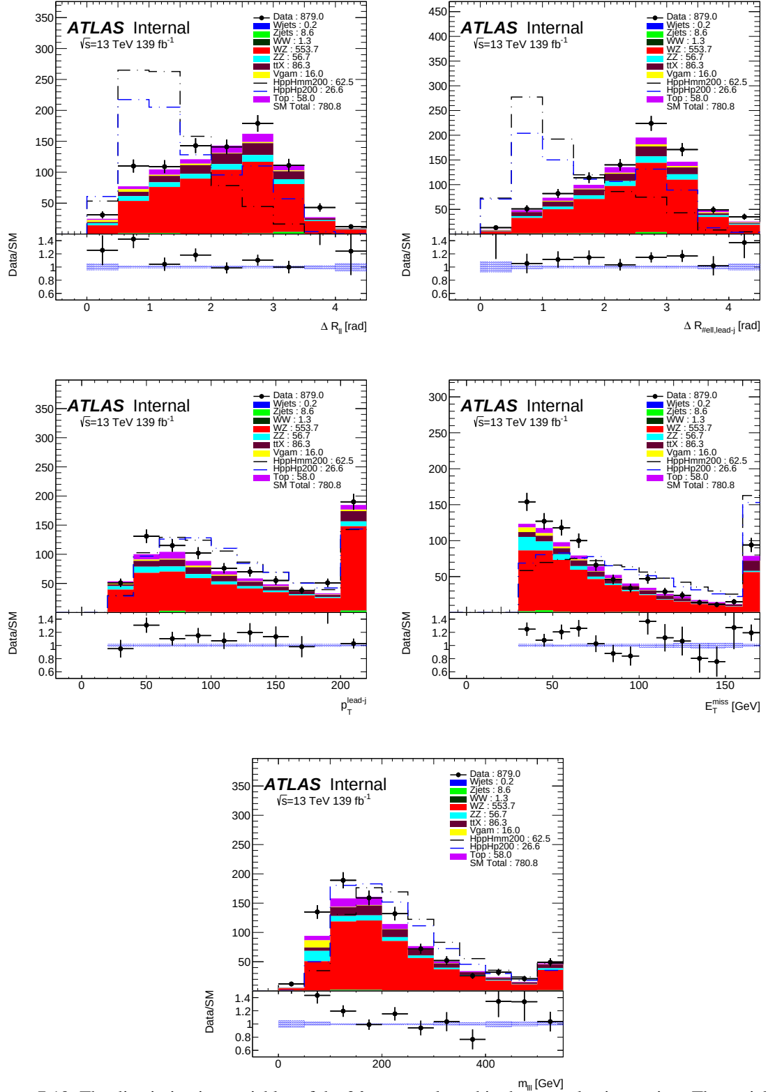
Figure 7.19: The discriminating variables of the 3\ell events selected in the pre-selection region. The variables shown from the left top are the \Delta R between same-charge leptons, \Delta R between the lepton-jet, p_T of the leading lepton, E_T^{miss} and tri-lepton mass. The non-prompt background is taken from the Monte-Carlo simulations. Note that the signal is scaled to data integral. The error band includes only the statistical uncertainty.
