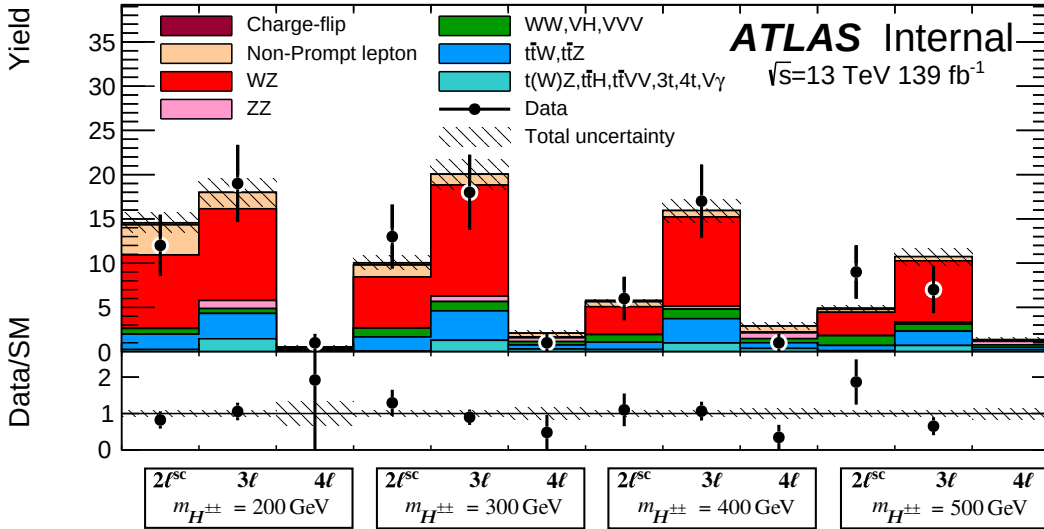
Figure 10.3: Data events yields compared with the expected contributions from relevant background sources, for the combination of the individual channels of the 2\ell^{sc} , 3\ell , and 4\ell SRs, respectively.
