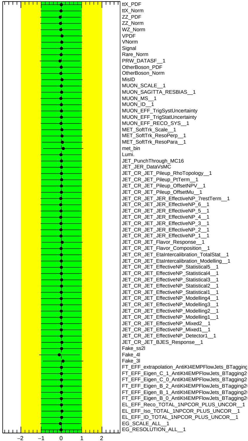
Figure 10.4: The fit values of nuisance parameters. After fitting, all nuisance parameters are kept within one standard deviation.
