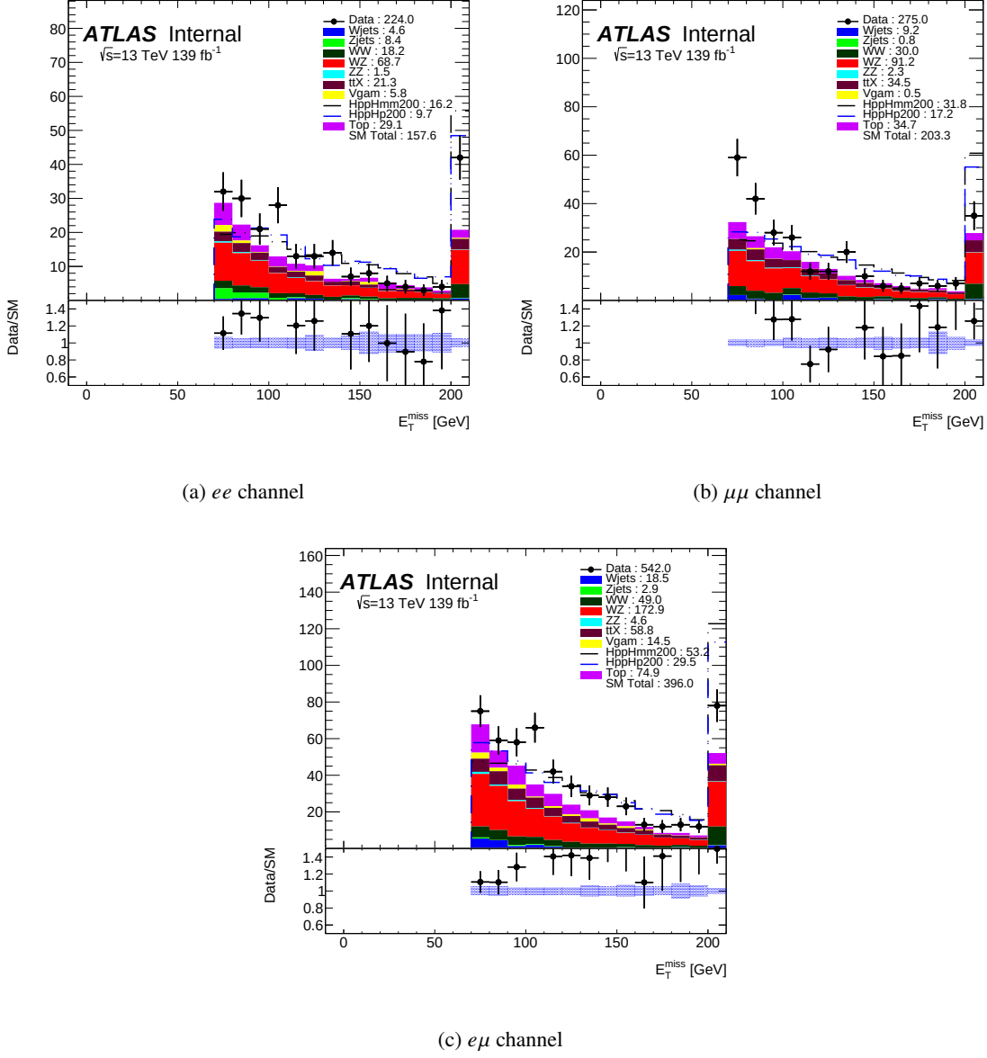
Figure 7.8: 2\ell^{sc} channel: E_T^{\text{miss}} distribution in the ee (Top left), \mu\mu (Top right) and e\mu (Bottom) channels at the event pre-selection stage. Only the statistical uncertainties are shown. The non-prompt lepton background is taken from the Monte-Carlo simulations. The signal is scaled to the same integral as data and that the prediction is given in the legend.
