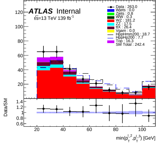
(b) x\mu\mu channel
