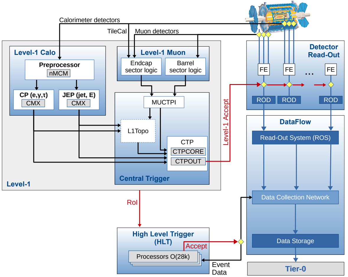
Figure 3.11: The ATLAS TDAQ system with emphasis on the components relevant for triggering. Taken from Figure 1 in Ref. [108].
