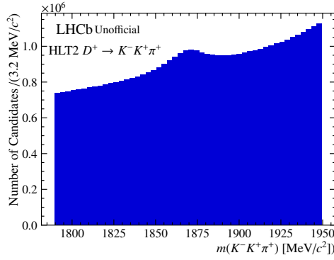
c: Hlt2Charm_DpToKmKpPip_XSec.
