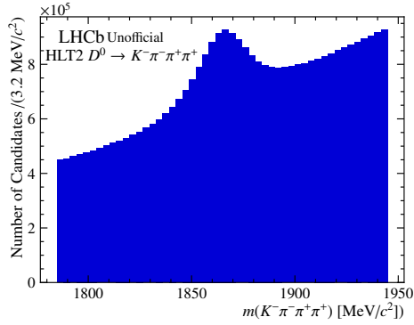
e: Hlt2Charm_D0ToKmPimPipPip_XSec.
