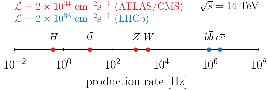
Figure 3.1: Production rates of main particles under study by LHCb and ATLAS/CMS [34].
