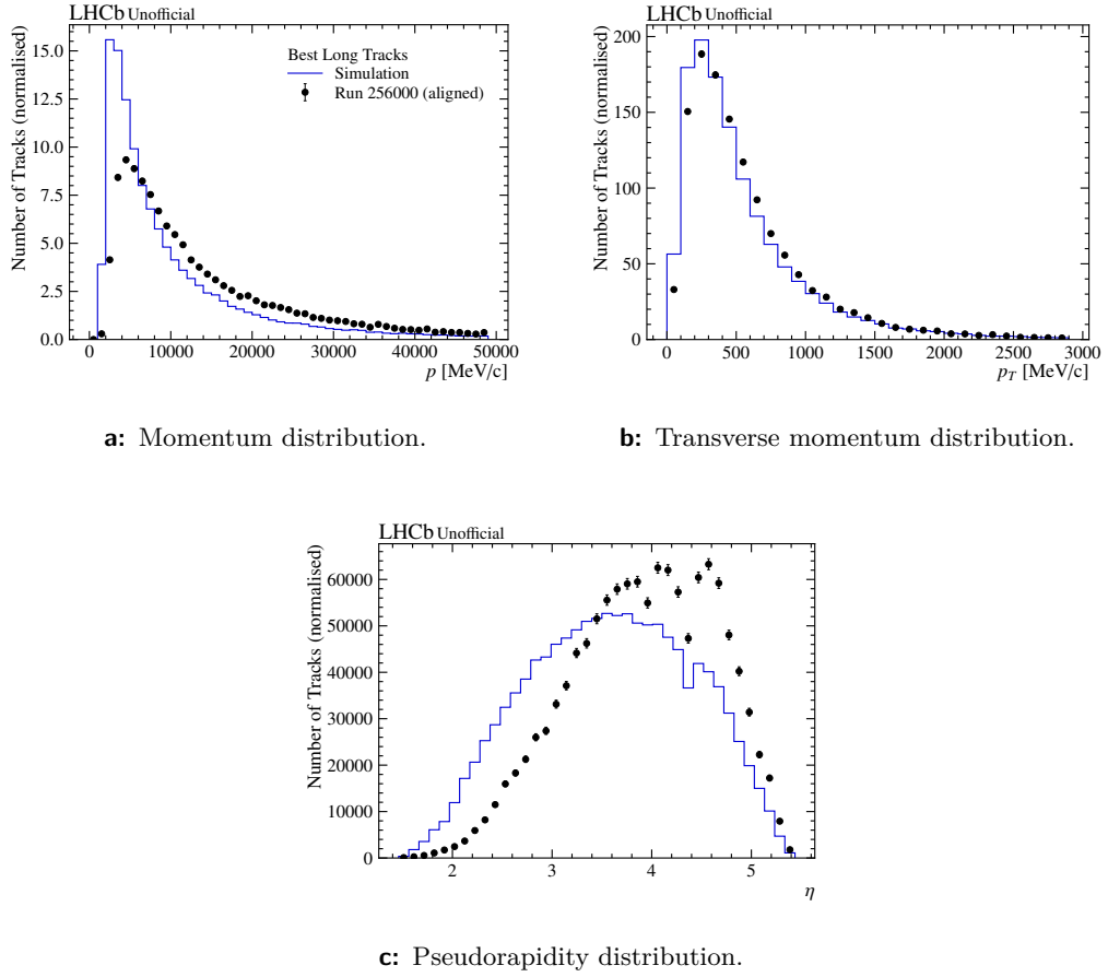
Figure 6.13: Comparison between data taken during Run 256000 with aligned tracking system and simulation for basic kinematic variables
