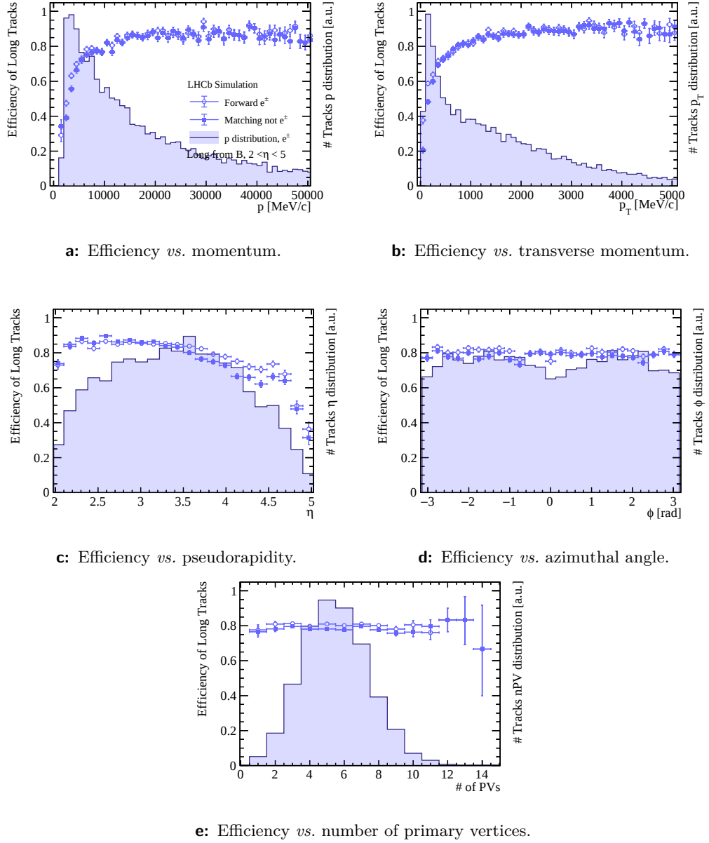
Figure A.12: Electron track finding efficiency of the Forward tracking algorithm with VELO input tracks compared to the Matching algorithm for simulated Long tracks with 2 < \eta < 5 from a B meson in dependence on various kinematic variables and the number of primary vertices. The Matching is shown in full blue rectangles and the Forward tracking is in empty blue circles.
