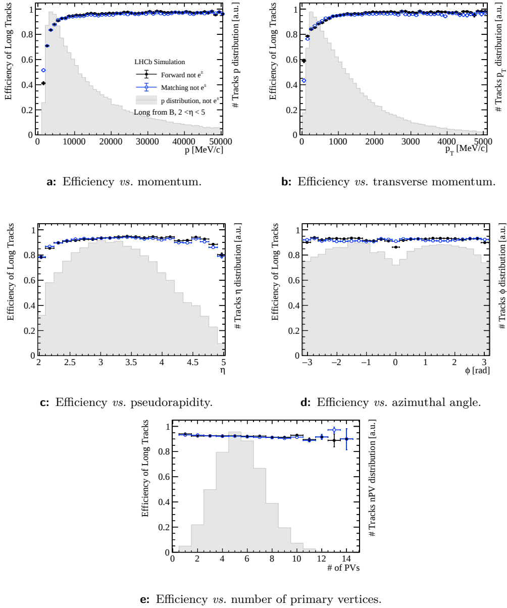
Figure A.11: Track finding efficiency of the Forward tracking algorithm with VELO input tracks compared to the Matching algorithm for simulated Long tracks with 2 < \eta < 5 from a B meson in dependence on various kinematic variables and the number of primary vertices. The Matching is shown in empty blue circles and the Forward tracking is in full black circles.
