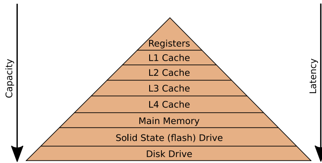
Figure 3.8: Sketch of the cache hierarchy, including CPU registers and larger storage devices ordered with increasing storage capacity and access latency from top to bottom [66].
