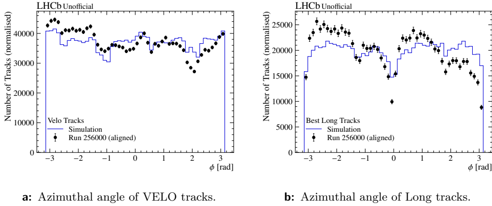
Figure 6.11: Comparison between data taken during Run 256000 with aligned tracking system (black dots) and simulation (solid blue line) using the baseline reconstruction sequence.
