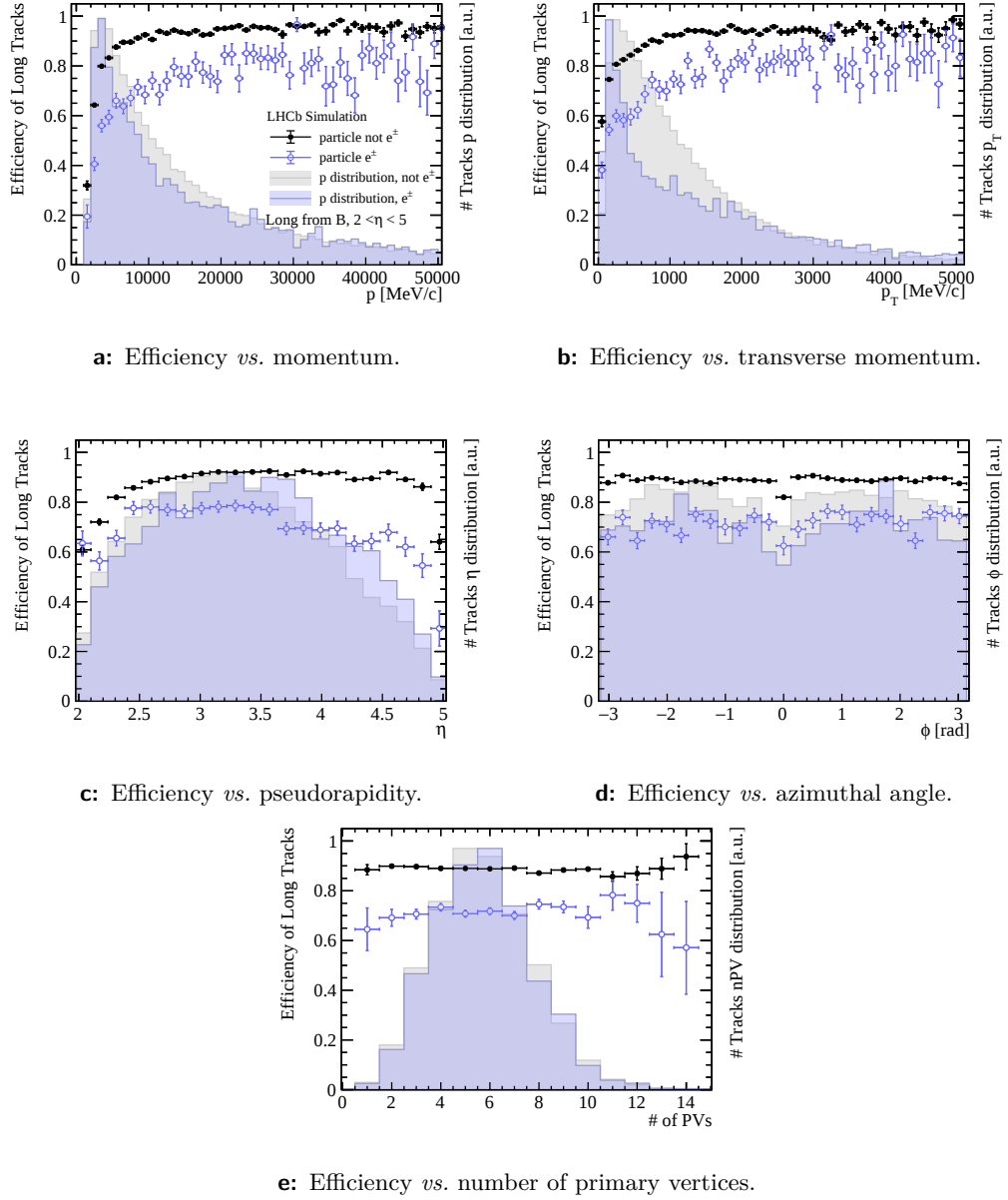
Figure A.4: Track finding efficiency of the Forward tracking algorithm with UT-filtered VELO tracks for simulated Long tracks with 2 < \eta < 5 originating from a B meson in dependence on various kinematic variables and the number of primary vertices. The momentum-dependent search window is applied. The simulated distributions of the variables and the efficiencies are given for reconstructible electrons and other reconstructible particles separately; electrons in blue with empty-circle markers and other particles in black with full-circle markers. The same samples as for the training of the fake track rejection classifier (Section 5.2.8) are used to avoid a specific bug related to UT hit decoding.
