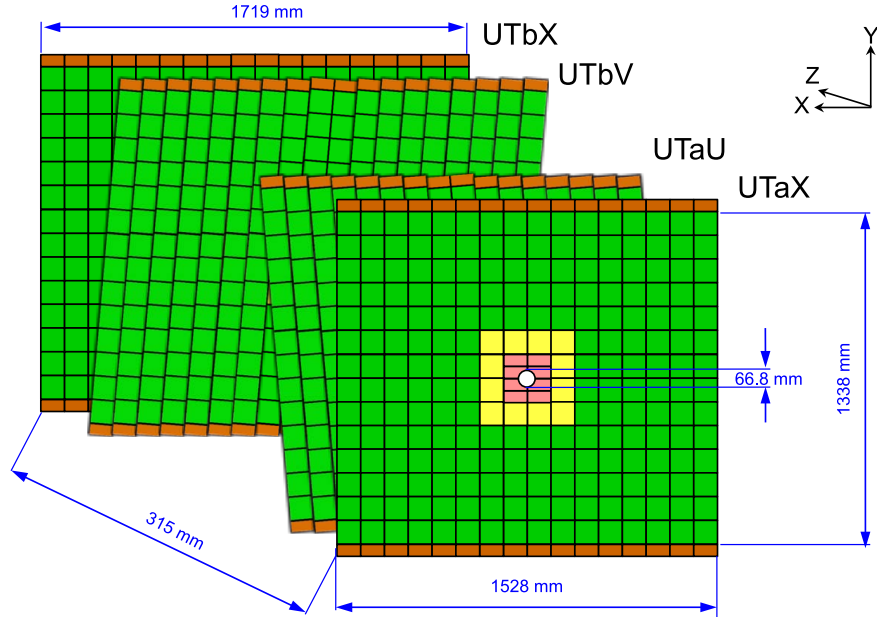
Figure 2.5: Sketch of the four UT silicon planes [19]. Different colours mark sensors with different pitches and lengths: pink sensors in the centre have a pitch of 93.5\text{ }\mu\text{m} at a length of roughly 5 cm, yellow sensors have the same pitch, but twice the length and green sensors have a pitch of 187.5\text{ }\mu\text{m} and are also twice as long the sensors in the centre.
