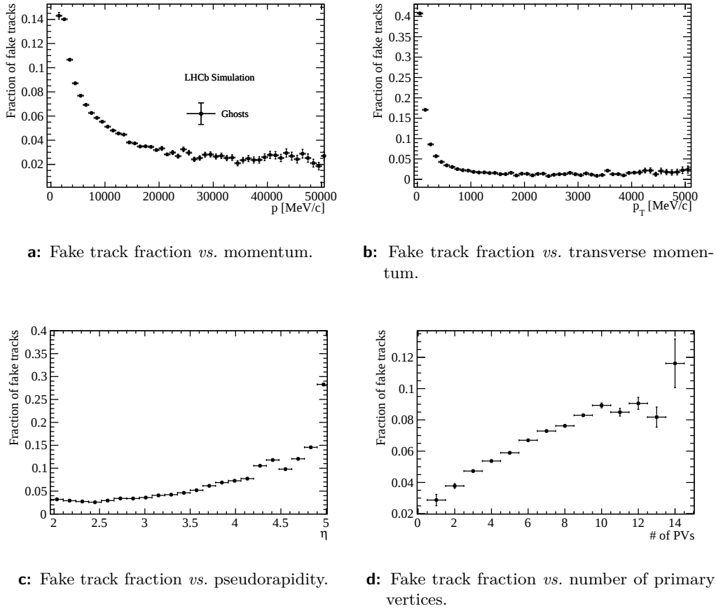
Figure A.5: Fake track fraction of the Forward tracking algorithm with UT-filtered VELO tracks as input in dependence on kinematic variables and the number of primary vertices. The momentum-dependent search window is applied.
