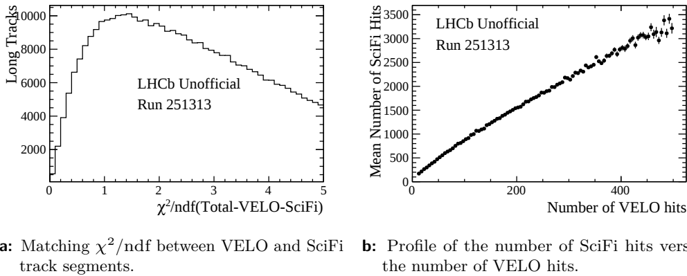
Figure 6.3: Distributions used to commission the track reconstruction. VELO and SciFi detector see the same bunch crossings here.
