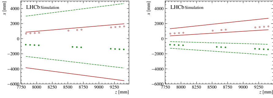
a: Hit search window using minimum-momentum boundary. b: Hit search window using momentum-dependent boundary.
