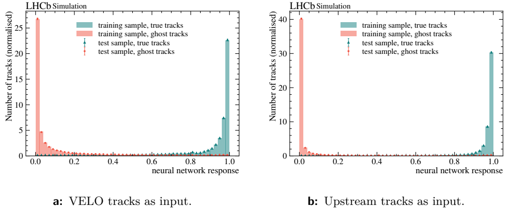
Figure 5.17: Output of the MLPs for the training (bar) and test (data point with error) sample. The distribution of true tracks is green with triangular markers, and the distribution of the fake tracks is red with circular markers.
