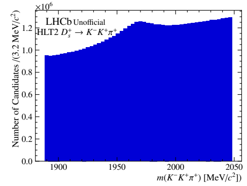
d: Hlt2Charm_DspToKmKpPip_XSec.
