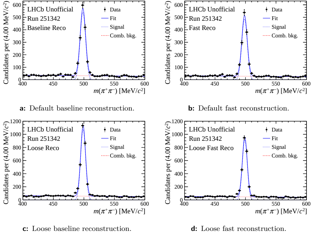
Figure 6.7: Comparison of reconstructed and selected K_S^0 \rightarrow \pi^+ \pi^- decays from the baseline and the fast reconstruction sequence with and without loosened Long tracking configuration as given in Table A.13. All candidates are built using Kalman filtered Long tracks.
