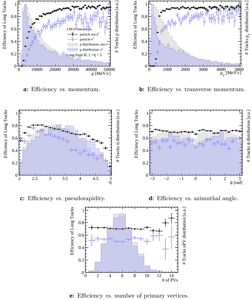
Figure A.6: Track finding efficiency of the Forward tracking algorithm with Upstream tracks for simulated Long tracks with 2 < \eta < 5 originating from a B meson in dependence on various kinematic variables and the number of primary vertices. The momentum-dependent search window is applied. The simulated distributions of the variables and the efficiencies are given for reconstructible electrons and other reconstructible particles separately; electrons in blue with empty-circle markers and other particles in black with full-circle markers. The same samples as for the training of the fake track rejection classifier (Section 5.2.8) are used to avoid a specific bug related to UT hit decoding.
