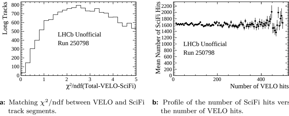
Figure 6.2: Distributions used to commission the track reconstruction. VELO and SciFi detector see different bunch crossings here.
