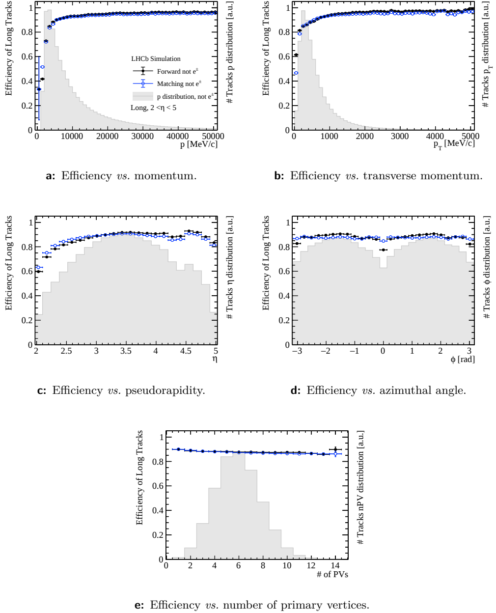
Figure 5.23: Track finding efficiency of the Forward tracking algorithm with VELO input tracks compared to the Matching algorithm for simulated Long tracks with 2 < \eta < 5 in dependence on various kinematic variables and the number of primary vertices. The Matching is shown in empty blue circles and the Forward tracking is in full black circles.
