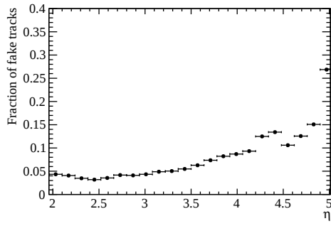
c: Fake track fraction vs. pseudorapidity.
