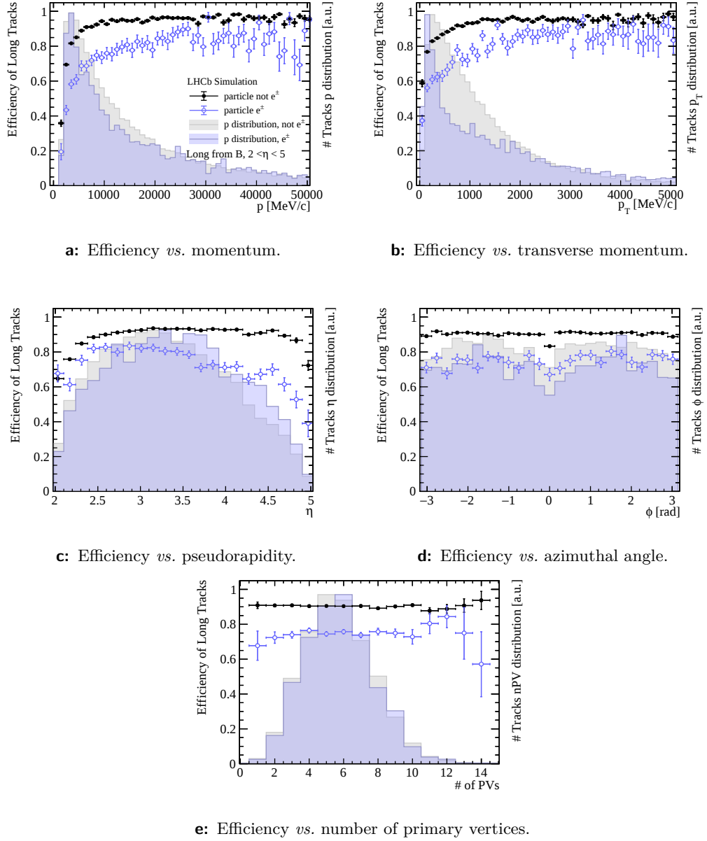
Figure A.2: Track finding efficiency of the Forward tracking algorithm with UT-filtered VELO tracks for simulated Long tracks with 2 < \eta < 5 originating from a B meson in dependence on various kinematic variables and the number of primary vertices. No momentum-dependent search window is applied. The simulated distributions of the variables and the efficiencies are given for reconstructible electrons and other reconstructible particles separately; electrons in blue with empty-circle markers and other particles in black with full-circle markers. The same samples as for the training of the fake track rejection classifier (Section 5.2.8) are used to avoid a specific bug related to UT hit decoding.
