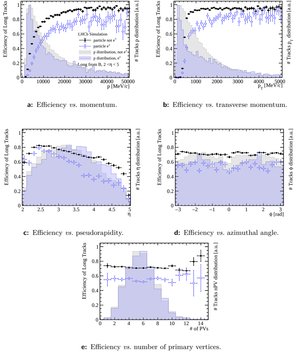
Figure A.8: Track finding efficiency of the Forward tracking algorithm with Upstream tracks for simulated Long tracks with 2 < \eta < 5 originating from a B meson in dependence on various kinematic variables and the number of primary vertices. No momentum-dependent search window is applied. The simulated distributions of the variables and the efficiencies are given for reconstructible electrons and other reconstructible particles separately; electrons in blue with empty-circle markers and other particles in black with full-circle markers. The same samples as for the training of the fake track rejection classifier (Section 5.2.8) are used to avoid a specific bug related to UT hit decoding.
