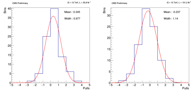
Figure 5.24: Pulls for CR1 as a function of the lepton's charge divided in bins, low mass PFNs and high mass PFNs are combined together. We show the prediction for 2016 separately (left) and for 2017+2018 (right).
