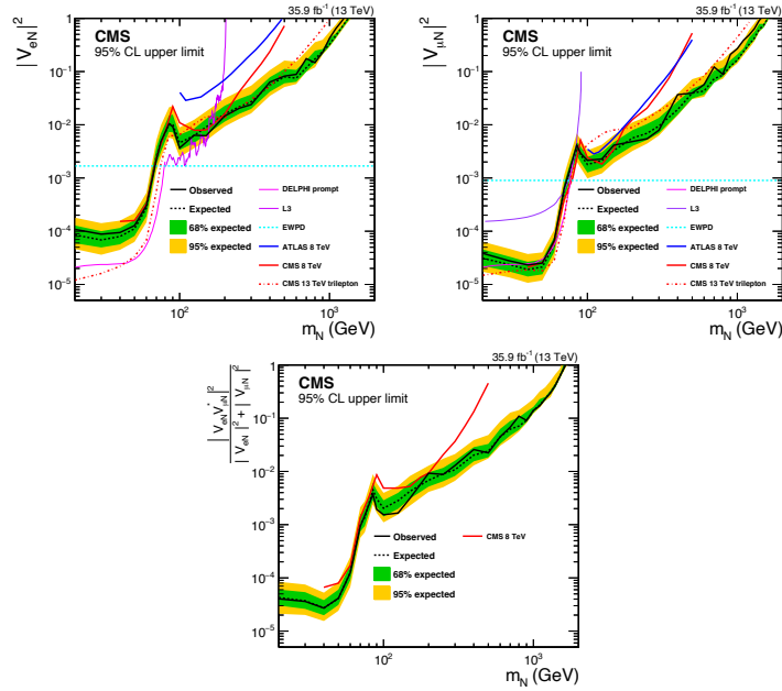
Figure 1.22: Exclusion region at 95% CL in the |V_N|^2 (top-left), |V_N|^2 (top-right) and, |V_{Ne} V_{N\mu}^*|^2 / (|V_N|^2 + |V_N|^2) (bottom) vs. m_N plane [17].
