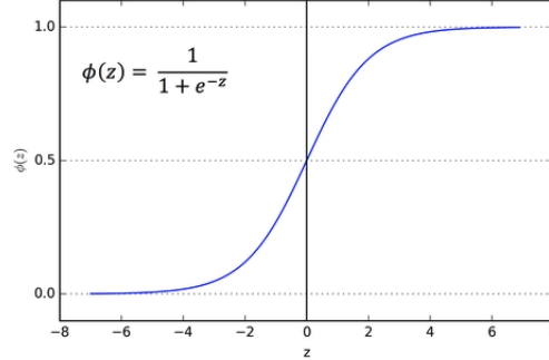
Figure 3.6: Sigmoid function
