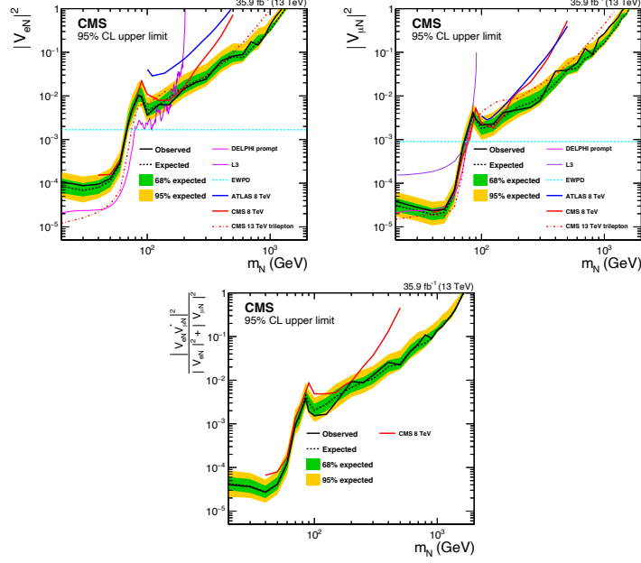
Figure 5.3: Exclusion region at 95% CL in the |V_{eN}| (top-left), |V| (top-right) and, |V_{Ne} V_{N\mu}^*|^2 / (|V_N|^2 + |V_{\nu}|^2) (bottom) vs. m_N plane [17].
