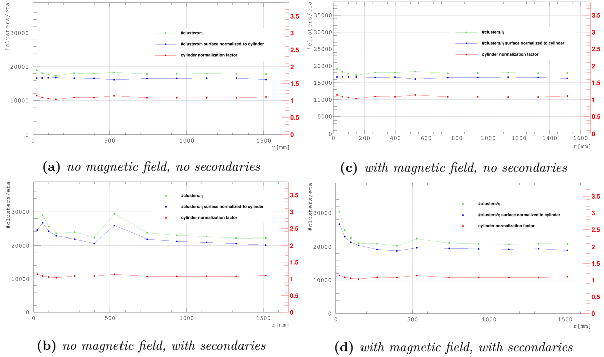
fig. A.13: Each point displays the number of cluster-measurements for the muon case divided by the \eta -coverage of each barrel layer, plotted against the barrel layer's radial position. Four different variations are shown: turning on/off the magnetic field and including/excluding secondary particles produced in the detector during simulation. The green line shows the pure value, while the blue line shows the values, when dividing by the surface normalization factor (accounting for overlap) of each layer. The factor, which corrects for overlap, is displayed in red, with the corresponding axis labels on the right in red.
