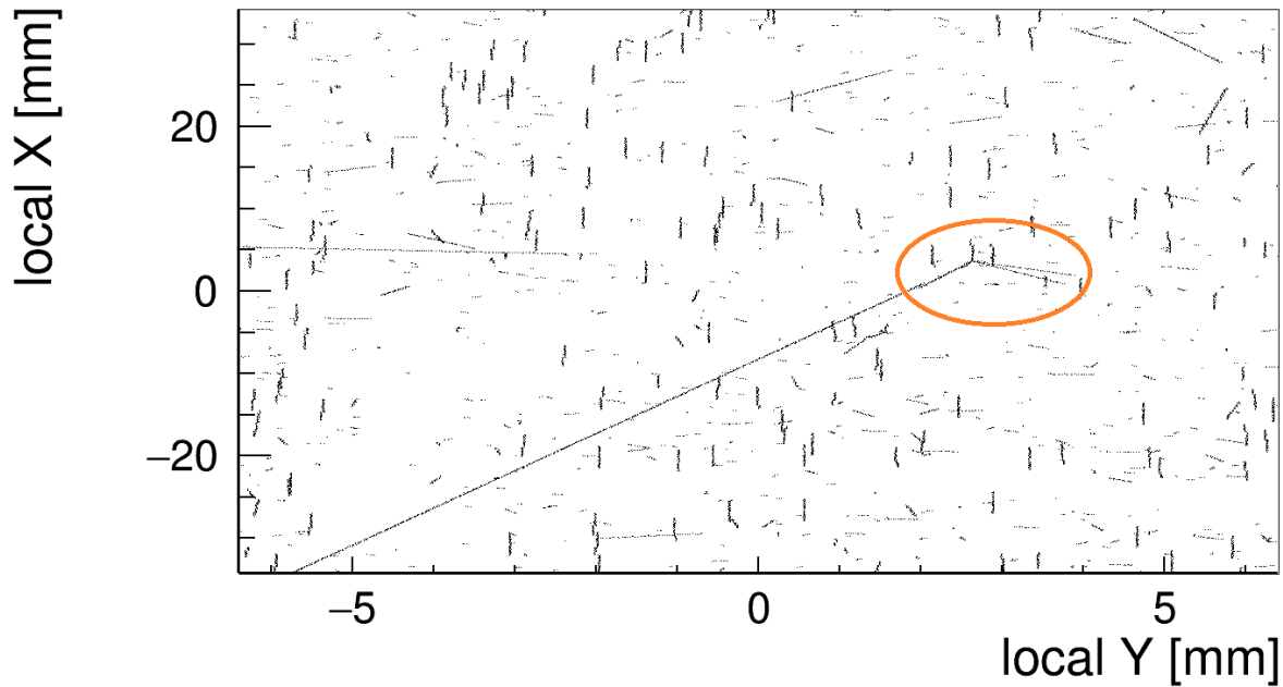
fig. 4.7: Activated cells in a module in the outermost ring of the first barrel layer at 100 TeV and \langle \mu \rangle = 1000 . The orange ellipse highlights a hadronic interaction occurring in the sensitive detector module, after a particle traversed a significant amount of material.
