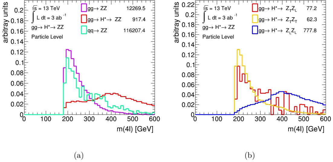
Figure 6.7.: Distribution of the invariant mass of the four lepton system. Each distribution is normalised to unity. (a) shows the distribution of the background processes gg \rightarrow ZZ , qq \rightarrow ZZ , and the signal process gg \rightarrow H \rightarrow ZZ respectively. (b) shows the distribution of the different polarisation states of the signal process.
