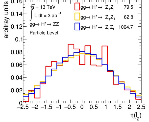
(b) \eta(\ell_2)
