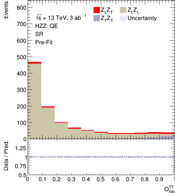
(a) Signal Region
