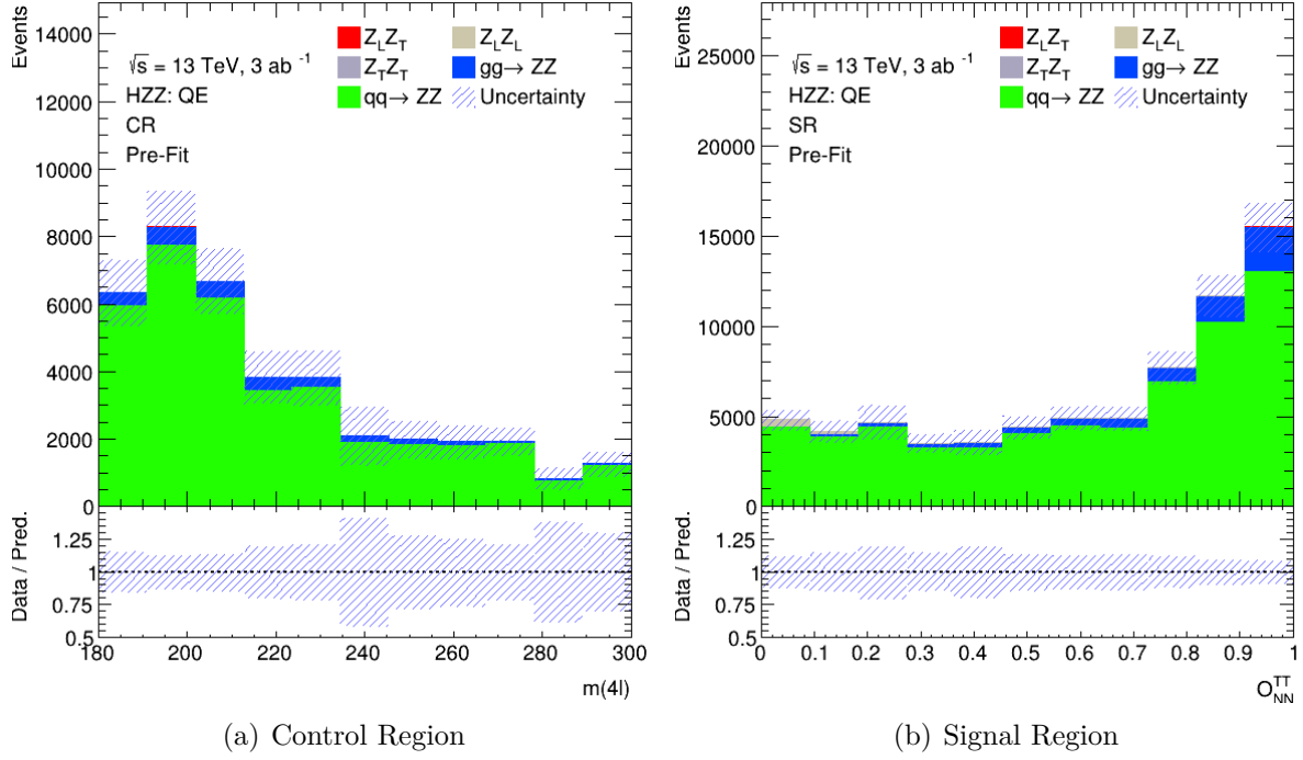
Figure A.2.: Plots of signal and control region with background scaling 0.75.
