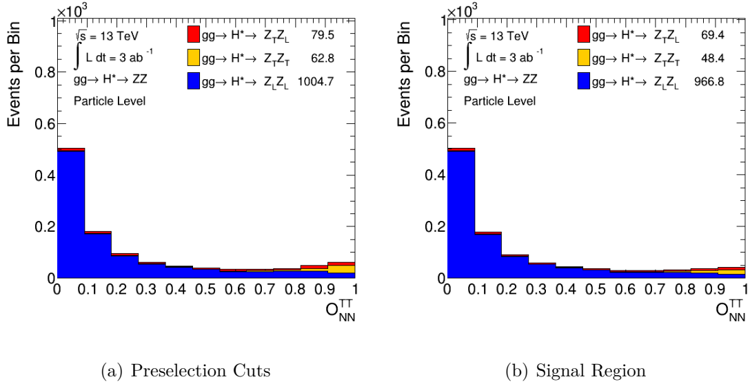
Figure 6.4.: The distribution of O_{NN}^{TT} for the gg \rightarrow H^* \rightarrow ZZ process (a) with only preselection cuts and (b) in the signal region.
