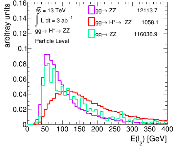
(b) E(\ell_2)
