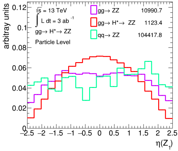
(c) \eta(Z_1)
