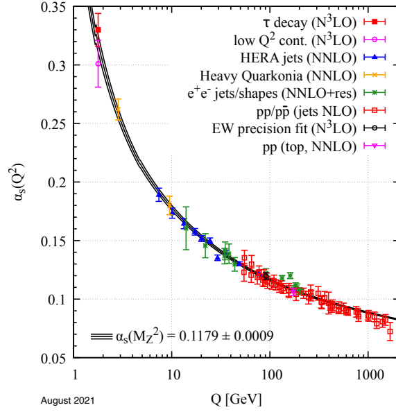
Figure 2.2.: Summary of measurements of \alpha_s as a function of the energy scale Q . The Measurements were performed by various groups [21–24]. The figure is taken from [1].
