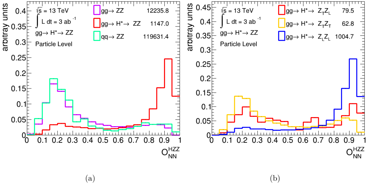
Figure 6.1.: The output variable of the event selection DNN O_{NN}^{HZZ} for the signal and background contribution in (a) and the different polarisation states of gg \rightarrow H^* \rightarrow ZZ in (b). Each distribution is normalised to unity.
