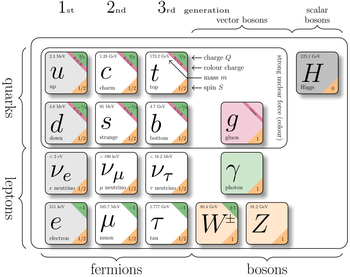
Figure 2.1.: Particles of the Standard Model of particle physics. The figure was created using data from [1].
