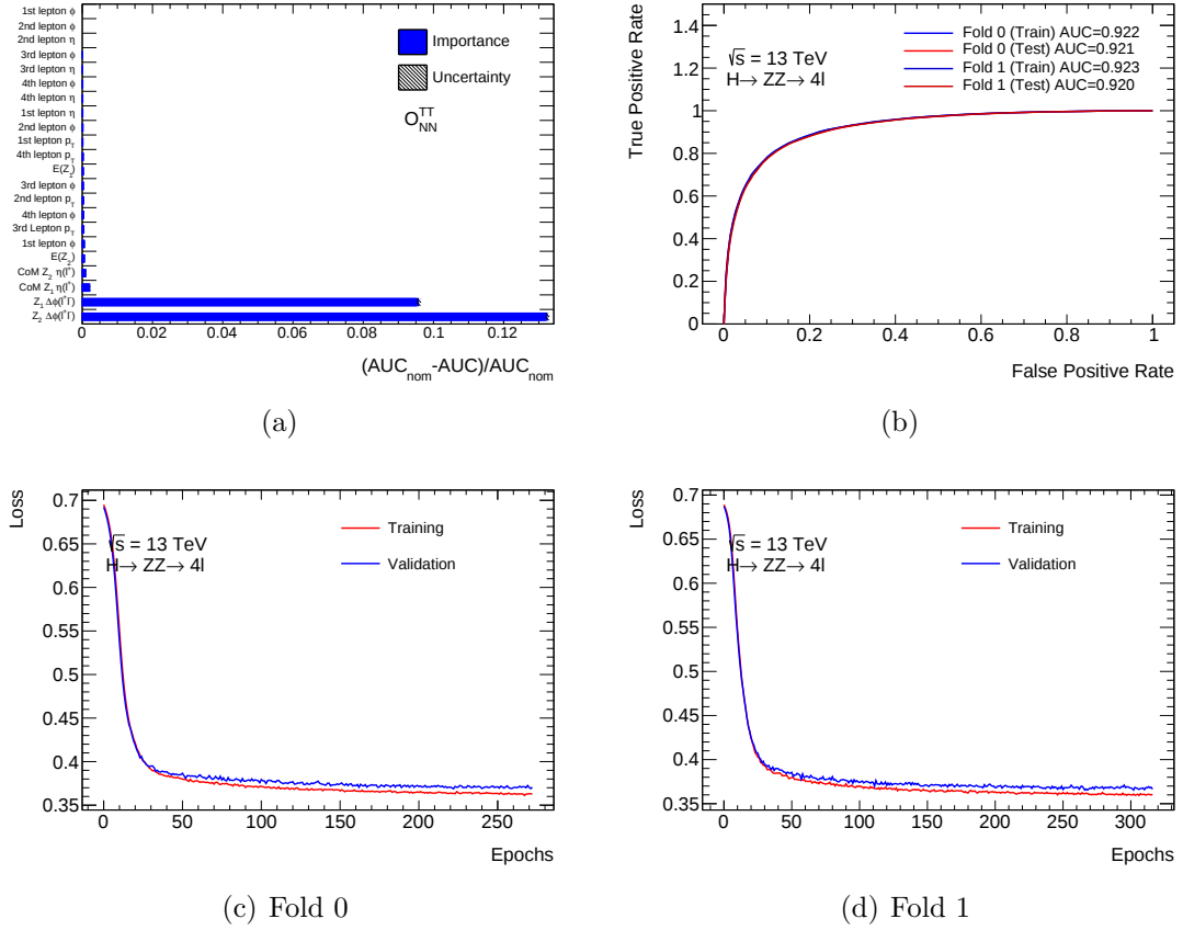
Figure 6.5.: Evaluation plots for the DNN of O_{NN}^{TT} . Figure (a) shows the permutation importance of the input variables, which is a measure of the contribution of the variable on the output calculated by the DNN. Figure (b) shows the ROC curves for validation and training for the two folds. Figure 6.5(c) and 6.5(d) show the loss value over the course of the training of the DNN for the two folds.
