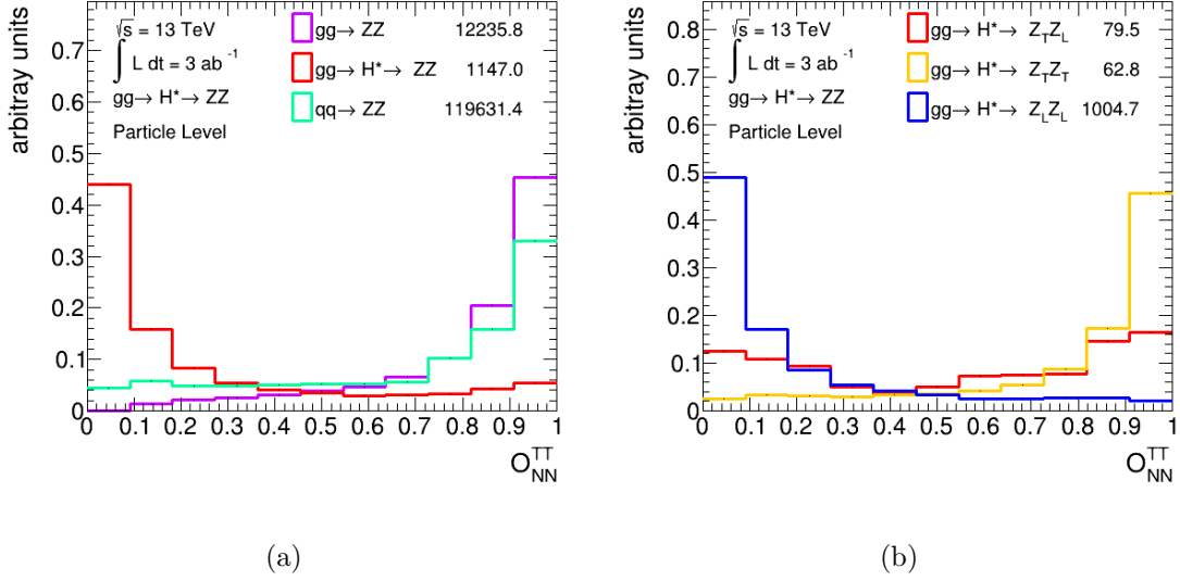
Figure 6.3.: The output variable of the event selection DNN O_{NN}^{TT} for the signal and background contribution in (a) and the different polarisation states of gg \rightarrow H^* \rightarrow ZZ in (b). Each distribution is normalised to unity.
