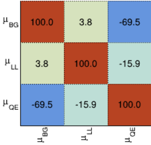
(c) Background scaling 0.5
