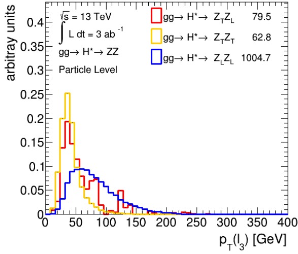
(c) p_T(\ell_3)
