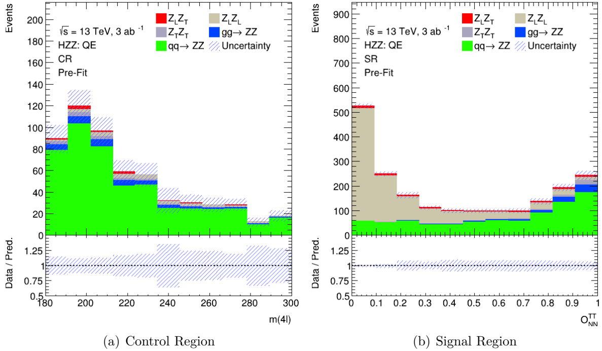
Figure A.7.: Plots of signal and control region with background scaling 0.01.
