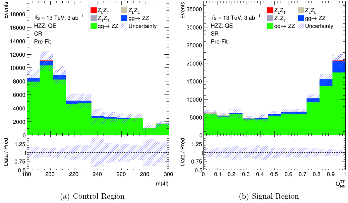
Figure A.1.: Plots of signal and control region with background scaling 1.00.
