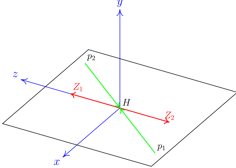
Figure 2.5.: Depiction of the reference system used in this analysis.
