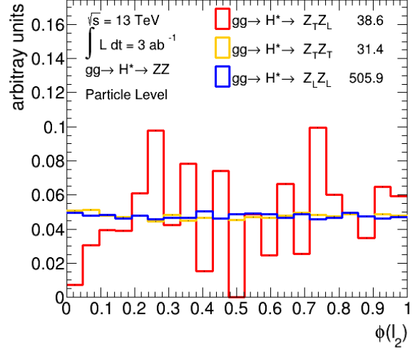
(b) \phi(\ell_2)
