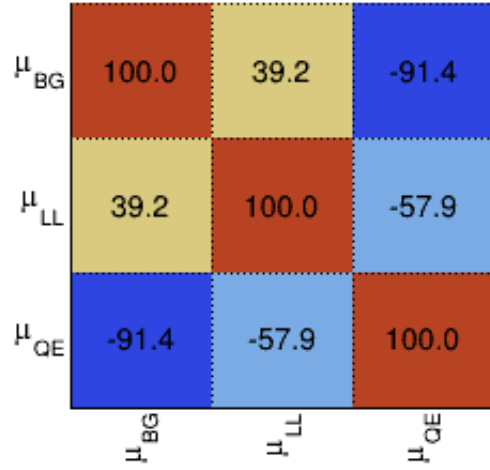
(f) Background scaling 0.05
