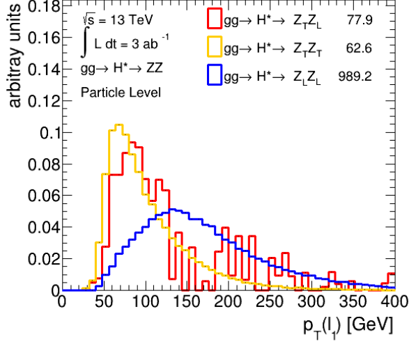
(a) p_T(\ell_1)
