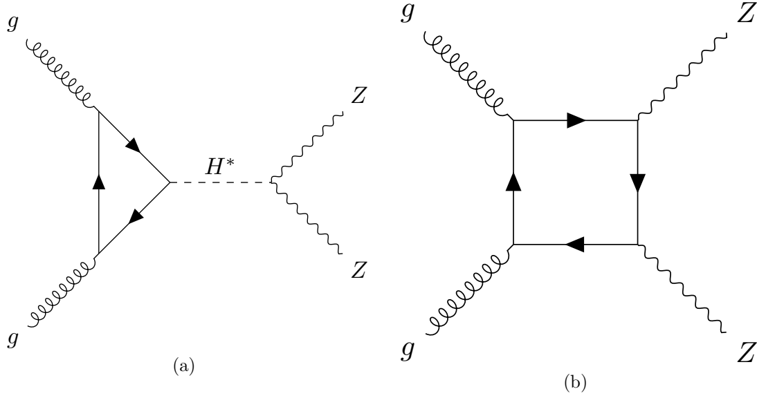
Figure 4.2.: The leading-order Feynman diagrams for the gg \rightarrow ZZ channel [61]. (a) is the gg \rightarrow H^* \rightarrow ZZ signal process and (b) the gg \rightarrow ZZ background process.
