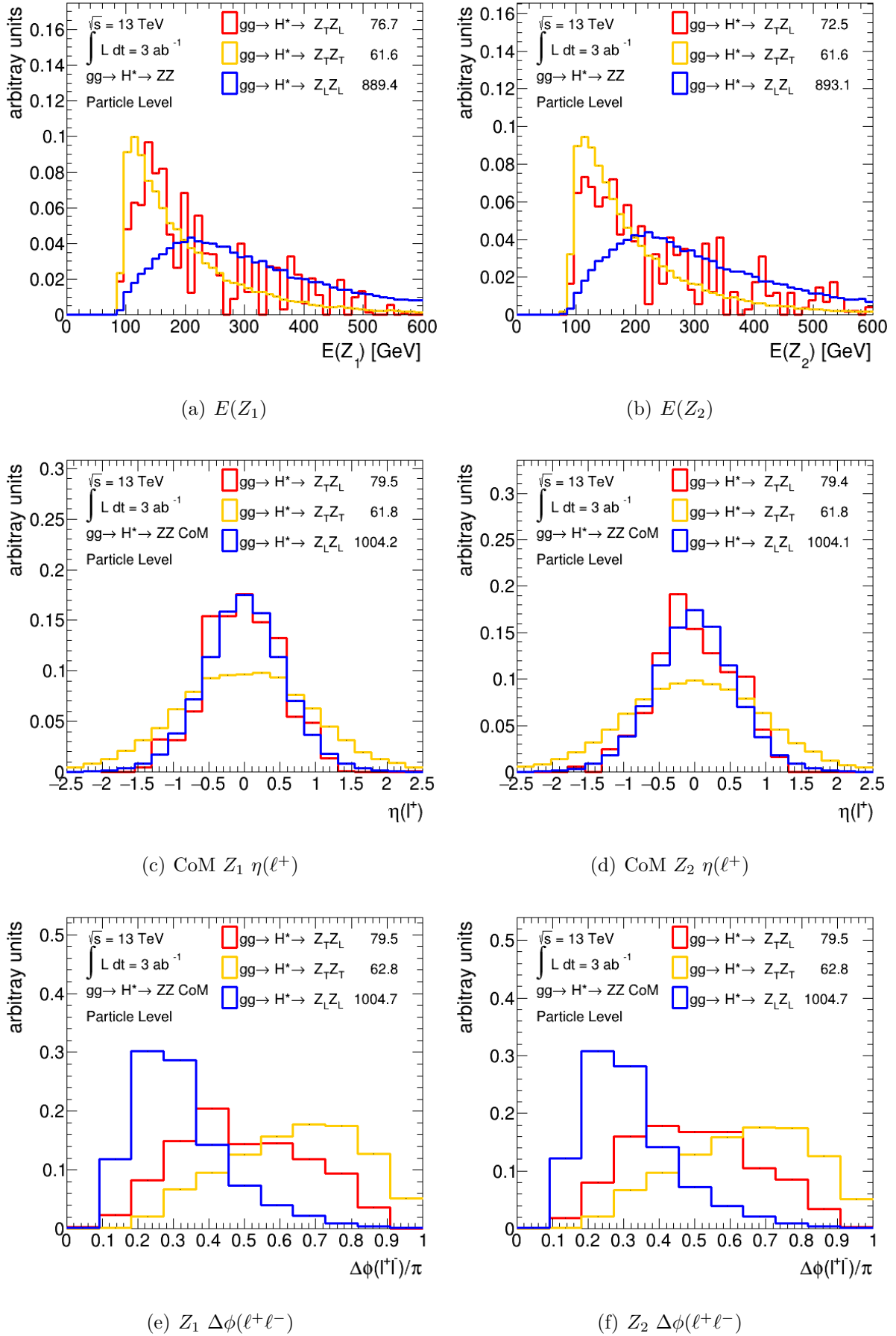
Figure B.10.: Distribution of E(Z_i) , CoM Z_i \eta(\ell^+) , and Z_i \Delta\phi(\ell^+\ell^-) .
