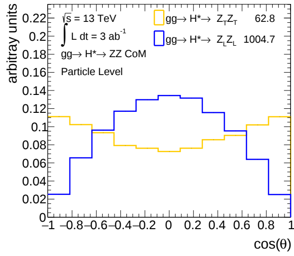
Figure A.10.: \cos(\theta) of the positive lepton emitted by Z_1 in the Z_1 centre-of-mass frame.
