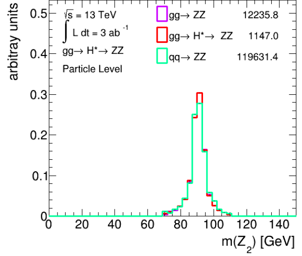
(b) m(Z_2)
