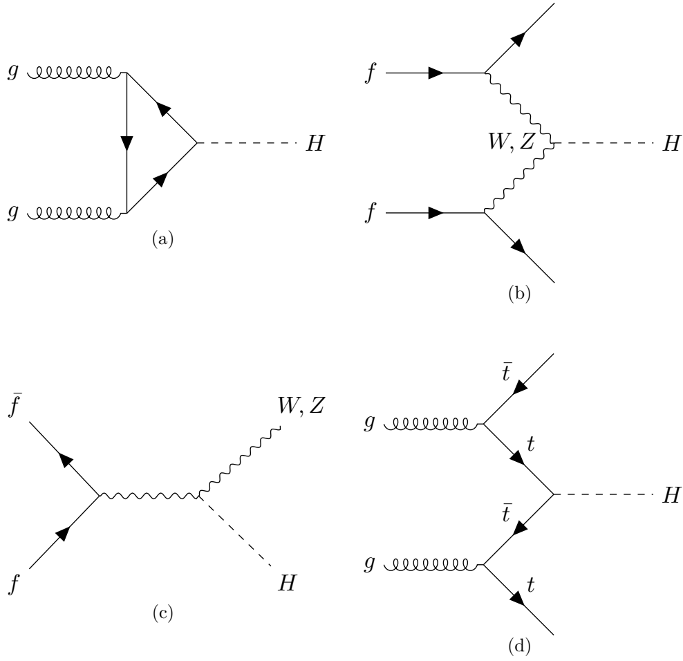
Figure 2.4.: Feynman diagrams for the leading order processes of the Higgs production (a) gluon fusion (ggF), (b) vector boson fusion (VBF), (c) Higgs Strahlung (WH and ZH); and, (d) top fusion (ttH) at the LHC at \sqrt{s} = 13 TeV [1].
