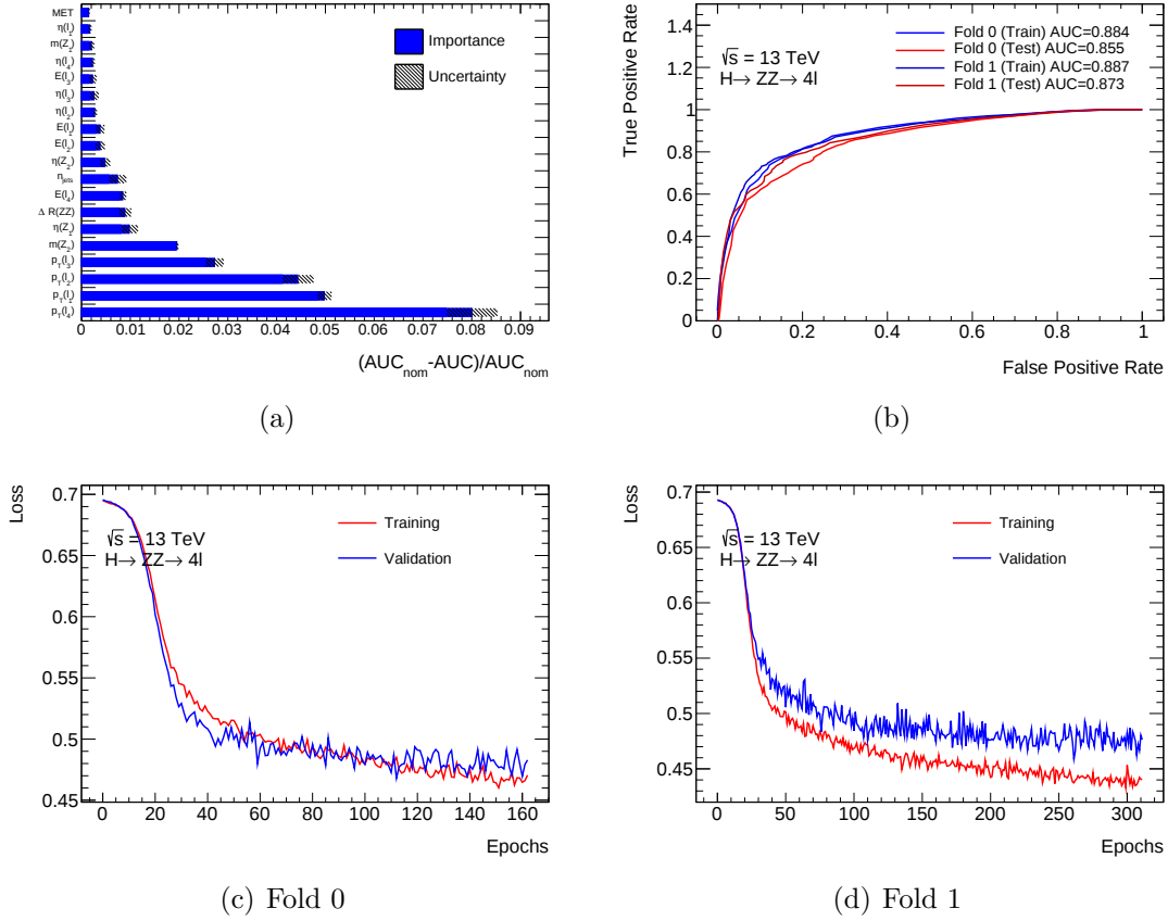
Figure 6.2.: Evaluation plots for the DNN of O_{NN}^{HZZ} . Figure (a) shows the permutation importance of the input variables, which is a measure of the contribution of this variable to the output calculated by the DNN. Figure (b) shows the ROC curves for validation and training for the two folds. Figure (c) and (d) show the loss value over the course of the training of the DNN for the two folds.
