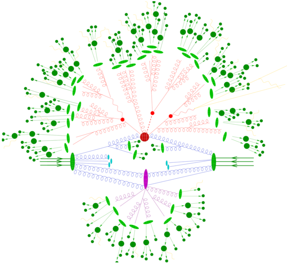
Figure 4.1.: Schematic depiction of a decay cascade involving hadronic interaction at different energy scales [55].
