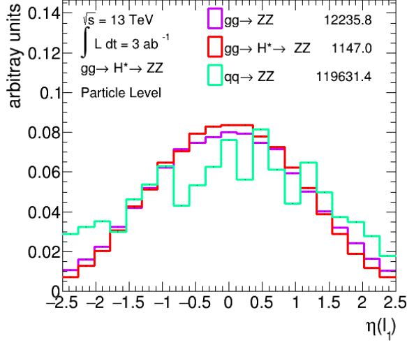
(a) \eta(l_1)
