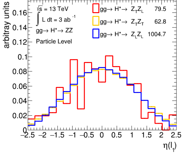
(a) \eta(\ell_1)
