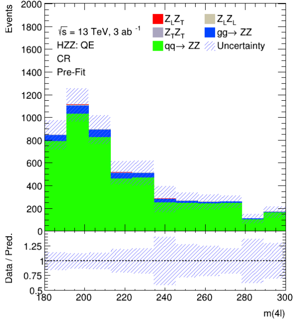
(a) Control Region
