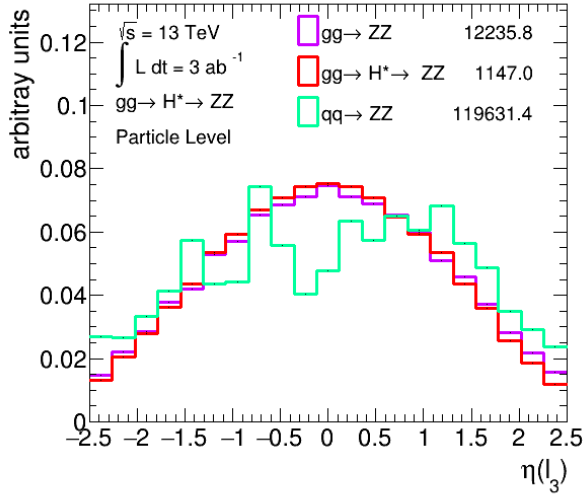
(c) \eta(l_3)
