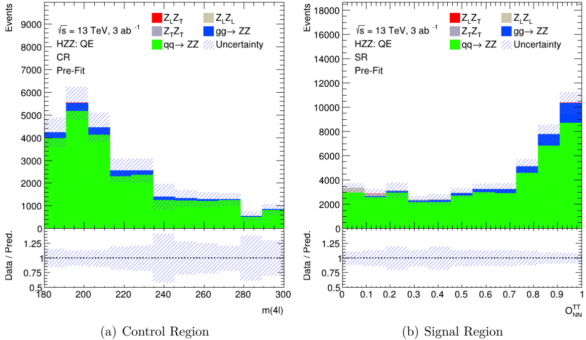
Figure A.3.: Plots of signal and control region with background scaling 0.50.
