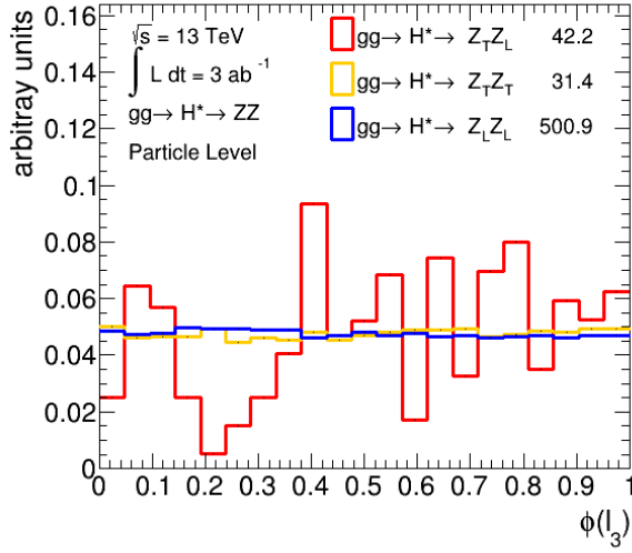
(c) \phi(\ell_3)
