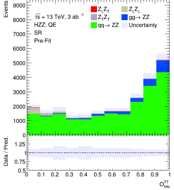
(b) Signal Region
