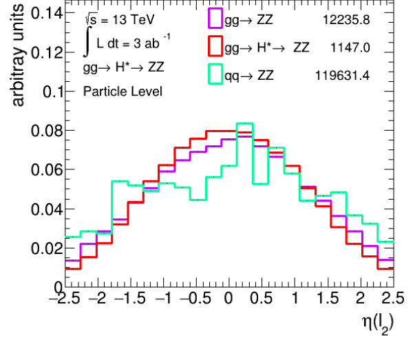
(b) \eta(l_2)
