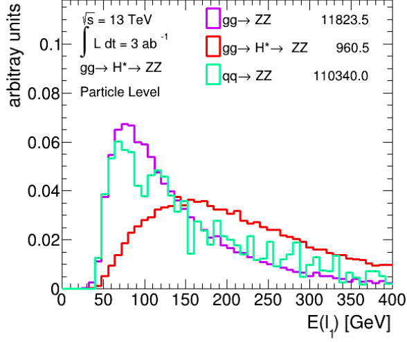
(a) E(\ell_1)
