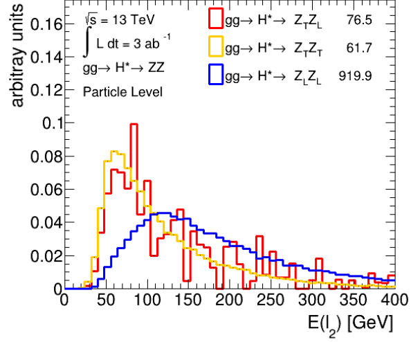
(b) E(\ell_2)
