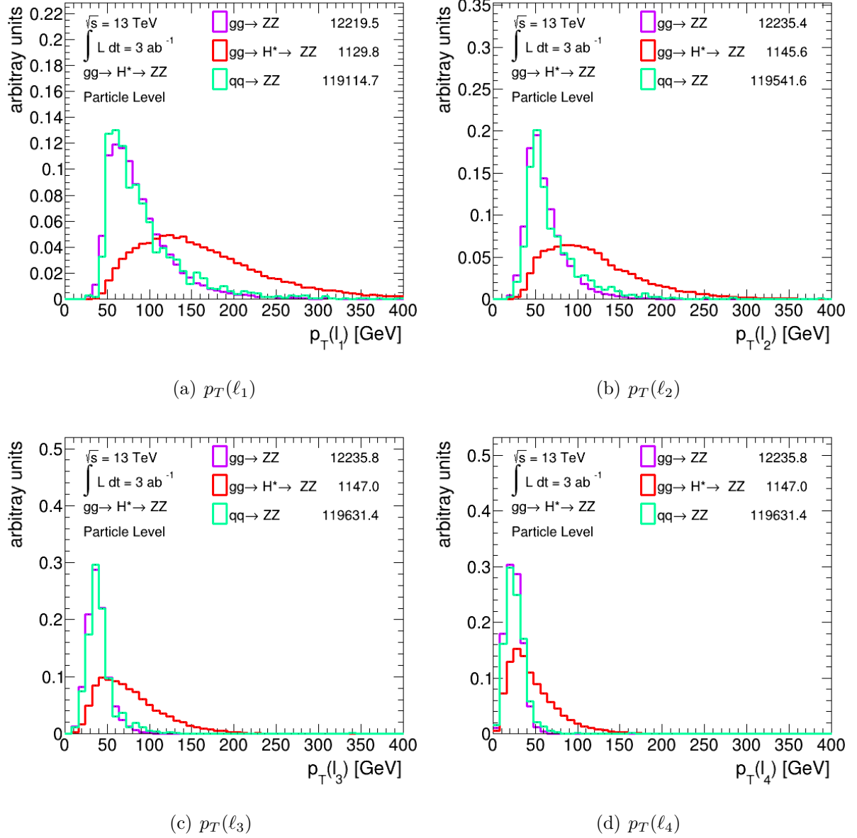
Figure B.1.: Distribution of p_T(\ell_i) .
