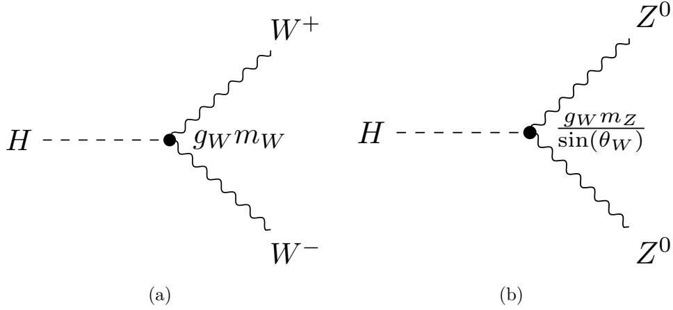
Figure 2.3.: Interaction vertices for the coupling of the Higgs boson to the (a) W boson; (b) Z^0 bosons.
