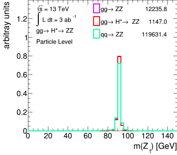
(a) m(Z_1)
