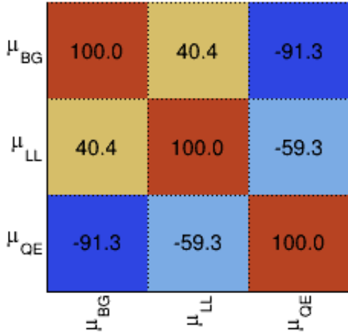
(e) Background scaling 0.10
