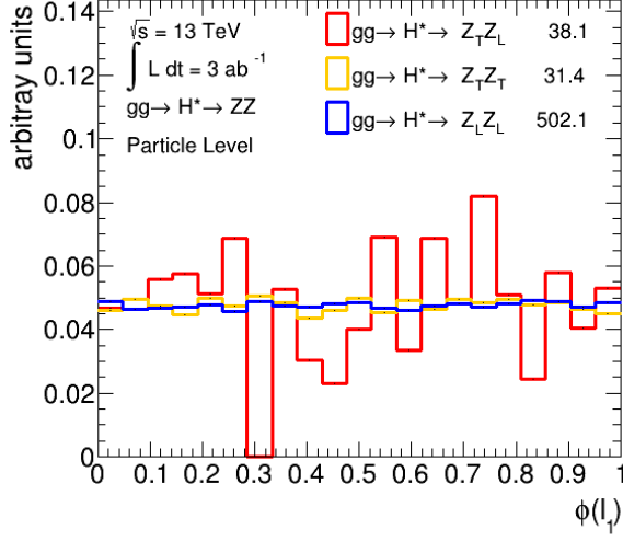
(a) \phi(\ell_1)
