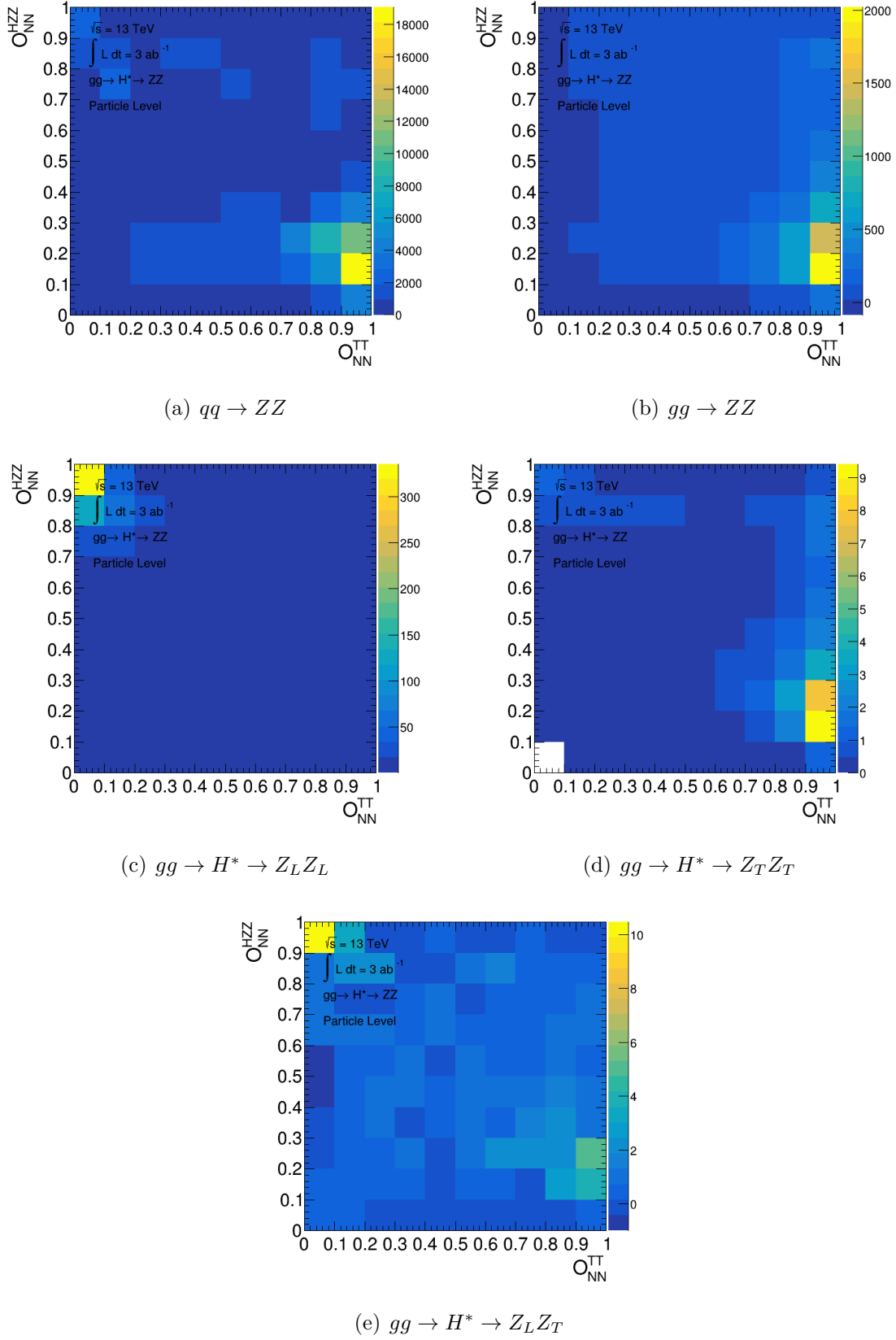
Figure 6.6.: Plots showing the distribution of the two DNN output variables for the different decay channels and background processes.
