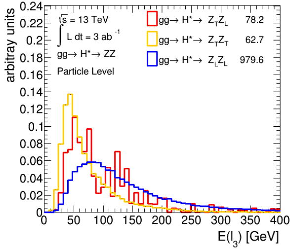
(c) E(\ell_3)
