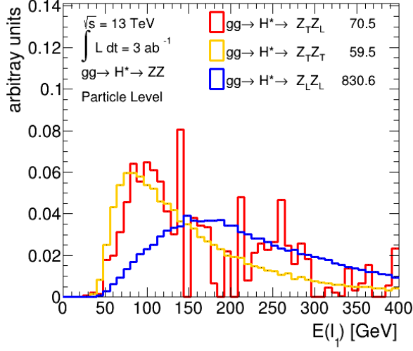
(a) E(\ell_1)
