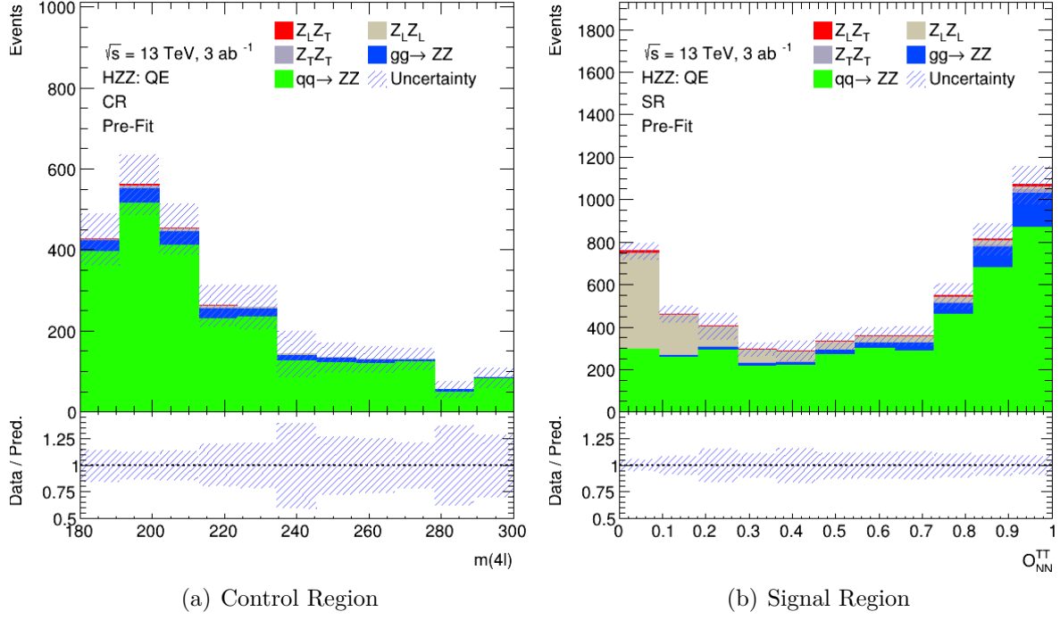
Figure A.6.: Plots of signal and control region with background scaling 0.05.
